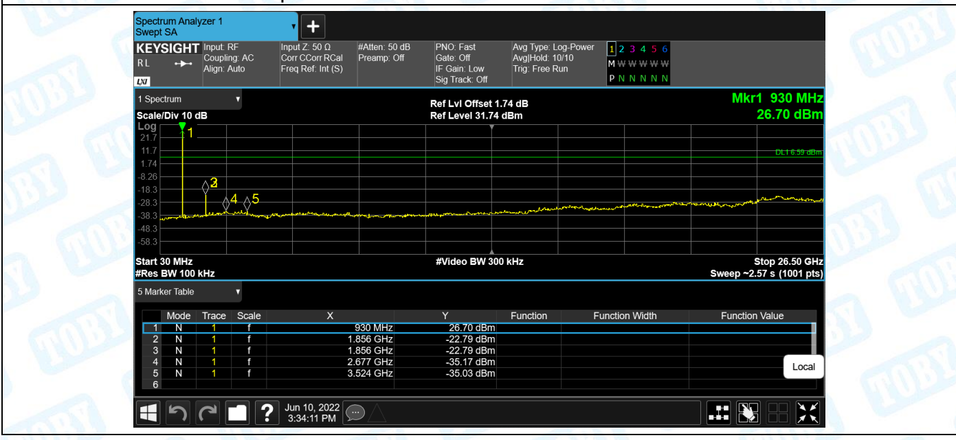
Tx. Spurious NVNT LoRa 923.3MHz Ant1 Emission
