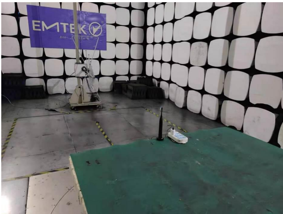
Spurious Emission Test Setup (Below 1000MHz)
