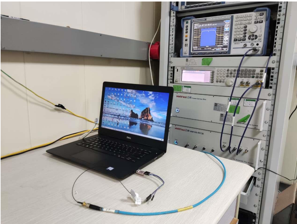
Photo of RF connect test
