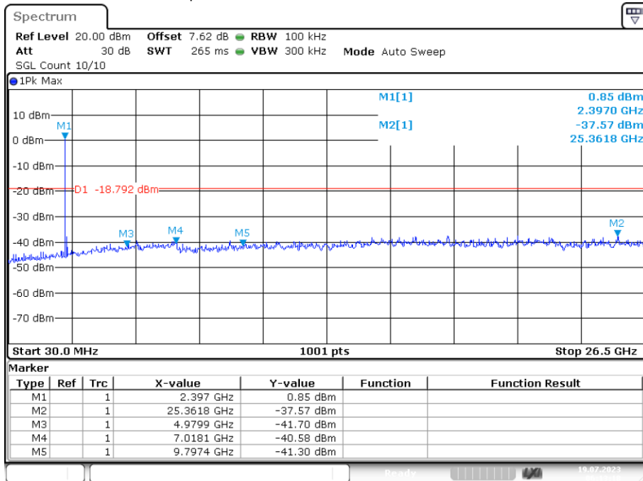
Tx. Spurious NVNT GFSK 2402MHz Ant1 Emission
