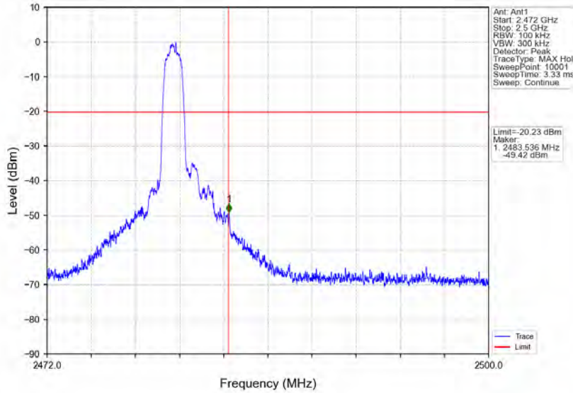
Pi/4DQPSK_2DH5_HCH_2480MHz_Ant1_NTNV
