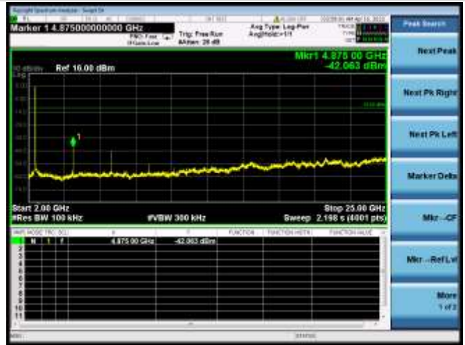
802.11b MIDDLE CHANNEL, SPURIOUS 2 GHz ~ 25 GHz
