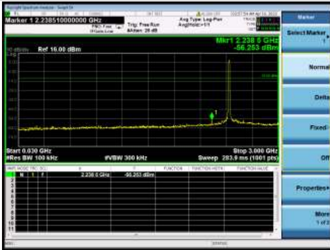
802.11b MIDDLE CHANNEL, SPURIOUS 30 MHz ~ 3 GHz
