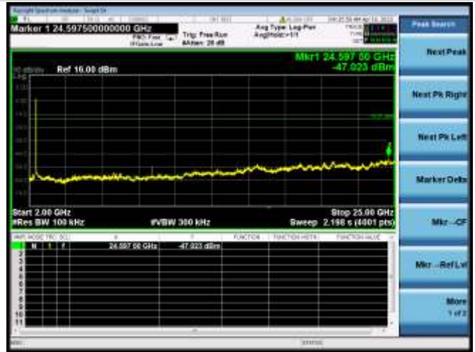
802.11n-20 MHz MIDDLE CHANNEL, SPURIOUS 2 GHz ~ 25 GHz
