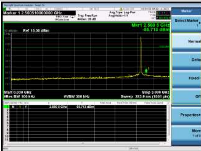
802.11b HIGH CHANNEL, SPURIOUS 30 MHz ~ 3 GHz
