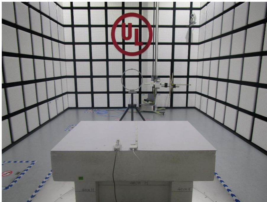
RADIATED RF MEASUREMENT SETUP (Below 30MHz) for NFC
