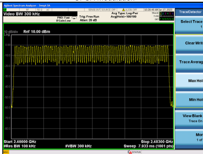
π/4DQPSK Modulation
