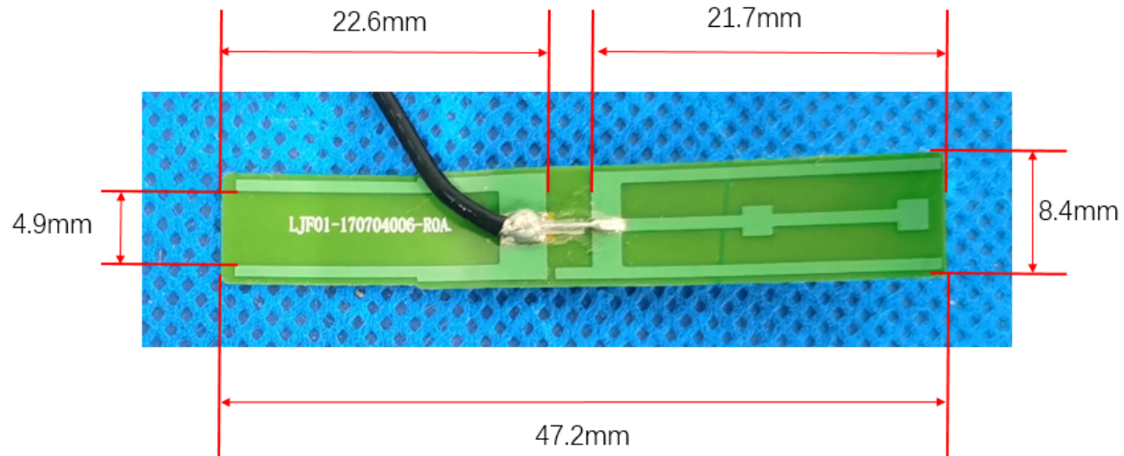
Antenna Photo & Length (mm)
