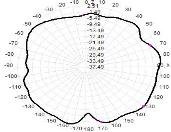
MHz Total(E1-XZ), Max= 2.51dBi
