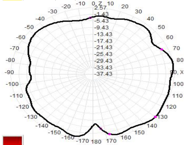
MHz Total(E1-XZ), Max= 2.57dBi
