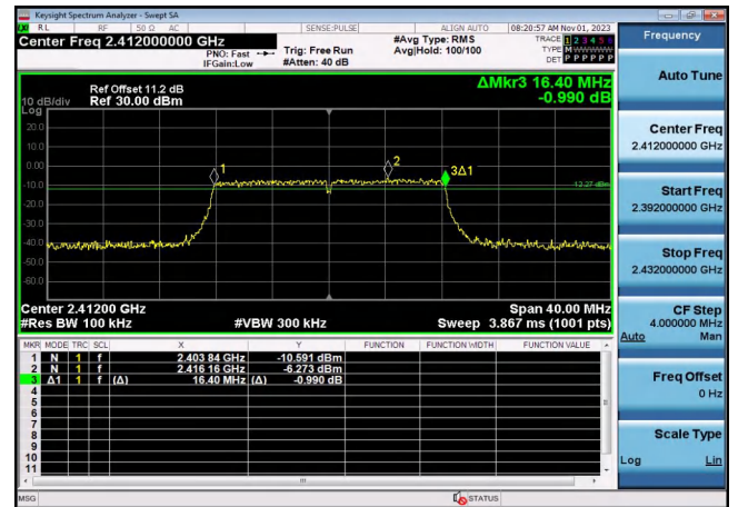
802.11g
