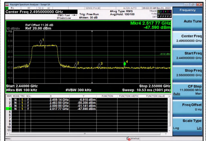
Right bandedge
