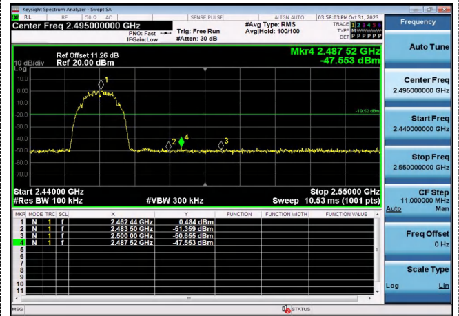
Right bandedge
