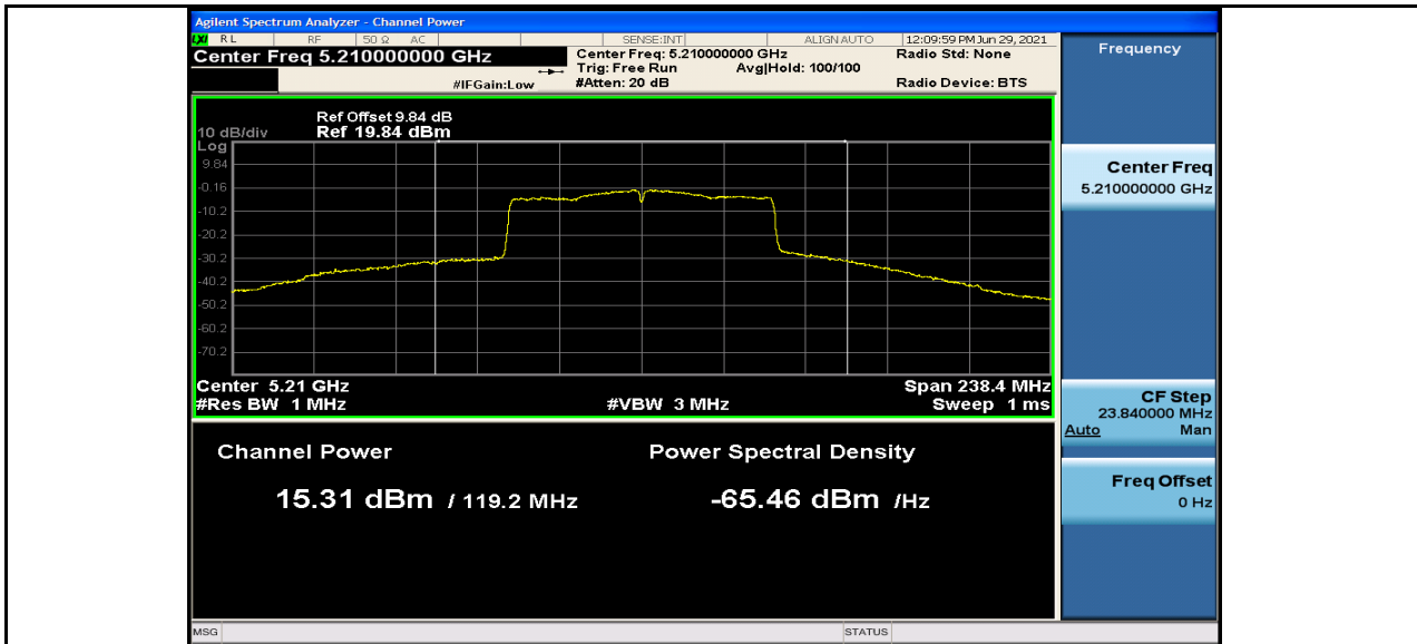
Maximum Conduct Output Power_11AC80_5290_Ant1
