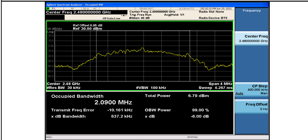
Occupied Bandwidth_BLE_2480_2M
