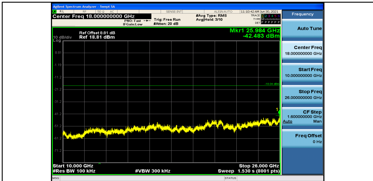
RF Conducted Spurious Emissions_DH5_2441
