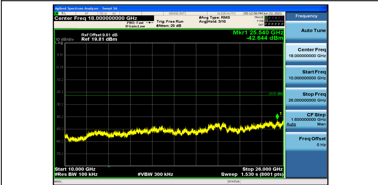
RF Conducted Spurious Emissions_BLE_2440_2M
