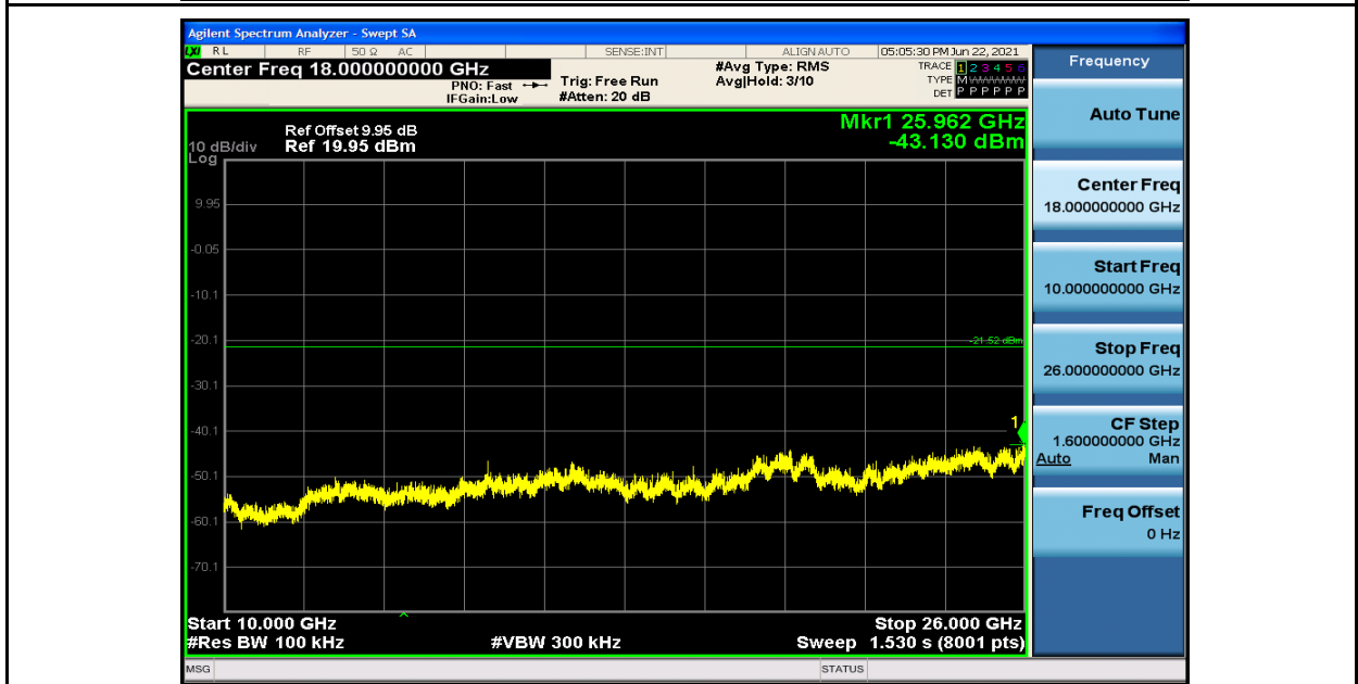
RF Conducted Spurious Emissions_BLE_2480_1M
