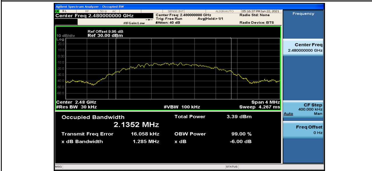
Occupied Bandwidth_BLE_2480_2M
