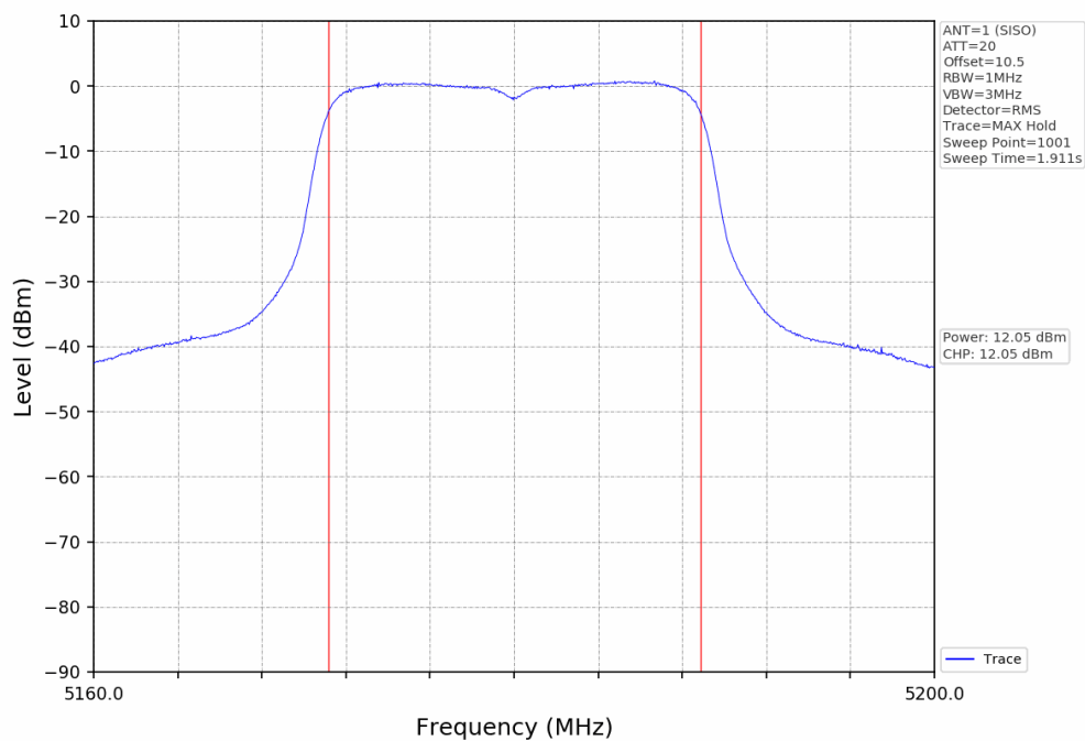
Maximum Conducted Outpower NTNV_802.11ac(VHT20)_SISO_5180MHz_ANT1
