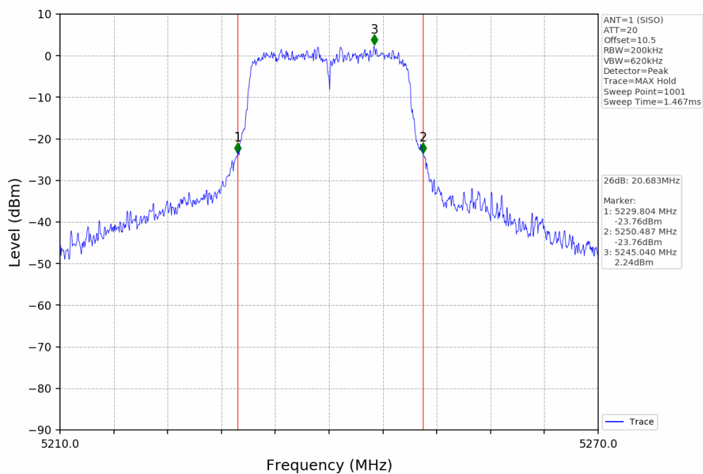
Bandwidth NTNV_802.11n(HT20)_SISO_5240MHz_ANT1
