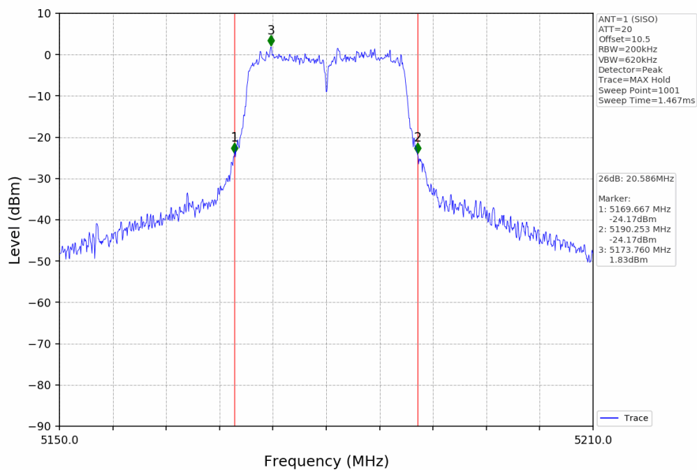
Bandwidth NTNV_802.11ac(VHT20)_SISO_5180MHz_ANT1
