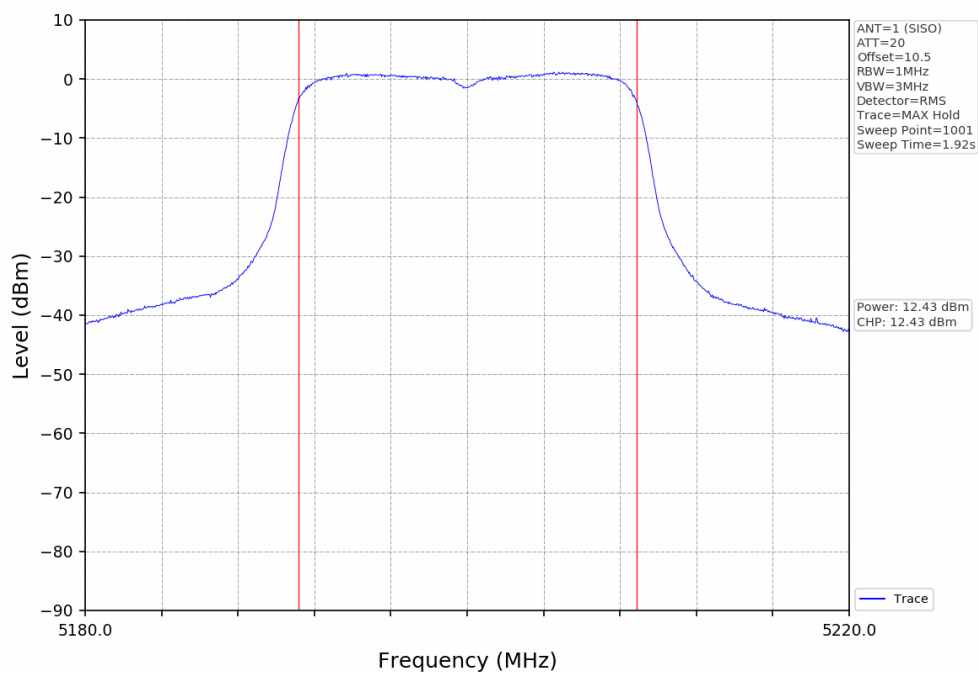
Maximum Conducted Outpower NTV 802.11ac(VHT20) SISO 5200MHz ANT1
