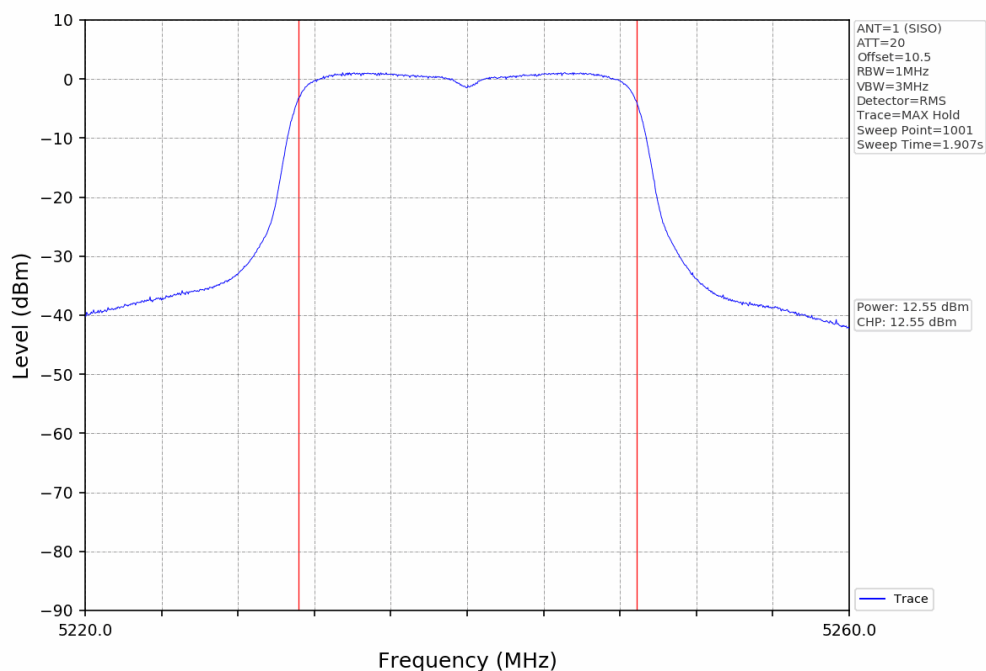
Maximum Conducted Outpower NTNV_802.11n(HT20)_SISO_5240MHz_ANT1
