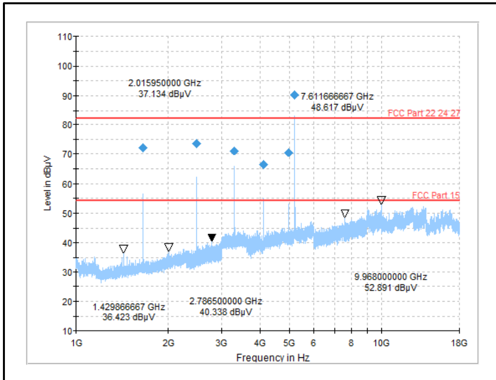
WLAN 5 GHz Mode/ UNII-1 / 802.11a / 20 MHz / PWR 12 / Bottom Channel / 6 Mbps + LTE /B5/Bottom Channel
