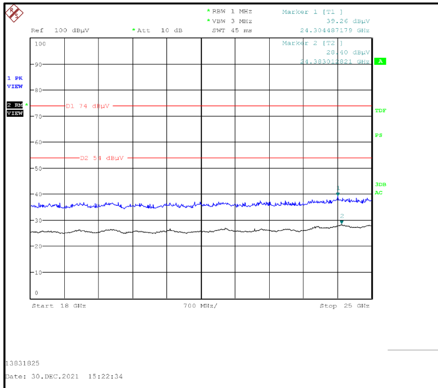
Plot: 18 GHz – 25 GHz: BT-LE Mode/1 Mbps/PRBS9/PWR MAX /Bottom Channel +LTE /B2/Bottom Channel
