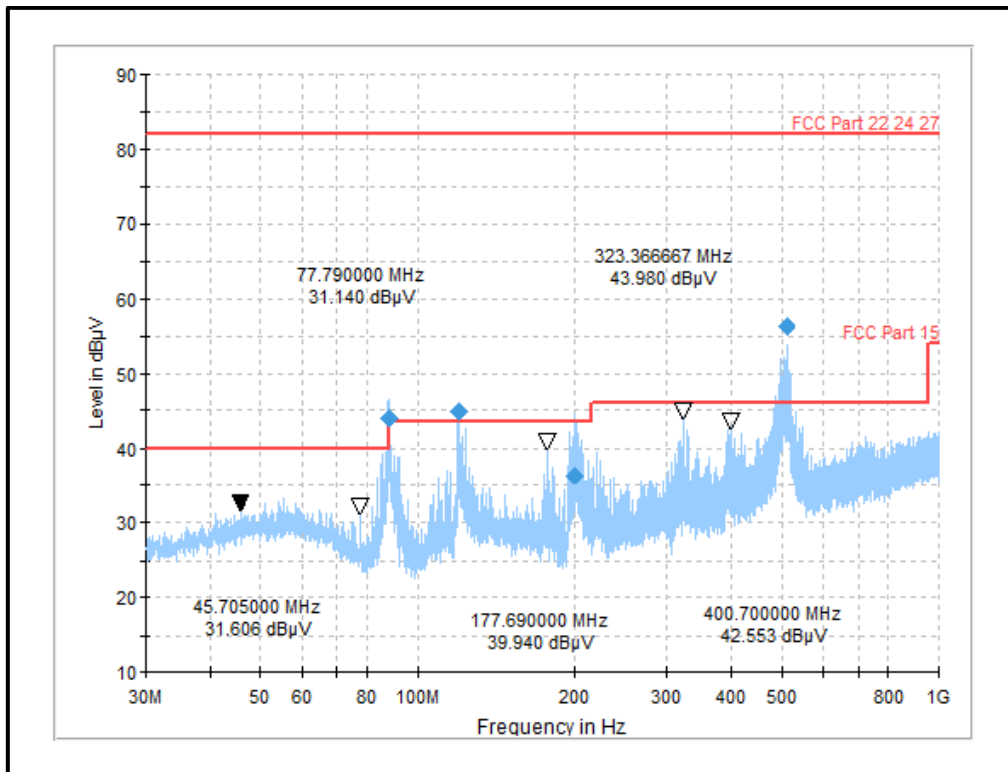
Plot: 30 MHz – 1 GHz: BT-LE Mode/1 Mbps/PRBS9/PWR MAX /Bottom Channel +LTE /B2/Bottom Channel
