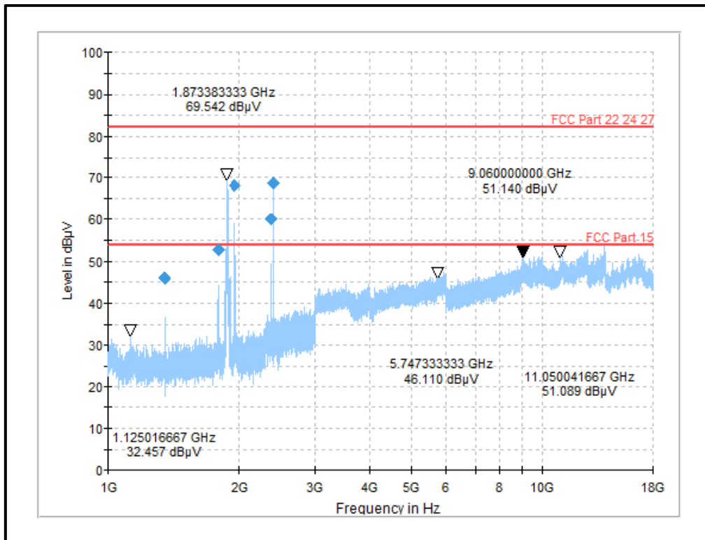
Plot: 1 GHz – 18 GHz : BT-LE Mode/1 Mbps/PRBS9/PWR MAX /Bottom Channel +LTE /B2/Bottom Channel
