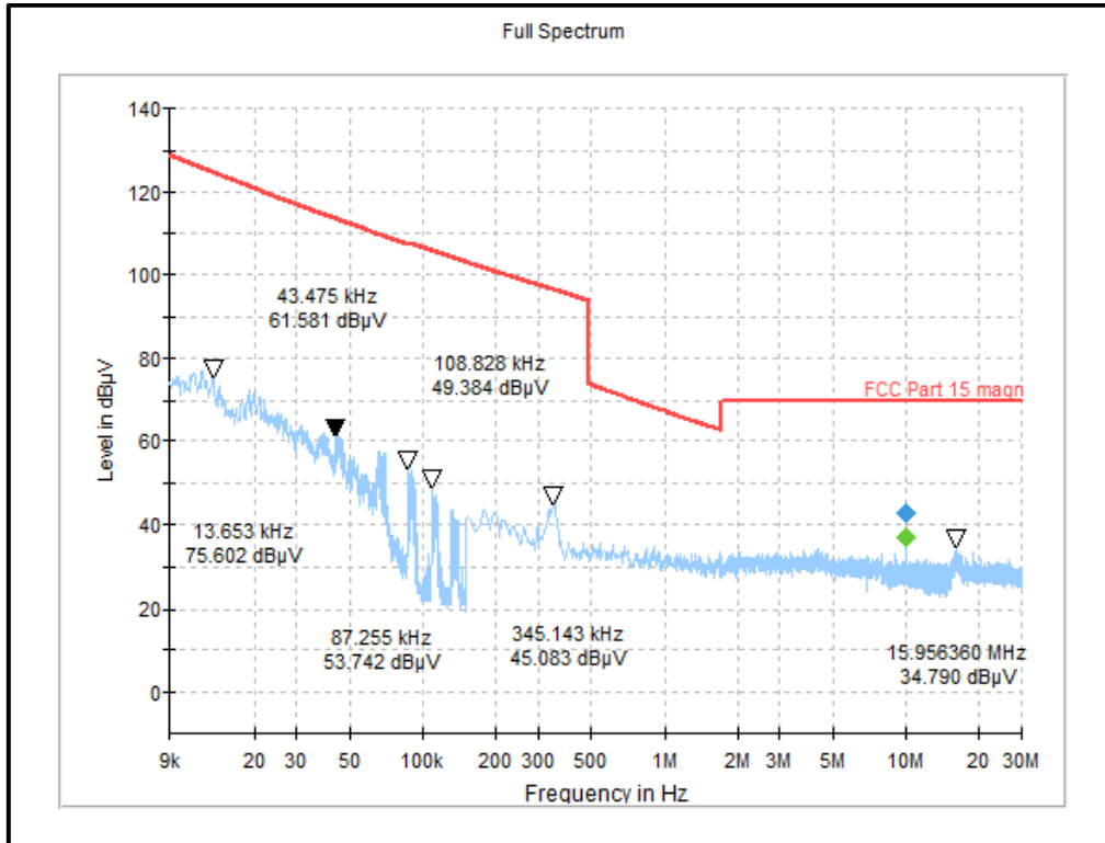
Plot: 9 kHz – 30 MHz: BT-LE Mode/1 Mbps/PRBS9/PWR MAX /Bottom Channel +LTE /B2/Bottom Channel
