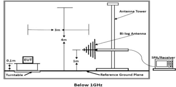
Figure 2. 30MHz to 1GHz
