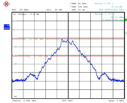
GFSK_Middle 0.880 MHz
