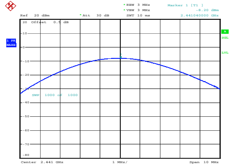
PI/4-DQPSK_Middle -8.20 dBm
