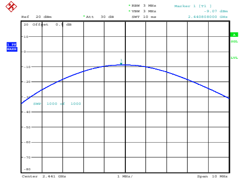
GFSK_Middle -9.07 dBm
