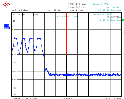
GFSK_Hopping_Upper 41.98 dB
