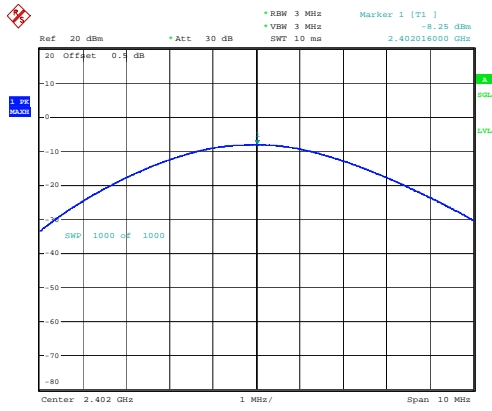
PI/4-DQPSK_Low -8.25 dBm
