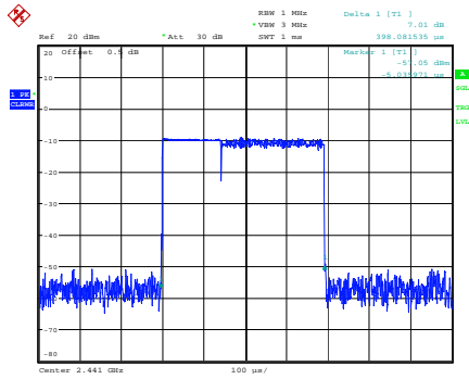
PI/4-DQPSK_Hopping_2DH1 0.398ms
