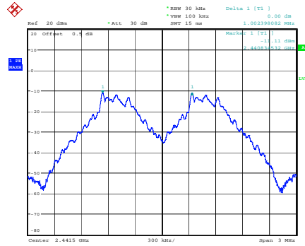
GFSK_Middle 1.002 MHz
