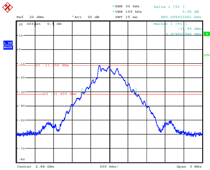
GFSK_High 0.880 MHz
