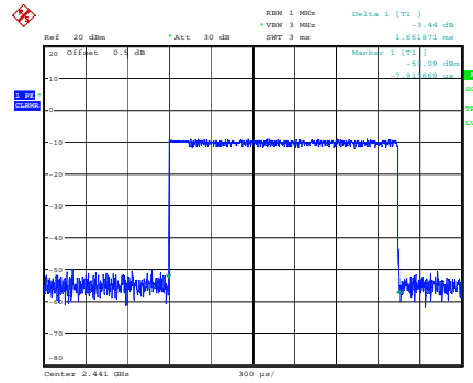
PI/4-DQPSK_Hopping_2DH3 1.662ms
