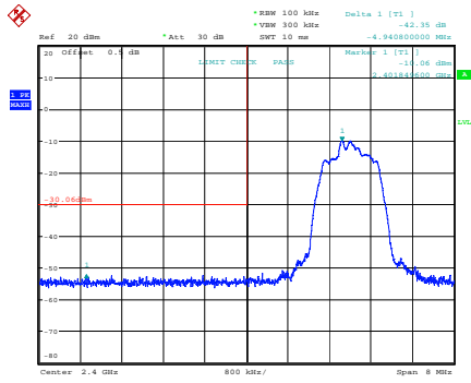
PI/4-DQPSK_Low 42.35 dB
