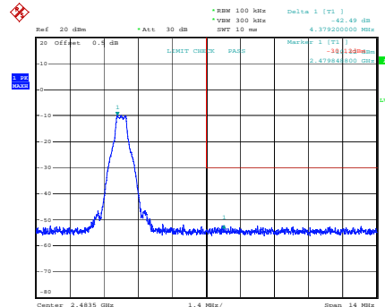
GFSK_High 42.49 dB
