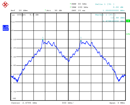
GFSK_High 1.000 MHz
