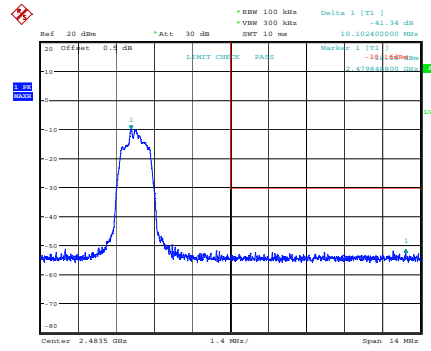
PI/4-DQPSK_High 41.34 dB
