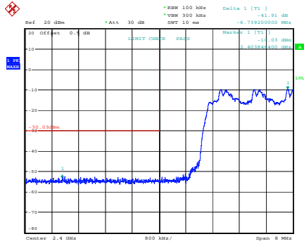
PI/4-DQPSK_Hopping_Lower 41.91 dB
