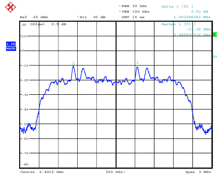
PI/4-DQPSK_Middle 1.002 MHz
