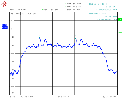
PI/4-DQPSK_High 1.000 MHz
