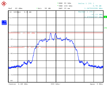
PI/4-DQPSK_High 1.247 MHz
