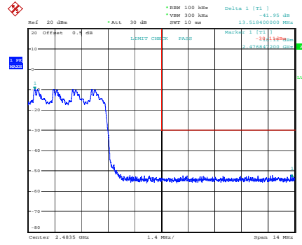
PI/4-DQPSK_Hopping_Upper 41.95 dB
