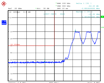
GFSK_Hopping_Lower 42.23 dB
