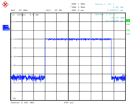
PI/4-DQPSK_Hopping_2DH5 2.910ms
