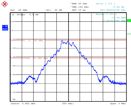
GFSK_Low 0.882 MHz
