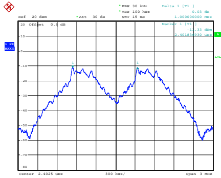
GFSK_Low 1.000 MHz
