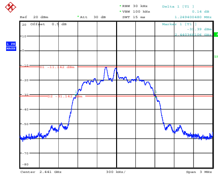
PI/4-DQPSK_Middle 1.249 MHz
