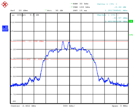
PI/4-DQPSK_Low 1.252 MHz
