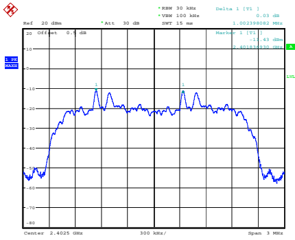
PI/4-DQPSK_Low 1.002 MHz
