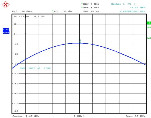
GFSK_High -9.41 dBm
