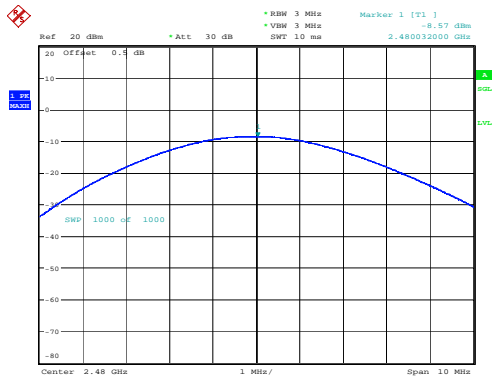
PI/4-DQPSK_High -8.57 dBm
