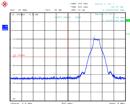
GFSK_Low 42.27 dB
