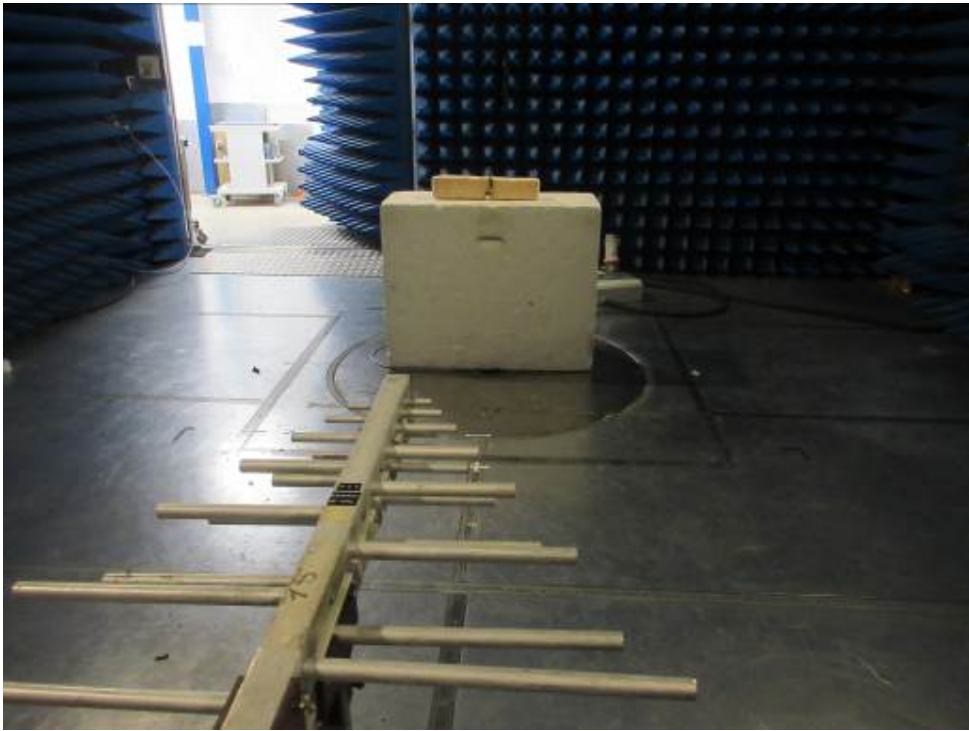
TEST SETUP PHOTO(S) RADIATED EMISSIONS (300MHz>F>1GHz)
