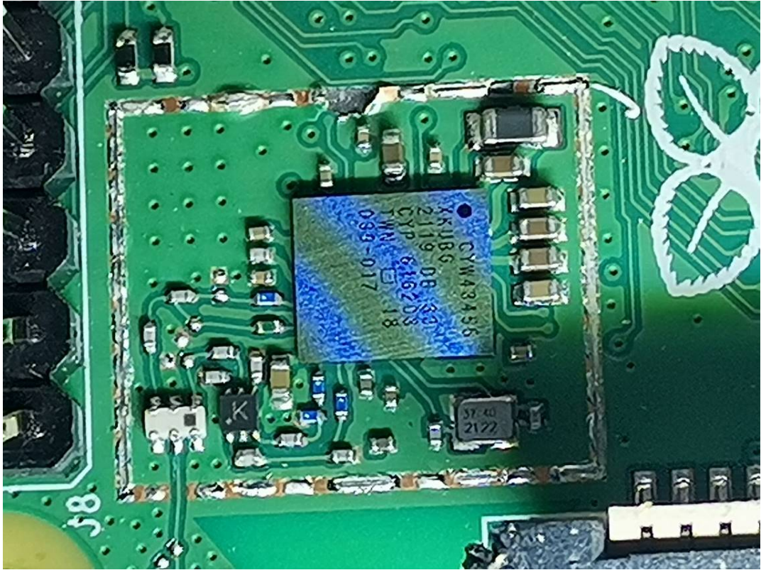
Wi-Fi/BLE Chip
