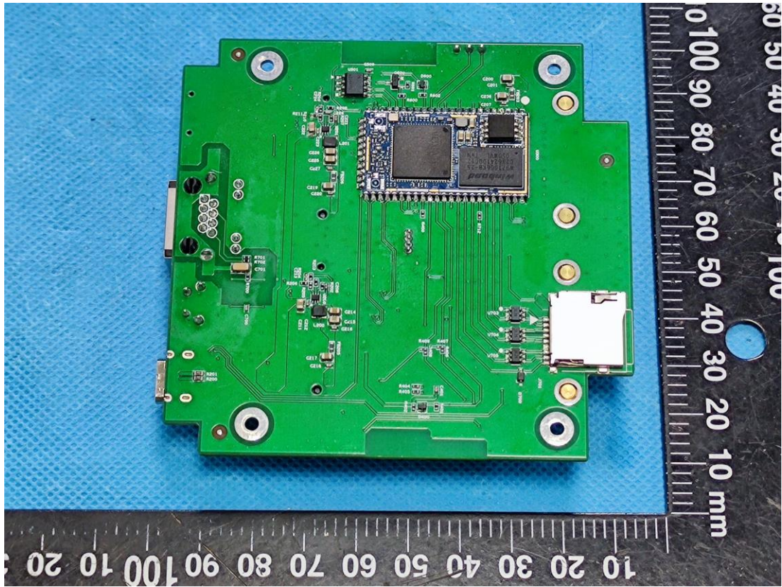
Wi-Fi chip
