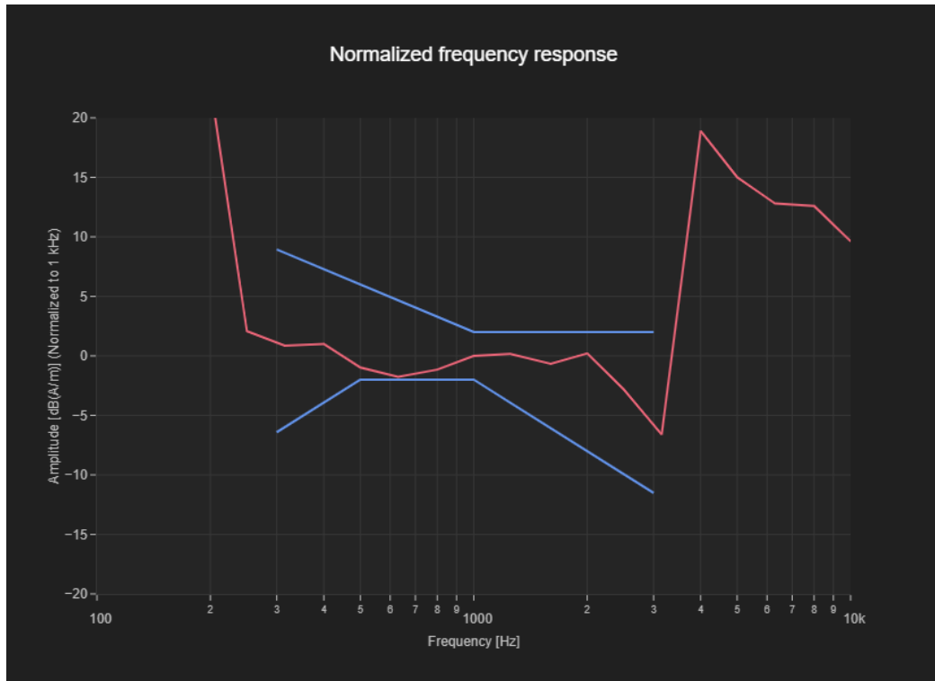
Figure C.1 Frequency Response of B30-N77
