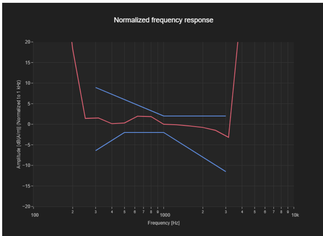
Figure C.2 Frequency Response of Band30-OTT
