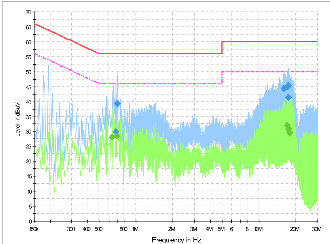
Fig.B.10.2 AC Powerline Conducted Emission-Idle
