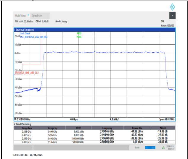
1-N41-30-40-L-3-DFT-PI2BPSK-Outer_Full-100@0-Ant3-1--PASS-see graph
