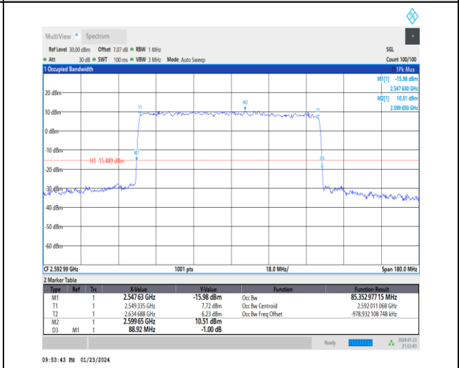
1-N41-30-90-M-1-DFT-QPSK-Outer_Full-240@0-Ant 3-85.353-88.920-<=90-PASS
