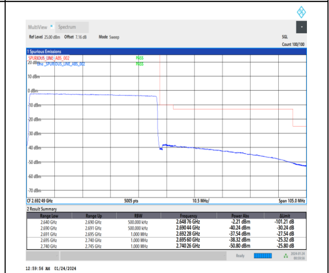
1-N41-30-50-H-6-CP-QPSK-Outer_Full-133@0-Ant3-1--PASS-see graph
