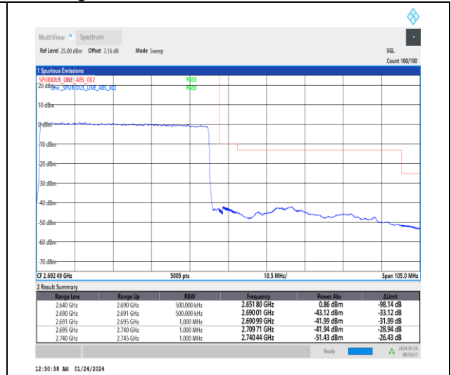
1-N41-30-50-H-3-DFT-PI2BPSK-Outer_Full-128@0-Ant3-1--PASS-see graph
