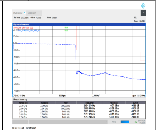
1-N41-30-60-H-3-DFT-PI2BPSK-Outer_Full-162 @ 0-Ant3-1--PASS-see graph
