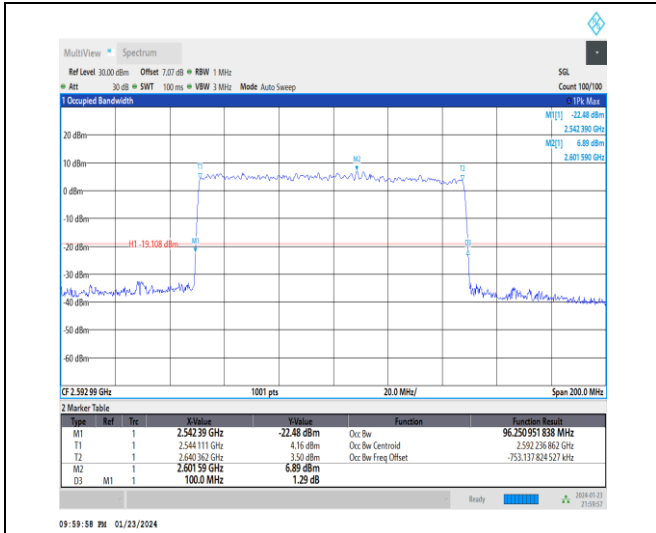
1-N41-30-100-M-5-DFT-256QAM-Outer_Full-270@0-Ant3-96.251-100.000-≤100-PASS
