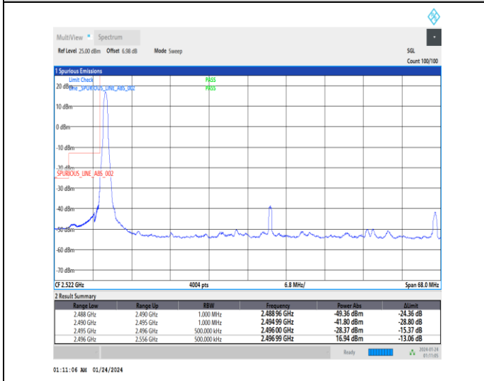
1-N41-30-60-L-4-CP-QPSK-Edge_1RB_Left-1@0-Ant3-1--PASS-see graph
