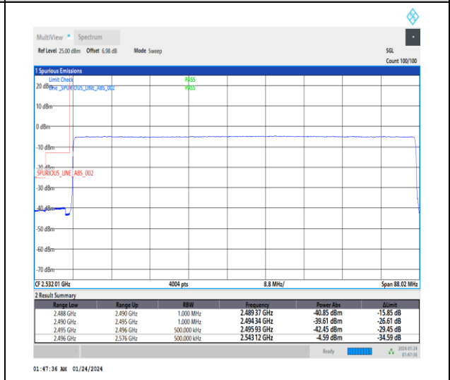
1-N41-30-80-L-6-CP-QPSK-Outer_Full-217@0-Ant3-1--PASS-see graph
