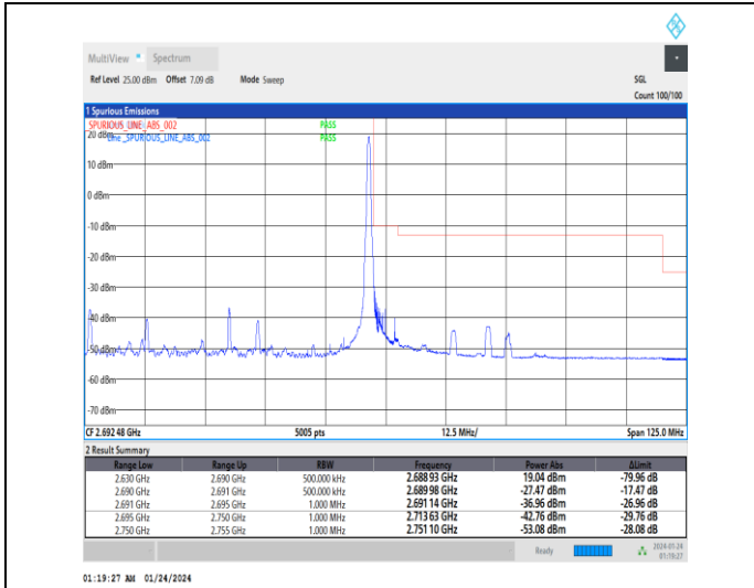
1-N41-30-60-H-2-DFT-PI2BPSK-Edge_1RB_Right-1 @ 161-Ant3-1--PASS-see graph
