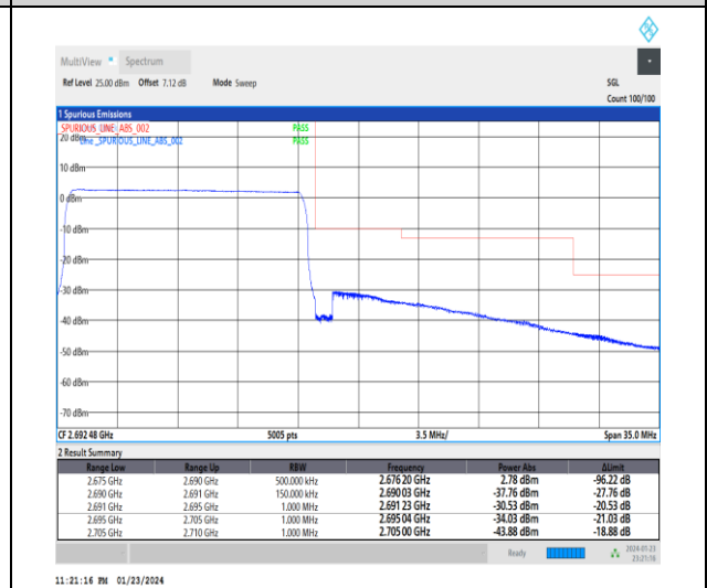
1-N41-30-15-H-6-CP-QPSK-Outer_Full-38@0-Ant3-1--PASS-see graph
