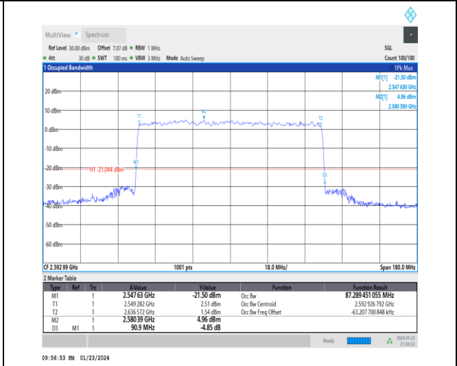
1-N41-30-90-M-9-CP-256QAM-Outer_Full-245@0-Ant3 t3-87.289-90.900-≤90-PASS
