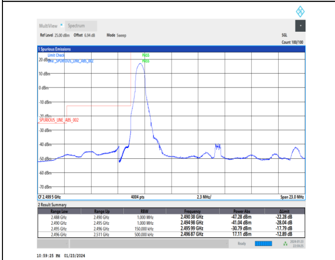
1-N41-30-15-L-4-CP-QPSK-Edge_1RB_Left-1@0-Ant3-1--PASS-see graph
