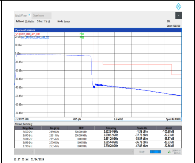
1-N41-30-40-H-6-CP-QPSK-Outer_Full-106@0-A nt3-1--PASS-see graph
