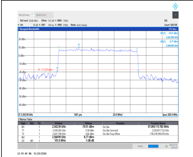
1-N41-30-100-M-7-CP-16QAM-Outer_Full-273@0-A nt3-97.093-101.000-≤100-PASS
