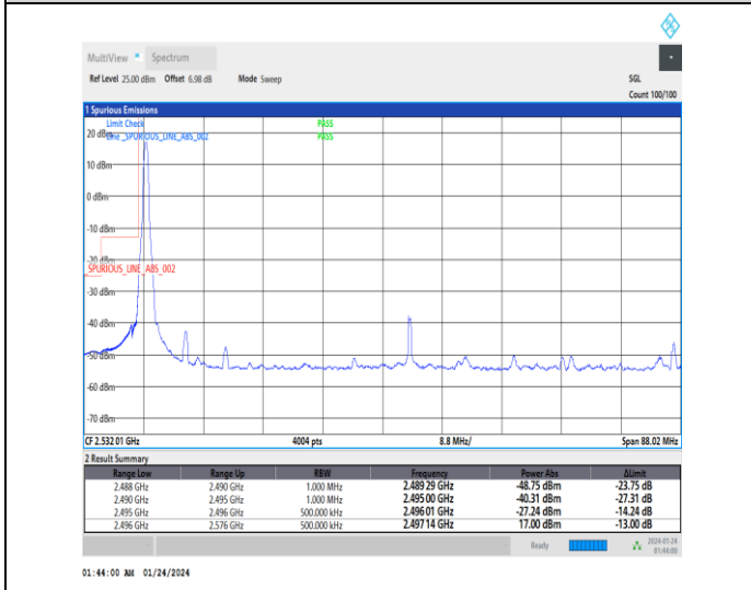
1-N41-30-80-L-4-CP-QPSK-Edge_1RB_Left-1@0-Ant3-1--PASS-see graph
