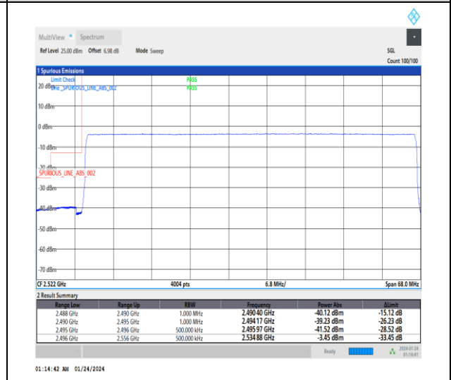
1-N41-30-60-L-6-CP-QPSK-Outer_Full-162@0-Ant3-1--PASS-see graph
