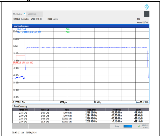
1-N41-30-80-L-3-DFT-PI2BPSK-Outer_Full-216@0-Ant3-1--PASS-see graph
