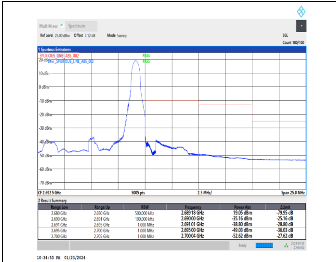
1-N41-30-10-H-2-DFT-PI2BPSK-Edge_1RB_Right-1@23-Ant3-1--PASS-see graph
