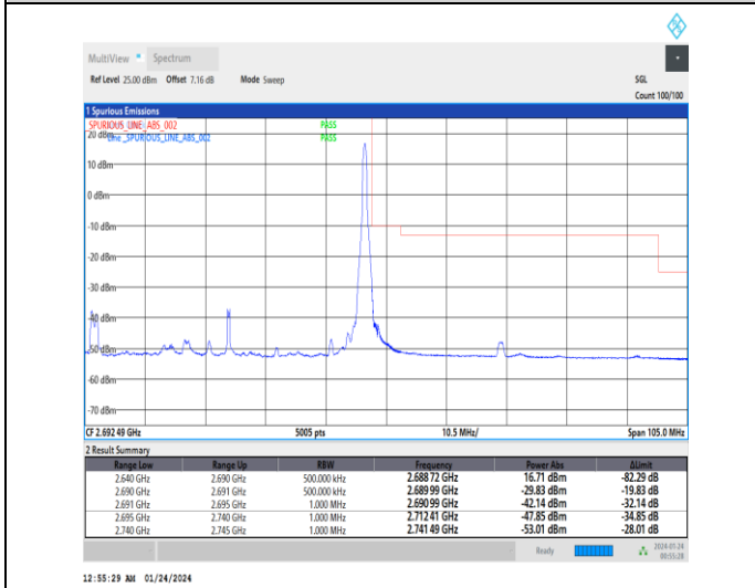
1-N41-30-50-H-5-CP-QPSK-Edge_1RB_Right-1@132-Ant3-1--PASS-see graph
