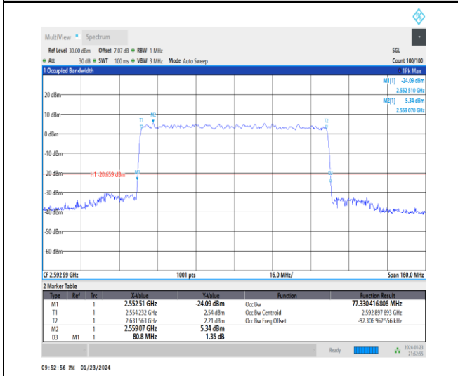
1-N41-30-80-M-9-CP-256QAM-Outer_Full-217@0-A nt3-77.33-80.800-<=80-PASS
