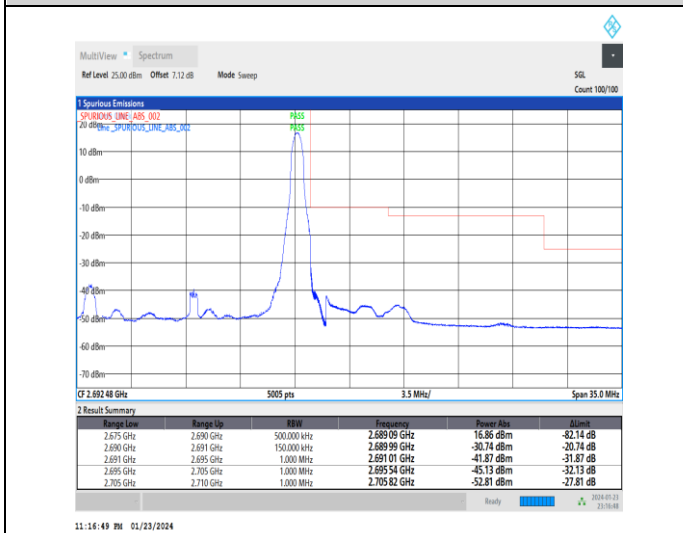
1-N41-30-15-H-5-CP-QPSK-Edge_1RB_Right-1@37-Ant3-1--PASS-see graph
