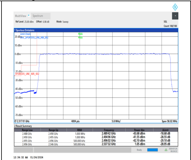
1-N41-30-50-L-3-DFT-PI2BPSK-Outer_Full-128@0-Ant3-1--PASS-see graph
