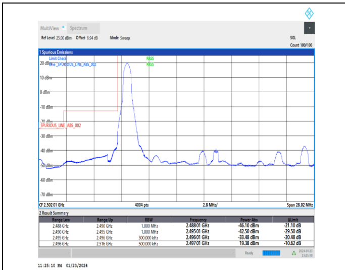
1-N41-30-20-L-1-DFT-PI2BPSK-Edge_1RB_Left-1@0-Ant3-1--PASS-see graph
