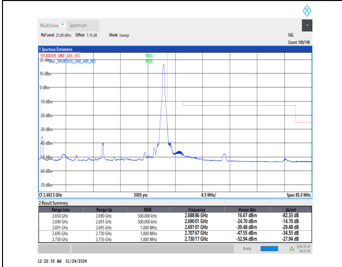
1-N41-30-40-H-5-CP-QPSK-Edge_1RB_Right-1 @ 105-Ant3-1--PASS-see graph
