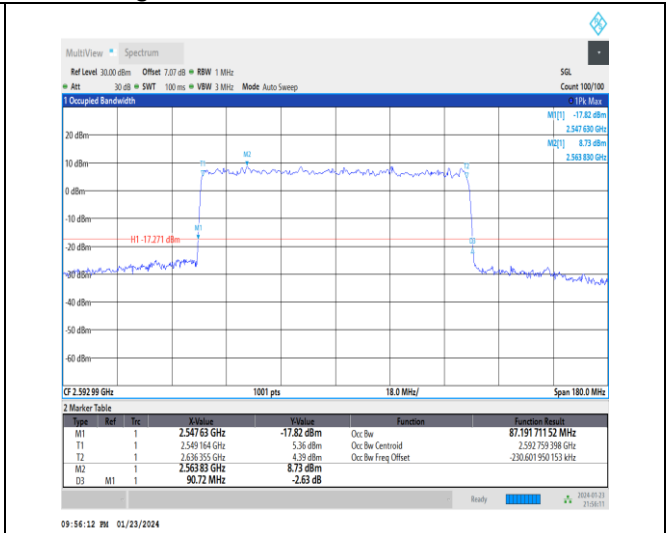
1-N41-30-90-M-7-CP-16QAM-Outer_Full-245@0-Ant3 3-87.192-90.720-≤90-PASS
