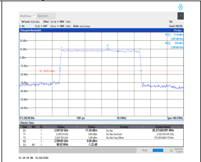
1-N41-30-90-M-3-DFT-16QAM-Outer_Full-240@0-Ant3-85.374-88.920-≤90-PASS
