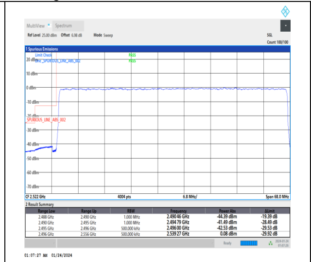
1-N41-30-60-L-3-DFT-PI2BPSK-Outer_Full-162@0-Ant3-1--PASS-see graph
