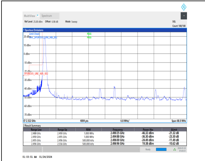
1-N41-30-60-L-1-DFT-PI2BPSK-Edge_1RB_Left-1@0-Ant3-1--PASS-see graph
