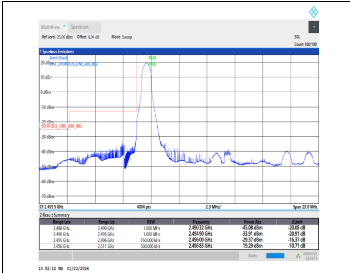
1-N41-30-15-L-1-DFT-PI2BPSK-Edge_1RB_Left-1@0-Ant3-1--PASS-see graph
