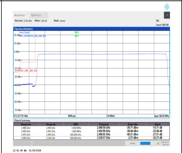
1-N41-30-50-L-6-CP-QPSK-Outer_Full-133@0-Ant3-1--PASS-see graph
