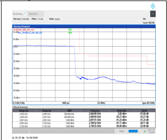
1-N41-30-40-H-3-DFT-PI2BPSK-Outer_Full-100@ 0-Ant3-1--PASS-see graph
