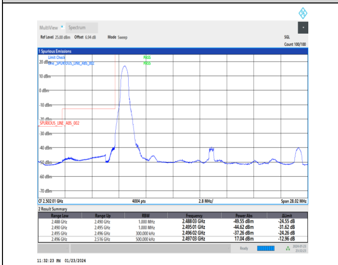
1-N41-30-20-L-4-CP-QPSK-Edge_1RB_Left-1@0-Ant3-1--PASS-see graph
