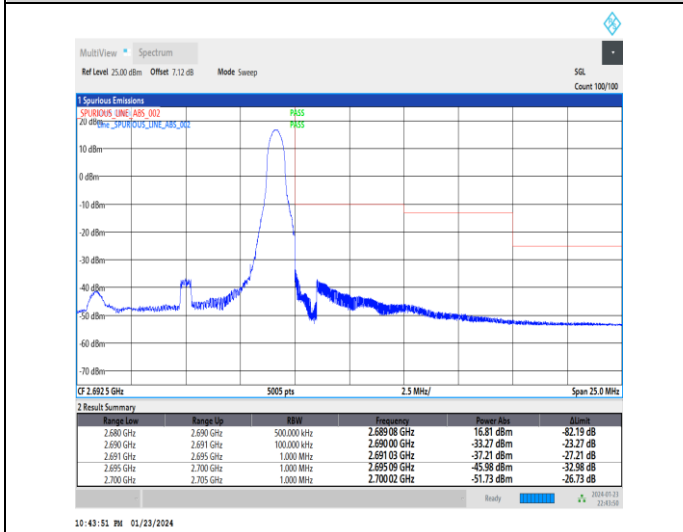
1-N41-30-10-H-5-CP-QPSK-Edge_1RB_Right-1@23-Ant3-1--PASS-see graph
