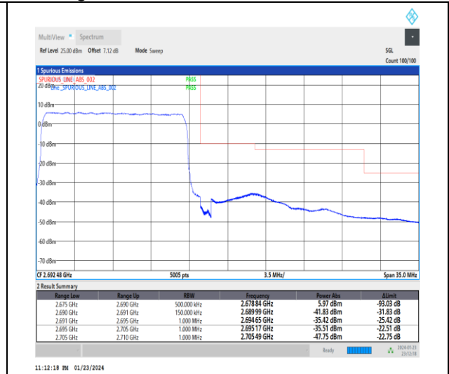
1-N41-30-15-H-3-DFT-PI2BPSK-Outer_Full-36@0-Ant3-1--PASS-see graph
