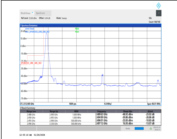
1-N41-30-40-L-4-CP-QPSK-Edge_1RB_Left-1@0-Ant3-1--PASS-see graph
