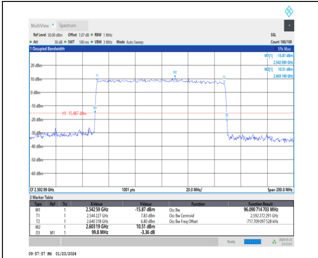
1-N41-30-100-M-1-DFT-QPSK-Outer_Full-270@0-Ant3-96.091-99.800-≤100-PASS
