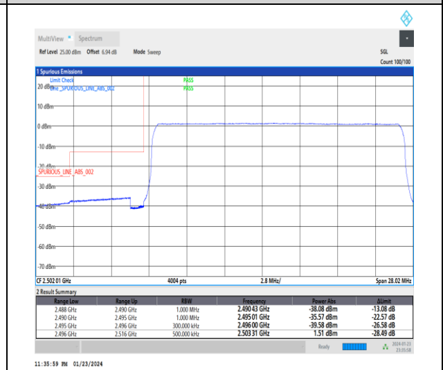
1-N41-30-20-L-6-CP-QPSK-Outer_Full-51@0-Ant3-1--PASS-see graph
