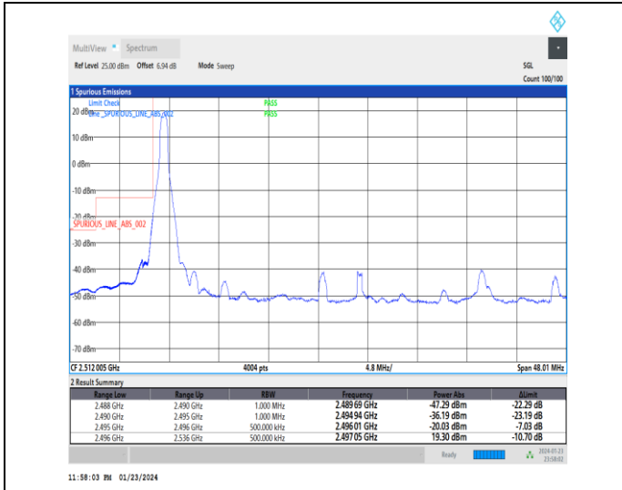
1-N41-30-40-L-1-DFT-PI2BPSK-Edge_1RB_Left-1@0-Ant3-1--PASS-see graph
