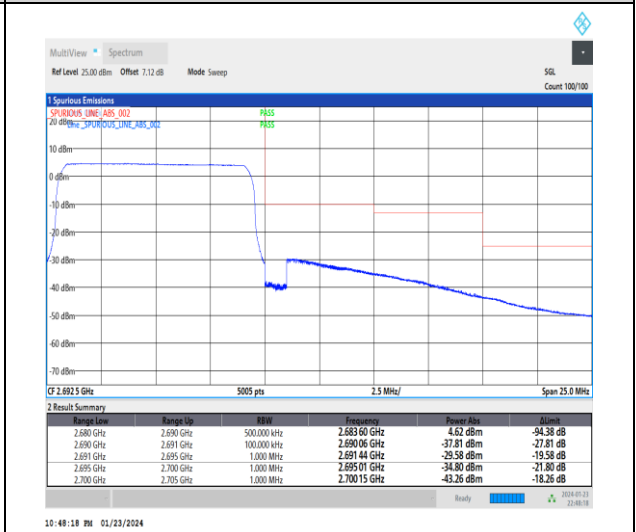
1-N41-30-10-H-6-CP-QPSK-Outer_Full-24@0-Ant3-1--PASS-see graph
