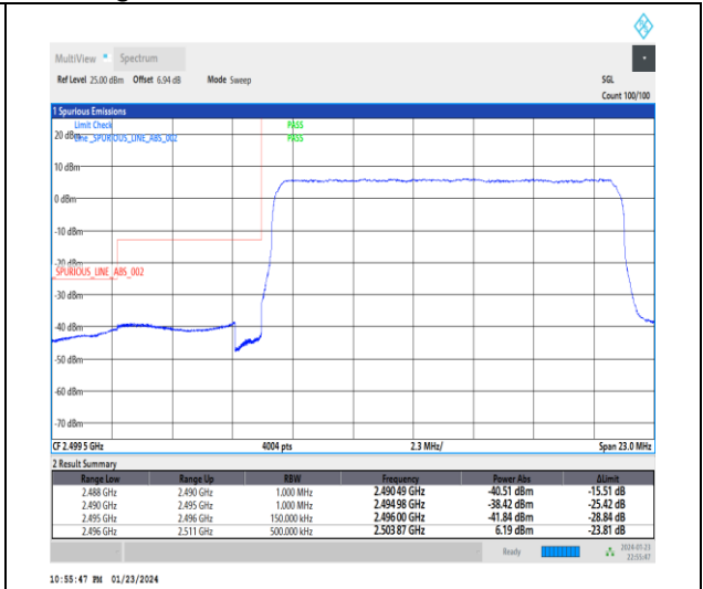
1-N41-30-15-L-3-DFT-PI2BPSK-Outer_Full-36@0-Ant3-1--PASS-see graph
