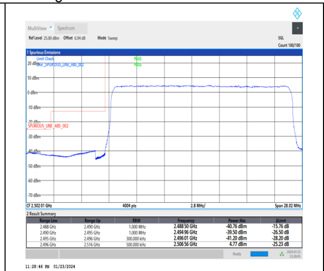
1-N41-30-20-L-3-DFT-PI2BPSK-Outer_Full-50@0-Ant3-1--PASS-see graph
