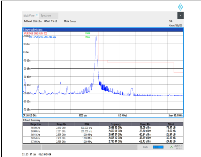
1-N41-30-40-H-2-DFT-PI2BPSK-Edge_1RB_Right-1 @ 105-Ant3-1--PASS-see graph
