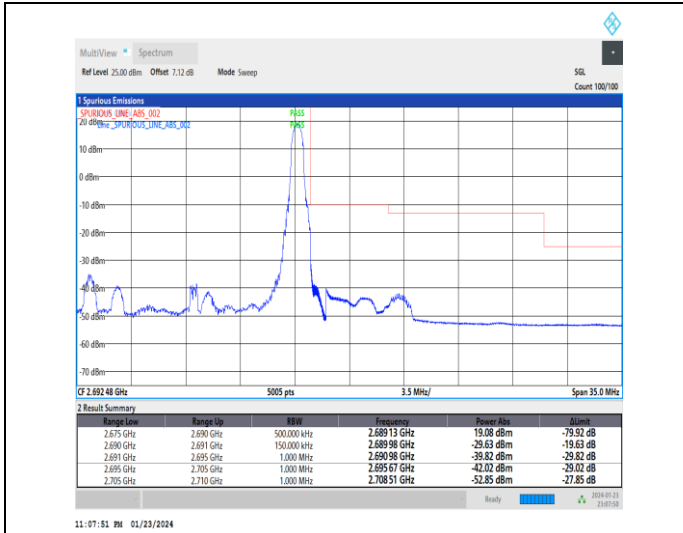
1-N41-30-15-H-2-DFT-PI2BPSK-Edge_1RB_Right-1@37-Ant3-1--PASS-see graph
