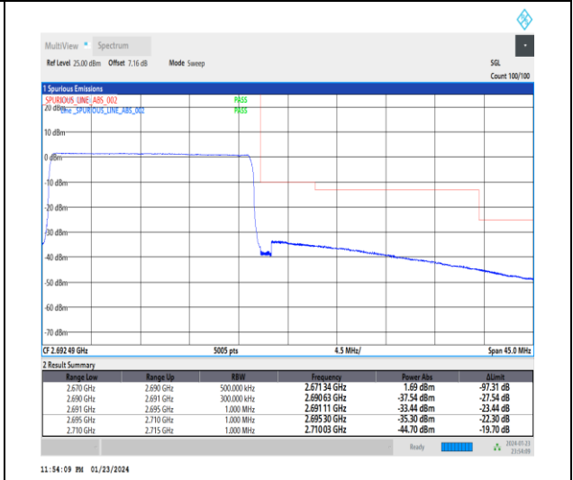
1-N41-30-20-H-6-CP-QPSK-Outer_Full-51@0-Ant3-1--PASS-see graph
