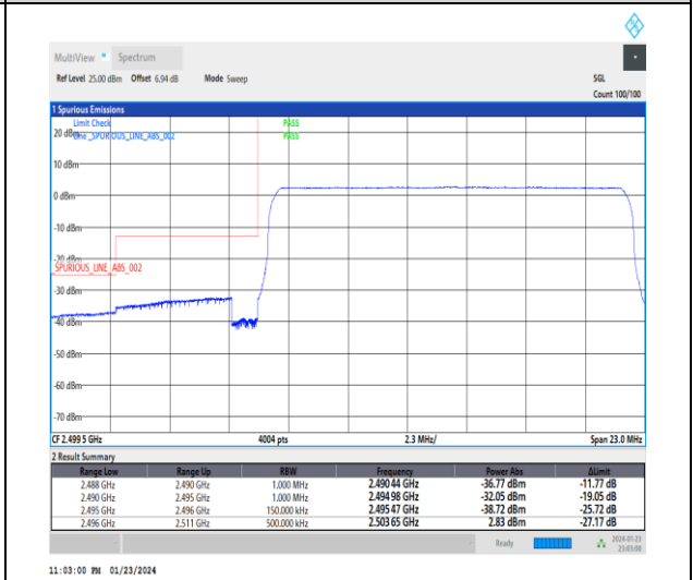
1-N41-30-15-L-6-CP-QPSK-Outer_Full-38@0-Ant3-1--PASS-see graph
