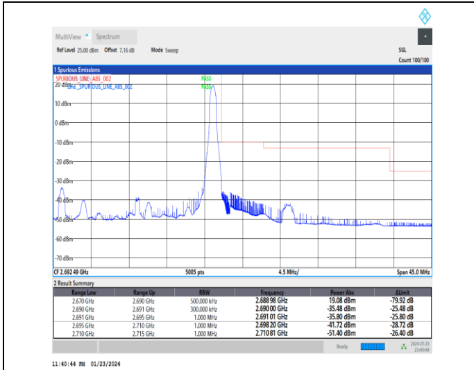
1-N41-30-20-H-2-DFT-PI2BPSK-Edge_1RB_Right-1 @ 50-Ant3-1--PASS-see graph
