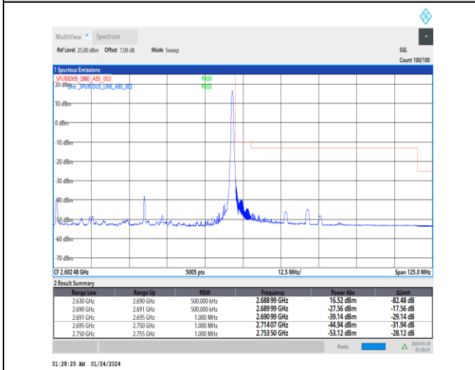
1-N41-30-60-H-5-CP-QPSK-Edge_1RB_Right-1 @ 161-Ant3-1--PASS-see graph
