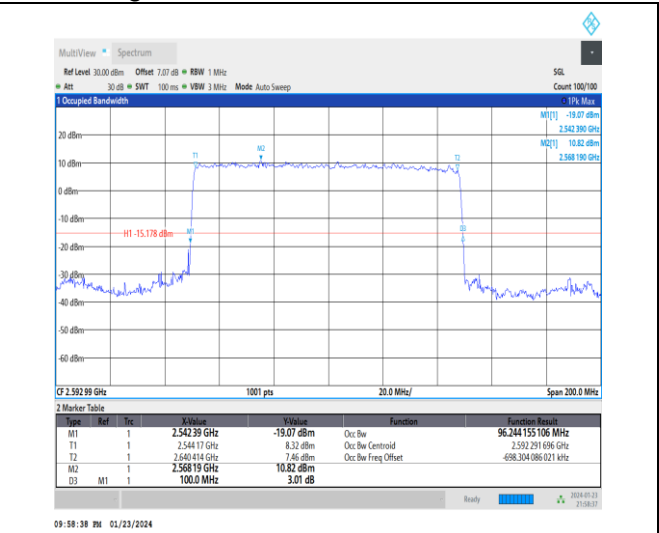
1-N41-30-100-M-2-DFT-PI2BPSK-Outer_Full-270@0-Ant3-96.244-100.000-≤100-PASS
