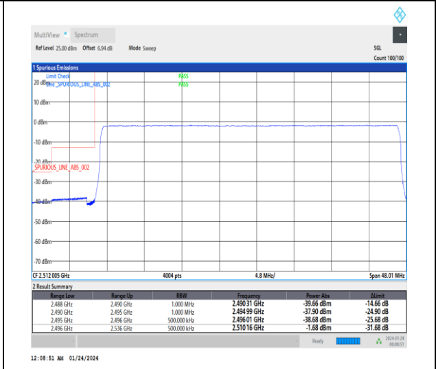
1-N41-30-40-L-6-CP-QPSK-Outer_Full-106@0-Ant3-1--PASS-see graph
