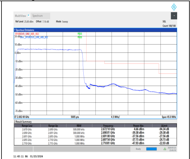
1-N41-30-20-H-3-DFT-PI2BPSK-Outer_Full-50@0 -Ant3-1--PASS-see graph
