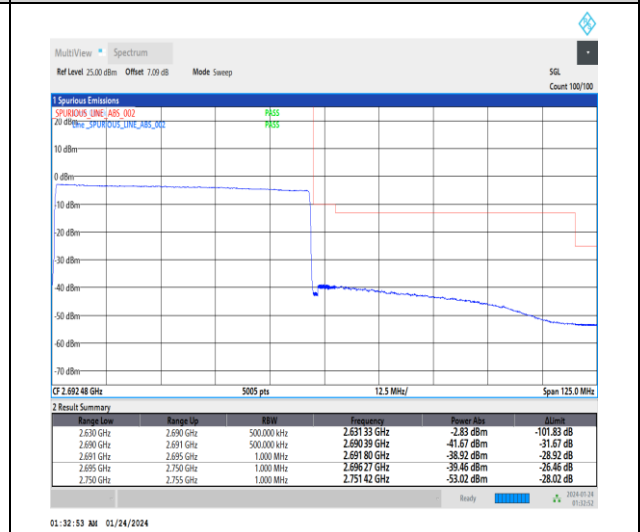
1-N41-30-60-H-6-CP-QPSK-Outer_Full-162 @ 0-Ant3-1--PASS-see graph
