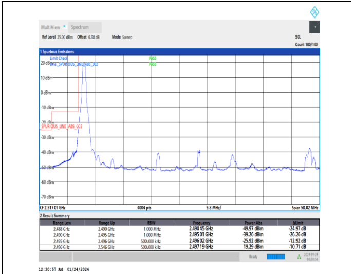
1-N41-30-50-L-1-DFT-PI2BPSK-Edge_1RB_Left-1@0-Ant3-1--PASS-see graph
