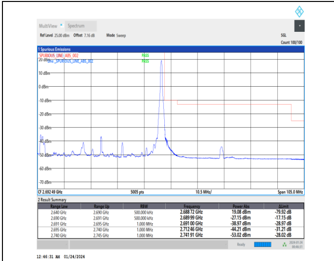
1-N41-30-50-H-2-DFT-PI2BPSK-Edge_1RB_Right-1@132-Ant3-1--PASS-see graph
