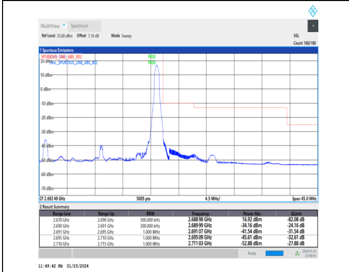
1-N41-30-20-H-5-CP-QPSK-Edge_1RB_Right-1 @ 50-Ant3-1--PASS-see graph
