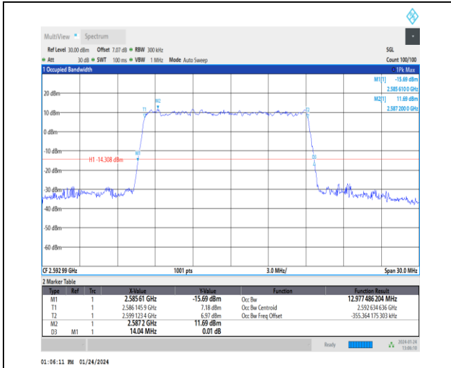
1-N41-30-15-M-4-DFT-64QAM-Outer_Full-36@0-Ant 3-12.977-14.040-≤15-PASS
