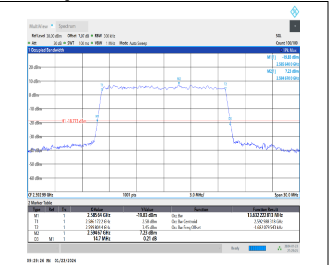
1-N41-30-15-M-9-CP-256QAM-Outer_Full-38@0-Ant 3-13.632-14.700-≤15-PASS
