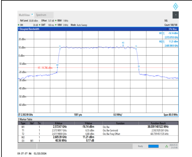
1-N41-30-40-M-8-CP-64QAM-Outer_Full-106@0-Ant3 t3-38.039-40.560-≤40-PASS
