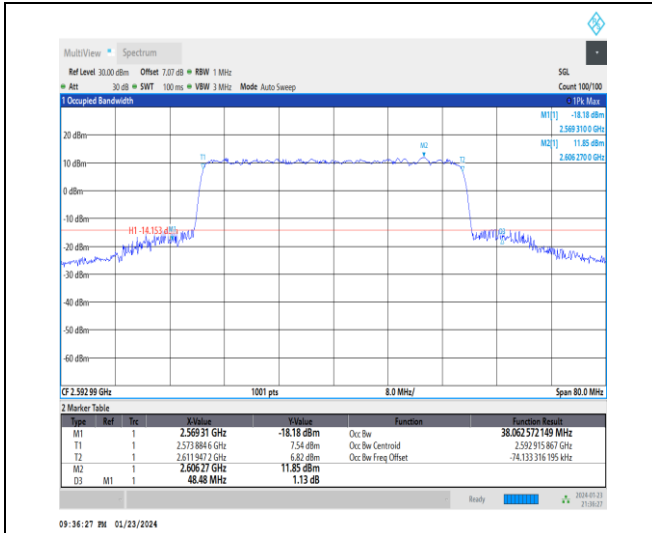
1-N41-30-40-M-6-CP-QPSK-Outer_Full-106@0-Ant3 -38.063-48.480-≤40-PASS
