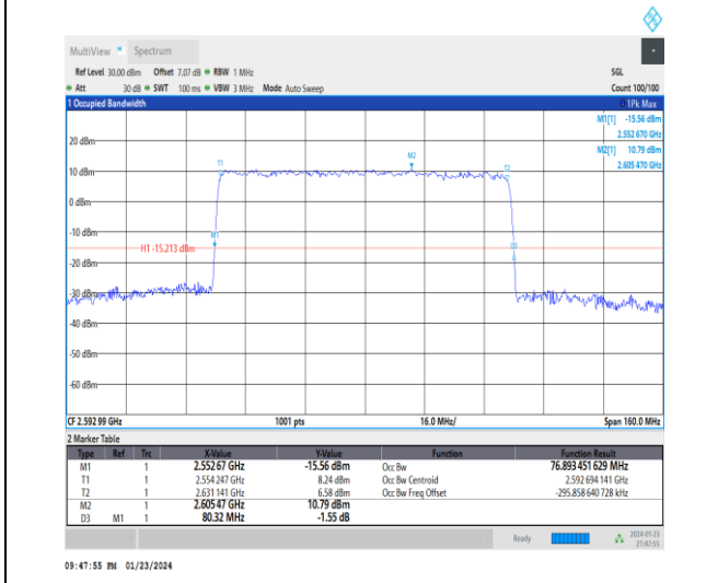
1-N41-30-80-M-1-DFT-QPSK-Outer_Full-216@0-Ant 3-76.893-80.320-<=80-PASS
