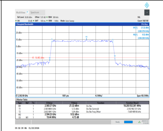
1-N41-30-20-M-6-CP-QPSK-Outer_Full-51@0-Ant3 18.204-19.440-≤20-PASS
