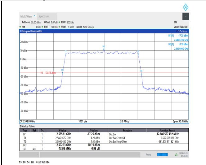
1-N41-30-15-M-5-DFT-256QAM-Outer_Full-36@0-A nt3-12.881-13.980-≤15-PASS
