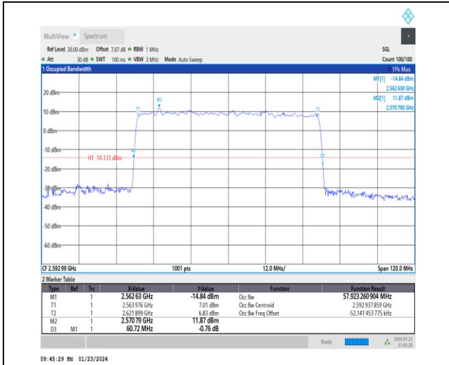
1-N41-30-60-M-4-DFT-64QAM-Outer_Full-162@0-Ant3-57.923-60.720-≤60-PASS
