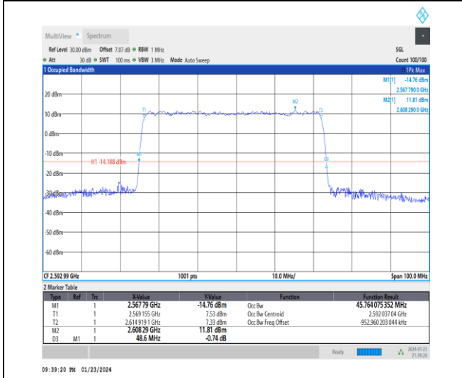
1-N41-30-50-M-3-DFT-16QAM-Outer_Full-128@0-Ant 3-45.764-48.600-≤50-PASS
