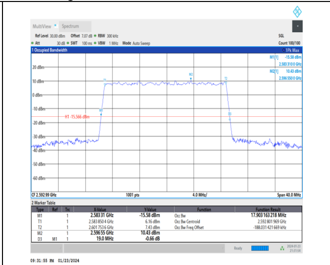
1-N41-30-20-M-4-DFT-64QAM-Outer_Full-50@0-Ant 3-17.903-19.000-≤20-PASS
