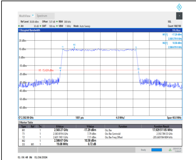
1-N41-30-20-M-3-DFT-16QAM-Outer_Full-50@0-Ant 3-17.93-19.080-≤20-PASS
