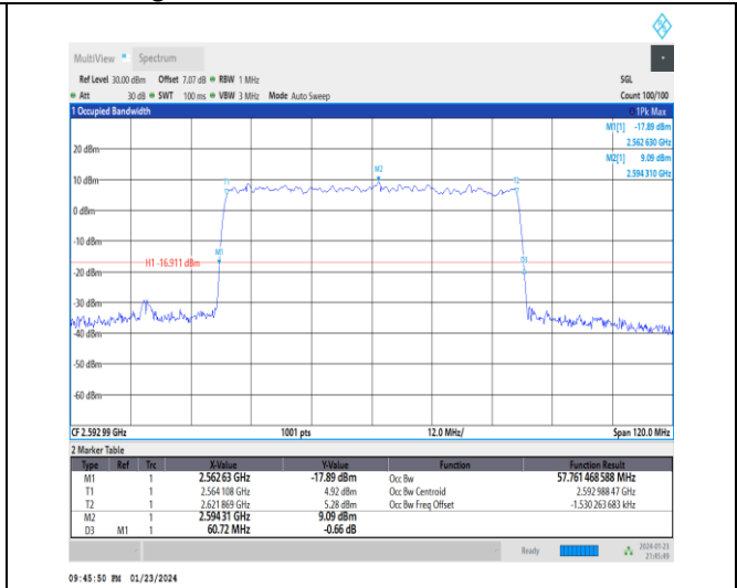
1-N41-30-60-M-5-DFT-256QAM-Outer_Full-162@0-Ant3-57.761-60.720-≤60-PASS
