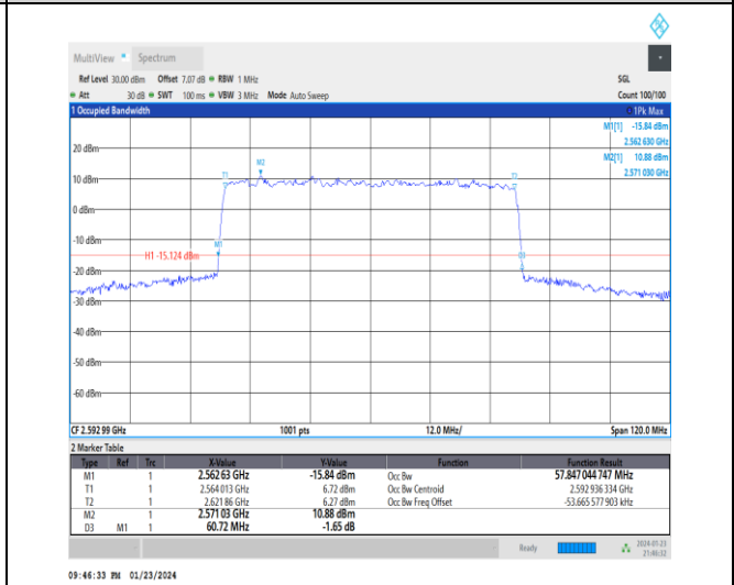
1-N41-30-60-M-7-CP-16QAM-Outer_Full-162@0-Ant3-57.847-60.720-≤60-PASS
