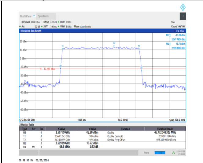
1-N41-30-50-M-2-DFT-PI2BPSK-Outer_Full-128@0-Ant 3-45.773-48.600-≤50-PASS
