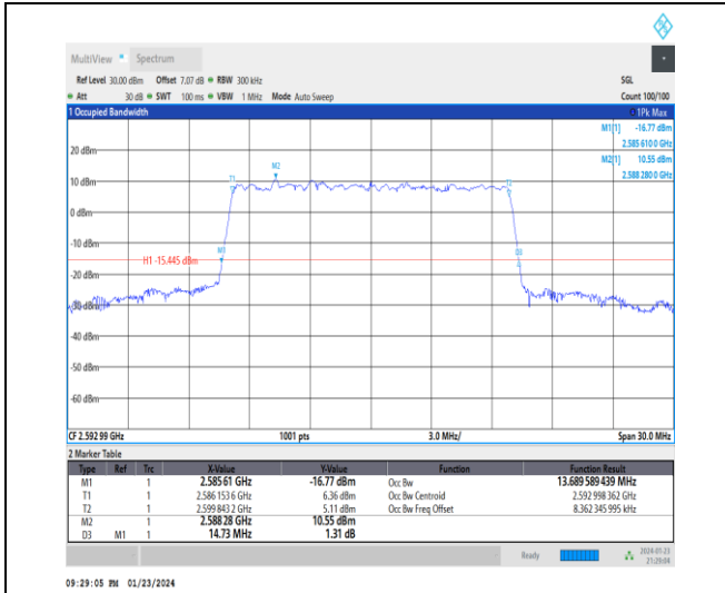
1-N41-30-15-M-8-CP-64QAM-Outer_Full-38@0-Ant 3-13.69-14.730-≤15-PASS
