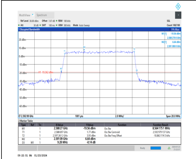
1-N41-30-10-M-7-CP-16QAM-Outer_Full-24@0-Ant 3-8.564-9.280-≤10-PASS
