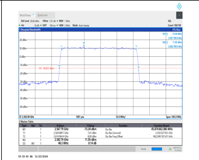
1-N41-30-50-M-4-DFT-64QAM-Outer_Full-128@0-Ant 3-45.875-48.500-≤50-PASS
