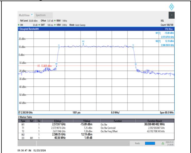
1-N41-30-40-M-7-CP-16QAM-Outer_Full-106@0-Ant3 3-38.038-40.560-≤40-PASS
