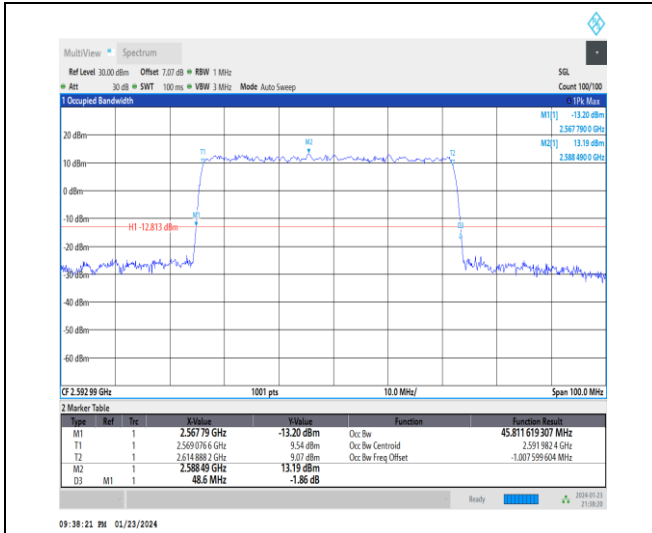
1-N41-30-50-M-1-DFT-QPSK-Outer_Full-128@0-Ant 3-45.812-48.600-≤50-PASS
