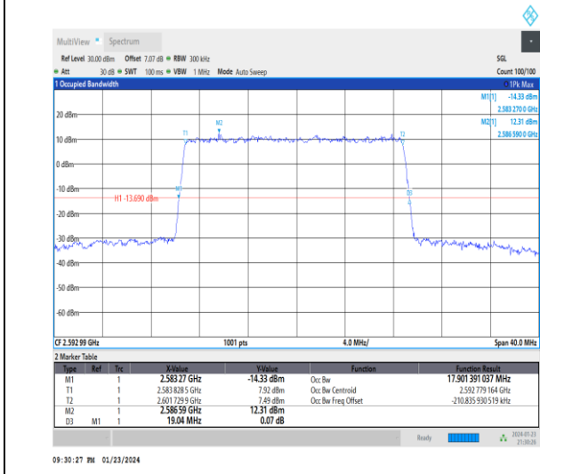
1-N41-30-20-M-1-DFT-QPSK-Outer_Full-50@0-Ant3 -17.901-19.040-≤20-PASS
