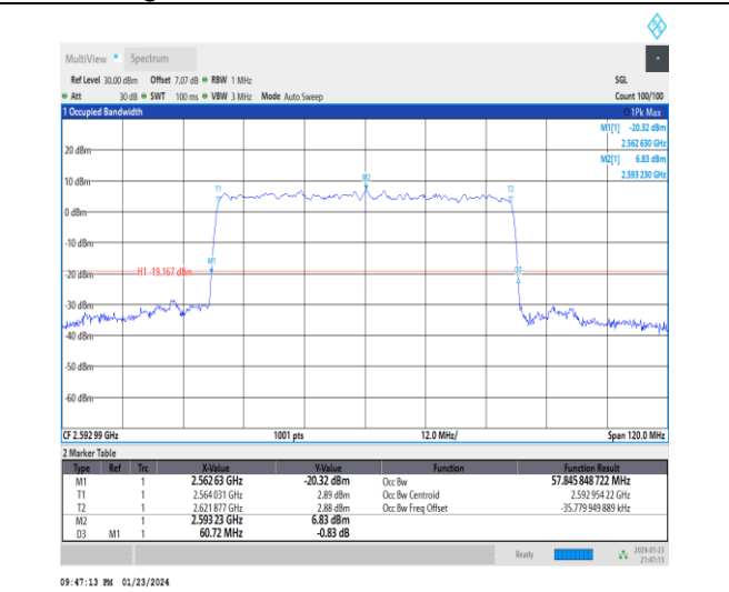
1-N41-30-60-M-9-CP-256QAM-Outer_Full-162@0-A nt3-57.846-60.720-<=60-PASS
