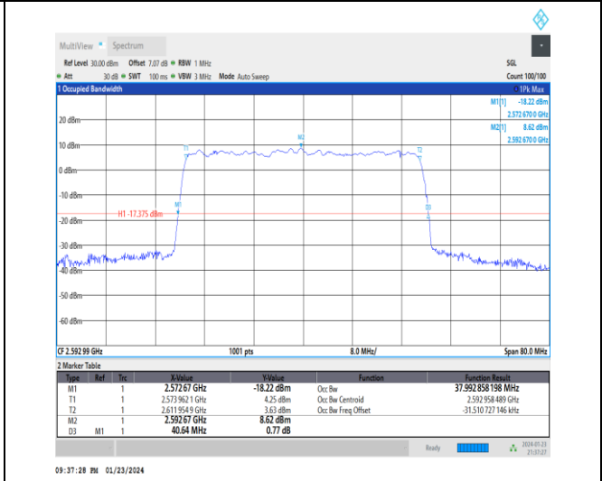
1-N41-30-40-M-9-CP-256QAM-Outer_Full-106@0-Ant3 nt3-37.993-40.640-≤40-PASS
