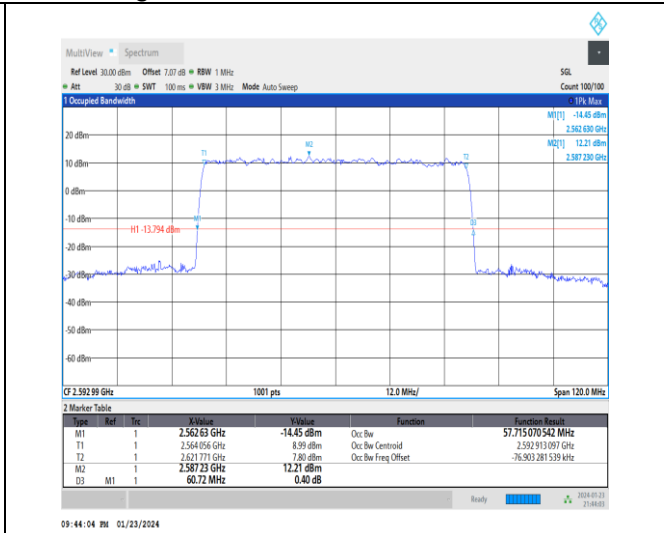
1-N41-30-60-M-1-DFT-QPSK-Outer_Full-162@0-Ant 3-57.715-60.720-≤60-PASS
