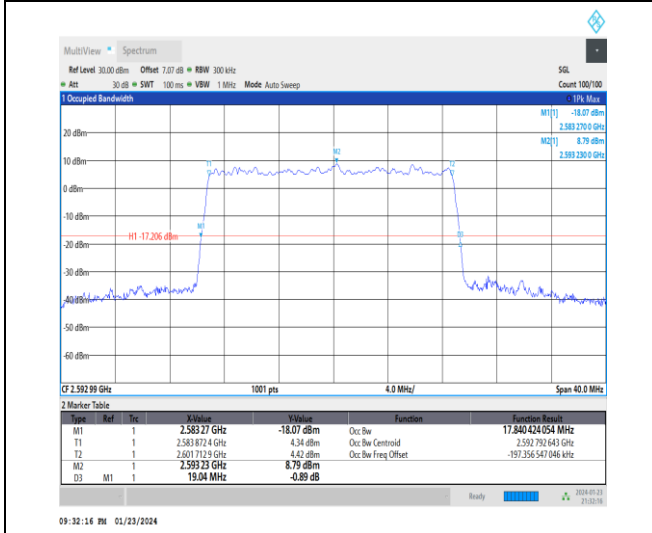
1-N41-30-20-M-5-DFT-256QAM-Outer_Full-50@0-A nt3-17.84-19.040-≤20-PASS
