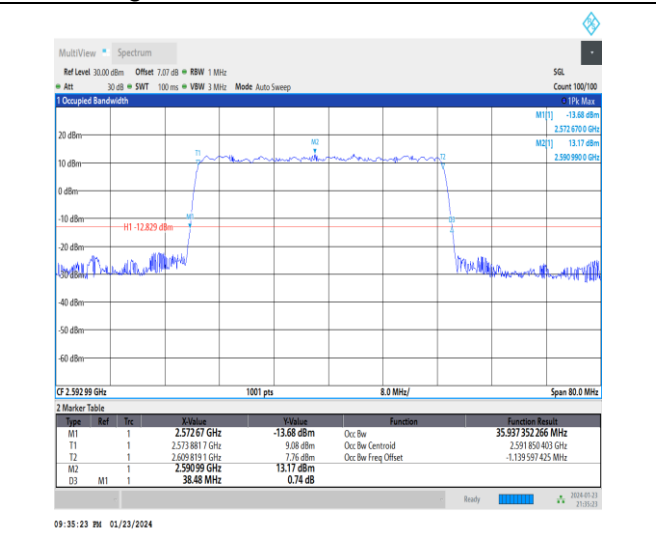
1-N41-30-40-M-3-DFT-16QAM-Outer_Full-100@0-Ant3-35.937-38.480-<math>\leq 40</math>-PASS
