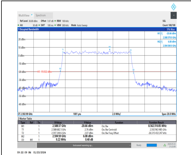
1-N41-30-10-M-5-DFT-256QAM-Outer_Full-24@0-A nt3-8.562-9.220-≤10-PASS
