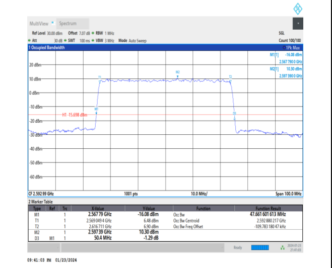
1-N41-30-50-M-8-CP-64QAM-Outer_Full-133@0-Ant3-47.662-50.400-≤50-PASS
