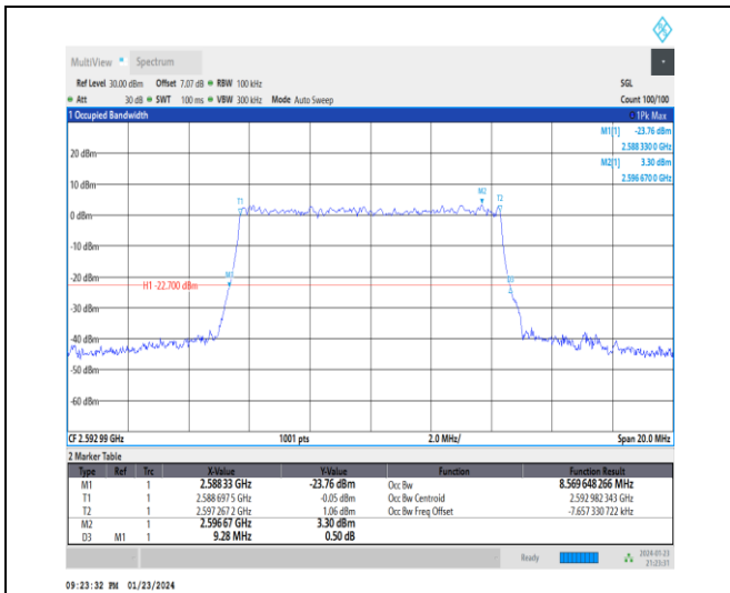
1-N41-30-10-M-9-CP-256QAM-Outer_Full-24@0-Ant3-8.57-9.280-≤10-PASS
