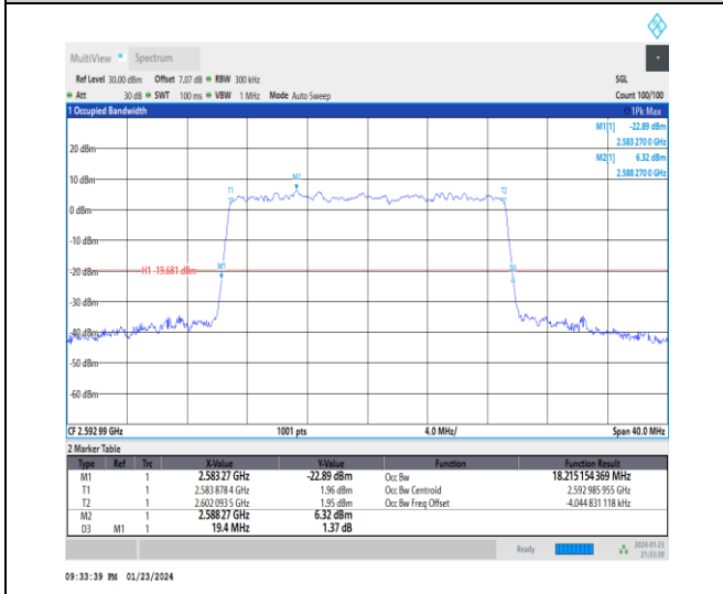
1-N41-30-20-M-9-CP-256QAM-Outer_Full-51@0-An t3-18.215-19.400-≤20-PASS
