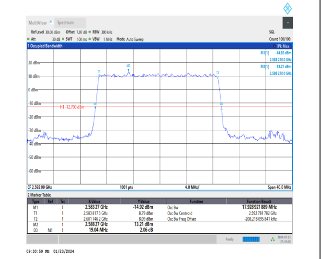
1-N41-30-20-M-2-DFT-PI2BPSK-Outer_Full-50@0-Ant3 -17.929-19.040-≤20-PASS
