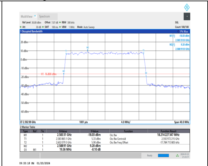
1-N41-30-20-M-8-CP-64QAM-Outer_Full-51@0-Ant3 -18.214-19.360-≤20-PASS
