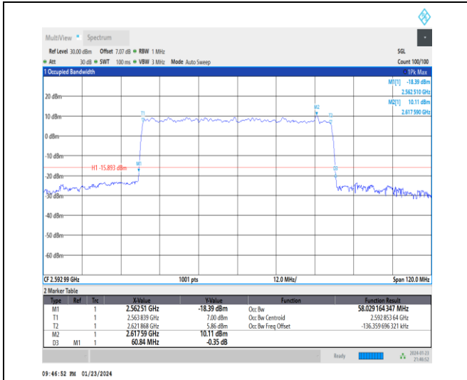
1-N41-30-60-M-8-CP-64QAM-Outer_Full-162@0-An t3-58.029-60.840-<=60-PASS
