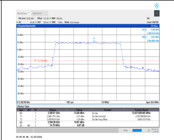
1-N41-30-15-M-7-CP-16QAM-Outer_Full-38@0-Ant3 -13.638-14.790-≤15-PASS
