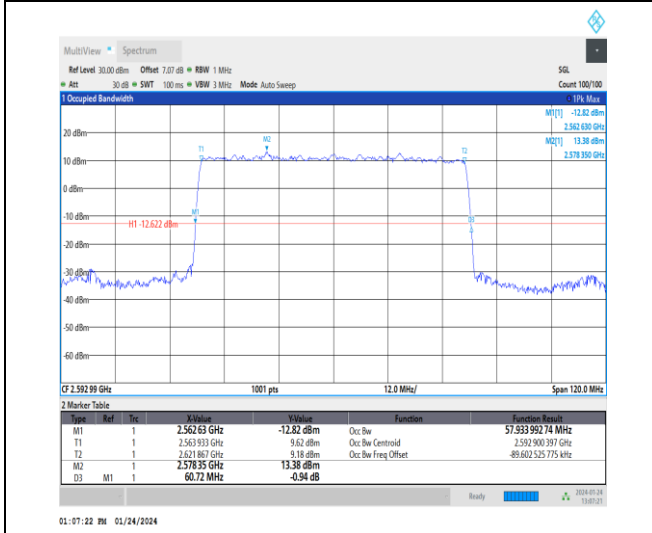
1-N41-30-60-M-2-DFT-PI2BPSK-Outer_Full-162@0-Ant3 57.934-60.720-≤60-PASS
