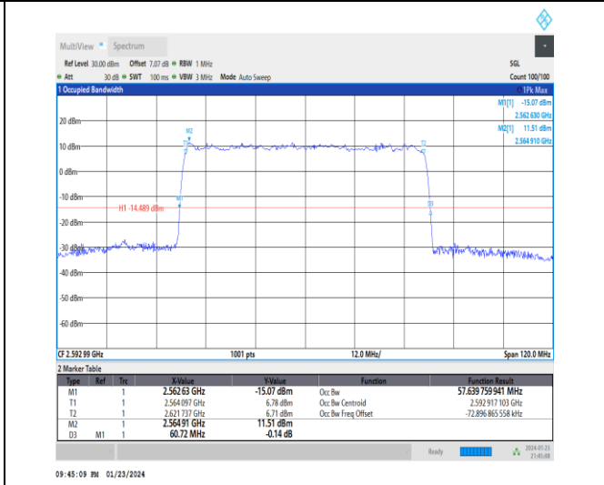
1-N41-30-60-M-3-DFT-16QAM-Outer_Full-162@0-A nt3-57.64-60.720-≤60-PASS
