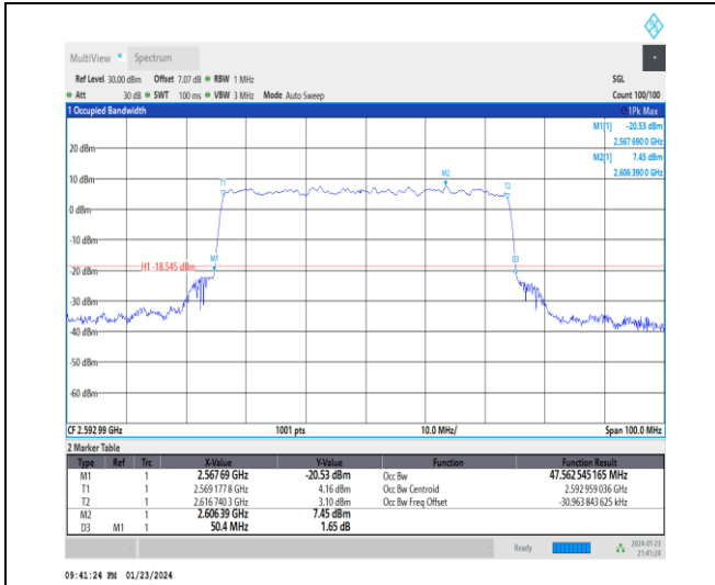
1-N41-30-50-M-9-CP-256QAM-Outer_Full-133@0-A nt3-47.563-50.400-≤50-PASS
