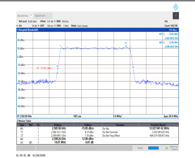
1-N41-30-15-M-3-DFT-16QAM-Outer_Full-36@0-Ant3-12.927-14.010-≤15-PASS
