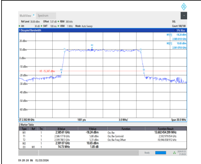
1-N41-30-15-M-6-CP-QPSK-Outer_Full-38@0-Ant3 13.602-14.730-≤15-PASS
