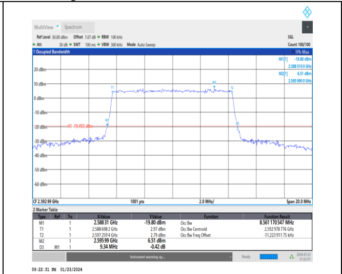
1-N41-30-10-M-6-CP-QPSK-Outer_Full-24@0-Ant3- 8.561-9.340-≤10-PASS
