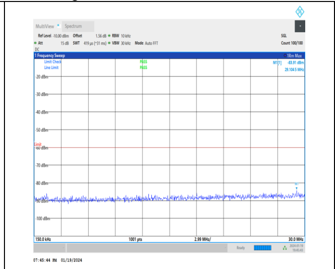
1-N30-30-10-H-1-DFT-PI2BPSK-Inner_1RB_Left-1 @ 1-0.15-30-Ant3-29.10--83.91--60-PASS
