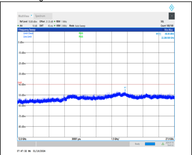
1-N30-30-10-H-1-DFT-PI2BPSK-Inner_1RB_Left-1 @ 1-12000-27000-Ant3-22286.50--46.44--40-PASS
