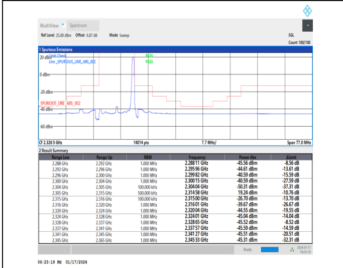
1-N30-15-10-H-5-CP-QPSK-Edge_1RB_Right-1@51-Ant3-1--PASS-see graph
