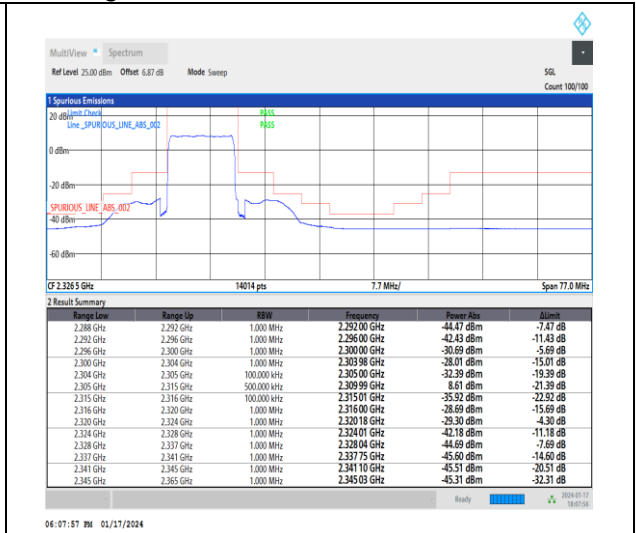
1-N30-15-10-H-3-DFT-PI2BPSK-Outer_Full-50@0-Ant3-1--PASS-see graph
