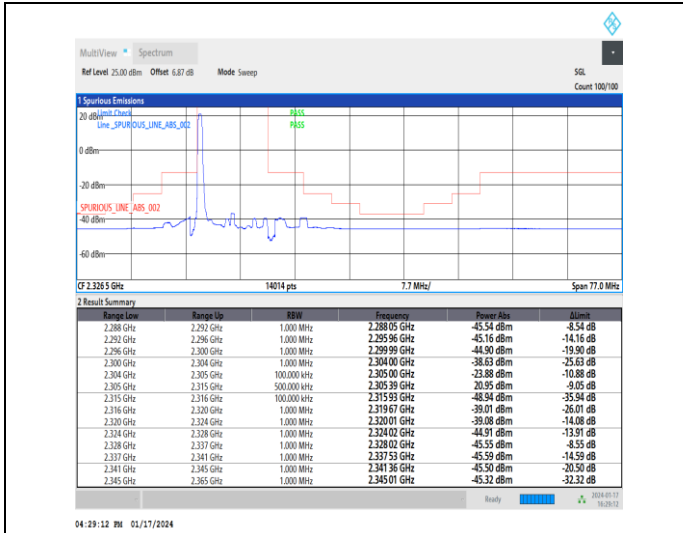
1-N30-15-10-L-1-DFT-PI2BPSK-Edge_1RB_Left-1@0-Ant3-1--PASS-see graph
