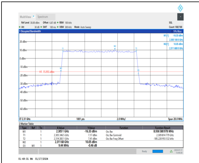
1-N30-15-10-M-4-DFT-64QAM-Outer_Full-50@0-Ant 3-8.937-9.440-≤10-PASS
