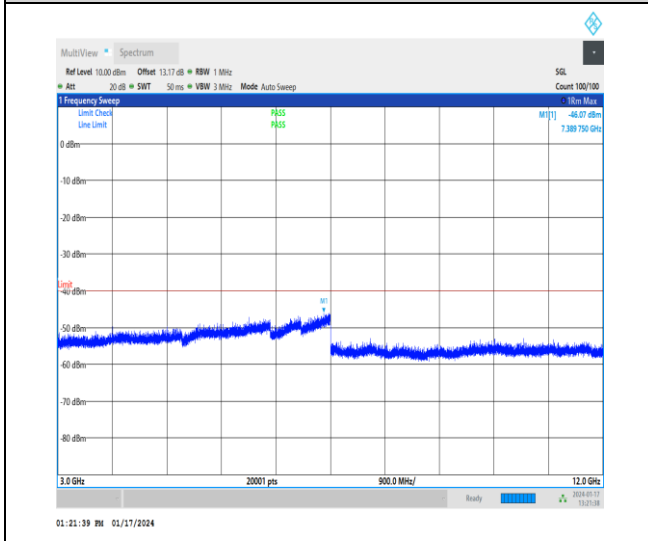
1-N30-30-10-M-1-DFT-PI2BPSK-Inner_1RB_Left-1 @ 1-3000-12000-Ant3-7389.75--46.07--40-PASS
