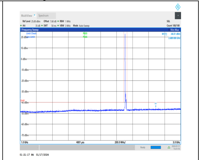
1-N30-30-10-M-1-DFT-PI2BPSK-Inner_1RB_Left-1 @ 1-1000-3000-Ant3-2689.00--44.51--40-PASS
