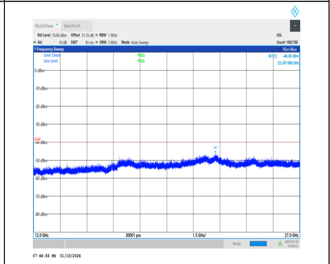
1-N30-30-10-M-1-DFT-PI2BPSK-Inner_1RB_Left-1 @ 1-12000-27000-Ant3-22247.00--46.43--40-PASS
