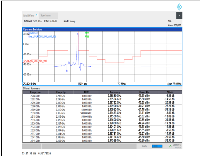
1-N30-15-5-H-2-DFT-PI2BPSK-Edge_1RB_Right-1@2 4-Ant3-1--PASS-see graph
