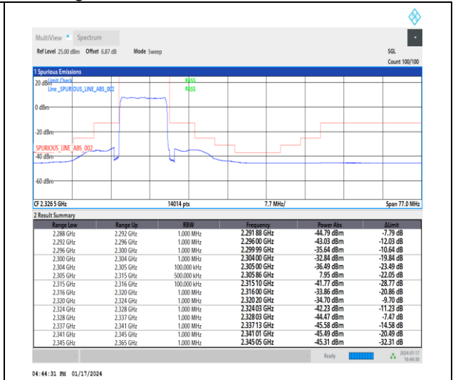
1-N30-15-10-L-3-DFT-PI2BPSK-Outer_Full-50@0-Ant3-1--PASS-see graph
