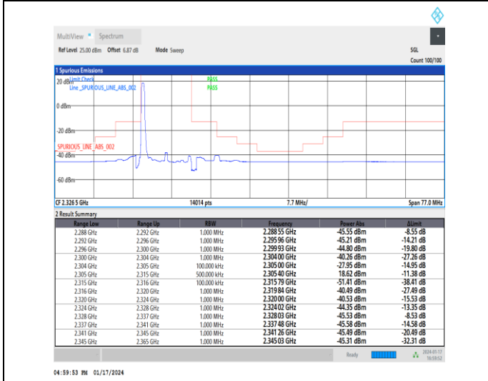
1-N30-15-10-L-4-CP-QPSK-Edge_1RB_Left-1@0-Ant3-1--PASS-see graph
