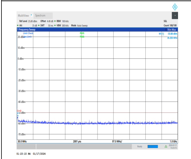
1-N30-30-10-H-1-DFT-PI2BPSK-Inner_1RB_Left-1 @ 1-30-1000-Ant3-35.34--53.88--50-PASS
