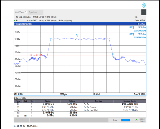
1-N30-15-5-M-8-CP-64QAM-Outer_Full-25@0-Ant3- 4.507-5.400-≤5-PASS
