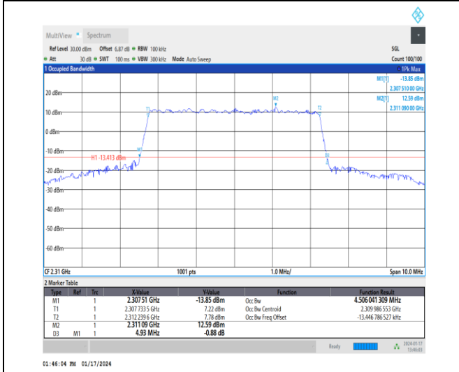
1-N30-15-5-M-7-CP-16QAM-Outer_Full-25@0-Ant3- 4.506-4.930-≤5-PASS
