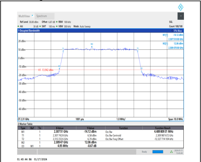
1-N30-15-5-M-6-CP-QPSK-Outer_Full-25@0-Ant3-4 .49-4.950-≤5-PASS
