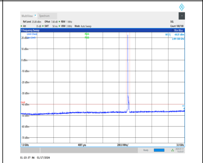
1-N30-30-10-H-1-DFT-PI2BPSK-Inner_1RB_Left-1 @ 1-1000-3000-Ant3-2991.50--44.81--40-PASS
