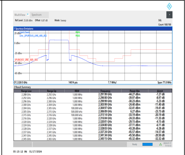
1-N30-15-10-L-6-CP-QPSK-Outer_Full-52@0-Ant3-1--PASS-see graph
