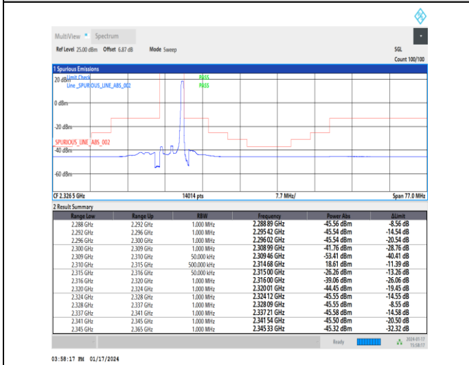
1-N30-15-5-H-5-CP-QPSK-Edge_1RB_Right-1@24-Ant3-1--PASS-see graph
