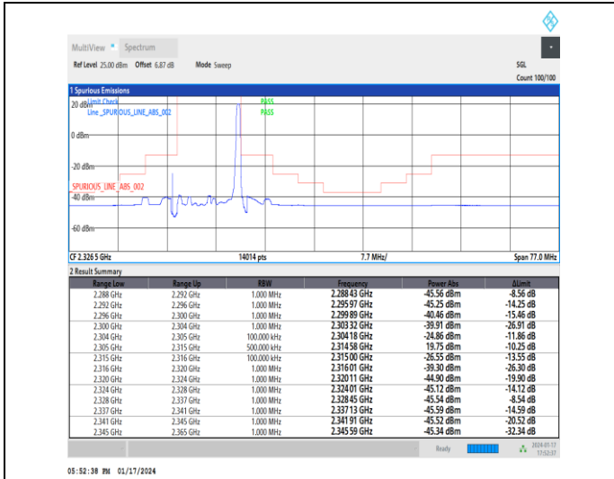
1-N30-15-10-H-2-DFT-PI2BPSK-Edge_1RB_Right-1@51-Ant3-1--PASS-see graph
