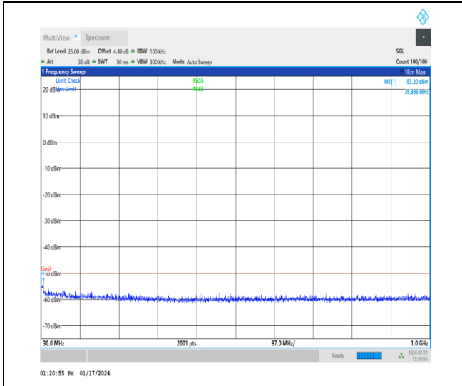
1-N30-30-10-M-1-DFT-PI2BPSK-Inner_1RB_Left-1 @ 1-30-1000-Ant3-35.34--53.20--50-PASS
