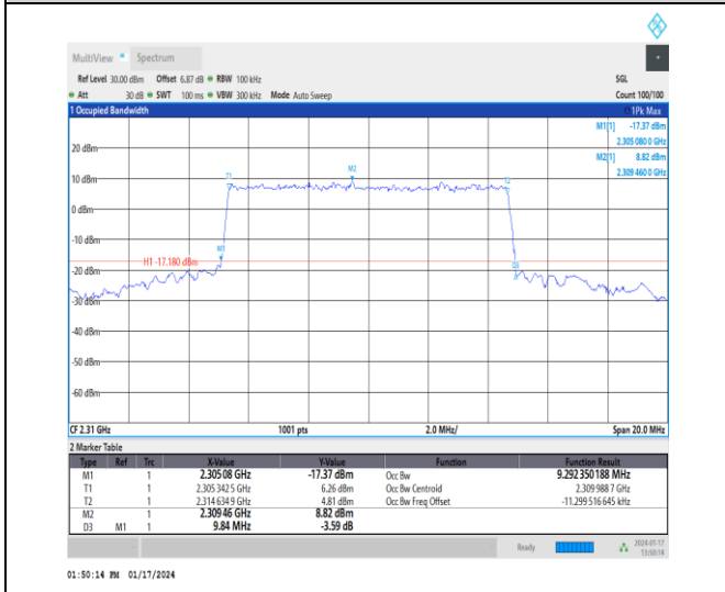
1-N30-15-10-M-6-CP-QPSK-Outer_Full-52@0-Ant3 9.292-9.840-≤10-PASS
