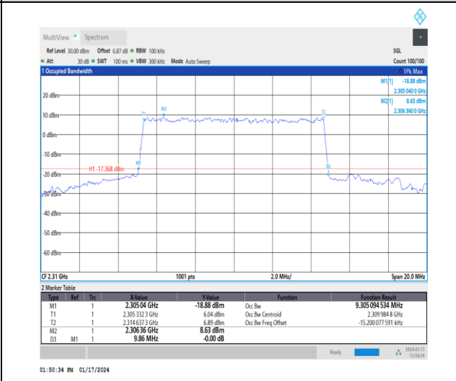
1-N30-15-10-M-7-CP-16QAM-Outer_Full-52@0-Ant 3-9.305-9.860-≤10-PASS
