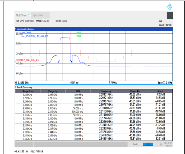
1-N30-15-5-H-3-DFT-PI2BPSK-Outer_Full-25@0-4-Ant3-1--PASS-see graph
