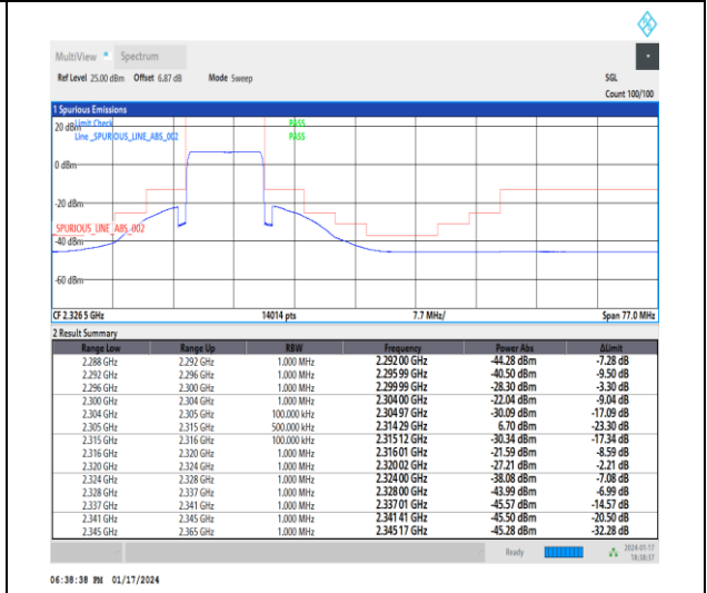
1-N30-15-10-H-6-CP-QPSK-Outer_Full-52@0-Ant3-1--PASS-see graph
