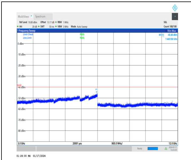
1-N30-30-10-H-1-DFT-PI2BPSK-Inner_1RB_Left-1 @ 1-3000-12000-Ant3-7445.55--45.48--40-PASS
