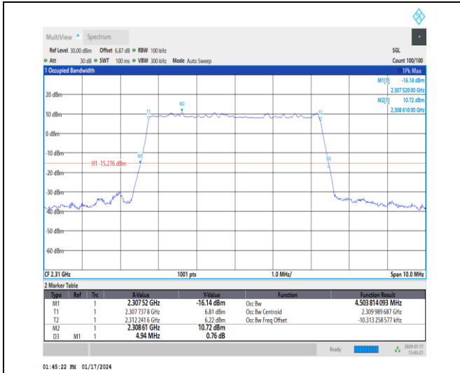
1-N30-15-5-M-5-DFT-256QAM-Outer_Full-25@0-Ant 3-4.504-4.940-≤5-PASS
