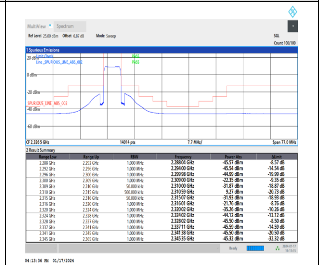
1-N30-15-5-H-6-CP-QPSK-Outer_Full-25@0-Ant3-1--PASS-see graph
