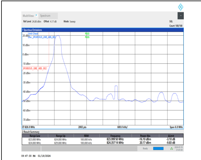
1-N26-824-849-15-10-L-1-DFT-PI2BPSK-Edge_1RB_L eft-1@0-Ant0-1-seegraph-PASS-see graph
