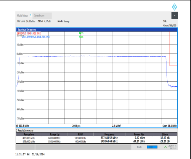
1-N26-824-849-15-20-H-6-CP-QPSK-Outer_Full-106 @ 0-Ant0-1-seegraph-PASS-see graph
