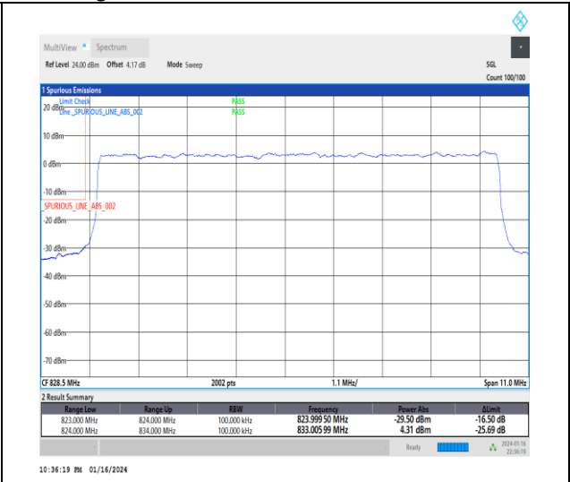
1-N26-824-849-15-10-L-3-DFT-PI2BPSK-Outer_F ull-50@0-Ant0-1-seegraph-PASS-see graph
