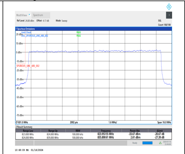
1-N26-824-849-15-15-L-3-DFT-PI2BPSK-Outer_F ull-75@0-Ant0-1-seegraph-PASS-see graph
