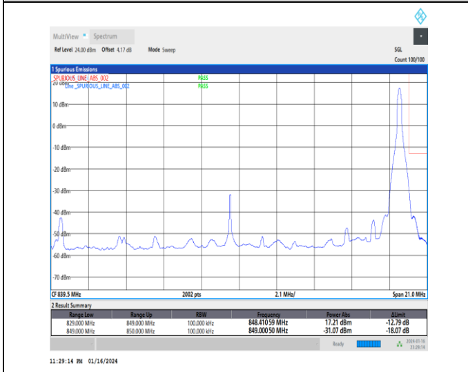
1-N26-824-849-15-20-H-5-CP-QPSK-Edge_1RB_Right-1 @ 105-Ant0-1-seegraph-PASS-see graph
