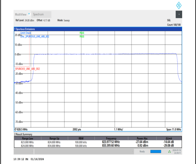
1-N26-824-849-15-10-L-6-CP-QPSK-Outer_Full-5 2@0-Ant0-1-seegraph-PASS-see graph
