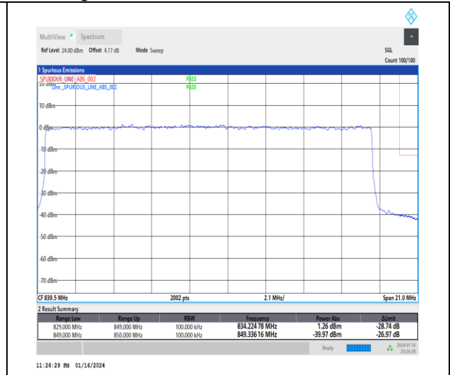
1-N26-824-849-15-20-H-3-DFT-PI2BPSK-Outer_Full-100 @ 0-Ant0-1-seegraph-PASS-see graph
