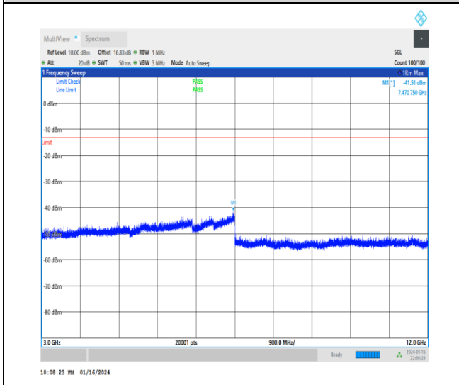
1-N26-824-849-15-20-M-1-DFT-PI2BPSK-Inner_1R B_Left-1@1-3000-12000-Ant0-7470.75--41.51--13-P ASS
