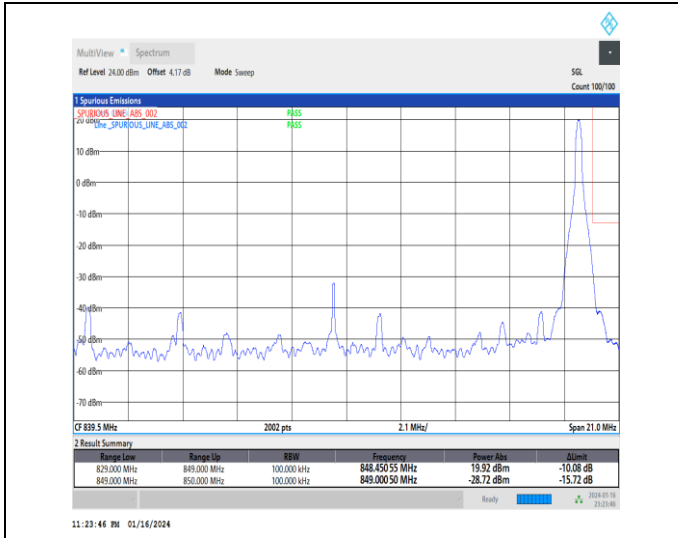
1-N26-824-849-15-20-H-2-DFT-PI2BPSK-Edge_1RB_Right-1 @ 105-Ant0-1-seegraph-PASS-see graph
