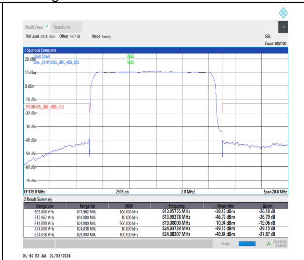
1-N26-814-824-15-10-H-3-DFT-PI2BPSK-Outer_Full-50@0-Ant0-1--PASS-see graph
