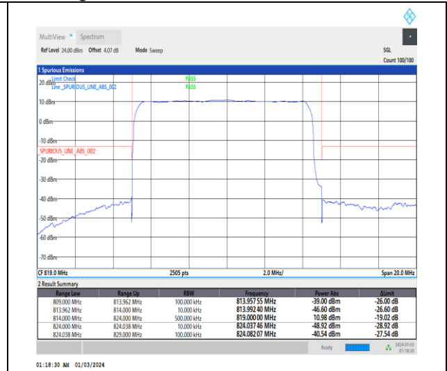
1-N26-814-824-15-10-L-3-DFT-PI2BPSK-Outer_F ull-50@0-Ant0-1--PASS-see graph
