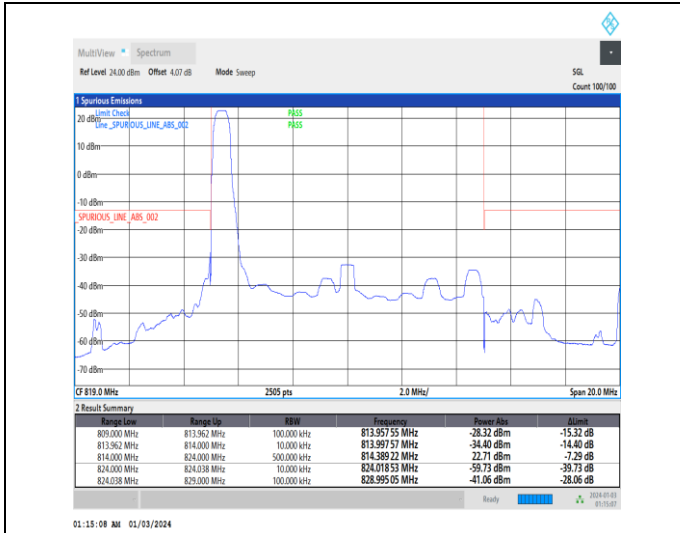
1-N26-814-824-15-10-L-1-DFT-PI2BPSK-Edge_1RB_L eft-1@0-Ant0-1--PASS-see graph
