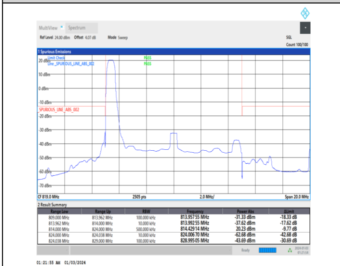
1-N26-814-824-15-10-L-4-CP-QPSK-Edge_1RB_Left-1 @0-Ant0-1--PASS-see graph
