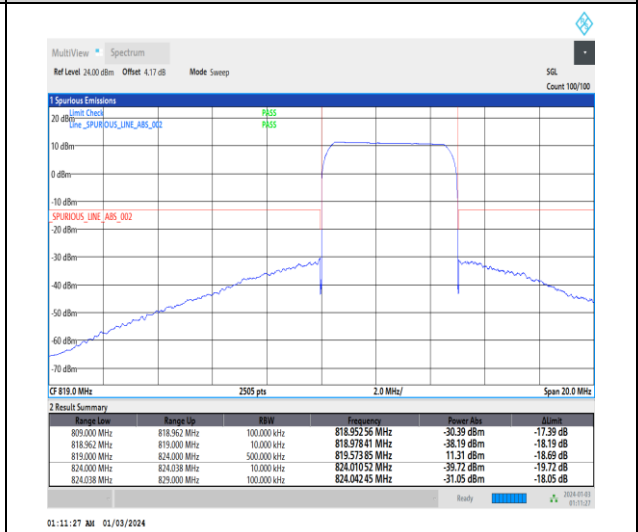
1-N26-814-824-15-5-H-6-CP-QPSK-Outer_Full-25@0-Ant0-1--PASS-see graph
