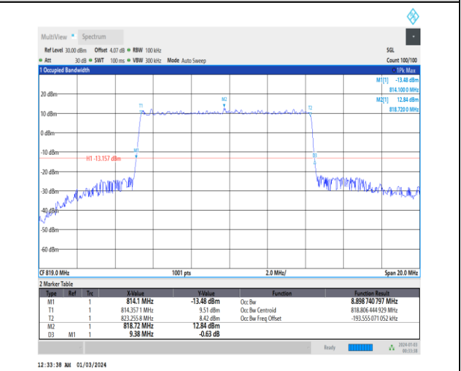
1-N26-814-824-15-10-M-3-DFT-16QAM-Outer_Full-5 0@0-Ant0-8.899-9.380-≤10-PASS
