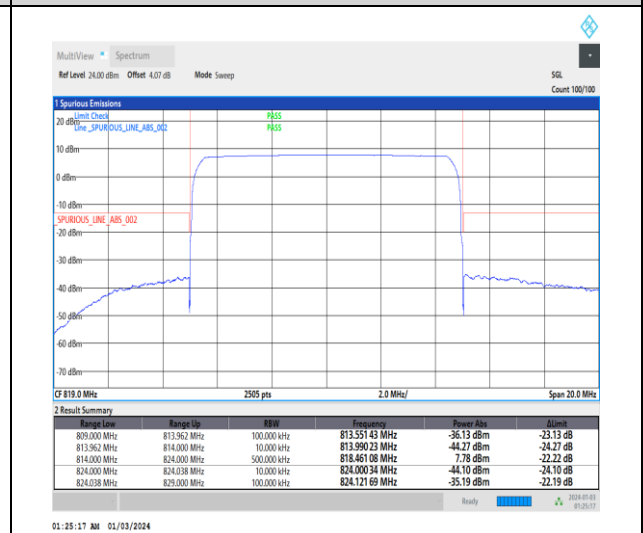
1-N26-814-824-15-10-L-6-CP-QPSK-Outer_Full-5 2@0-Ant0-1--PASS-see graph
