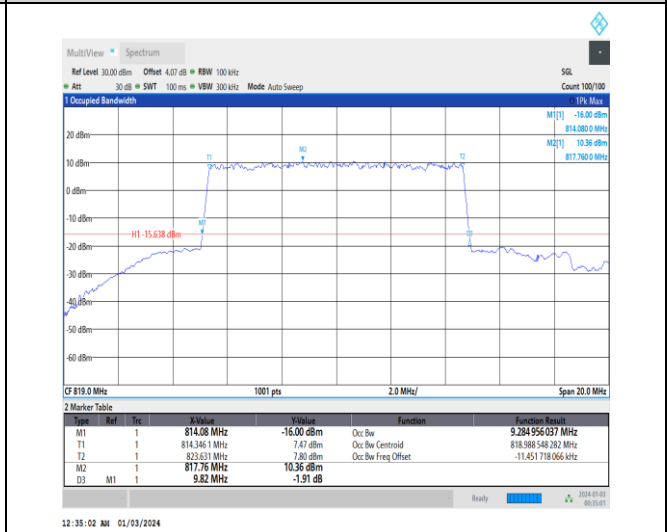
1-N26-814-824-15-10-M-7-CP-16QAM-Outer_Full-52@0-Ant0-9.285-9.820-≤10-PASS
