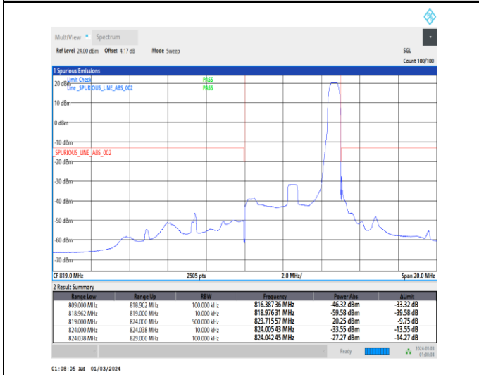
1-N26-814-824-15-5-H-5-CP-QPSK-Edge_1RB_Right-1@24-Ant0-1--PASS-see graph
