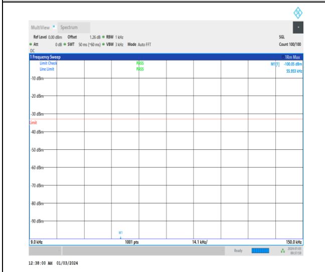
1-N26-814-824-15-10-M-1-DFT-PI2BPSK-Inner_1RB _Left-1@1-0.009-0.15-Ant0-0.06--100.05--33-PAS S
