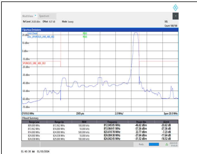
1-N26-814-824-15-10-H-2-DFT-PI2BPSK-Edge_1RB_Right-1@51-Ant0-1--PASS-see graph
