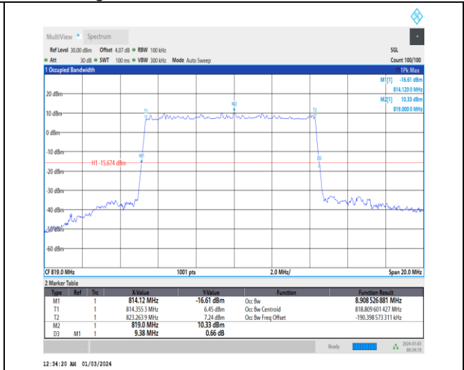
1-N26-814-824-15-10-M-5-DFT-256QAM-Outer_Full-50@0-Ant0-8.909-9.380-≤10-PASS
