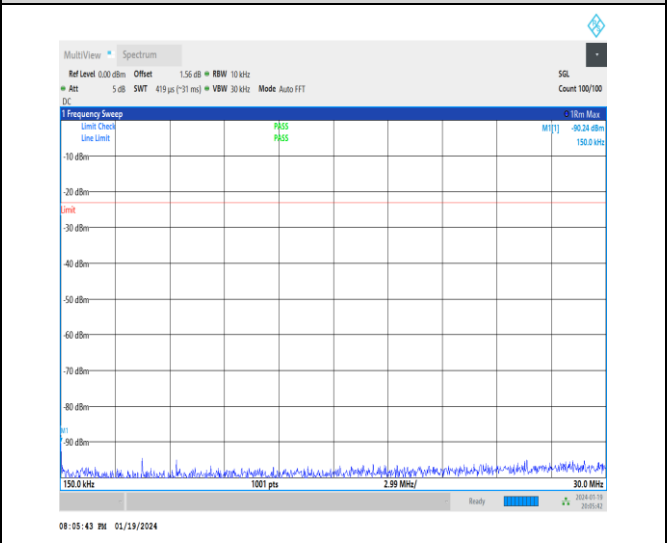
1-N26-814-824-15-10-M-1-DFT-PI2BPSK-Inner_1RB _Left-1@1-0.15-30-Ant0-0.15--90.24--23-PASS
