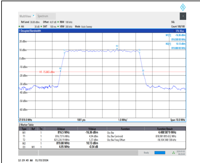
1-N26-814-824-15-5-M-9-CP-256QAM-Outer_Full-2 5@0-Ant0-4.489-4.950-≤5-PASS
