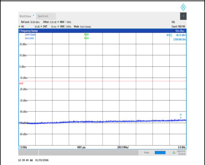
1-N26-814-824-15-10-H-1-DFT-PI2BPSK-Inner_1RB _Left-1@1-1000-3000-Ant0-2936.00--46.12--13-PASS
