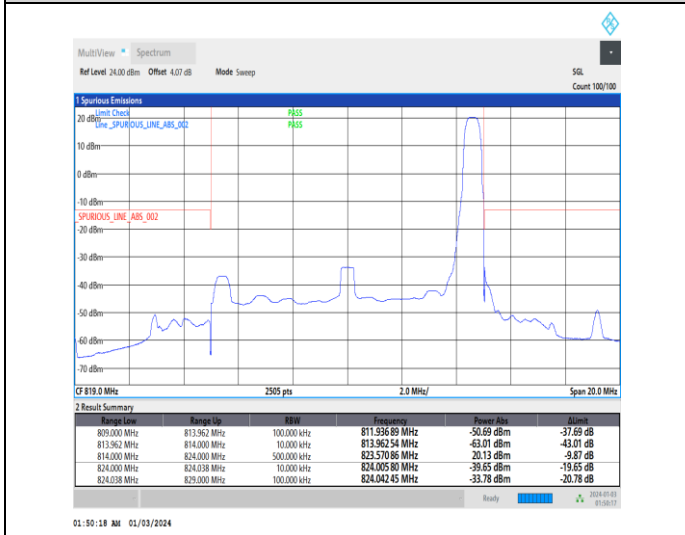
1-N26-814-824-15-10-H-5-CP-QPSK-Edge_1RB_Right-1@51-Ant0-1--PASS-see graph
