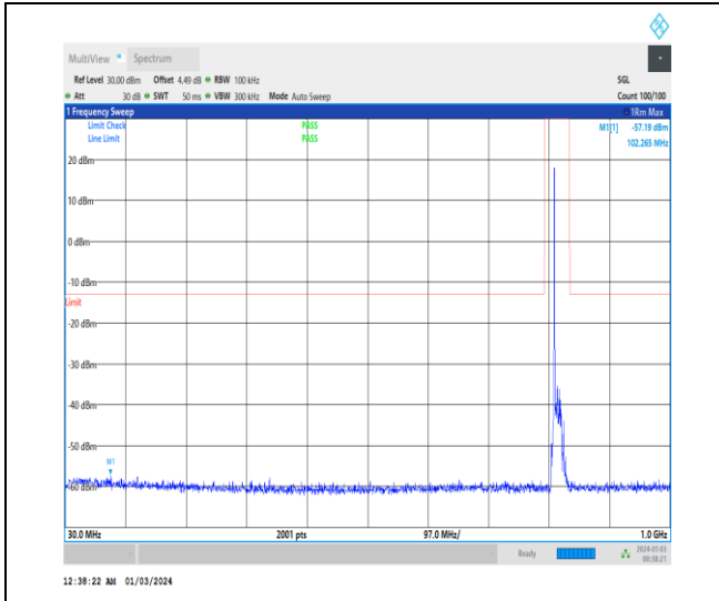
1-N26-814-824-15-10-M-1-DFT-PI2BPSK-Inner_1R B_Left-1@1-30-1000-Ant0-102.27--57.19--13-PASS
