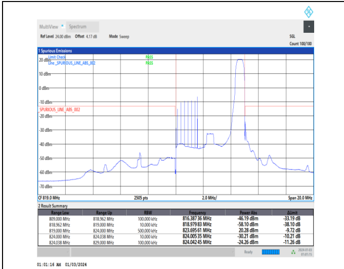
1-N26-814-824-15-5-H-2-DFT-PI2BPSK-Edge_1RB_Right-1@24-Ant0-1--PASS-see graph
