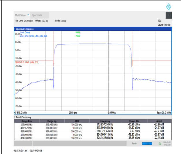
1-N26-814-824-15-10-H-6-CP-QPSK-Outer_Full-52@0-Ant0-1--PASS-see graph
