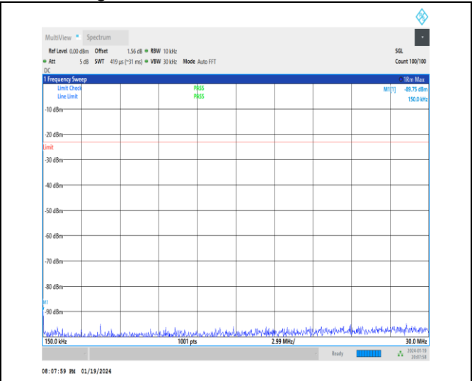
1-N26-814-824-15-10-H-1-DFT-PI2BPSK-Inner_1RB _Left-1@1-0.15-30-Ant0-0.15--89.75--23-PASS
