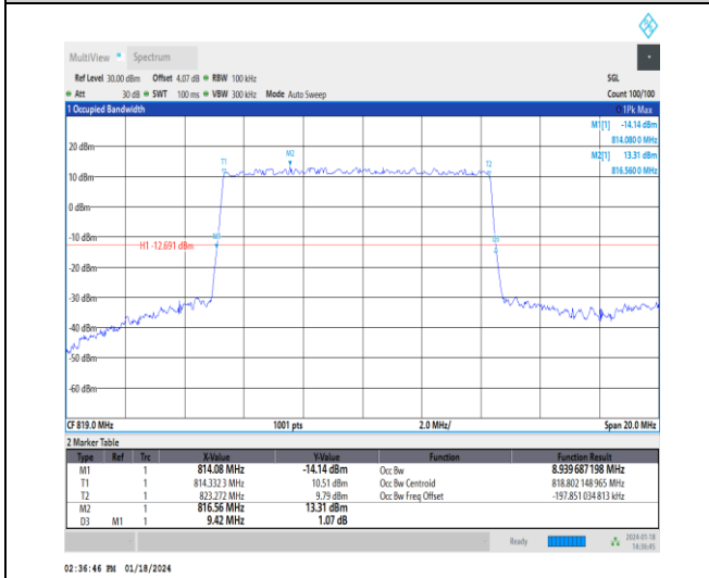
1-N26-814-824-15-10-M-2-DFT-PI2BPSK-Outer_Full-50 @0-Ant0-8.94-9.420-≤10-PASS
