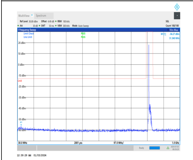
1-N26-814-824-15-10-H-1-DFT-PI2BPSK-Inner_1R B_Left-1@1-30-1000-Ant0-51.34--56.27--13-PASS
