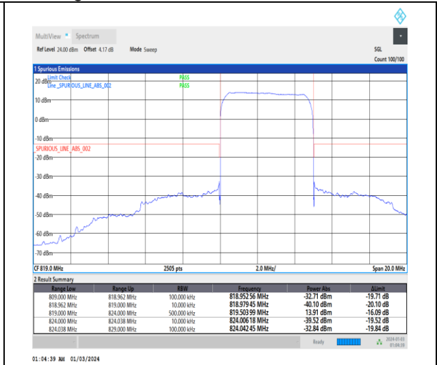
1-N26-814-824-15-5-H-3-DFT-PI2BPSK-Outer_Full-25@0-Ant0-1--PASS-see graph
