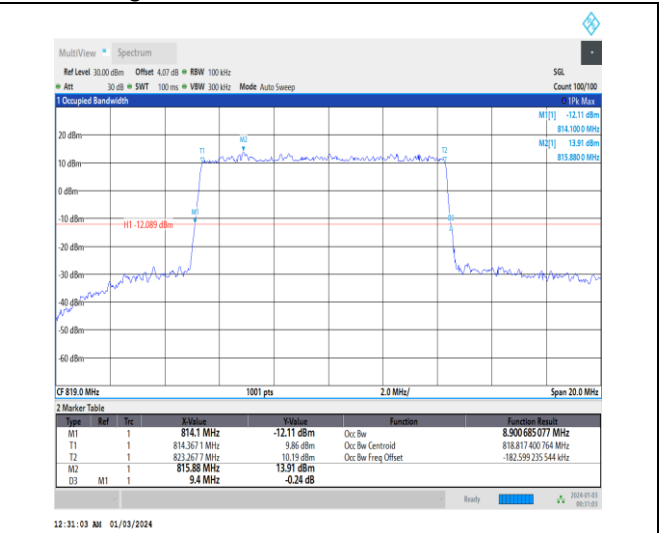
1-N26-814-824-15-10-M-1-DFT-QPSK-Outer_Full-50 @0-Ant0-8.901-9.400-≤10-PASS
