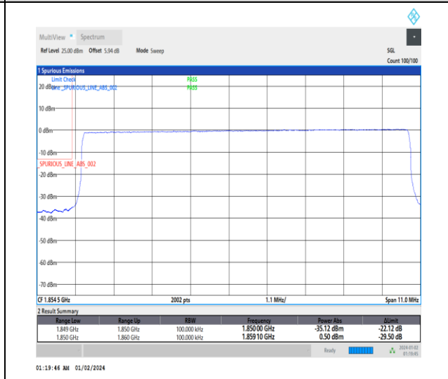
1-N25-15-10-L-6-CP-QPSK-Outer_Full-52@0-Ant3-1-seegraph-PASS-see graph
