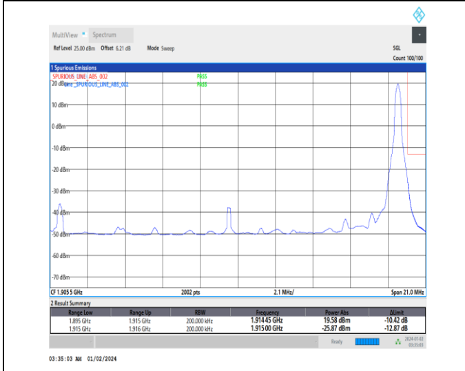
1-N25-15-20-H-5-CP-QPSK-Edge_1RB_Right-1@105-Ant3-1-seegraph-PASS-see graph
