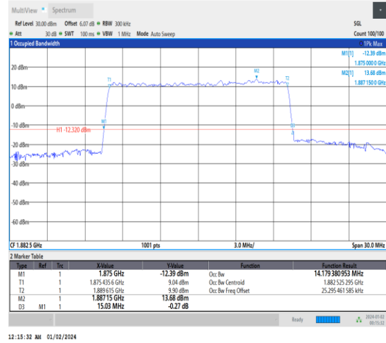
1-N25-15-15-M-8-CP-64QAM-Outer_Full-79@0-Ant 3-14.179-15.030-≤15-PASS
