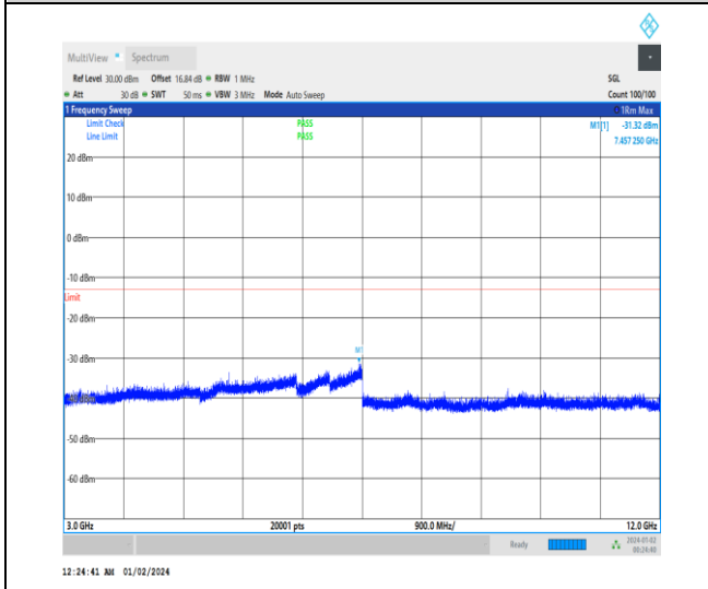
1-N25-15-20-M-1-DFT-PI2BPSK-Inner_1RB_Left-1 @ 1-3000-12000-Ant3-7457.25--31.32--13-PASS
