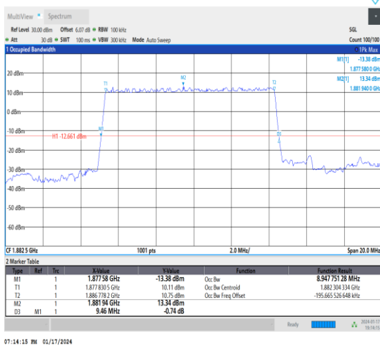
1-N25-15-10-M-2-DFT-PI2BPSK-Outer_Full-50@0-Ant3 nt3-8.948-9.460-≤10-PASS
