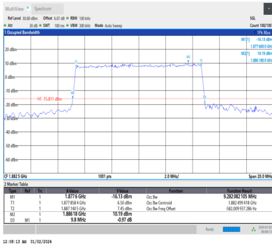
1-N25-15-10-M-6-CP-QPSK-Outer_Full-52@0-Ant3- 9.282-9.800-≤10-PASS
