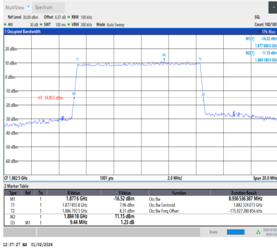
1-N25-15-10-M-4-DFT-64QAM-Outer_Full-50@0-Ant 3-8.937-9.440-≤10-PASS
