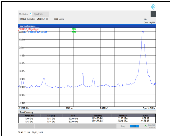
1-N25-15-15-H-2-DFT-PI2BPSK-Edge_1RB_Right-1@78-Ant3-1-seegraph-PASS-see graph
