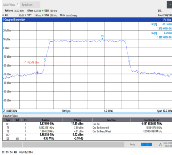
1-N25-15-5-M-9-CP-256QAM-Outer_Full-25@0-Ant3 -4.482-4.960-≤5-PASS
