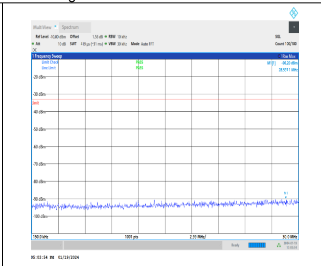
1-N25-15-20-H-1-DFT-PI2BPSK-Inner_1RB_Left-1 @ 1-0.15-30-Ant3-28.59--90.20--33-PASS
