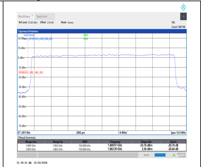
1-N25-15-15-L-3-DFT-PI2BPSK-Outer_Full-75@0-Ant3-1-seegraph-PASS-see graph
