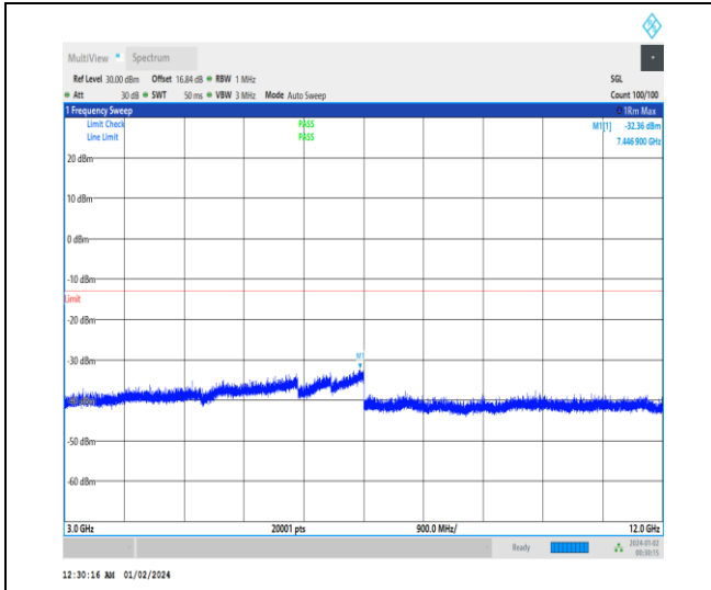
1-N25-15-20-H-1-DFT-PI2BPSK-Inner_1RB_Left-1 @ 1-3000-12000-Ant3-7446.90--32.36--13-PASS
