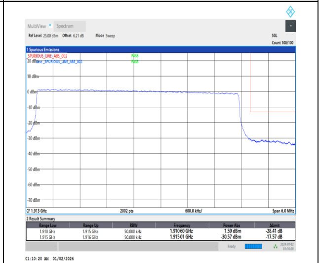
1-N25-15-5-H-6-CP-QPSK-Outer_Full-25@0-Ant3-1-seegraph-PASS-see graph
