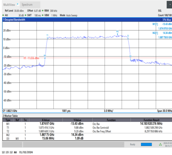
1-N25-15-15-M-7-CP-16QAM-Outer_Full-79@0-Ant3 -14.184-15.060-≤15-PASS
