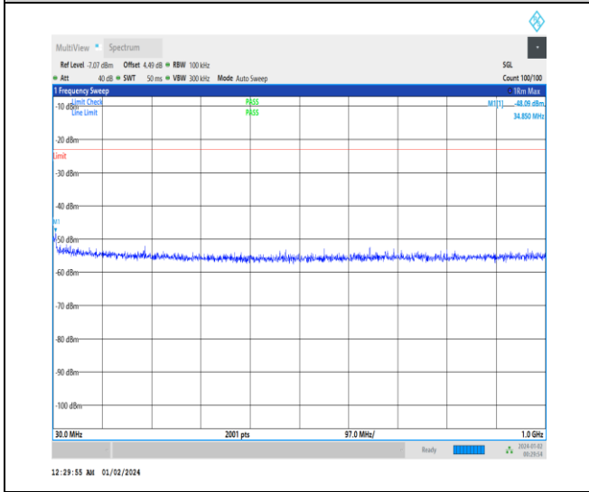
1-N25-15-20-H-1-DFT-PI2BPSK-Inner_1RB_Left-1 @ 1-30-1000-Ant3-34.85--48.09--23-PASS
