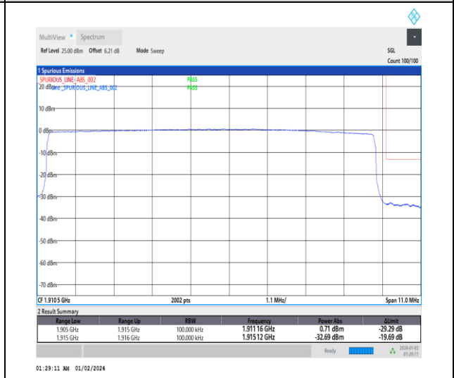
1-N25-15-10-H-6-CP-QPSK-Outer_Full-52@0-Ant3-1-seegraph-PASS-see graph
