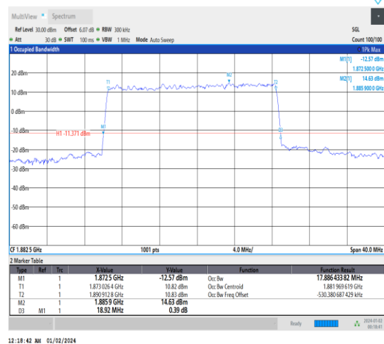
1-N25-15-20-M-1-DFT-QPSK-Outer_Full-100@0-An t3-17.886-18.920-≤20-PASS
