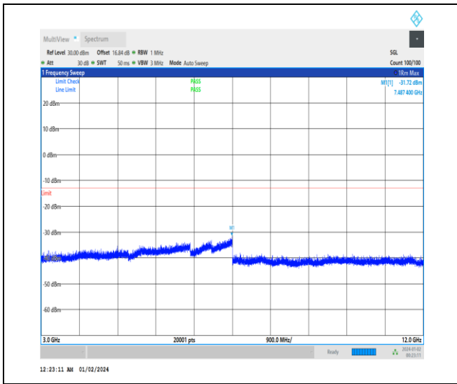
1-N25-15-20-L-1-DFT-PI2BPSK-Inner_1RB_Left-1 @ 1-3000-12000-Ant3-7487.40--31.72--13-PASS
