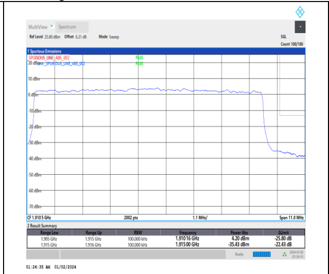
1-N25-15-10-H-3-DFT-PI2BPSK-Outer_Full-50@0-Ant3-1-seegraph-PASS-see graph
