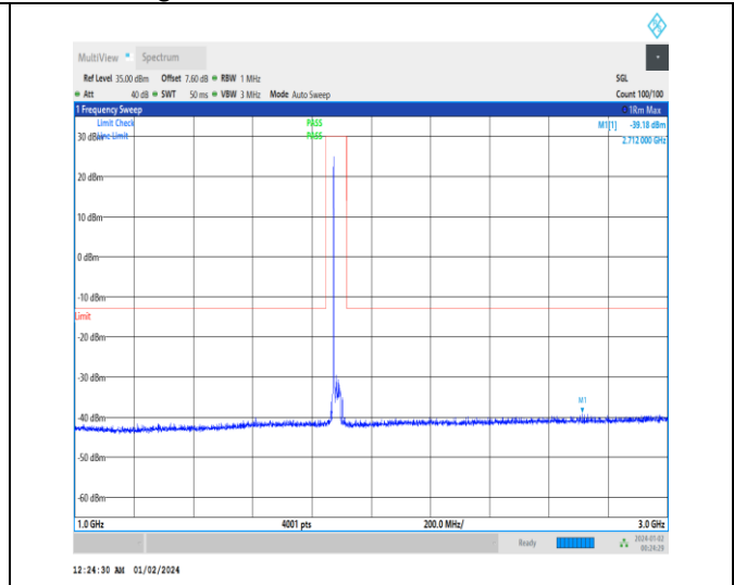
1-N25-15-20-M-1-DFT-PI2BPSK-Inner_1RB_Left-1 @ 1-1000-3000-Ant3-2712.00--39.18--13-PASS
