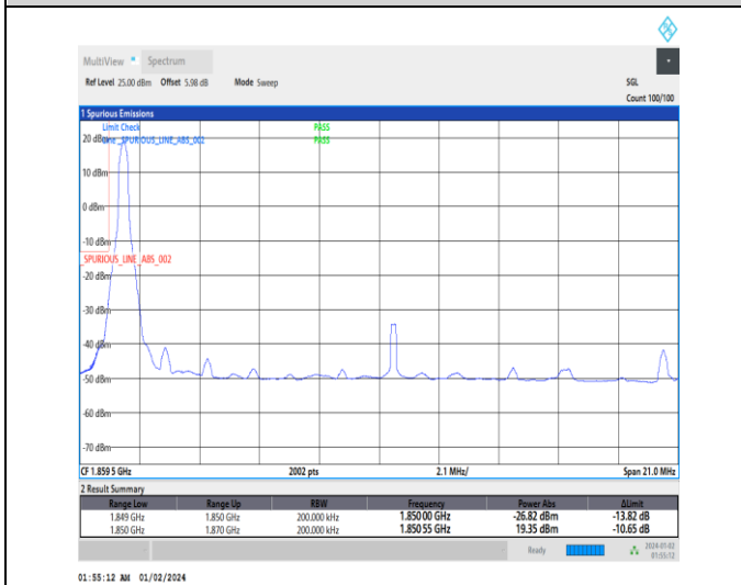
1-N25-15-20-L-4-CP-QPSK-Edge_1RB_Left-1@0-Ant3-1-seegraph-PASS-see graph
