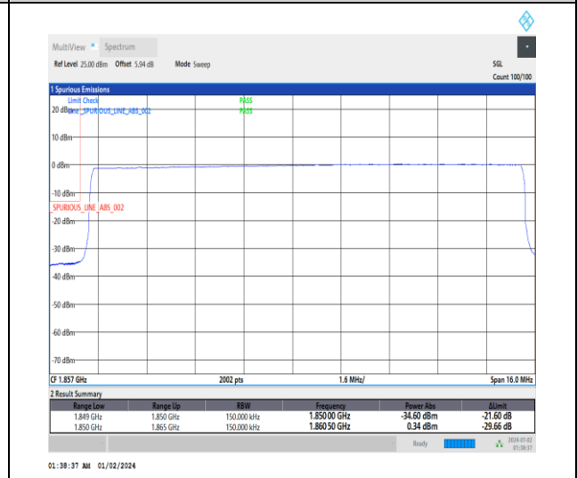
1-N25-15-15-L-6-CP-QPSK-Outer_Full-79@0-Ant3-1-seegraph-PASS-see graph
