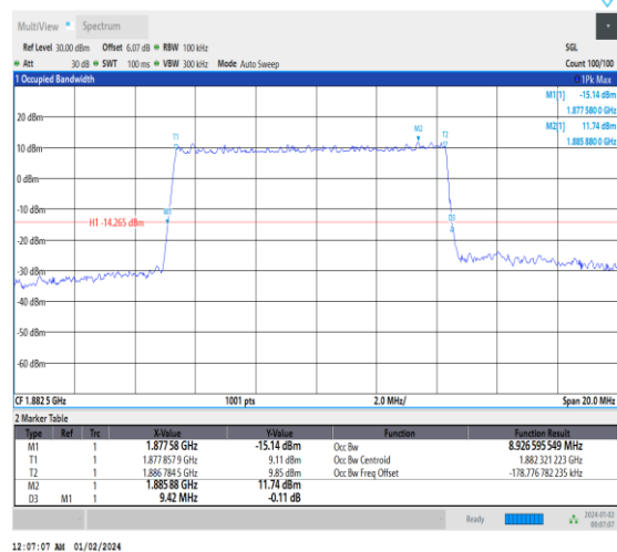
1-N25-15-10-M-3-DFT-16QAM-Outer_Full-50@0-Ant3 t3-8.927-9.420-≤10-PASS
