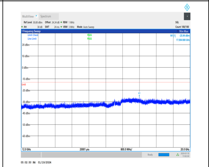
1-N25-15-20-M-1-DFT-PI2BPSK-Inner_1RB_Left-1 @ 1-12000-20000-Ant3-17594--25.94
