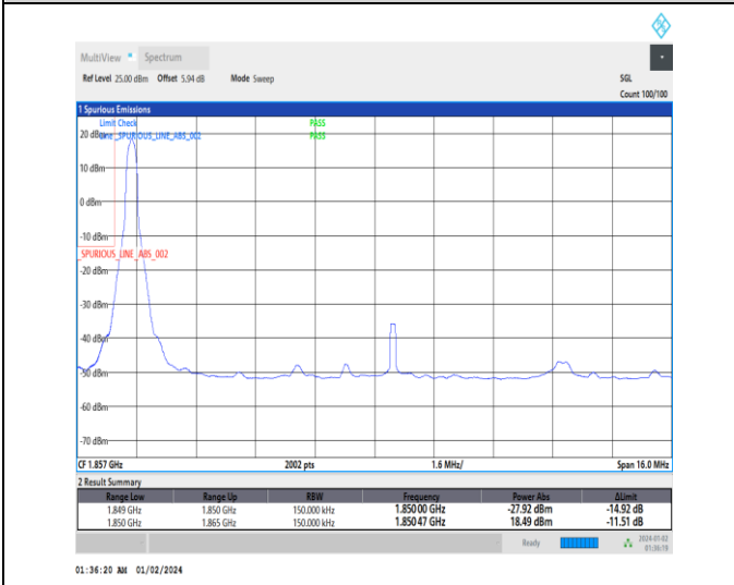
1-N25-15-15-L-4-CP-QPSK-Edge_1RB_Left-1@0-Ant3-1-seegraph-PASS-see graph
