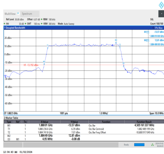
1-N25-15-5-M-8-CP-64QAM-Outer_Full-25@0-Ant3- 4.505-4.950-≤5-PASS
