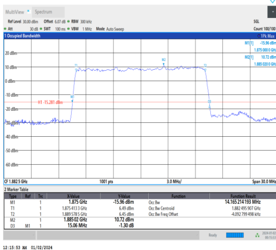
1-N25-15-15-M-9-CP-256QAM-Outer_Full-79@0-Ant 3-14.165-15.060-≤15-PASS
