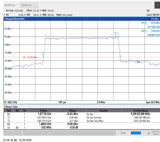
1-N25-15-10-M-7-CP-16QAM-Outer_Full-52@0-Ant 3-9.299-9.820-≤10-PASS
