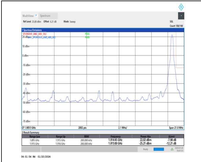
1-N25-15-20-H-3-DFT-PI2BPSK-Outer_Full-1105@0-Ant3-1-seegraph-PASS-see graph
