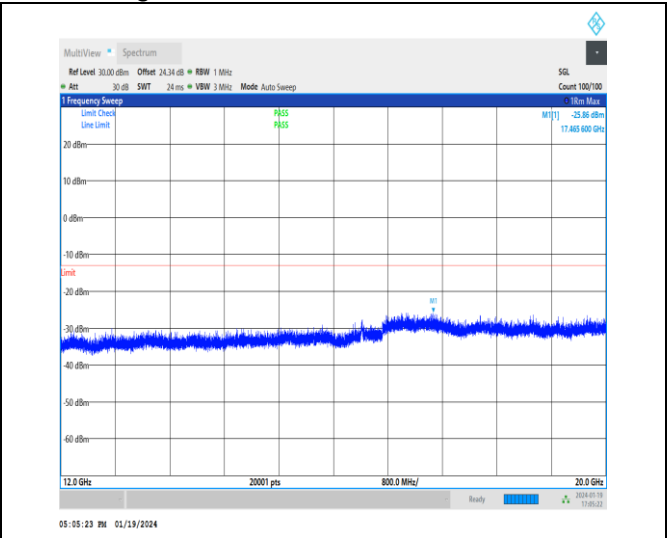
1-N25-15-20-H-1-DFT-PI2BPSK-Inner_1RB_Left-1 @ 1-12000-20000-Ant3-17465.60--25.86--13-PASS
