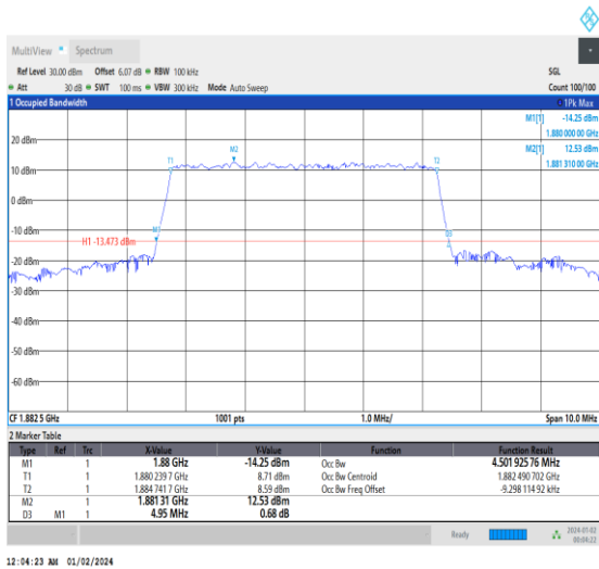
1-N25-15-5-M-7-CP-16QAM-Outer_Full-25@0-Ant3- 4.502-4.950-≤5-PASS
