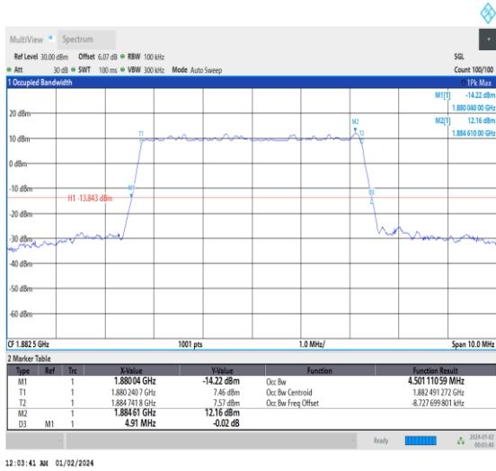
1-N25-15-5-M-5-DFT-256QAM-Outer_Full-25@0-Ant 3-4.501-4.910-≤5-PASS
