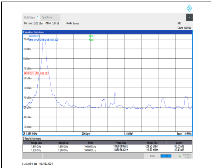
1-N25-15-10-L-1-DFT-PI2BPSK-Edge_1RB_Left-1@0-Ant3-1-seegraph-PASS-see graph
