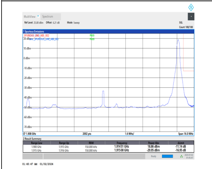
1-N25-15-15-H-5-CP-QPSK-Edge_1RB_Right-1@78-Ant3-1-seegraph-PASS-see graph
