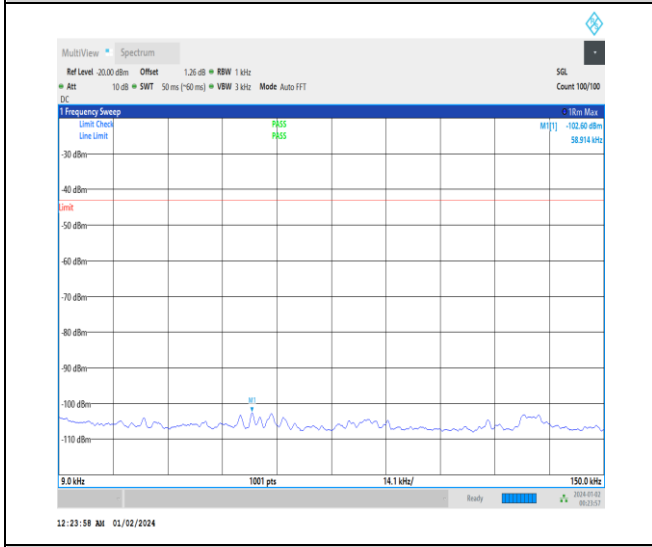
1-N25-15-20-M-1-DFT-PI2BPSK-Inner_1RB_Left-1 @ 1-0.009-0.15-Ant3-0.06--102.60--43-PASS
