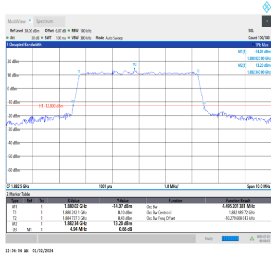
1-N25-15-5-M-6-CP-QPSK-Outer_Full-25@0-Ant3-4 .495-4.940-≤5-PASS
