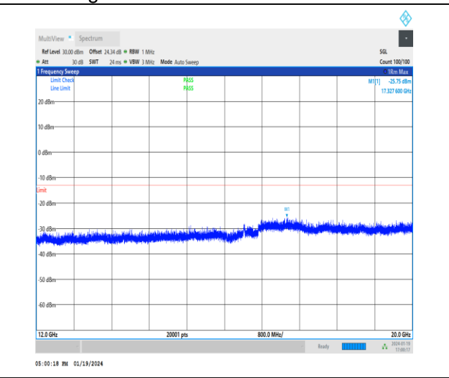
1-N25-15-20-L-1-DFT-PI2BPSK-Inner_1RB_Left-1 @ 1-12000-20000-Ant3-17327.60--25.75--13-PASS
