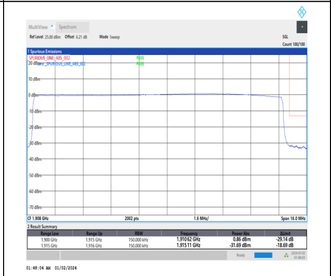
1-N25-15-15-H-6-CP-QPSK-Outer_Full-79@0-Ant3-1-seegraph-PASS-see graph
