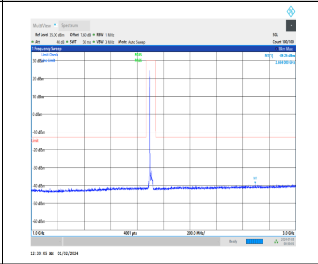
1-N25-15-20-H-1-DFT-PI2BPSK-Inner_1RB_Left-1 @ 1-1000-3000-Ant3-2694.00--39.25--13-PASS
