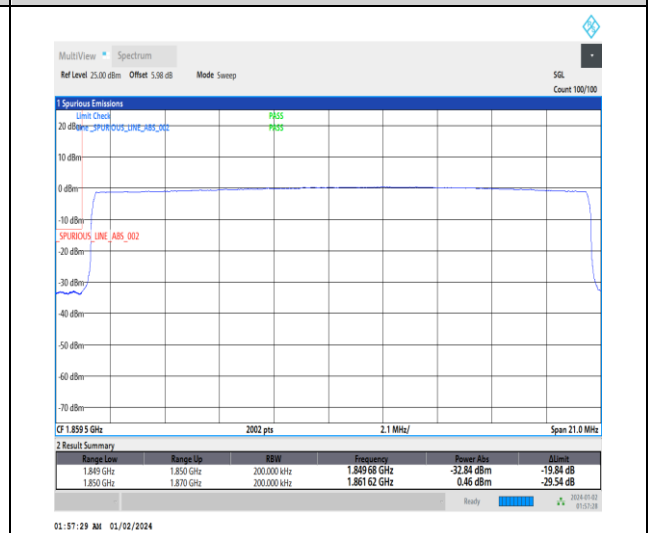
1-N25-15-20-L-6-CP-QPSK-Outer_Full-106@0-Ant3-1-seegraph-PASS-see graph
