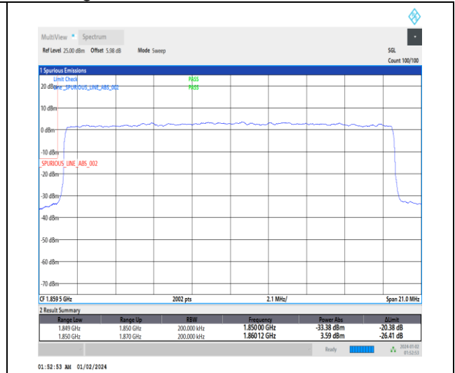
1-N25-15-20-L-3-DFT-PI2BPSK-Outer_Full-100@0-Ant3-1-seegraph-PASS-see graph
