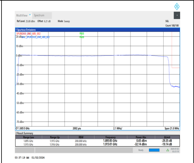
1-N25-15-20-H-6-CP-QPSK-Outer_Full-106@0-Ant3-1-seegraph-PASS-see graph
