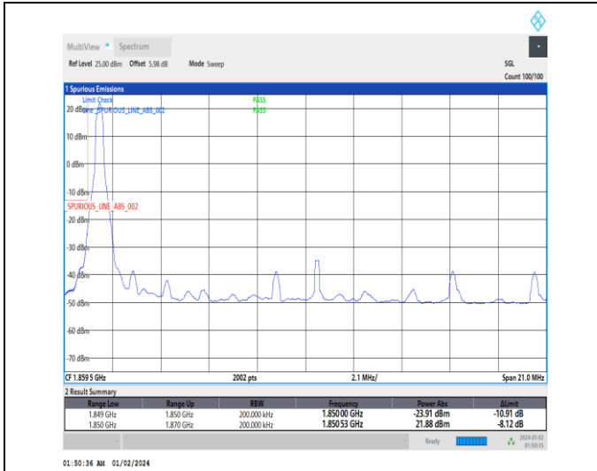
1-N25-15-20-L-1-DFT-PI2BPSK-Edge_1RB_Left-1@0-Ant3-1-seegraph-PASS-see graph
