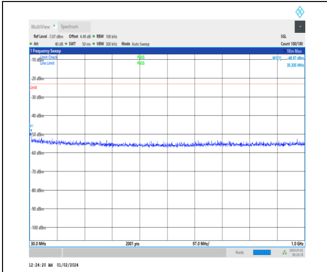
1-N25-15-20-M-1-DFT-PI2BPSK-Inner_1RB_Left-1 @ 1-30-1000-Ant3-35.34--48.97--23-PASS
