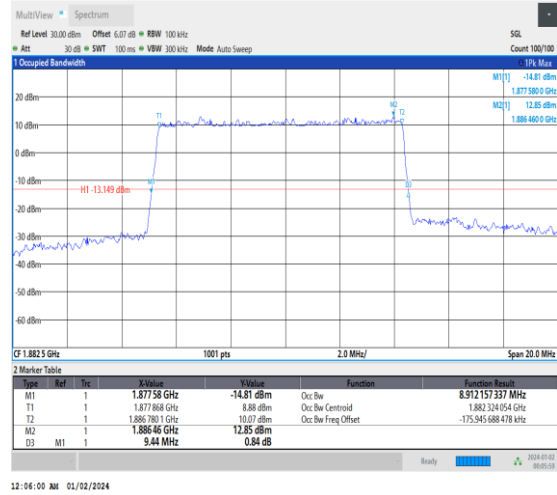
1-N25-15-10-M-1-DFT-QPSK-Outer_Full-50@0-Ant 3-8.912-9.440-≤10-PASS
