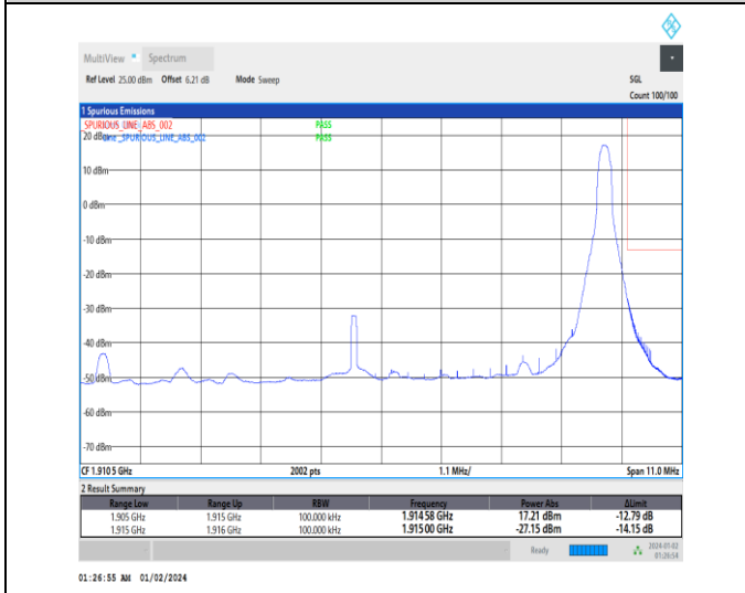
1-N25-15-10-H-5-CP-QPSK-Edge_1RB_Right-1@51-Ant3-1-seegraph-PASS-see graph
