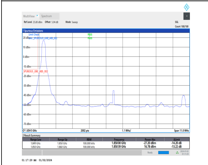
1-N25-15-10-L-4-CP-QPSK-Edge_1RB_Left-1@0-Ant3-1-seegraph-PASS-see graph
