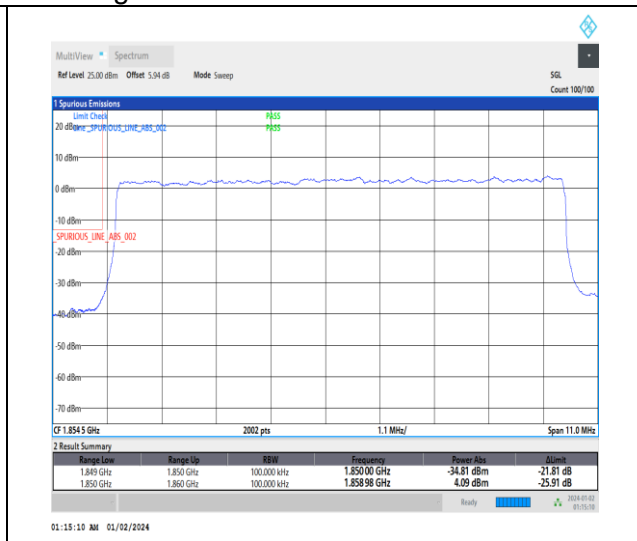
1-N25-15-10-L-3-DFT-PI2BPSK-Outer_Full-50@0-Ant3-1-seegraph-PASS-see graph
