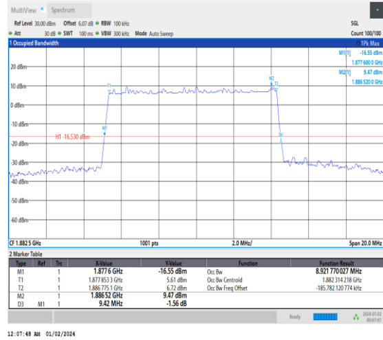
1-N25-15-10-M-5-DFT-256QAM-Outer_Full-50@0-A nt3-8.922-9.420-≤10-PASS
