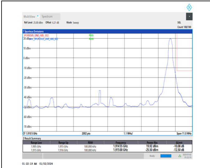
1-N25-15-10-H-2-DFT-PI2BPSK-Edge_1RB_Right-1@51-Ant3-1-seegraph-PASS-see graph
