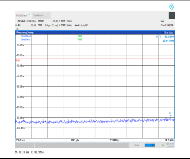
1-N25-15-20-M-1-DFT-PI2BPSK-Inner_1RB_Left-1 @ 1-0.15-30-Ant3-29.19--89.29--33-PASS
