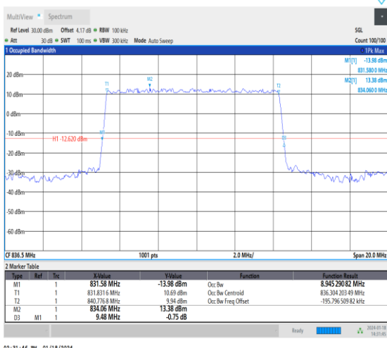
1-N5-15-10-M-2-DFT-PI2BPSK-Outer_Full-50@0-Ant0-8.945-9.480-≤10-PASS
