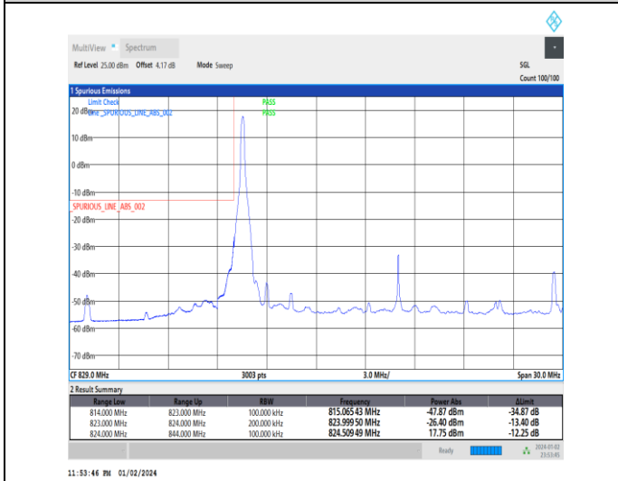
1-N5-15-20-L-4-CP-QPSK-Edge_1RB_Left-1@0-Ant0-1--PASS-see graph
