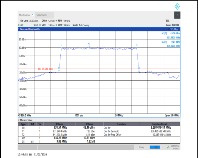
1-N5-15-10-M-7-CP-16QAM-Outer_Full-52@0-Ant0-9 9.298-9.880-≤10-PASS
