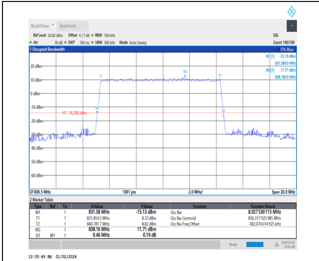
1-N5-15-10-M-4-DFT-64QAM-Outer_Full-50@0-Ant 0-8.928-9.460-≤10-PASS
