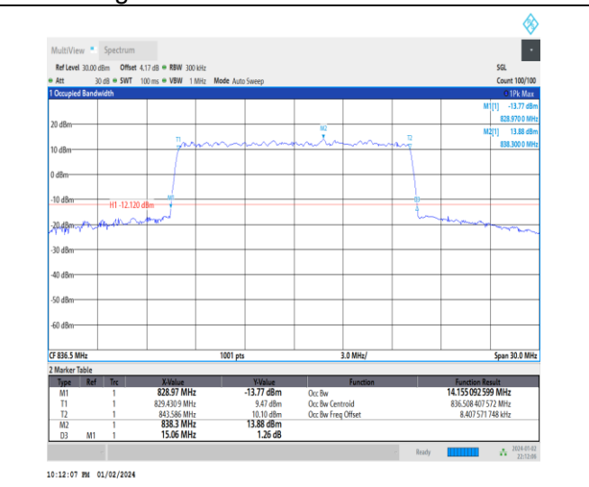
1-N5-15-15-M-8-CP-64QAM-Outer_Full-79@0-Ant0-14.155-15.060-≤15-PASS
