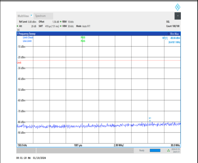
1-N5-15-20-H-1-DFT-PI2BPSK-Inner_1RB_Left-1@ 1 -0.15-30-Ant0-24.42--80.04--23-PASS
