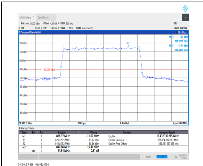
1-N5-15-15-M-3-DFT-16QAM-Outer_Full-75@0-Ant 0-13.433-14.340-≤15-PASS
