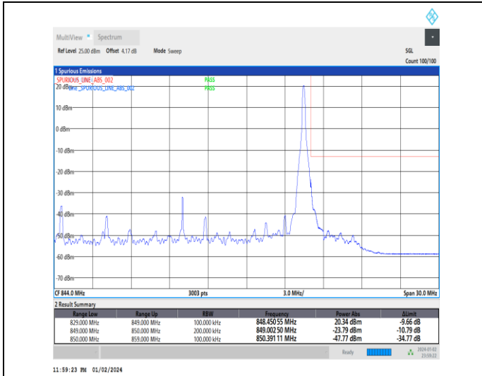
1-N5-15-20-H-2-DFT-PI2BPSK-Edge_1RB_Right-1@105-Ant0-1--PASS-see graph
