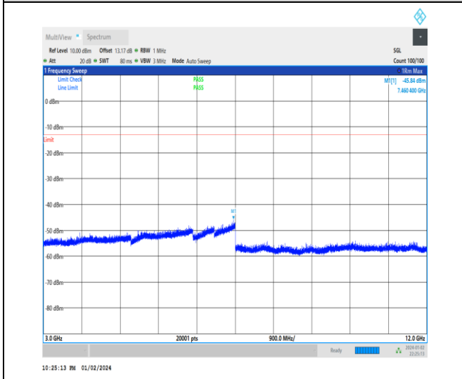
1-N5-15-20-H-1-DFT-PI2BPSK-Inner_1RB_Left-1@1 -3000-12000-Ant0-7460.40--45.84--13-PASS
