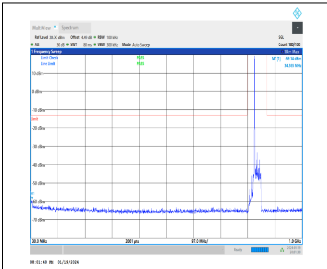
1-N5-15-20-H-1-DFT-PI2BPSK-Inner_1RB_Left-1@1 -30-1000-Ant0-34.37--59.14--13-PASS
