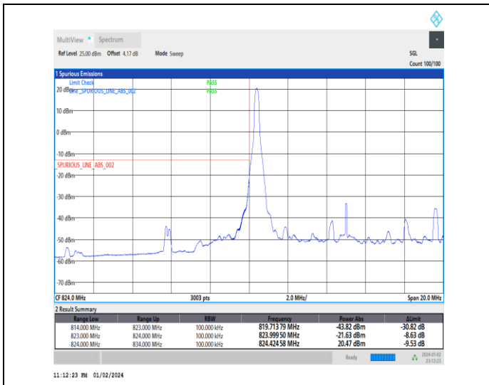
1-N5-15-10-L-1-DFT-PI2BPSK-Edge_1RB_Left-1@0-A nt0-1--PASS-see graph
