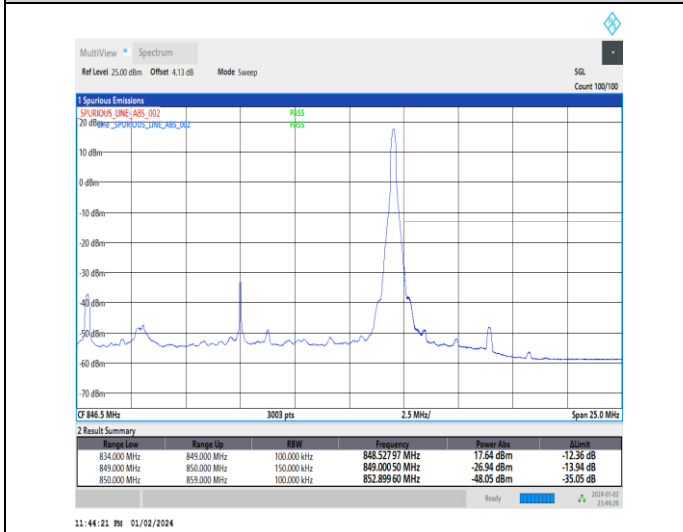
1-N5-15-15-H-5-CP-QPSK-Edge_1RB_Right-1@78-Ant0-1--PASS-see graph
