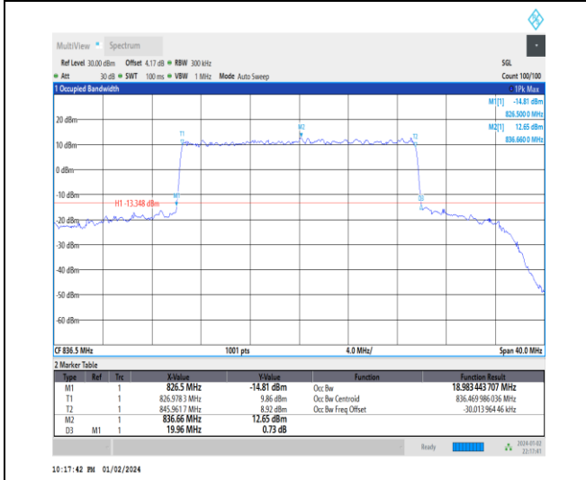
1-N5-15-20-M-8-CP-64QAM-Outer_Full-106@0-Ant0-18.983-19.960-≤20-PASS
