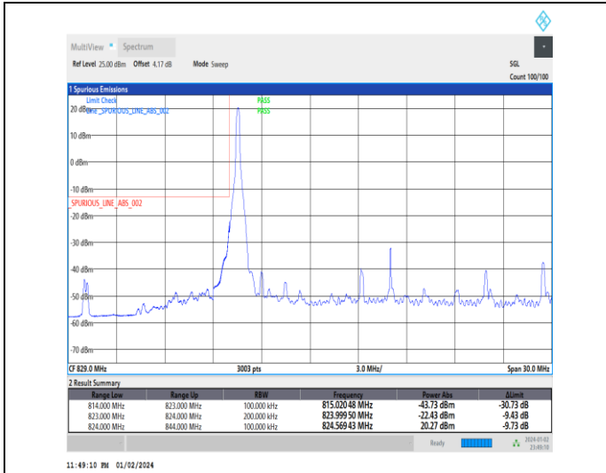
1-N5-15-20-L-1-DFT-PI2BPSK-Edge_1RB_Left-1@0-Ant0-1--PASS-see graph
