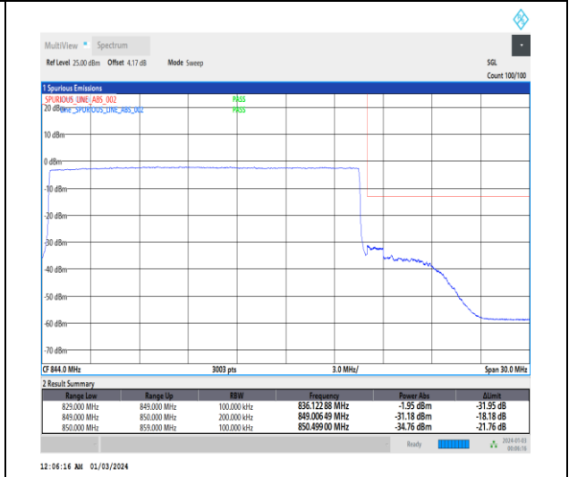
1-N5-15-20-H-6-CP-QPSK-Outer_Full-106@0-Ant0-1--PASS-see graph
