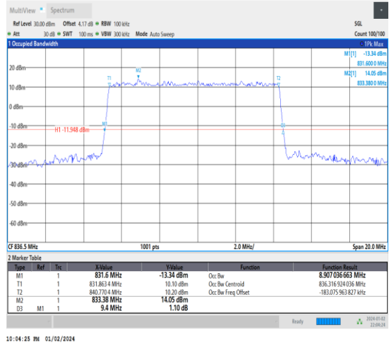
1-N5-15-10-M-1-DFT-QPSK-Outer_Full-50@0-Ant0-8.907-9.400-≤10-PASS
