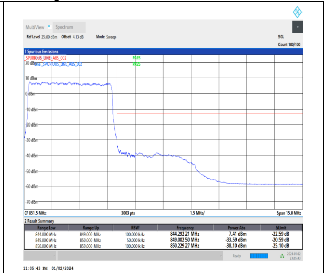
1-N5-15-5-H-3-DFT-PI2BPSK-Outer_Full-25@0-Ant0-1--PASS-see graph
