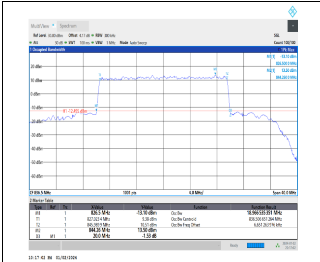
1-N5-15-20-M-6-CP-QPSK-Outer_Full-106@0-Ant0-18.967-20.000-≤20-PASS
