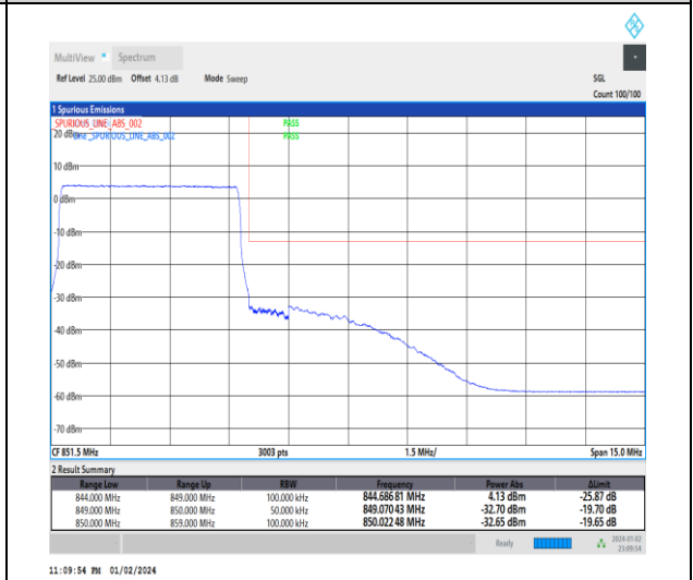
1-N5-15-5-H-6-CP-QPSK-Outer_Full-25@0-Ant0-1--PASS-see graph
