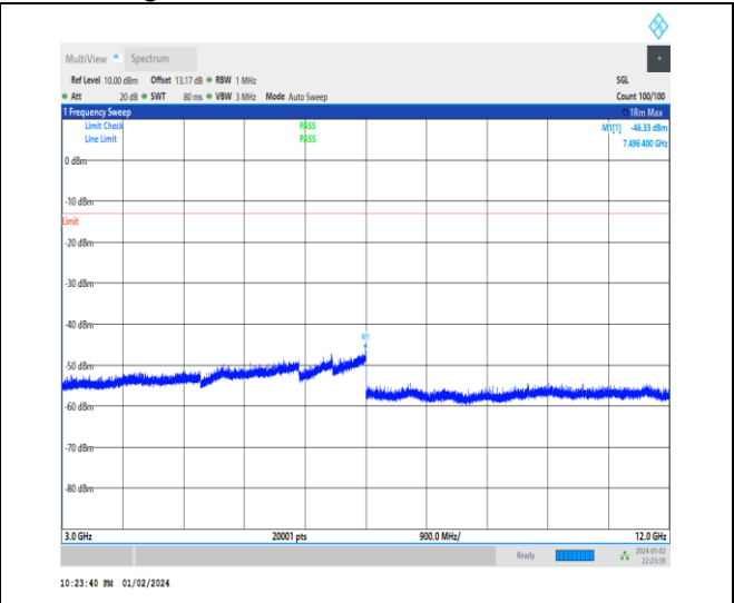
1-N5-15-20-M-1-DFT-PI2BPSK-Inner_1RB_Left-1@ 1-3000-12000-Ant0-7496.40--46.33--13-PASS
