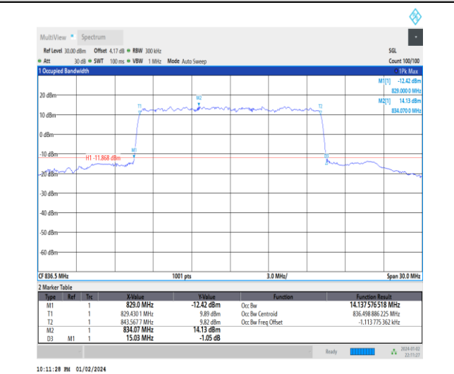
1-N5-15-15-M-6-CP-QPSK-Outer_Full-79@0-Ant0-1 4.138-15.030-≤15-PASS
