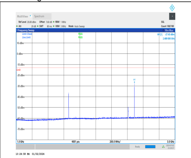
1-N5-15-20-H-1-DFT-PI2BPSK-Inner_1RB_Left-1@1 -1000-3000-Ant0-2489.00--27.43--13-PASS
