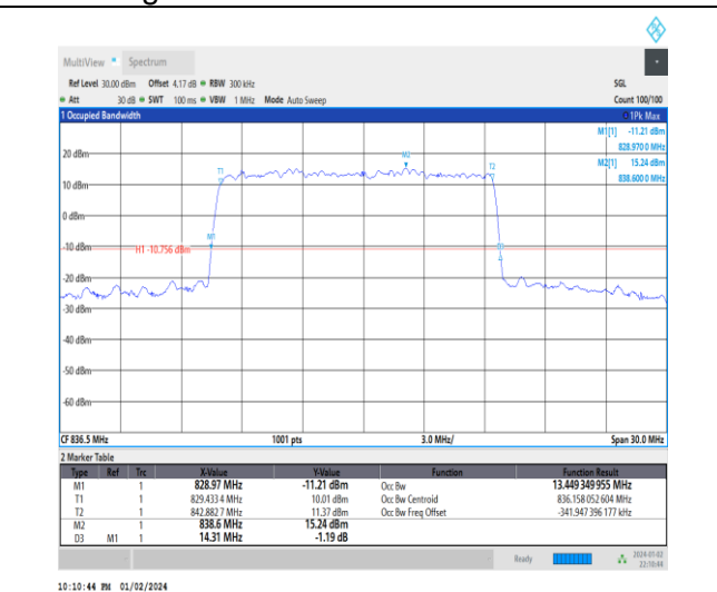
1-N5-15-15-M-4-DFT-64QAM-Outer_Full-75@0-Ant0 -13.449-14.310-≤15-PASS
