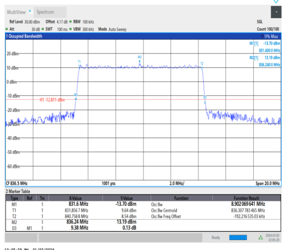
1-N5-15-10-M-3-DFT-16QAM-Outer_Full-50@0-Ant0-8.902-9.380-≤10-PASS
