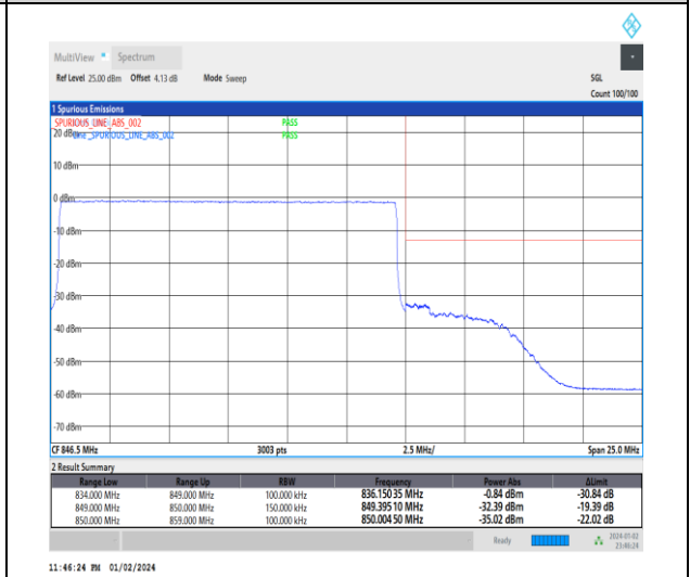
1-N5-15-15-H-6-CP-QPSK-Outer_Full-79@0-Ant0-1--PASS-see graph
