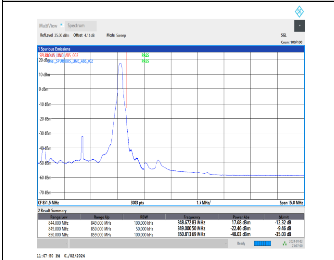
1-N5-15-5-H-5-CP-QPSK-Edge_1RB_Right-1@24-Ant0-1--PASS-see graph
