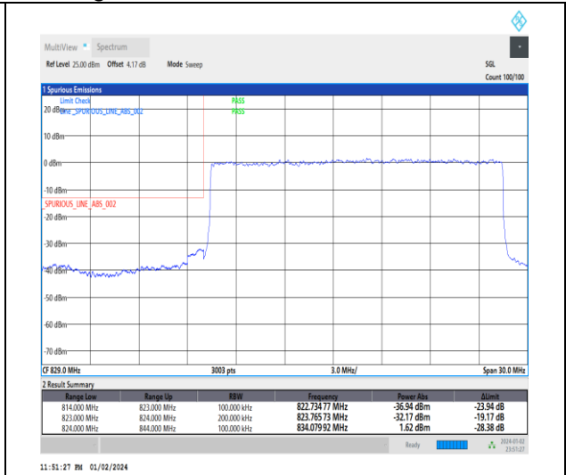
1-N5-15-20-L-3-DFT-PI2BPSK-Outer_Full-100@0-Ant0-1--PASS-see graph
