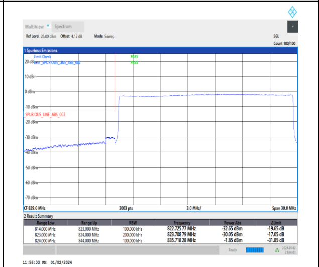
1-N5-15-20-L-6-CP-QPSK-Outer_Full-106@0-Ant0-1--PASS-see graph
