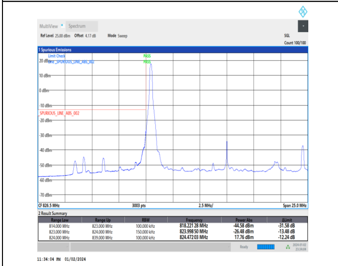
1-N5-15-15-L-4-CP-QPSK-Edge_1RB_Left-1@0-Ant0-1--PASS-see graph
