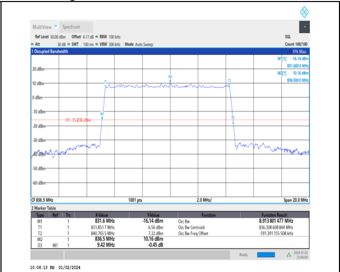
1-N5-15-10-M-5-DFT-256QAM-Outer_Full-50@0-Ant 0-8.914-9.420-≤10-PASS
