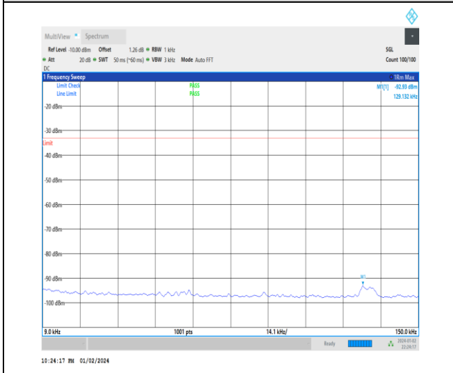
1-N5-15-20-H-1-DFT-PI2BPSK-Inner_1RB_Left-1@ 1 -0.009-0.15-Ant0-0.13--92.93--33-PASS
