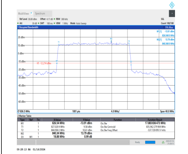
1-N5-15-20-M-4-DFT-64QAM-Outer_Full-100@0-Ant 0-17.884-18.880-≤20-PASS
