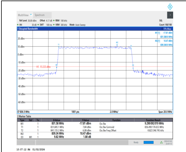
1-N5-15-10-M-8-CP-64QAM-Outer_Full-52@0-Ant0-9.29-9.820-≤10-PASS
