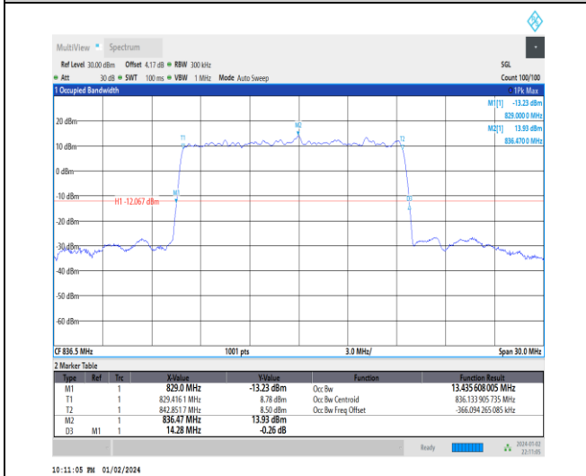
1-N5-15-15-M-5-DFT-256QAM-Outer_Full-75@0-An t0-13.436-14.280-≤15-PASS
