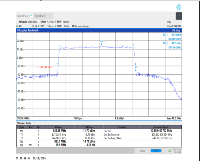
1-N5-15-20-M-3-DFT-16QAM-Outer_Full-100@0-Ant 0-17.856-18.800-≤20-PASS
