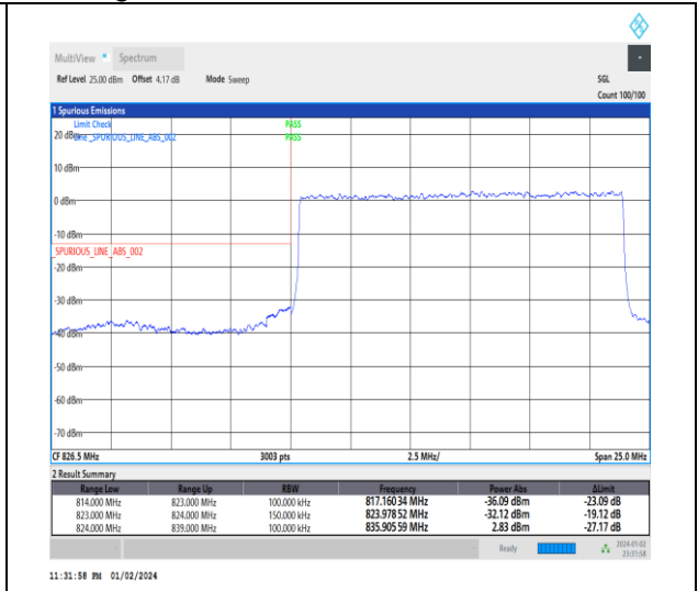
1-N5-15-15-L-3-DFT-PI2BPSK-Outer_Full-75@0-Ant0-1--PASS-see graph
