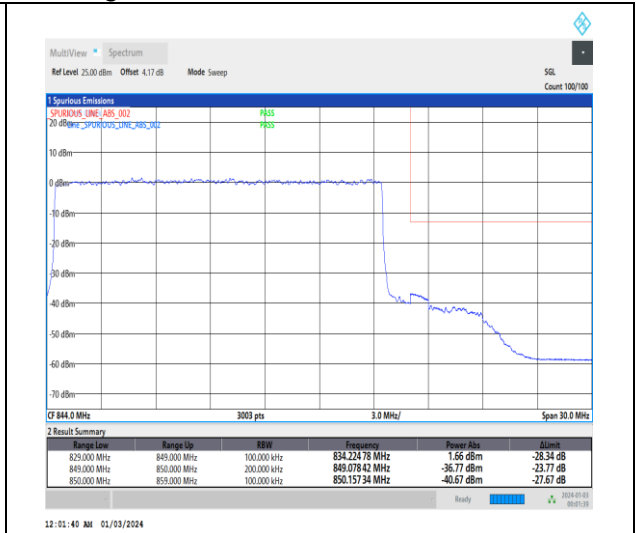
1-N5-15-20-H-3-DFT-PI2BPSK-Outer_Full-100@0-Ant0-1--PASS-see graph
