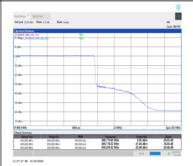
1-N5-15-10-H-6-CP-QPSK-Outer_Full-52@0-Ant0 -1--PASS-see graph
