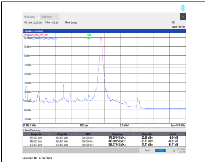
1-N5-15-10-H-2-DFT-PI2BPSK-Edge_1RB_Right-1@5 1-Ant0-1--PASS-see graph
