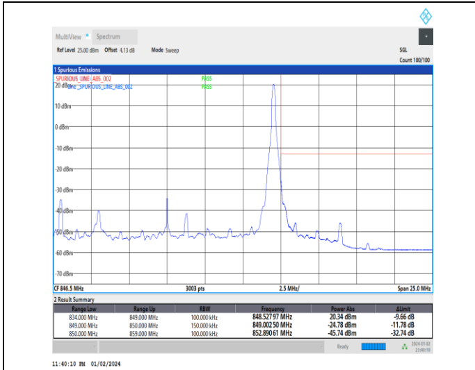
1-N5-15-15-H-2-DFT-PI2BPSK-Edge_1RB_Right-1@78-Ant0-1--PASS-see graph
