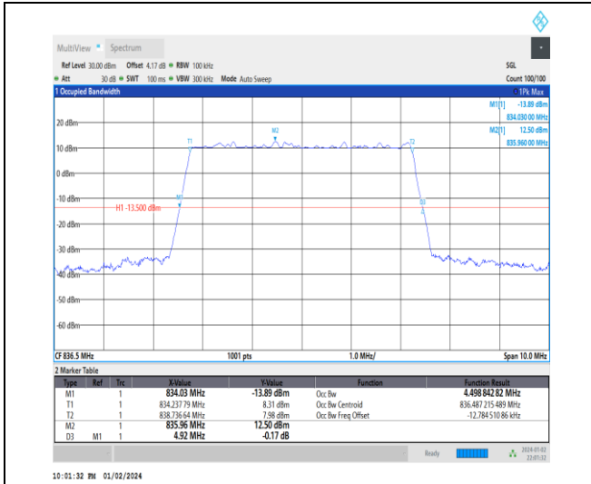
1-N5-15-5-M-5-DFT-256QAM-Outer_Full-25@0-Ant0-4.99-4.920-≤5-PASS
