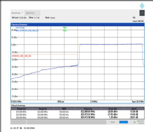
1-N5-15-10-L-6-CP-QPSK-Outer_Full-52@0-Ant0-1--PASS-see graph
