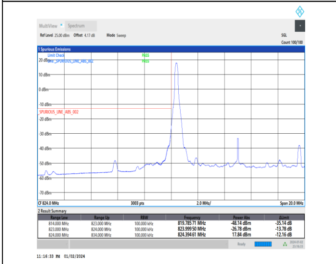
1-N5-15-10-L-4-CP-QPSK-Edge_1RB_Left-1@0-Ant0-1--PASS-see graph
