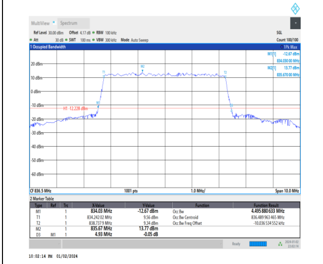
1-N5-15-5-M-7-CP-16QAM-Outer_Full-25@0-Ant0-4 .496-4.930-≤5-PASS
