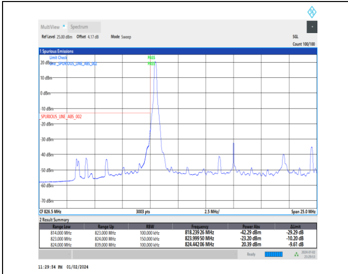
1-N5-15-15-L-1-DFT-PI2BPSK-Edge_1RB_Left-1@0-Ant0-1--PASS-see graph
