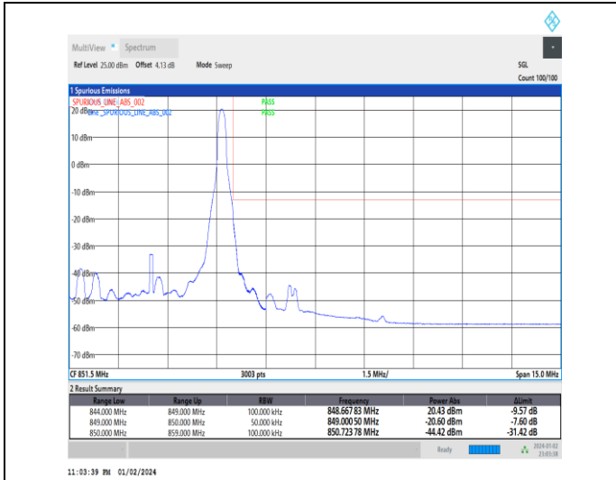
1-N5-15-5-H-2-DFT-PI2BPSK-Edge_1RB_Right-1@24-Ant0-1--PASS-see graph
