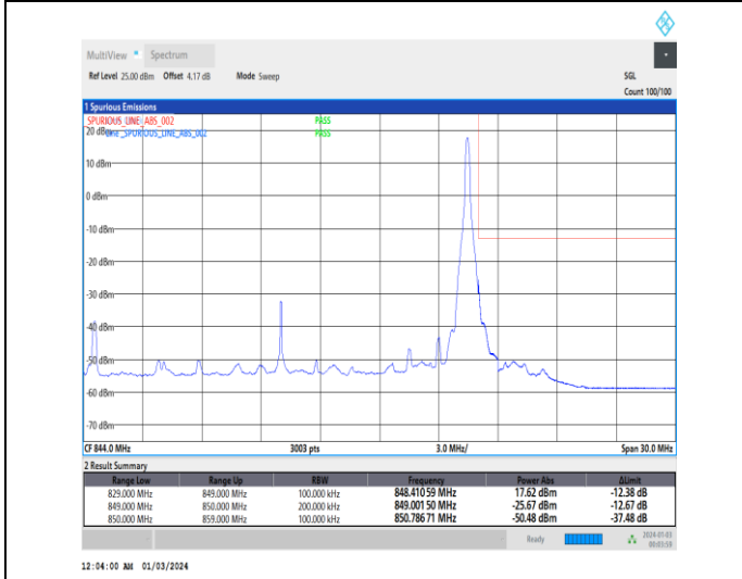
1-N5-15-20-H-5-CP-QPSK-Edge_1RB_Right-1@105-Ant0-1--PASS-see graph
