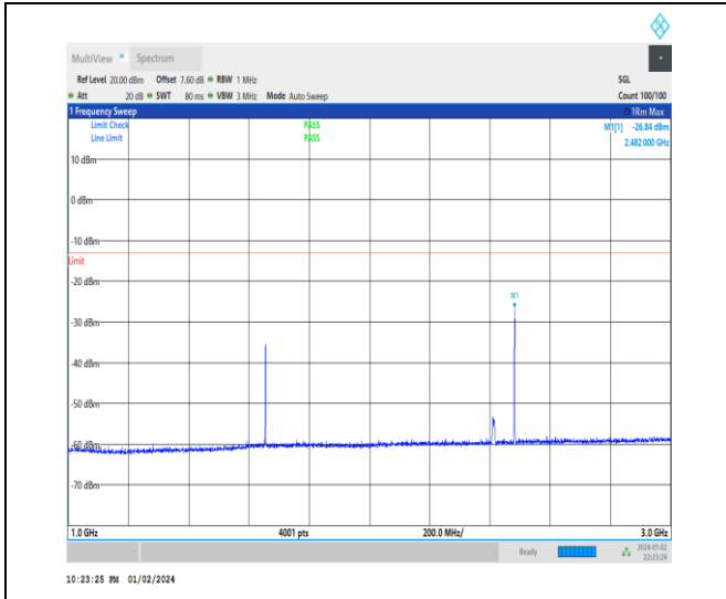
1-N5-15-20-M-1-DFT-PI2BPSK-Inner_1RB_Left-1@ 1-1000-3000-Ant0-2482.00--26.84--13-PASS
