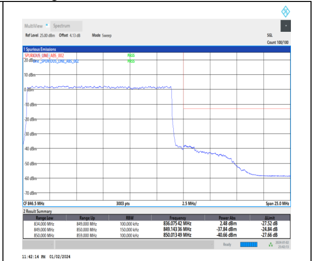
1-N5-15-15-H-3-DFT-PI2BPSK-Outer_Full-75@0-Ant0-1--PASS-see graph
