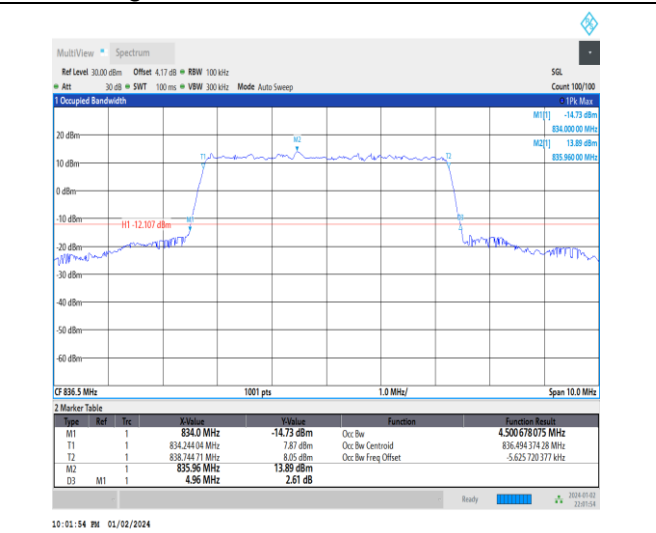
1-N5-15-5-M-6-CP-QPSK-Outer_Full-25@0-Ant0-4.5 01-4.960-≤5-PASS
