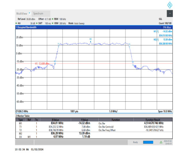
1-N5-15-5-M-8-CP-64QAM-Outer_Full-25@0-Ant0-4. 515-4.970-≤5-PASS
