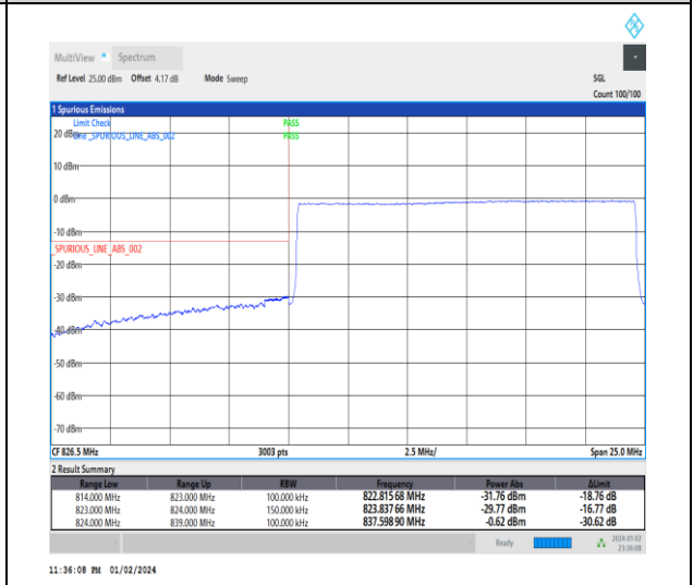
1-N5-15-15-L-6-CP-QPSK-Outer_Full-79@0-Ant0-1--PASS-see graph
