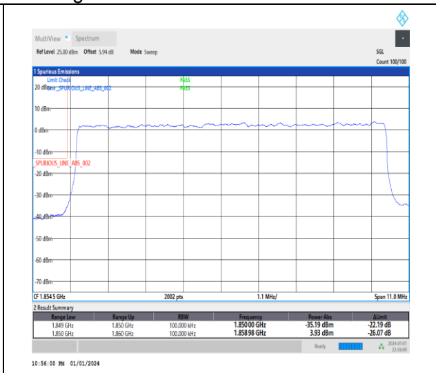
1-N2-15-10-L-3-DFT-PI2BPSK-Outer_Full-50@0-Ant3-1-seegraph-PASS-see graph
