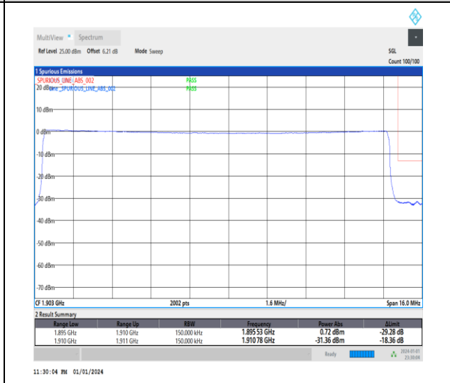
1-N2-15-15-H-6-CP-QPSK-Outer_Full-79@0-Ant3-1-seegraph-PASS-see graph
