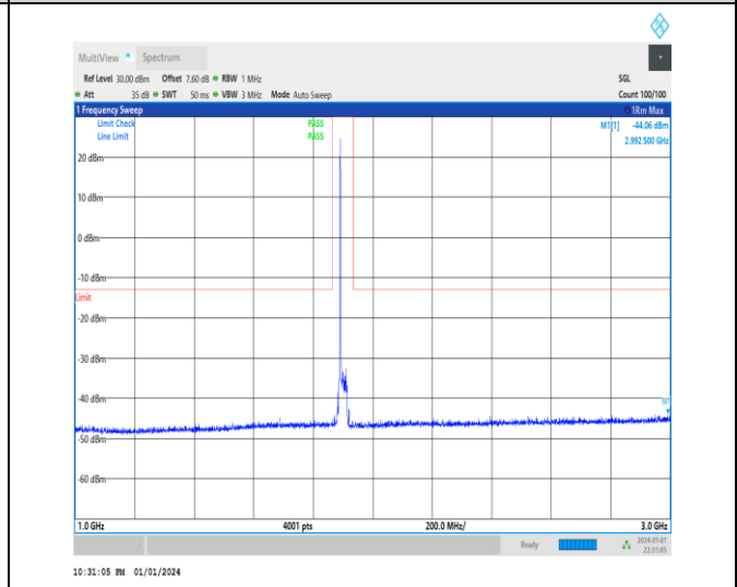
1-N2-15-20-H-1-DFT-PI2BPSK-Inner_1RB_Left-1@ -1000-3000-Ant3-2992.50--44.06--13-PASS
