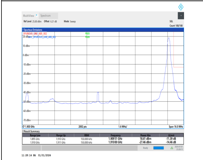
1-N2-15-15-H-5-CP-QPSK-Edge_1RB_Right-1@78-Ant3-1-seegraph-PASS-see graph
