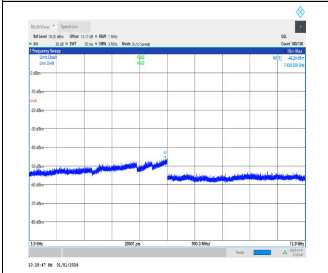
1-N2-15-20-M-1-DFT-PI2BPSK-Inner_1RB_Left-1@ 1-3000-12000-Ant3-7429.35--46.24--13-PASS
