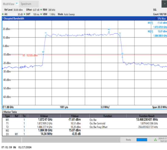
1-N2-15-15-M-3-DFT-16QAM-Outer_Full-75@0-Ant3 -13.468-14.340≤15-PASS
