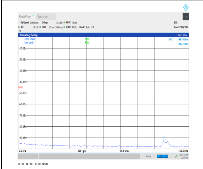
1-N2-15-20-M-1-DFT-PI2BPSK-Inner_1RB_Left-1@ 1-0.009-0.15-Ant3-0.13--93.33--43-PASS
