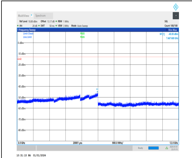
1-N2-15-20-H-1-DFT-PI2BPSK-Inner_1RB_Left-1@ 1-3000-12000-Ant3-7467.60--45.93--13-PASS
