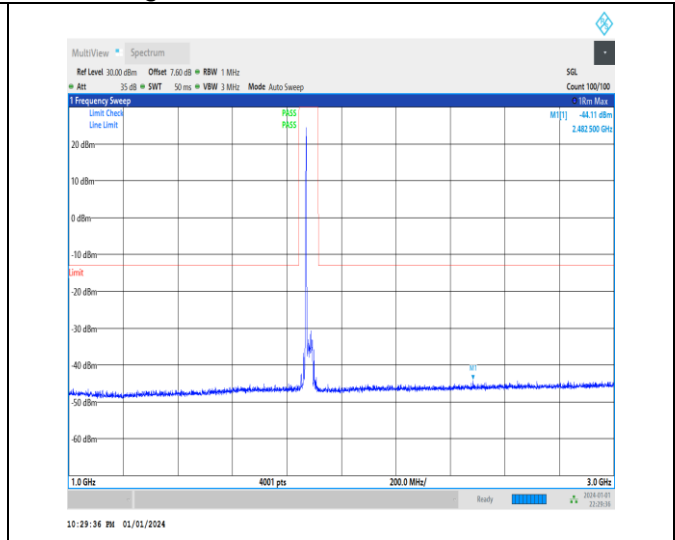
1-N2-15-20-M-1-DFT-PI2BPSK-Inner_1RB_Left-1@ 1 -1000-3000-Ant3-2482.50--44.11--13-PASS
