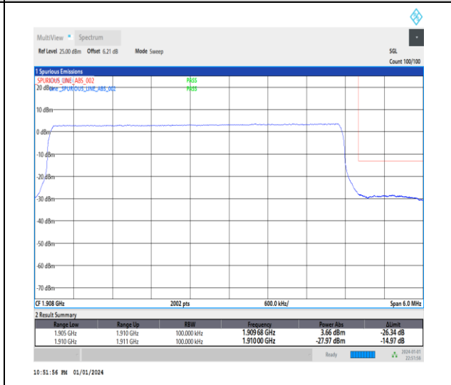
1-N2-15-5-H-6-CP-QPSK-Outer_Full-25@0-Ant3-1-seegraph-PASS-see graph
