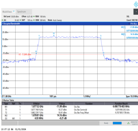
1-N2-15-5-M-7-CP-16QAM-Outer_Full-25@0-Ant3-4. 499-4.930-≤5-PASS
