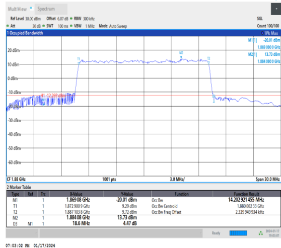
1-N2-15-15-M-6-CP-QPSK-Outer_Full-79@0-Ant3-1 4.203-18.600≤15-PASS
