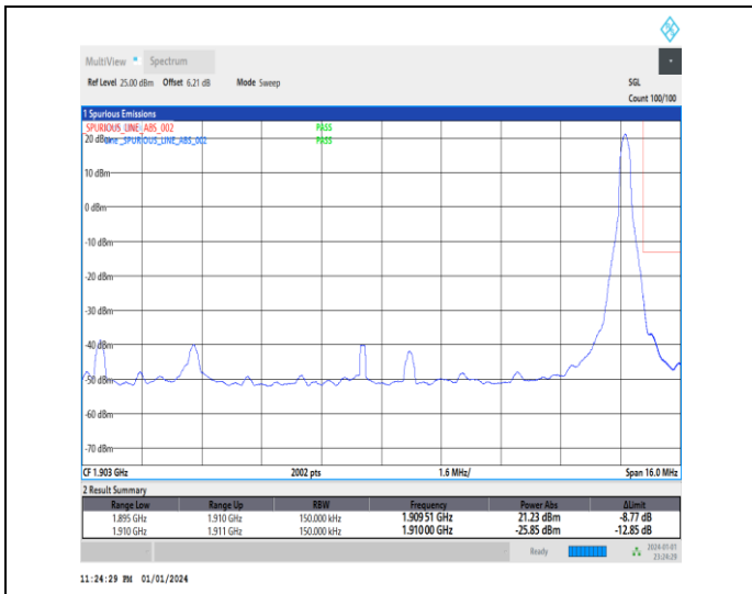
1-N2-15-15-H-2-DFT-PI2BPSK-Edge_1RB_Right-1@78-Ant3-1-seegraph-PASS-see graph
