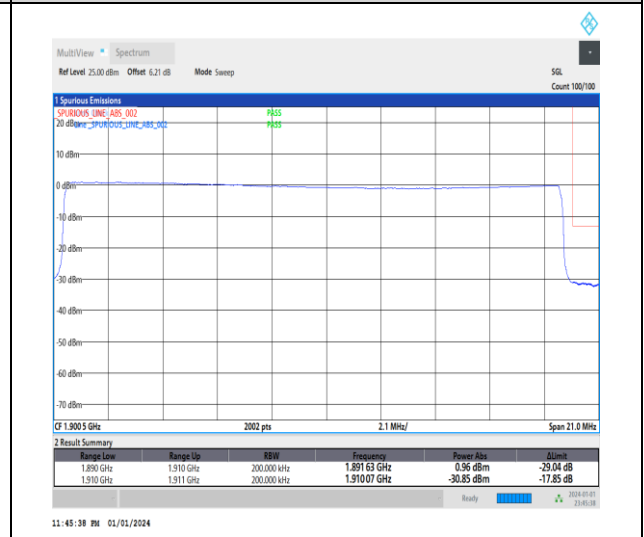
1-N2-15-20-H-6-CP-QPSK-Outer_Full-106@0-Ant3-1-seegraph-PASS-see graph
