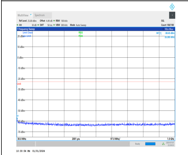
1-N2-15-20-H-1-DFT-PI2BPSK-Inner_1RB_Left-1@ 1-30-1000-Ant3-33.40--58.43--23-PASS
