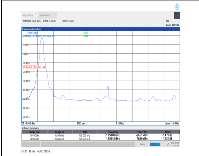
1-N2-15-10-L-4-CP-QPSK-Edge_1RB_Left-1@0-Ant3-1-seegraph-PASS-see graph
