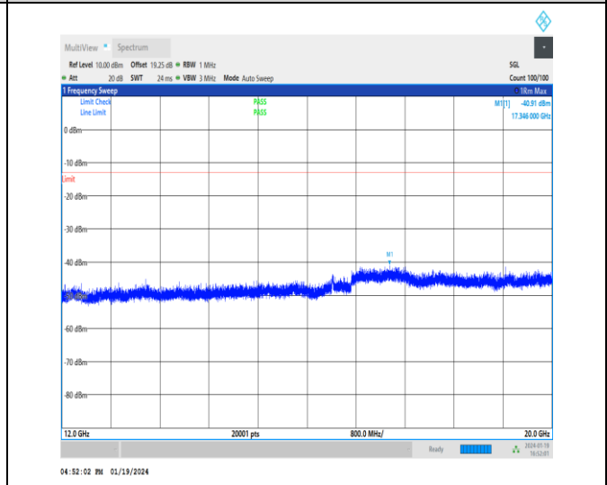
1-N2-15-20-M-1-DFT-PI2BPSK-Inner_1RB_Left-1@ 1 -12000-20000-Ant3-17346.00--40.91--13-PASS
