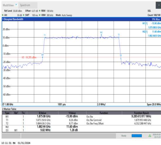
1-N2-15-10-M-6-CP-QPSK-Outer_Full-52@0-Ant3-9. 286-9.820≤10-PASS
