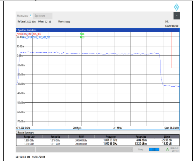
1-N2-15-20-H-3-DFT-PI2BPSK-Outer_Full-100@0-Ant3-1-seegraph-PASS-see graph
