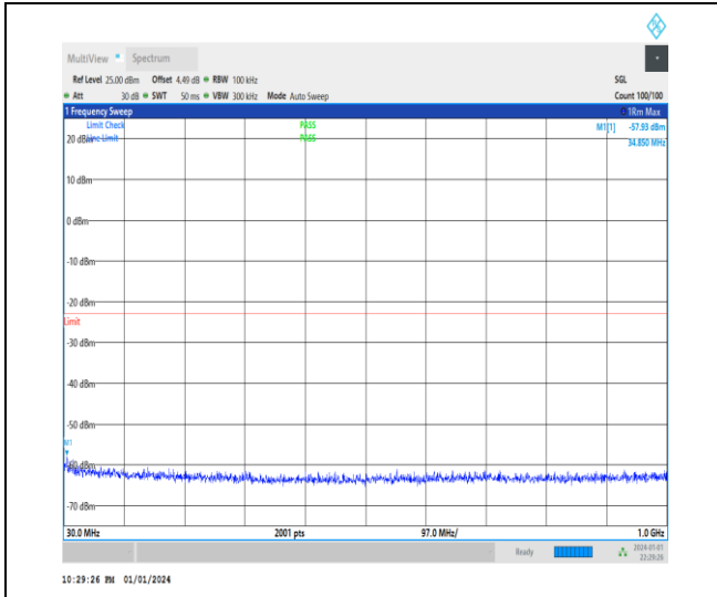
1-N2-15-20-M-1-DFT-PI2BPSK-Inner_1RB_Left-1@ 1-30-1000-Ant3-34.85--57.93--23-PASS
