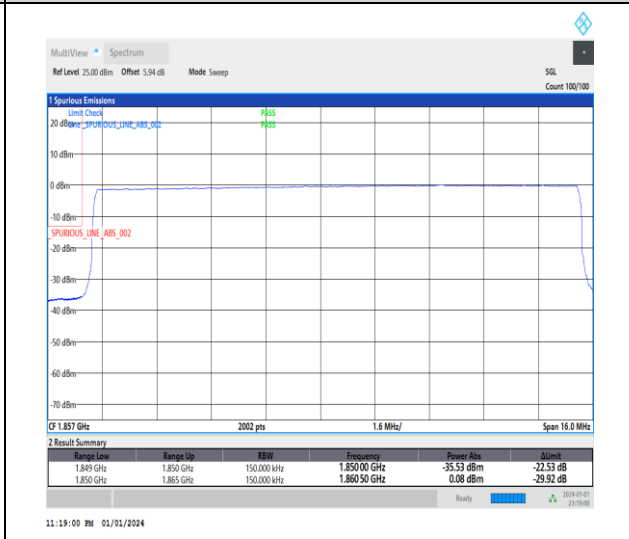
1-N2-15-15-L-6-CP-QPSK-Outer_Full-79@0-Ant3-1-seegraph-PASS-see graph
