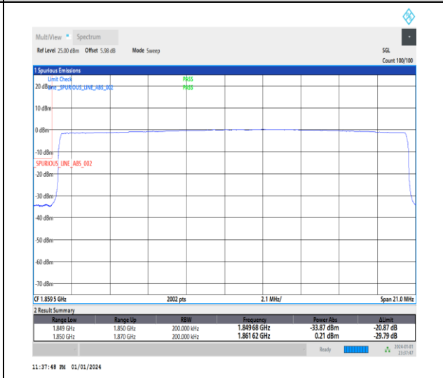
1-N2-15-20-L-6-CP-QPSK-Outer_Full-106@0-Ant3-1-seegraph-PASS-see graph
