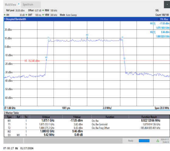
1-N2-15-10-M-5-DFT-256QAM-Outer_Full-50@0-Ant 3-8.922-9.420≤10-PASS
