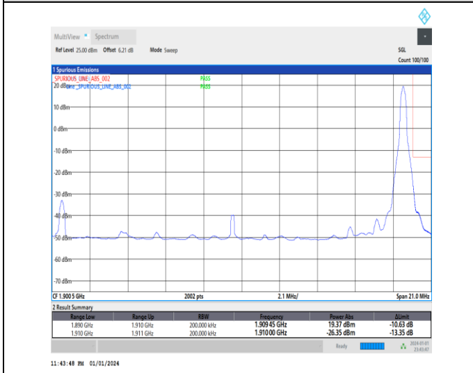
1-N2-15-20-H-5-CP-QPSK-Edge_1RB_Right-1@105-Ant3-1-seegraph-PASS-see graph
