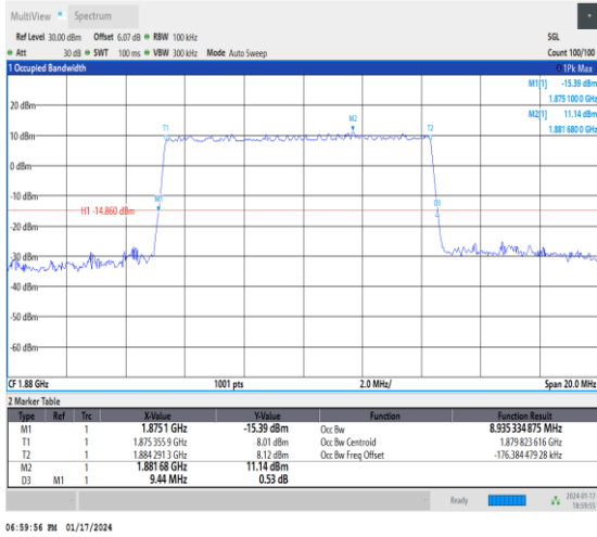
1-N2-15-10-M-4-DFT-64QAM-Outer_Full-50@0-Ant3 -8.935-9.440≤10-PASS
