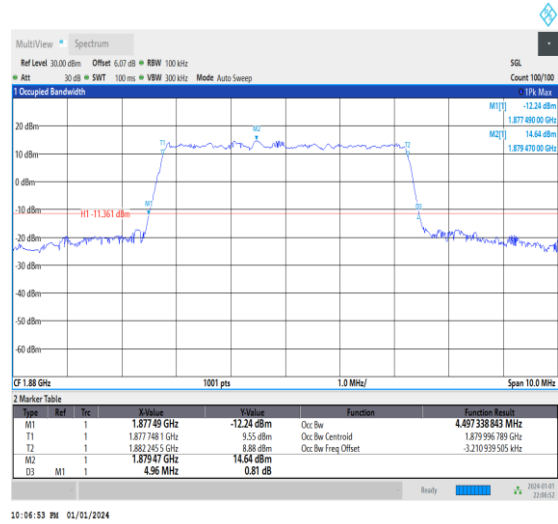
1-N2-15-5-M-6-CP-QPSK-Outer_Full-25@0-Ant3-4. 497-4.960-≤5-PASS
