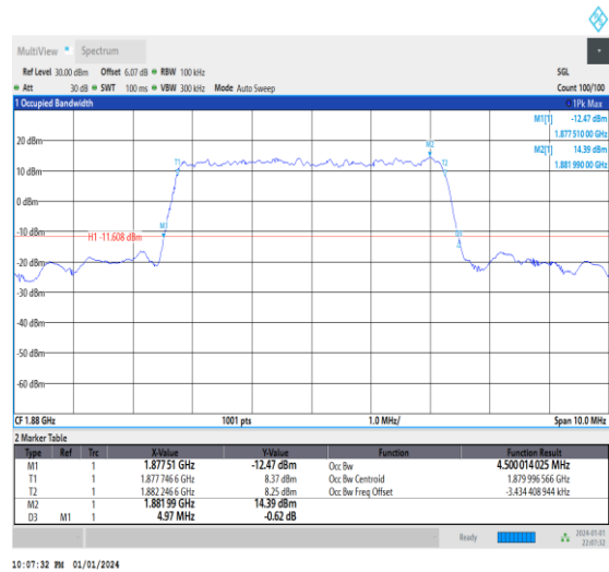
1-N2-15-5-M-8-CP-64QAM-Outer_Full-25@0-Ant3-4. .5-4.970-≤5-PASS
