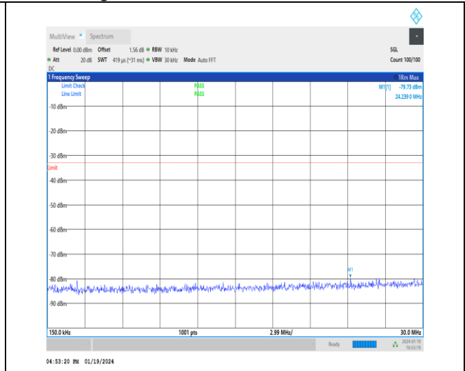
1-N2-15-20-H-1-DFT-PI2BPSK-Inner_1RB_Left-1@ -0.15-30-Ant3-24.24--79.73--33-PASS
