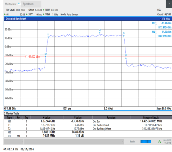
1-N2-15-15-M-4-DFT-64QAM-Outer_Full-75@0-Ant3 -13.495-14.340≤15-PASS
