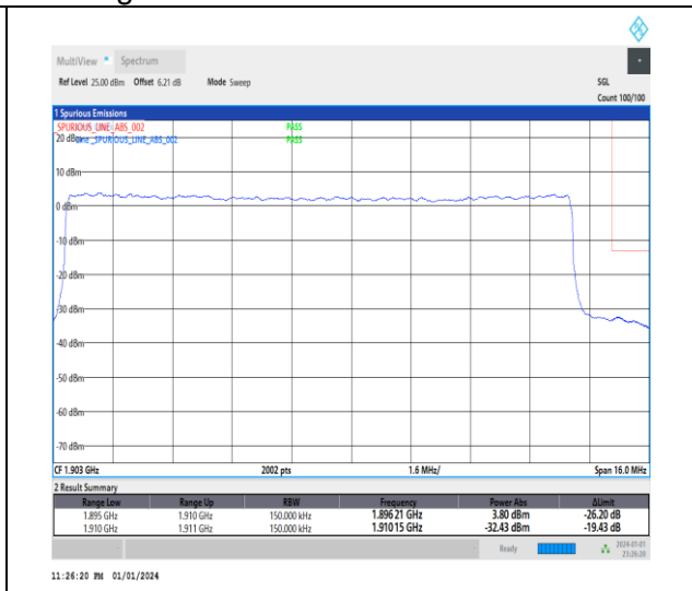
1-N2-15-15-H-3-DFT-PI2BPSK-Outer_Full-75@0-Ant3-1-seegraph-PASS-see graph
