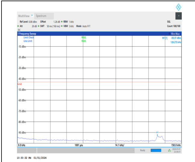
1-N2-15-20-H-1-DFT-PI2BPSK-Inner_1RB_Left-1@ 1-0.009-0.15-Ant3-0.13--93.37--43-PASS
