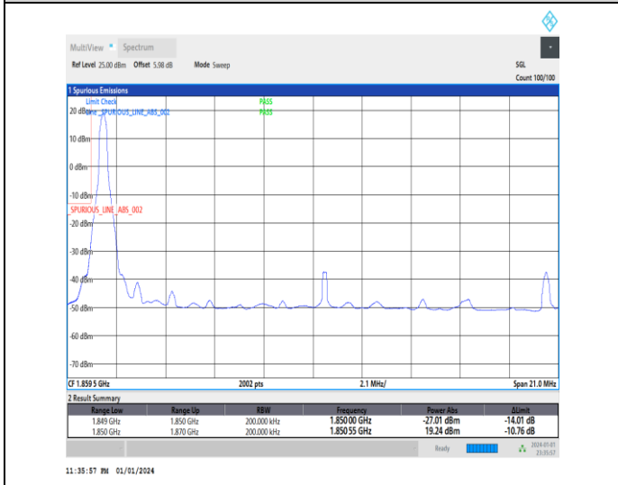
1-N2-15-20-L-4-CP-QPSK-Edge_1RB_Left-1@0-Ant3-1-seegraph-PASS-see graph
