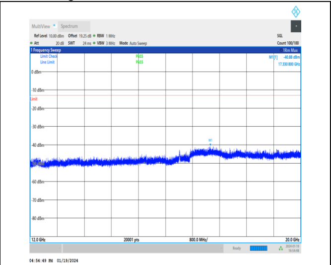
1-N2-15-20-H-1-DFT-PI2BPSK-Inner_1RB_Left-1@ -12000-20000-Ant3-17300.00--40.88--13-PASS
