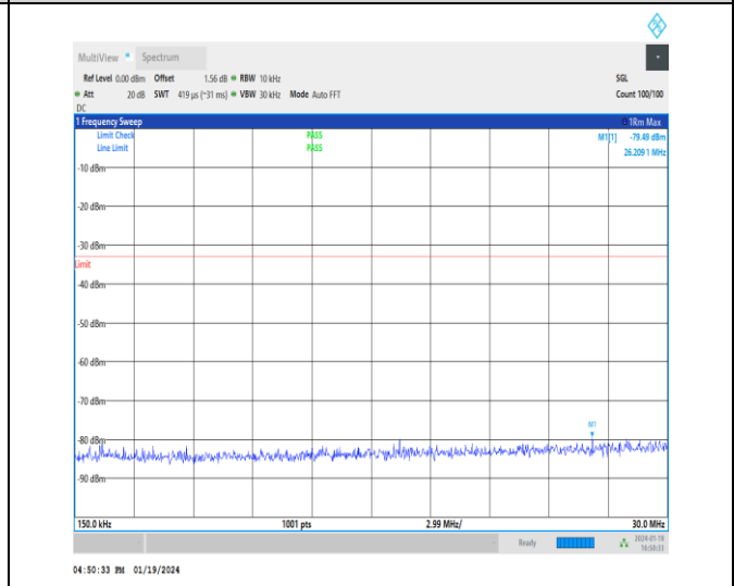
1-N2-15-20-M-1-DFT-PI2BPSK-Inner_1RB_Left-1@1 -0.15-30-Ant3-26.21--79.49--33-PASS
