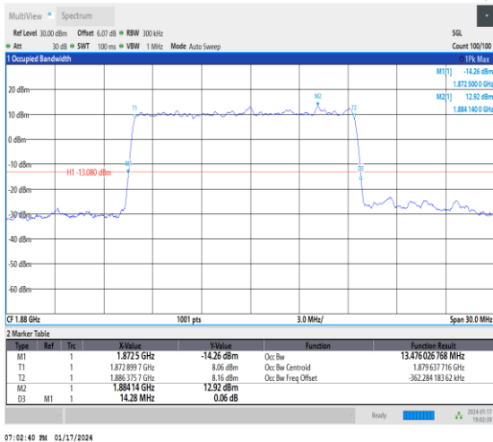
1-N2-15-15-M-5-DFT-256QAM-Outer_Full-75@0-Ant 3-13.476-14.280≤15-PASS
