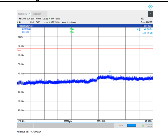
1-N2-15-20-L-1-DFT-PI2BPSK-Inner_1RB_Left-1@1- 12000-20000-Ant3-17448.4--41.09--13-PASS
