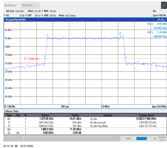
1-N2-15-10-M-7-CP-16QAM-Outer_Full-52@0-Ant3- 9.298-9.880≤10-PASS
