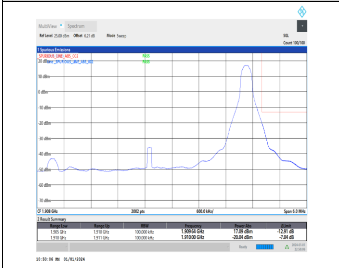
1-N2-15-5-H-5-CP-QPSK-Edge_1RB_Right-1@24-Ant3-1-seegraph-PASS-see graph
