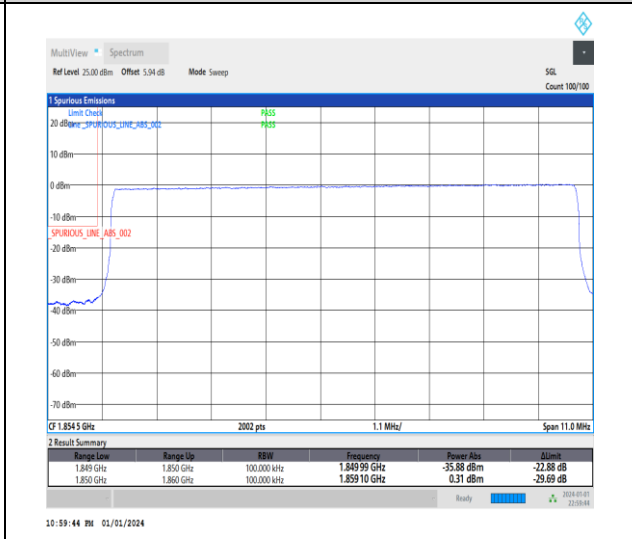
1-N2-15-10-L-6-CP-QPSK-Outer_Full-52@0-Ant3-1-seegraph-PASS-see graph
