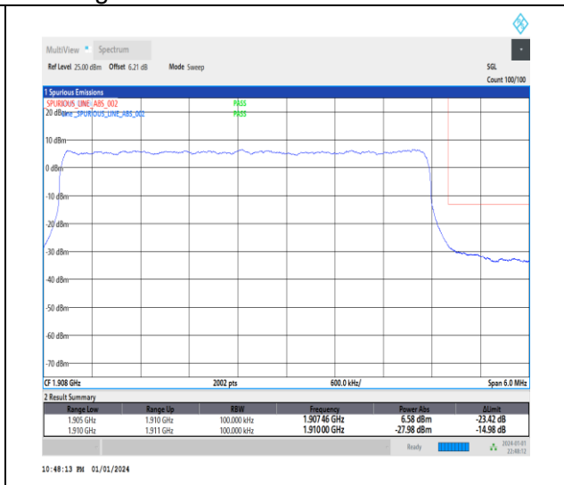
1-N2-15-5-H-3-DFT-PI2BPSK-Outer_Full-25@0-Ant3-1-seegraph-PASS-see graph
