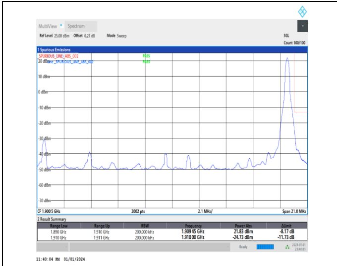
1-N2-15-20-H-2-DFT-PI2BPSK-Edge_1RB_Right-1@105-Ant3-1-seegraph-PASS-see graph
