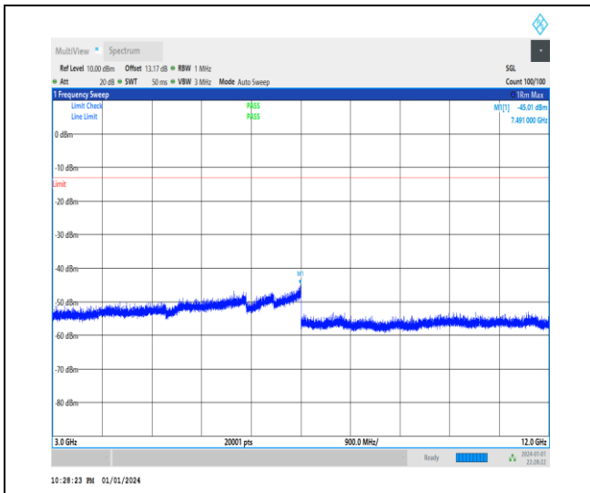
1-N2-15-20-L-1-DFT-PI2BPSK-Inner_1RB_Left-1@ 1-3000-12000-Ant3-7491.00--45.01--13-PASS
