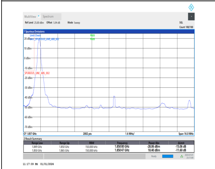
1-N2-15-15-L-4-CP-QPSK-Edge_1RB_Left-1@0-Ant3-1-seegraph-PASS-see graph
