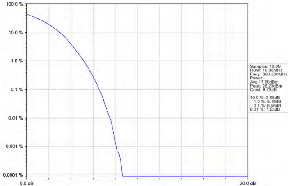
Band71 10MHz 256QAM MCH 680.5MHz RB 50 0 NTN
