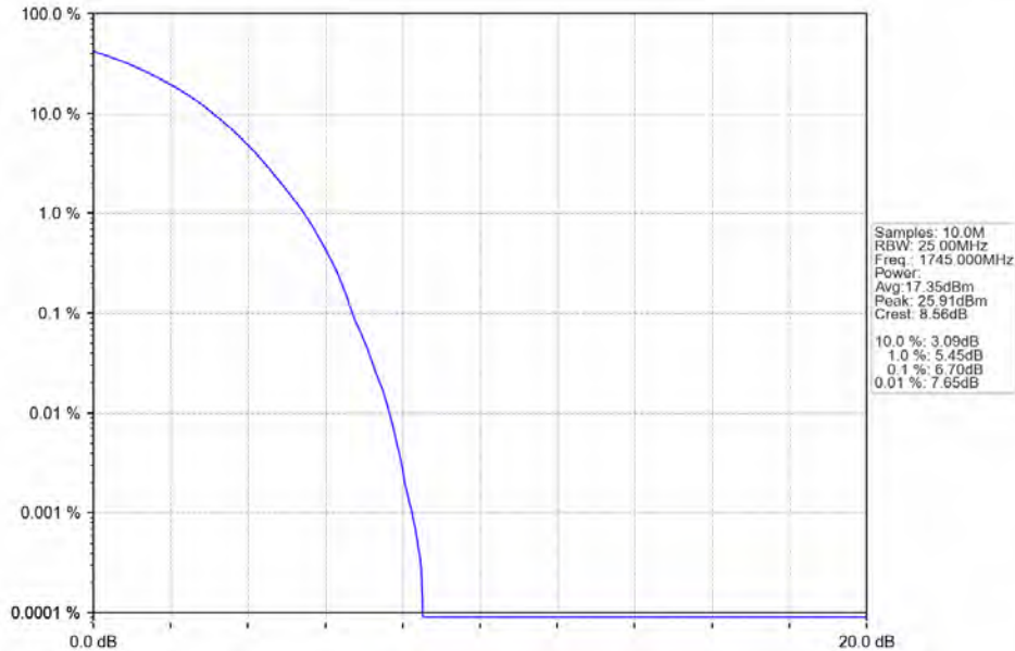
Band66 15MHz 256QAM MCH 1745MHz RB 75 0 NTN
