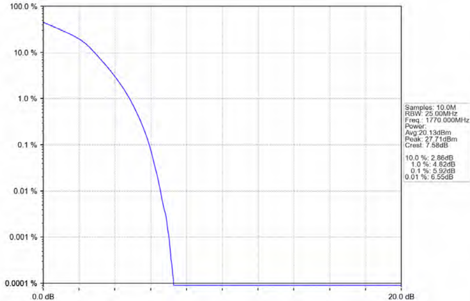
Band66 20MHz 16QAM HCH 1770MHz RB 100 0 NTN
