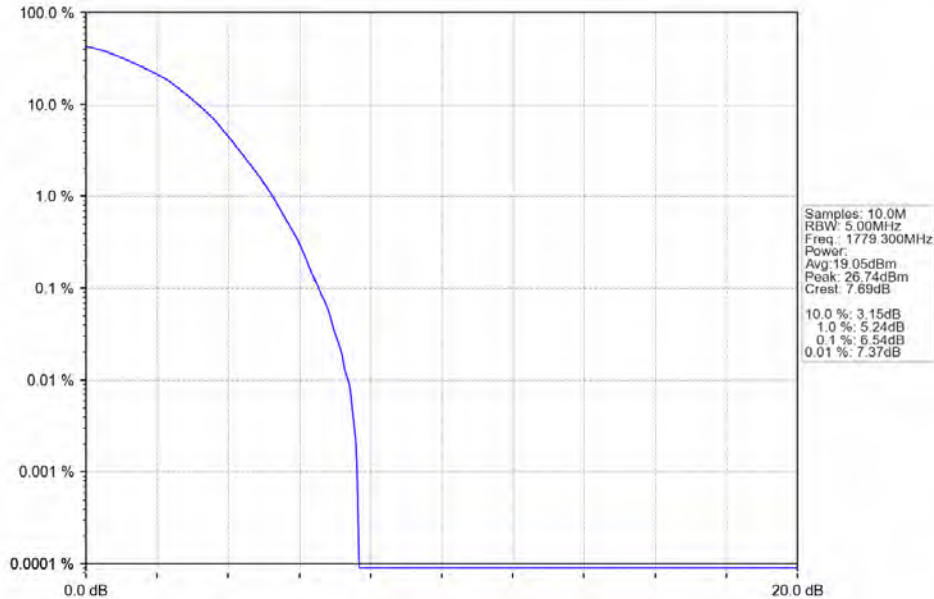
Band66 1.4MHz 64QAM HCH 1779.3MHz RB 6 0 NTN
