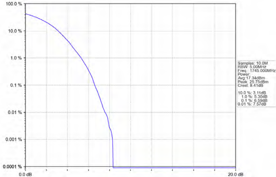
Band66 1.4MHz 256QAM MCH 1745MHz RB 6.0 NTNV
