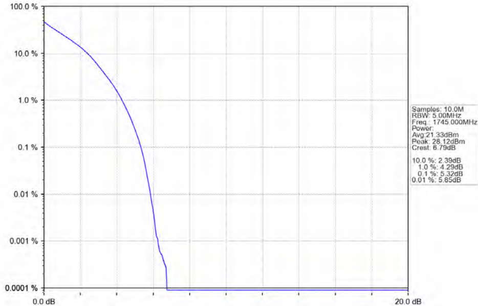
Band66 5MHz QPSK MCH 1745MHz RB 25 0 NTV
