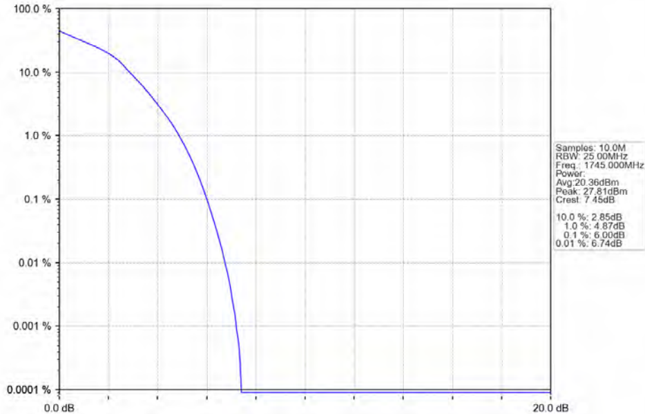
Band66 20MHz 16QAM MCH 1745MHz RB 100 0 NTN
