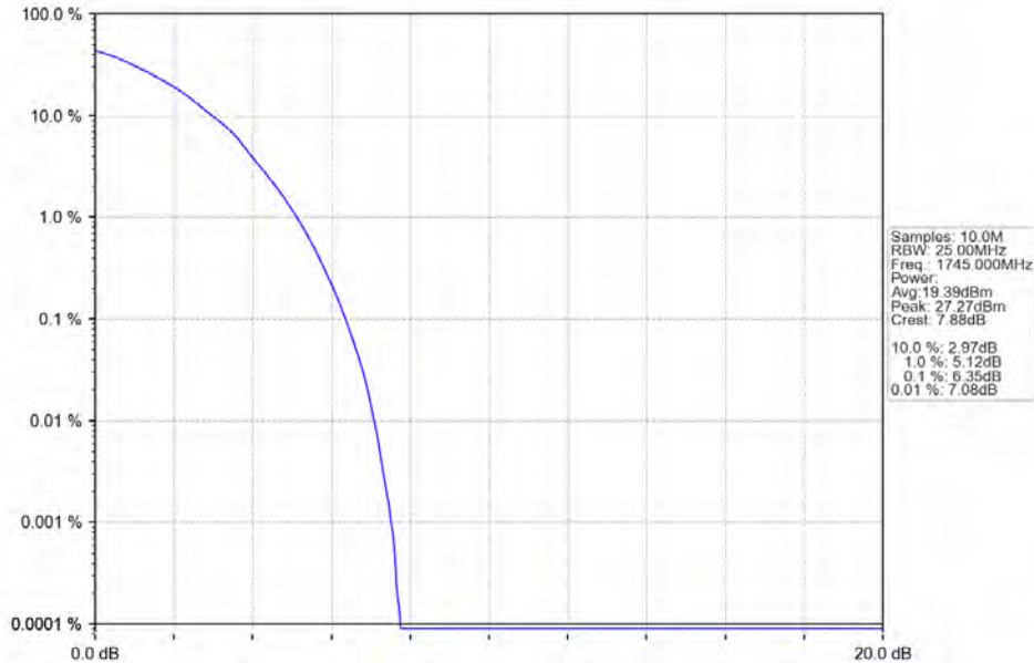
Band66 20MHz 64QAM MCH 1745MHz RB 100 0 NTN
