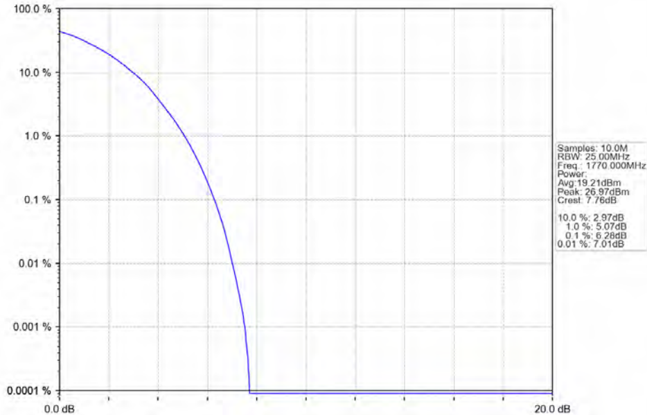
Band66 20MHz 64QAM HCH 1770MHz RB 100 0 NTN
