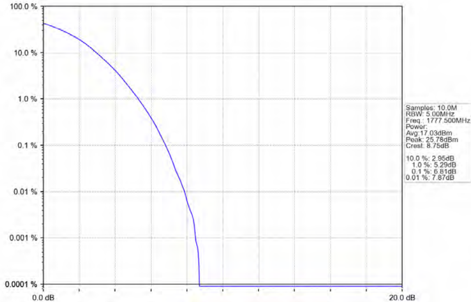
Band66 5MHz 256QAM HCH 1777.5MHz RB 25 0 NTN
