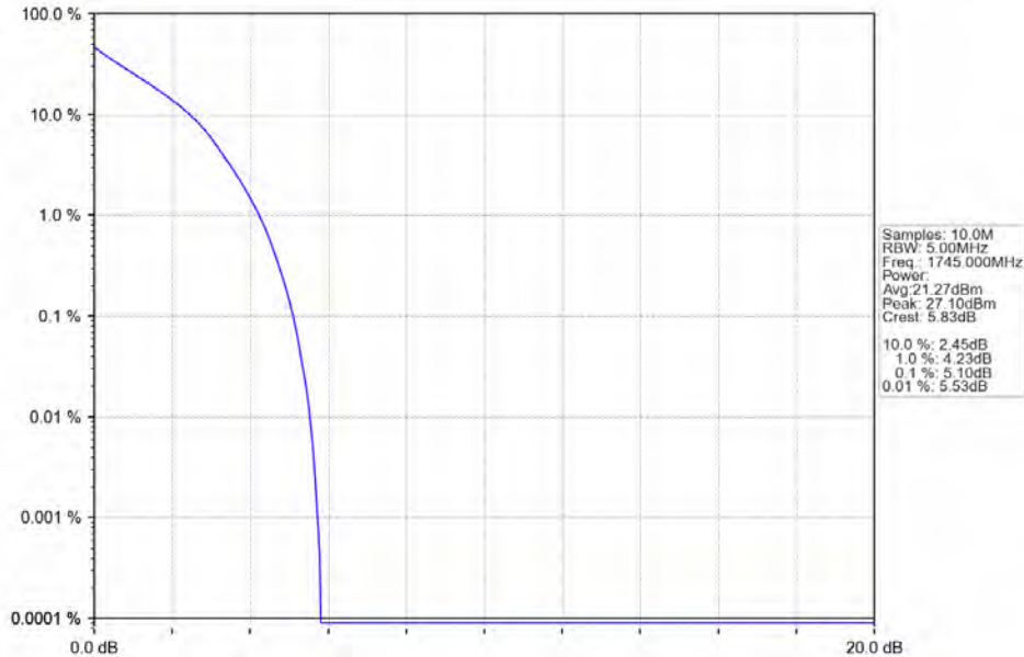
Band66 3MHz QPSK MCH 1745MHz RB 15 0 NTV
