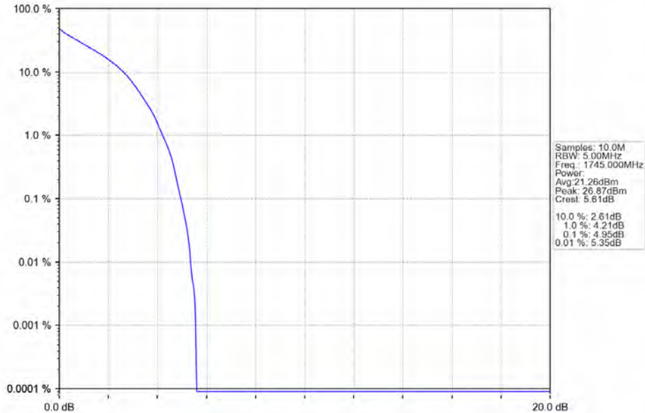
Band66 1.4MHz QPSK MCH 1745MHz RB 6 0 NTV
