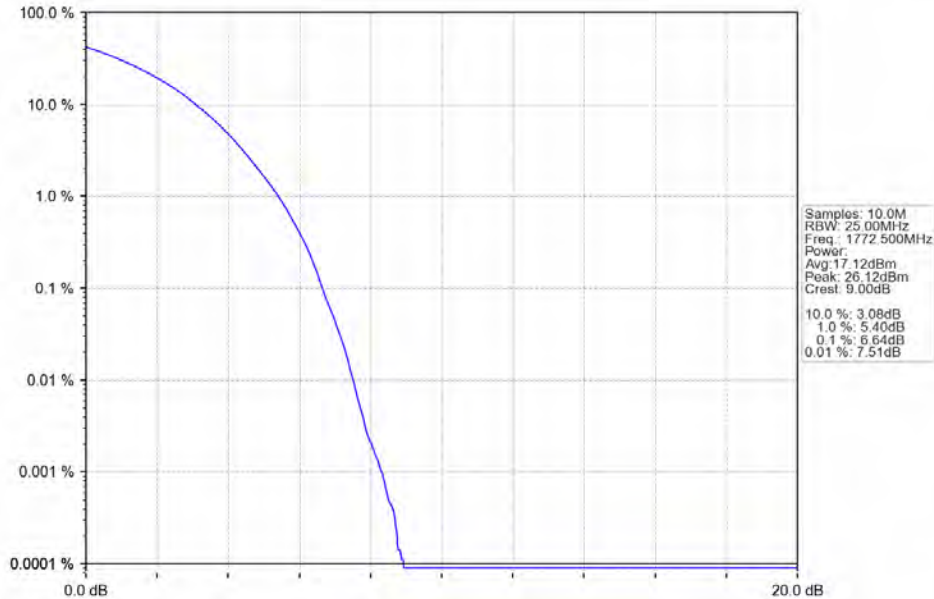
Band66 15MHz 256QAM HCH 1772.5MHz RB 75 0 NTNv
