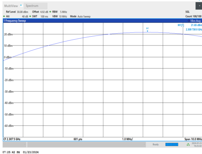
Band30-5MHz-QPSK-27685-1RB#24
