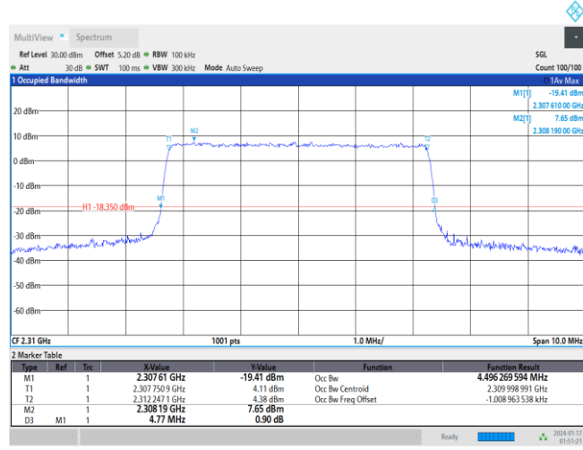
Band30-5MHz-QPSK-27710-25RB#0
