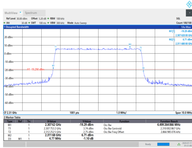
Band30-5MHz-16QAM-27710-25RB#0
