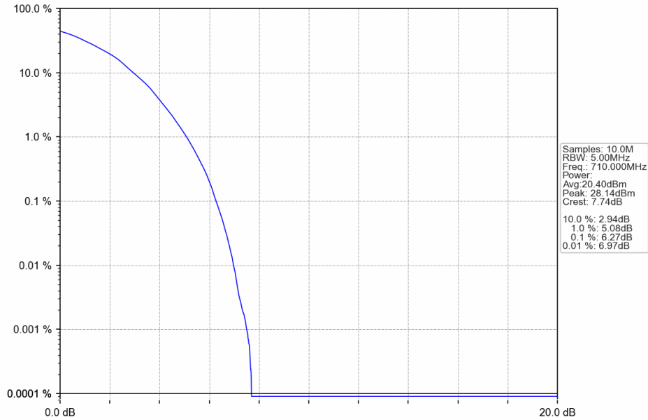
Band17_5MHz_QPSK_MCH_710MHz_RB_25_0_NTNV
