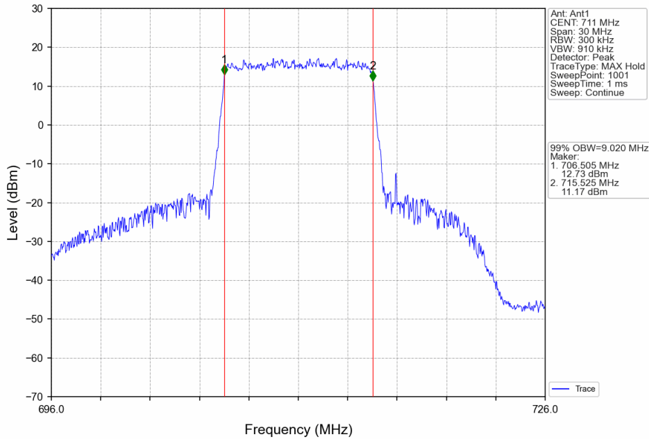
Band17_10MHz_QPSK_HCH_711MHz_RB_50_0_NTNV
