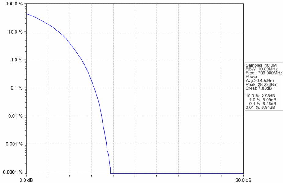
Band17_10MHz_16QAM_LCH_709MHz_RB_50_0_NTNV
