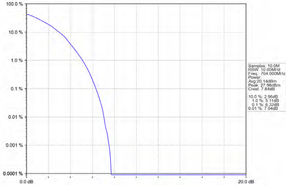
Band12 10MHz 64QAM LCH 704MHz RB 50 0 NTV
