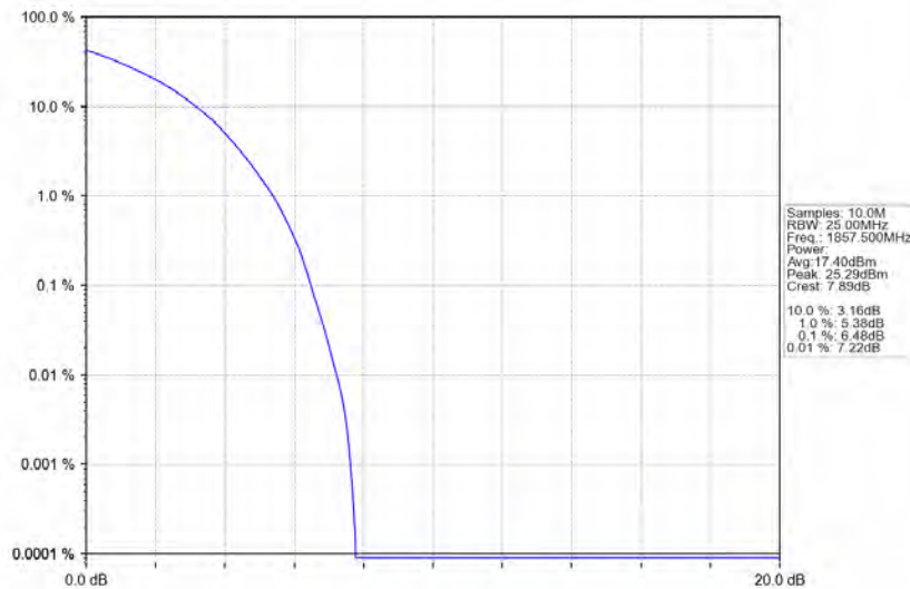
Band2 15MHz 64QAM LCH 1857.5MHz RB 75 0 NTN
