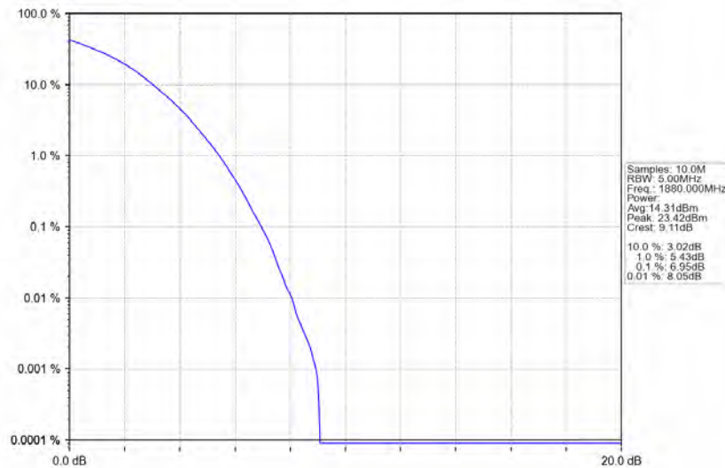
Band2 5MHz 256QAM MCH 1880MHz RB 25 0 NTV
