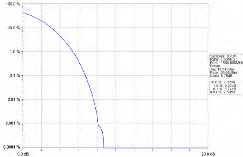
Band2 5MHz 64QAM MCH 1880MHz RB 25 0 NTV
