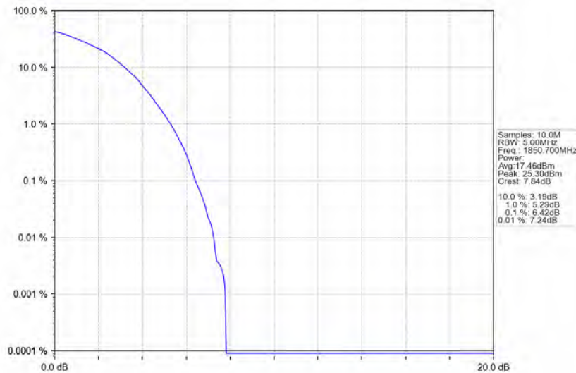
Band2 1.4MHz 64QAM LCH 1850.7MHz RB 6 0 NTN
