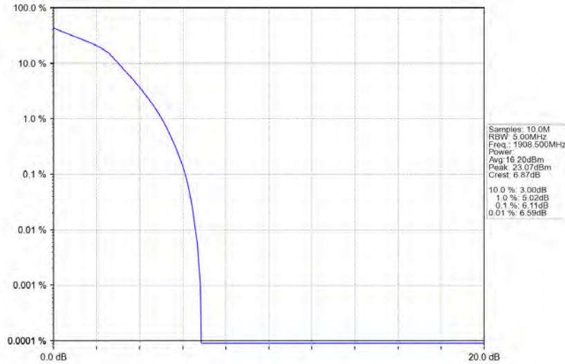
Band2 3MHz 16QAM HCH 1908.5MHz RB 15 0 NTV
