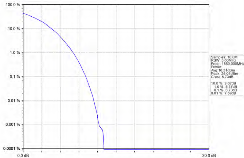
Band2 5MHz 16QAM MCH 1880MHz RB 25 0 NTN
