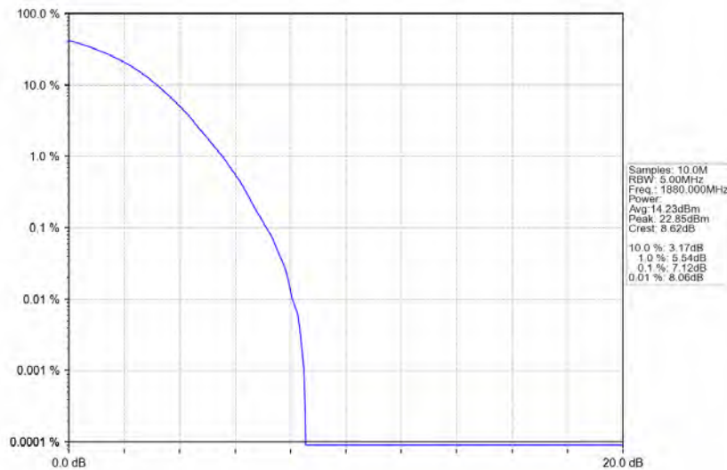
Band2 1.4MHz 256QAM MCH 1880MHz RB 6 0 NTN
