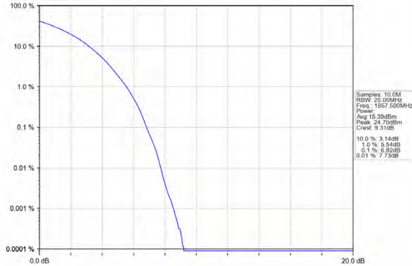
Band2 15MHz 256QAM LCH 1857.5MHz RB 75 0 NTN
