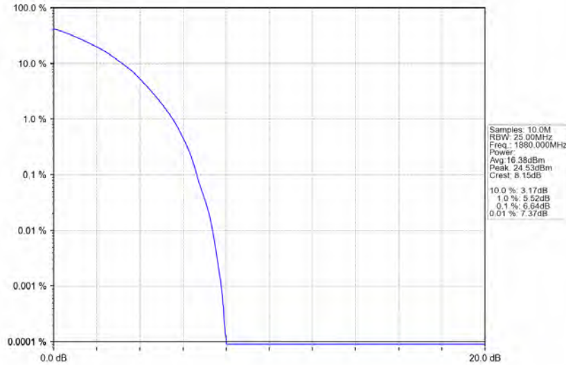
Band2 15MHz 64QAM MCH 1880MHz RB 75 0 NTN
