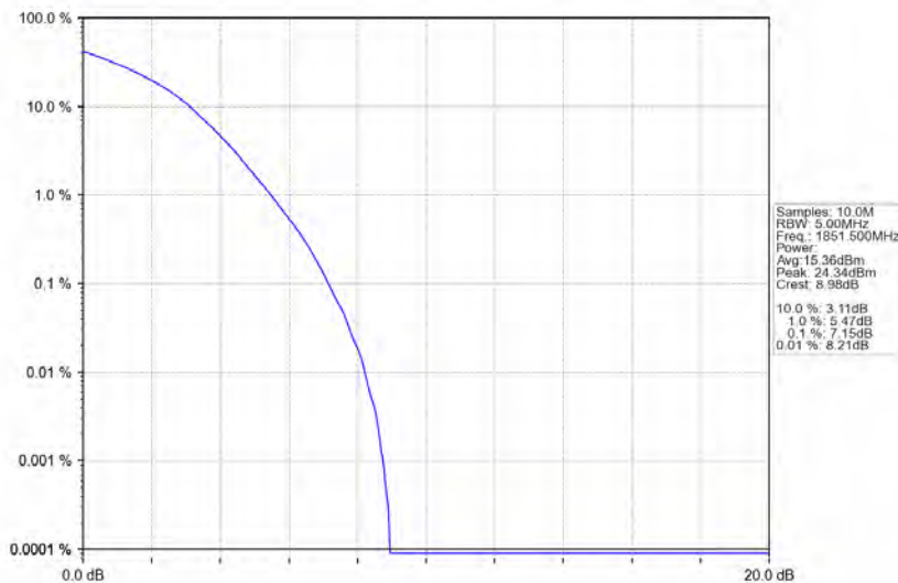
Band2 3MHz 256QAM LCH 1851.5MHz RB 15 0 NTV
