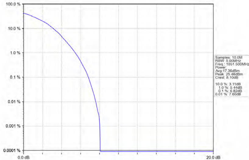
Band2 3MHz 64QAM LCH 1851.5MHz RB 15 0 NTV
