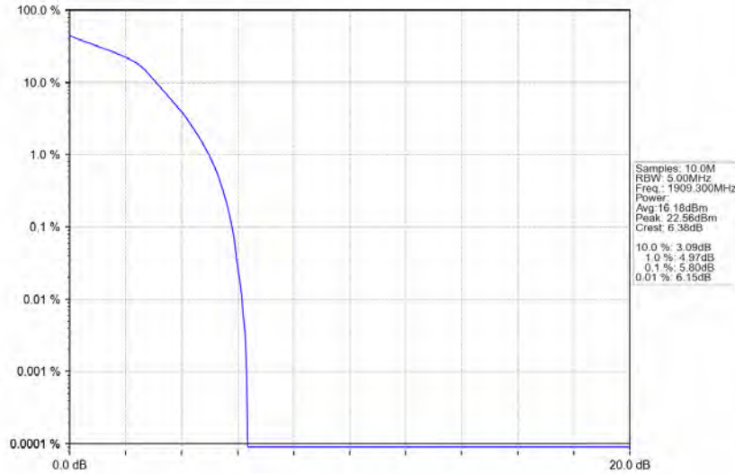
Band2 1.4MHz 16QAM HCH 1909.3MHz RB 6 0 NTN
