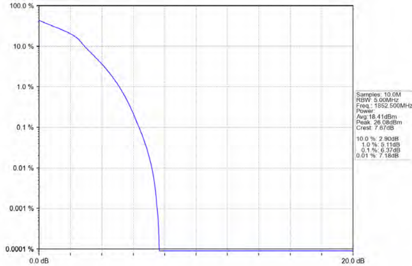
Band2 5MHz 16QAM LCH 1852.5MHz RB 25 0 NTN
