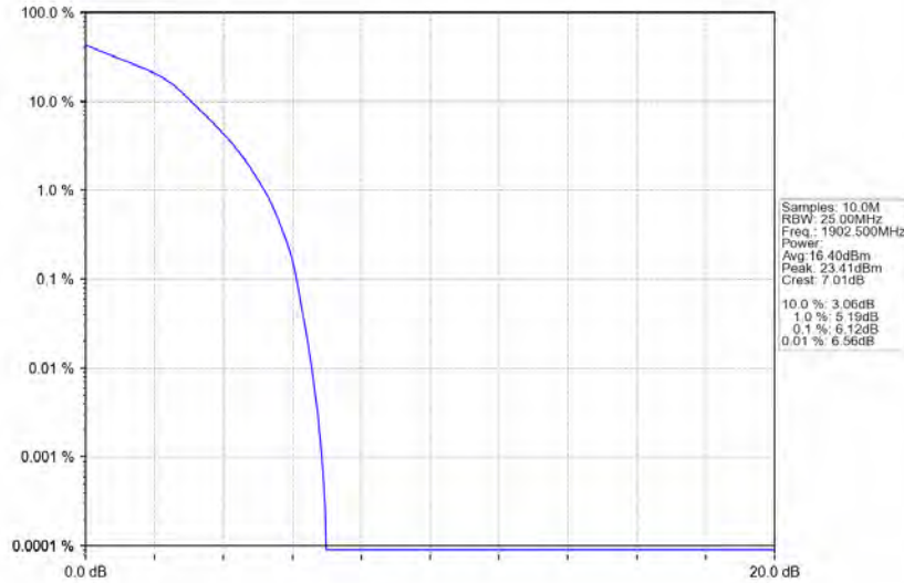
Band2 15MHz 16QAM HCH 1902.5MHz RB 75 0 NTN
