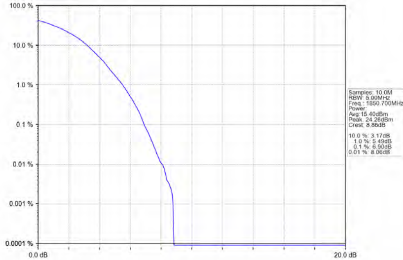
Band2 1.4MHz 256QAM LCH 1850.7MHz RB 6 0 NTN
