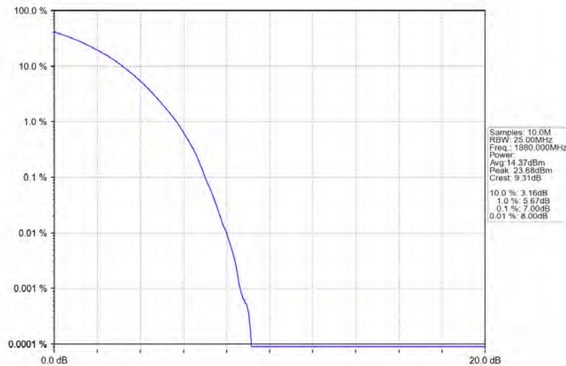
Band2 15MHz 256QAM MCH 1880MHz RB 75 0 NTN
