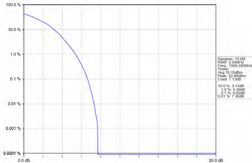
Band2 3MHz 64QAM HCH 1908.5MHz RB 15 0 NTV
