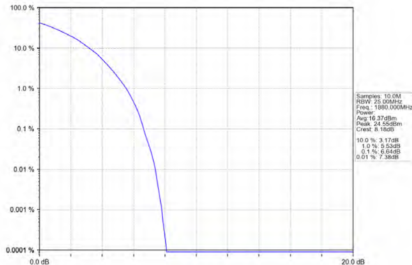
Band2 15MHz 16QAM MCH 1880MHz RB 75 0 NTV
