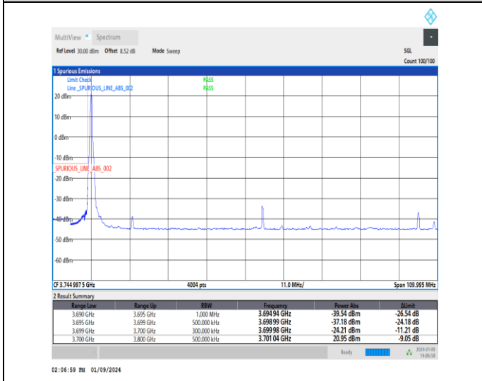
1-N77-3700-3980-30-100-L-4-CP-QPSK-Edge_1RB_Left-1@0-Ant4-1--PASS-see graph
