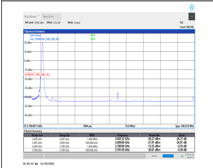
1-N77-3700-3980-30-90-L-4-CP-QPSK-Edge_1RB_Lef t-1@0-Ant4-1--PASS-see graph
