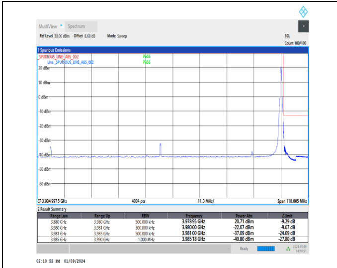
1-N77-3700-3980-30-100-H-2-DFT-PI2BPSK-Edge_1R_B_Right-1@272-Ant4-1--PASS-see graph
