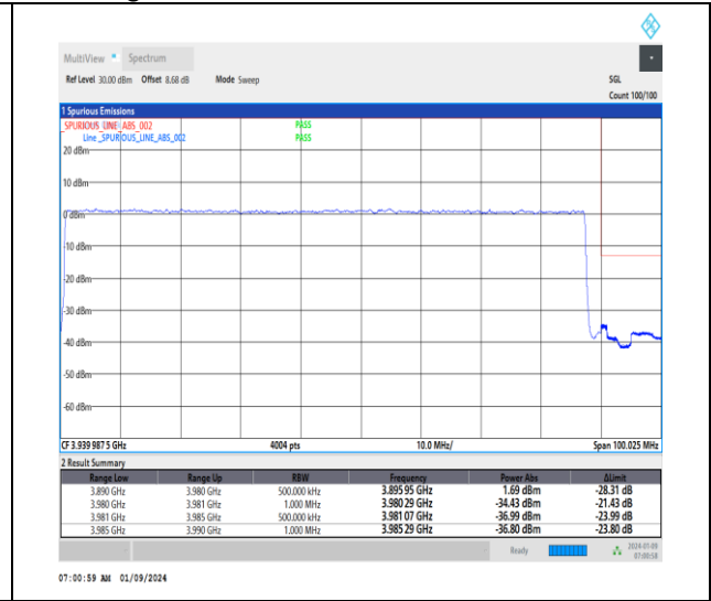
1-N77-3700-3980-30-90-H-3-DFT-PI2BPSK-Outer_Full-240@0-Ant4-1--PASS-see graph
