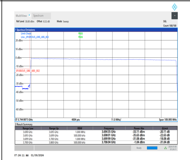
1-N77-3700-3980-30-100-L-6-CP-QPSK-Outer_Full-273@0-Ant4-1--PASS-see graph
