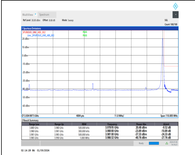
1-N77-3700-3980-30-100-H-5-CP-QPSK-Edge_1RB_Right-1@272-Ant4-1--PASS-see graph
