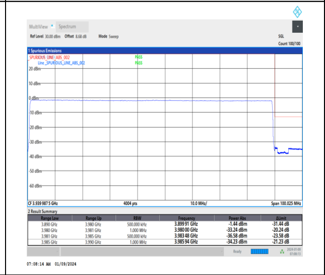
1-N77-3700-3980-30-90-H-6-CP-QPSK-Outer_Full-245@0-Ant4-1--PASS-see graph
