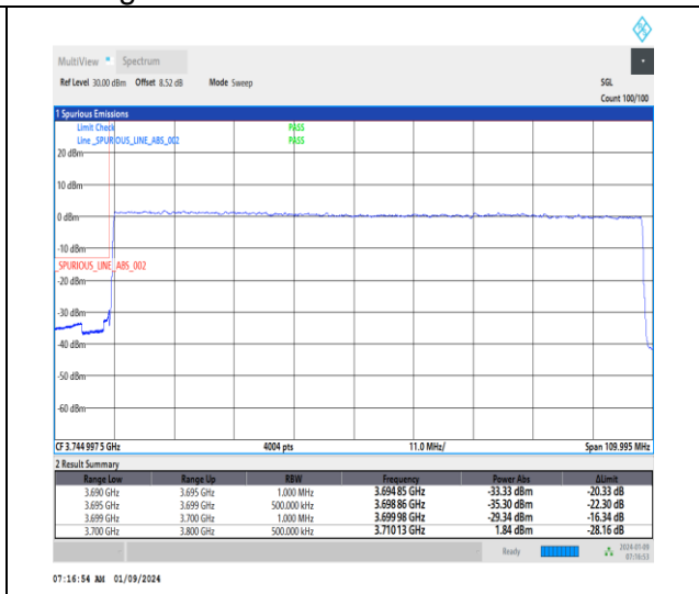
1-N77-3700-3980-30-100-L-3-DFT-PI2BPSK-Outer_Full-270@0-Ant4-1--PASS-see graph
