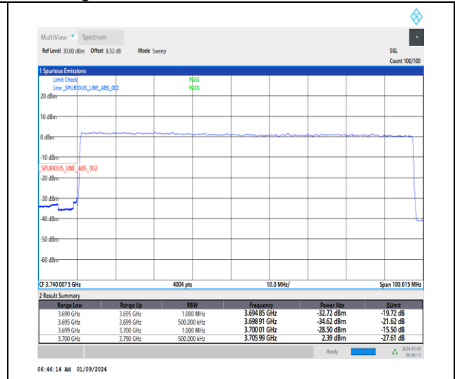
1-N77-3700-3980-30-90-L-3-DFT-PI2BPSK-Outer _Full-240@0-Ant4-1--PASS-see graph
