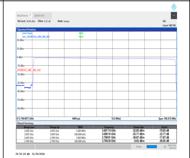
1-N77-3700-3980-30-90-L-6-CP-QPSK-Outer_Full -245@0-Ant4-1--PASS-see graph
