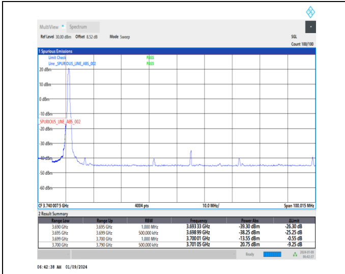
1-N77-3700-3980-30-90-L-1-DFT-PI2BPSK-Edge_1RB _Left-1@0-Ant4-1--PASS-see graph
