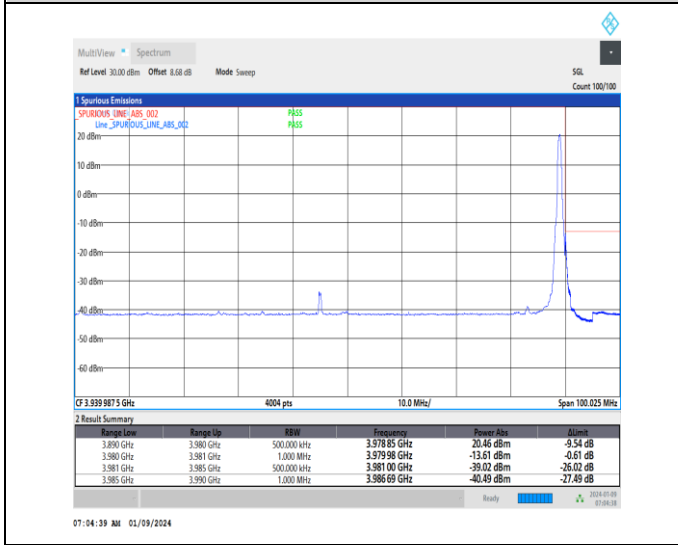
1-N77-3700-3980-30-90-H-5-CP-QPSK-Edge_1RB_Right-1@244-Ant4-1--PASS-see graph
