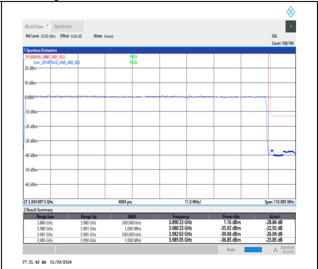
1-N77-3700-3980-30-100-H-3-DFT-PI2BPSK-Outer_Full-270@0-Ant4-1--PASS-see graph
