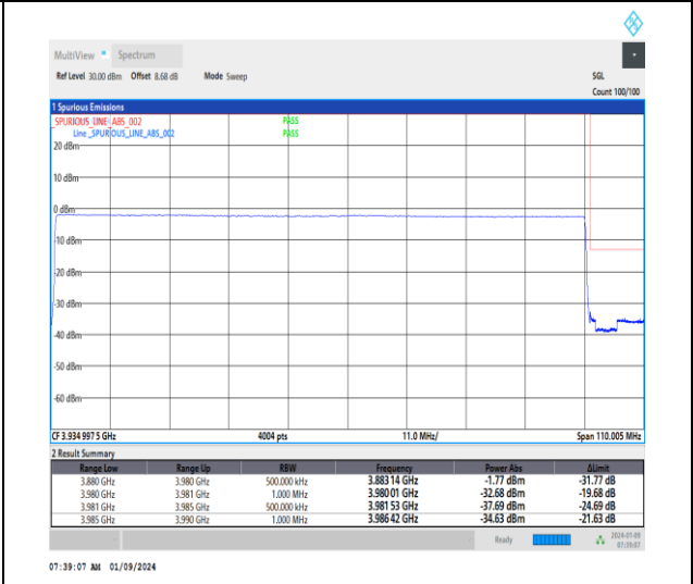
1-N77-3700-3980-30-100-H-6-CP-QPSK-Outer_Full-273@0-Ant4-1--PASS-see graph
