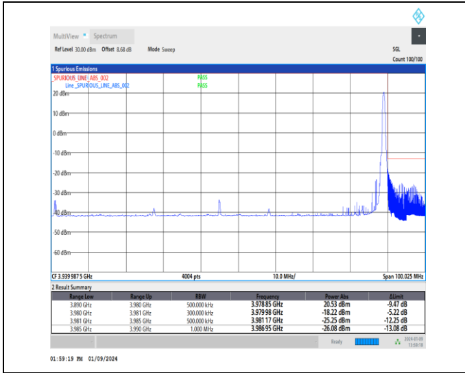
1-N77-3700-3980-30-90-H-2-DFT-PI2BPSK-Edge_1R_B_Right-1@244-Ant4-1--PASS-see graph
