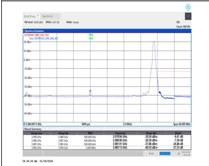
1-N77-3700-3980-30-40-H-5-CP-QPSK-Edge_1RB_Right-1@105-Ant4-1--PASS-see graph
