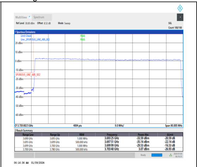
1-N77-3700-3980-30-80-L-3-DFT-PI2BPSK-Outer_Full-216@0-Ant4-1--PASS-see graph
