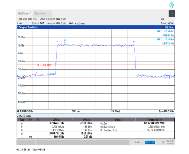
1-N77-3700-3980-30-90-M-8-CP-64QAM-Outer_Full-245@0-Ant4-87.359-90.900-≤90-PASS
