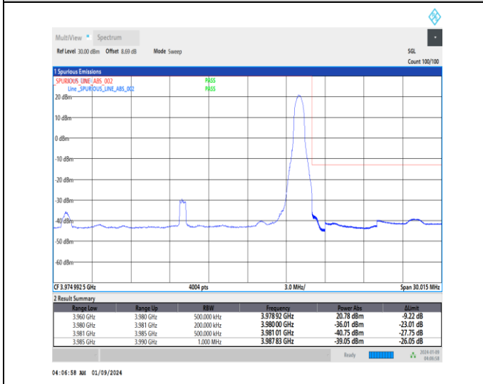
1-N77-3700-3980-30-20-H-5-CP-QPSK-Edge_1RB_Right-1@50-Ant4-1--PASS-see graph
