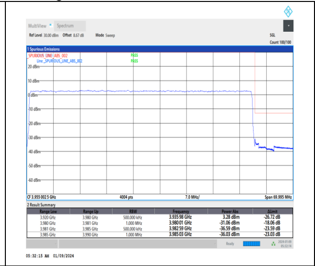
1-N77-3700-3980-30-60-H-3-DFT-PI2BPSK-Outer_Full-162@0-Ant4-1--PASS-see graph
