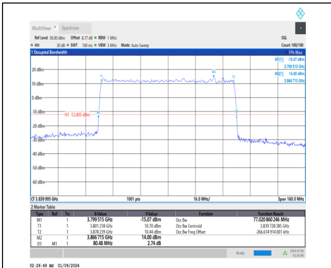
1-N77-3700-3980-30-80-M-3-DFT-16QAM-Outer_Fu II-216@0-Ant4-77.021-80.480-≤80-PASS
