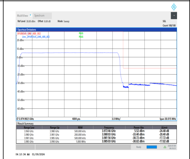
1-N77-3700-3980-30-20-H-6-CP-QPSK-Outer_Full-51@0-Ant4-1--PASS-see graph
