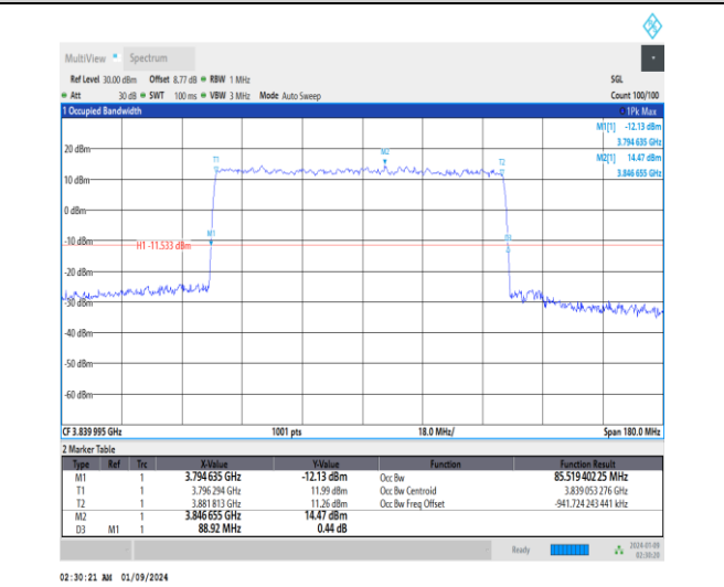
1-N77-3700-3980-30-90-M-1-DFT-QPSK-Outer_Full- 240@0-Ant4-85.519-88.920-≤90-PASS
