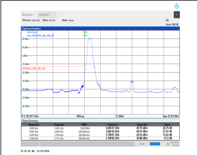
1-N77-3700-3980-30-15-L-4-CP-QPSK-Edge_1RB_Lef t-1@0-Ant4-1--PASS-see graph
