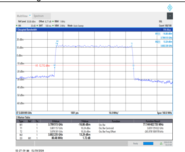
1-N77-3700-3980-30-80-M-4-DFT-64QAM-Outer_Ful I-216@0-Ant4-77.144-80.480-≤80-PASS
