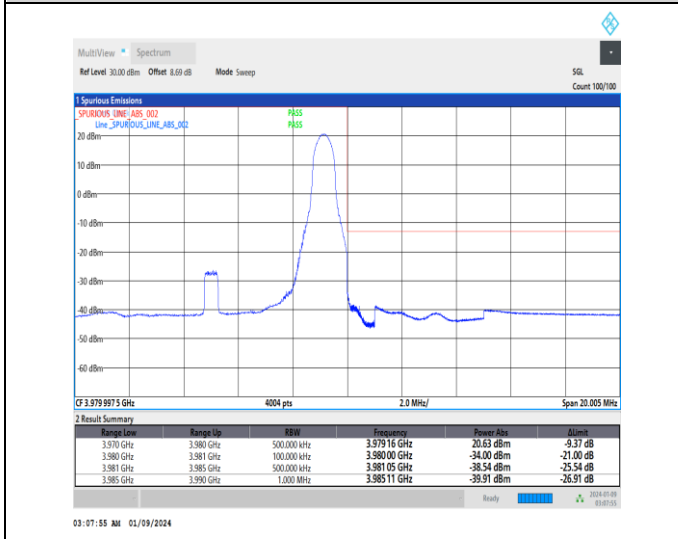
1-N77-3700-3980-30-10-H-5-CP-QPSK-Edge_1RB_Right-1@23-Ant4-1--PASS-see graph
