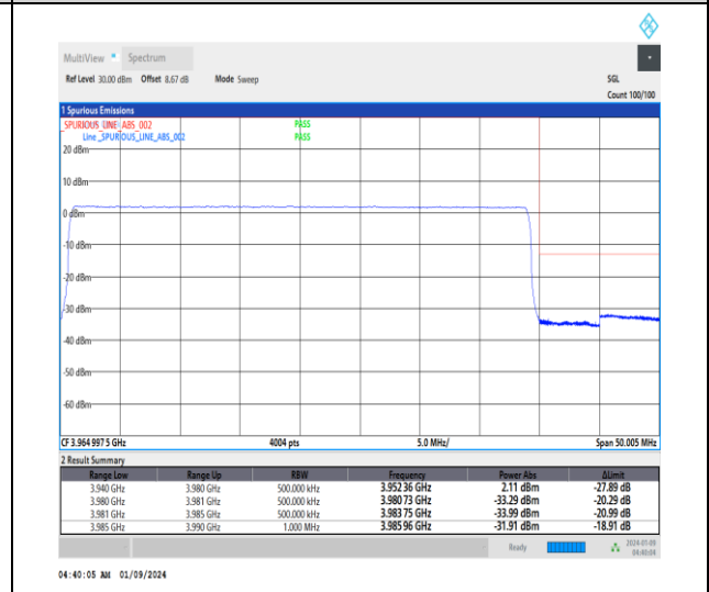
1-N77-3700-3980-30-40-H-6-CP-QPSK-Outer_Full-106@0-Ant4-1--PASS-see graph
