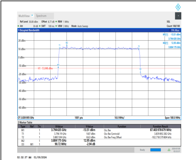
1-N77-3700-3980-30-90-M-6-CP-QPSK-Outer_Full-245@0-Ant4-87.404-90.720-≤90-PASS
