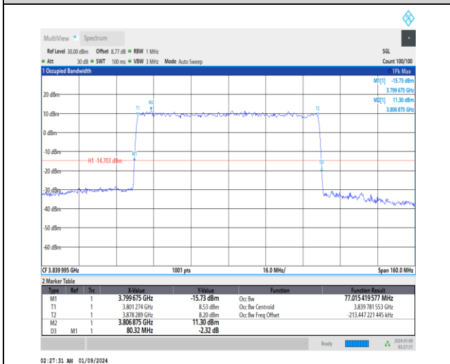
1-N77-3700-3980-30-80-M-5-DFT-256QAM-Outer_Full-216@0-Ant4-77.015-80.320-≤80-PASS
