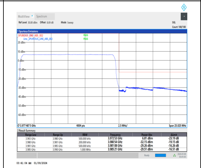
1-N77-3700-3980-30-15-H-6-CP-QPSK-Outer_Full-38@0-Ant4-1--PASS-see graph
