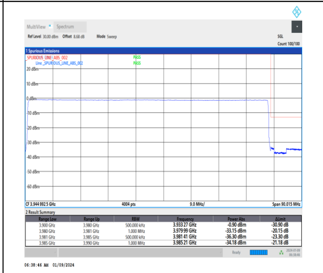
1-N77-3700-3980-30-80-H-6-CP-QPSK-Outer_Full-217@0-Ant4-1--PASS-see graph
