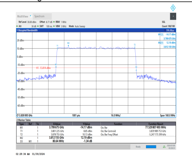
1-N77-3700-3980-30-80-M-8-CP-64QAM-Outer_Full -217@0-Ant4-77.53-80.640-≤80-PASS
