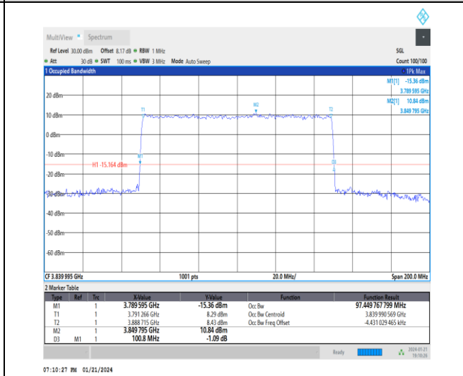
1-N77-3700-3980-PC2-30-100-M-8-CP-64QAM-Outer_Full-273@0-Ant4-97.45-100.800-≤100-PASS
