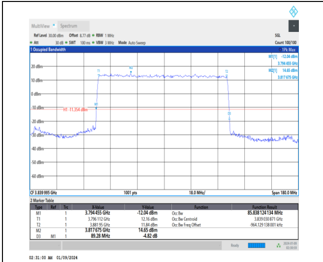
1-N77-3700-3980-30-90-M-2-DFT-Pl2BPSK-Outer_Full-240@0-Ant4-85.838-89.280-<=90-PASS
