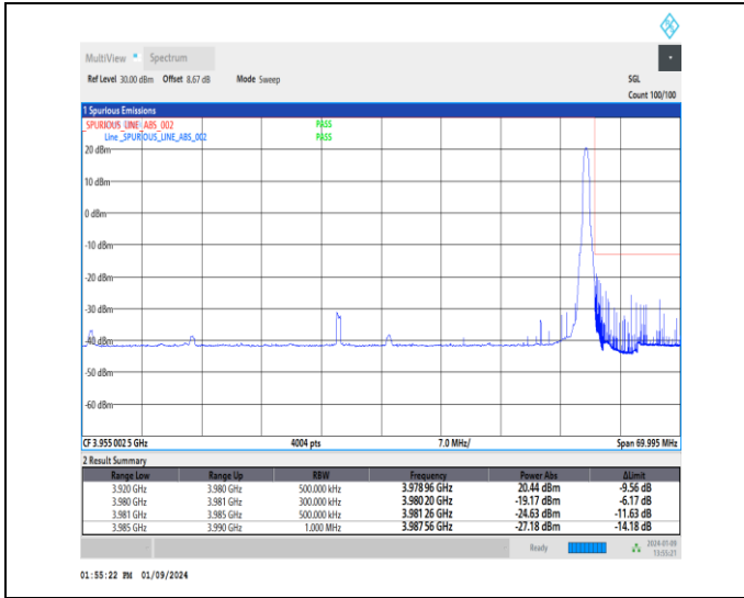
1-N77-3700-3980-30-60-H-2-DFT-PI2BPSK-Edge_1R_B_Right-1@161-Ant4-1--PASS-see graph
