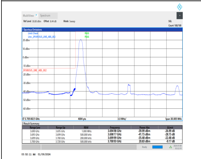
1-N77-3700-3980-30-20-L-4-CP-QPSK-Edge_1RB_Lef t-1@0-Ant4-1--PASS-see graph
