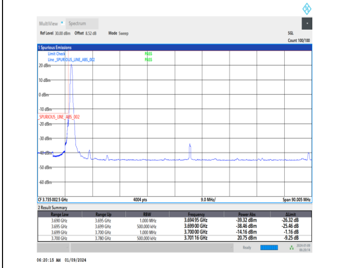
1-N77-3700-3980-30-80-L-4-CP-QPSK-Edge_1RB_Lef t-1@0-Ant4-1--PASS-see graph
