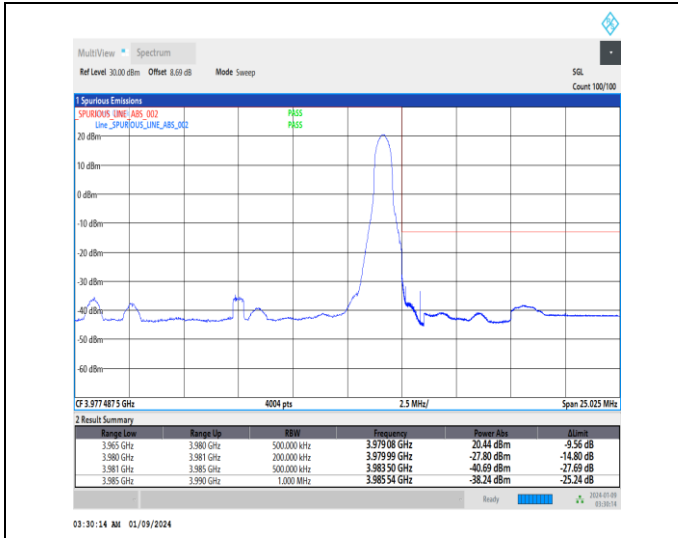
1-N77-3700-3980-30-15-H-2-DFT-PI2BPSK-Edge_1R_B_Right-1@37-Ant4-1--PASS-see graph
