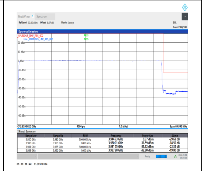
1-N77-3700-3980-30-60-H-6-CP-QPSK-Outer_Full-162@0-Ant4-1--PASS-see graph
