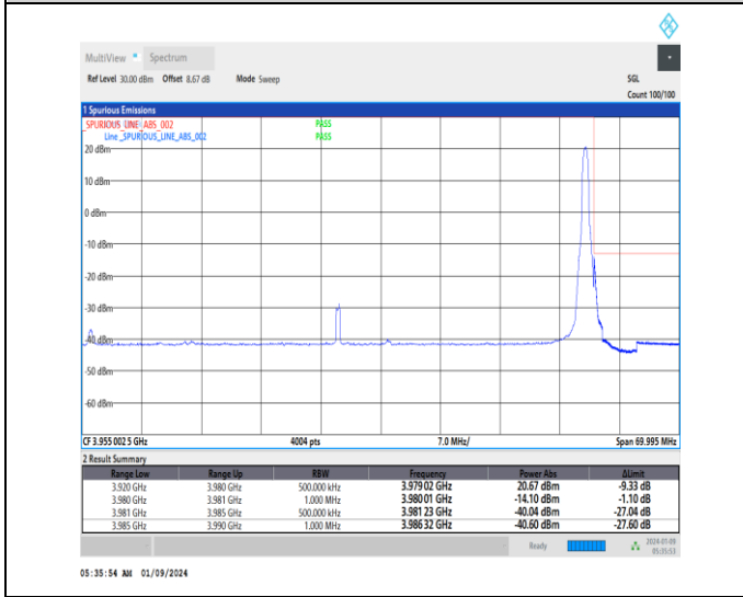
1-N77-3700-3980-30-60-H-5-CP-QPSK-Edge_1RB_Right-1@161-Ant4-1--PASS-see graph
