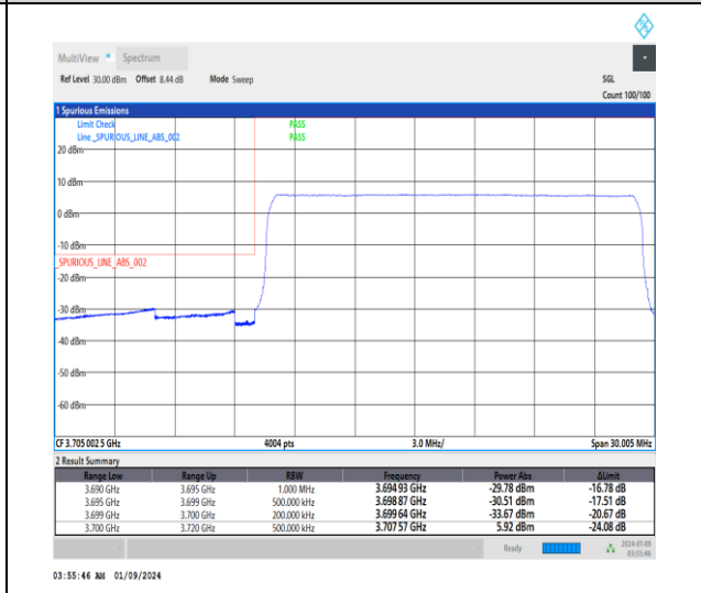
1-N77-3700-3980-30-20-L-6-CP-QPSK-Outer_Full -51@0-Ant4-1--PASS-see graph
