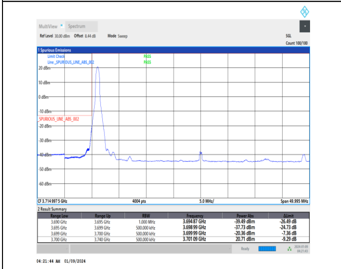
1-N77-3700-3980-30-40-L-4-CP-QPSK-Edge_1RB_Lef t-1@0-Ant4-1--PASS-see graph
