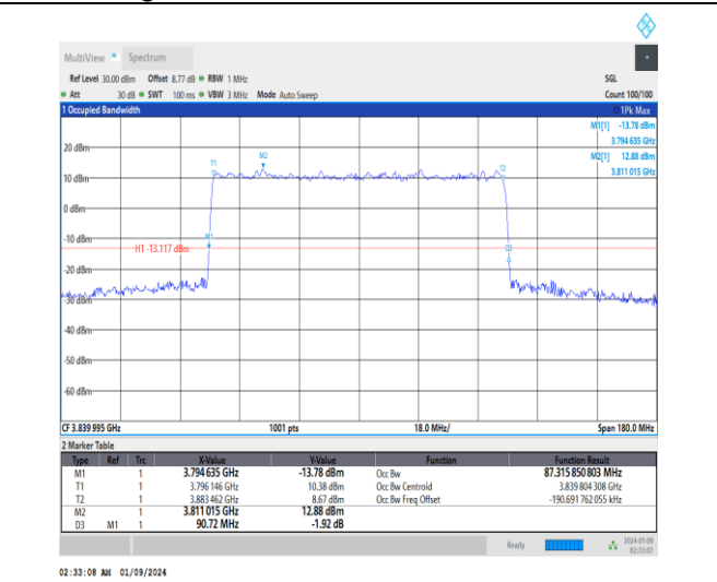
1-N77-3700-3980-30-90-M-7-CP-16QAM-Outer_Full-245@0-Ant4-87.316-90.720-≤90-PASS
