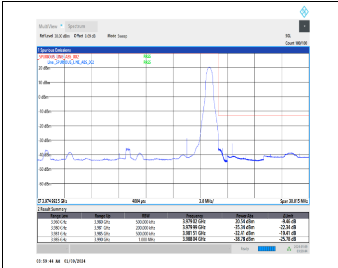
1-N77-3700-3980-30-20-H-2-DFT-PI2BPSK-Edge_1R_B_Right-1@50-Ant4-1--PASS-see graph
