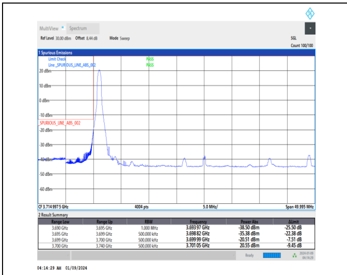
1-N77-3700-3980-30-40-L-1-DFT-PI2BPSK-Edge_1RB _Left-1@0-Ant4-1--PASS-see graph
