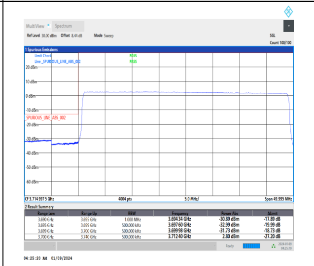
1-N77-3700-3980-30-40-L-6-CP-QPSK-Outer_Full -106@0-Ant4-1--PASS-see graph
