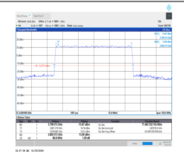
1-N77-3700-3980-30-80-M-6-CP-QPSK-Outer_Full-217@0-Ant4-77.465-80.800-≤80-PASS
