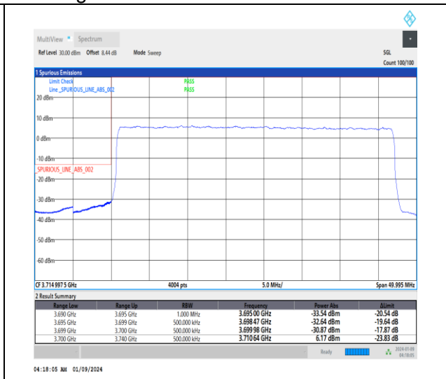
1-N77-3700-3980-30-40-L-3-DFT-PI2BPSK-Outer _Full-100@0-Ant4-1--PASS-see graph
