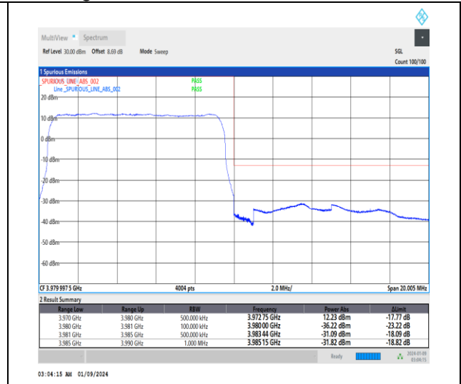
1-N77-3700-3980-30-10-H-3-DFT-PI2BPSK-Outer_Full-24@0-Ant4-1--PASS-see graph
