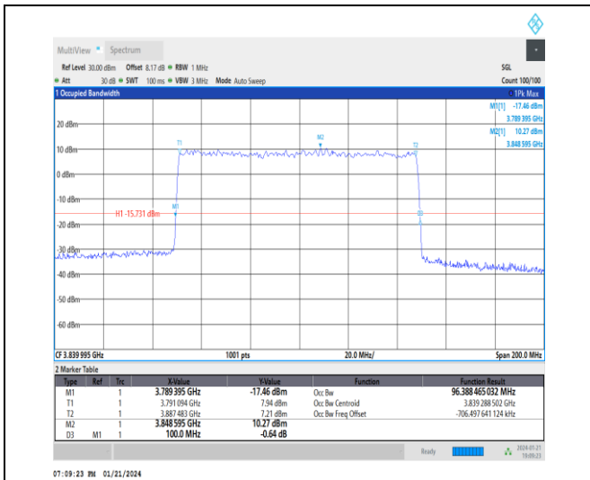
1-N77-3700-3980-PC2-30-100-M-5-DFT-256QAM-Outer_Full-270@0-Ant4-96.388-100.000-≤100-PASS
