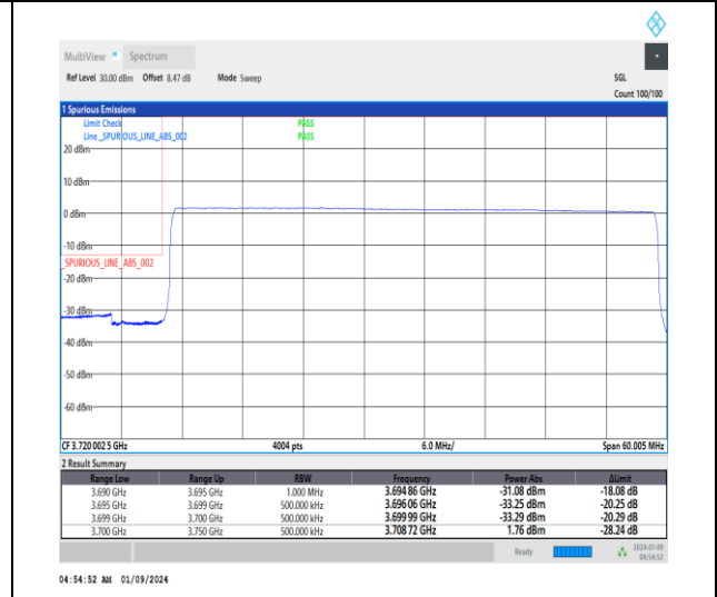
1-N77-3700-3980-30-50-L-6-CP-QPSK-Outer_Full -133@0-Ant4-1--PASS-see graph
