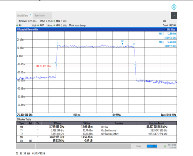
1-N77-3700-3980-30-90-M-3-DFT-16QAM-Outer_Full-I-240@0-Ant4-85.527-88.920-<=90-PASS
