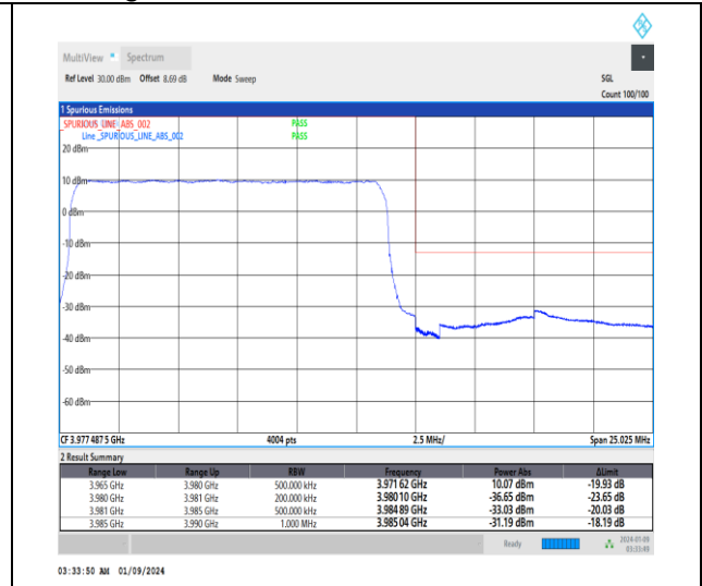
1-N77-3700-3980-30-15-H-3-DFT-PI2BPSK-Outer_Full-36@0-Ant4-1--PASS-see graph
