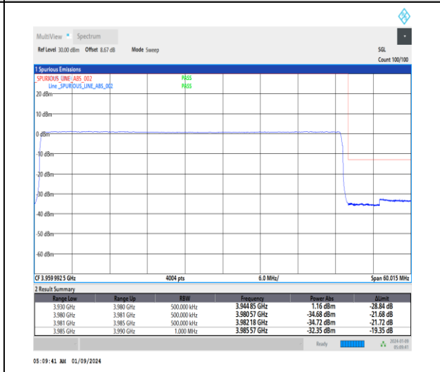
1-N77-3700-3980-30-50-H-6-CP-QPSK-Outer_Full-133@0-Ant4-1--PASS-see graph
