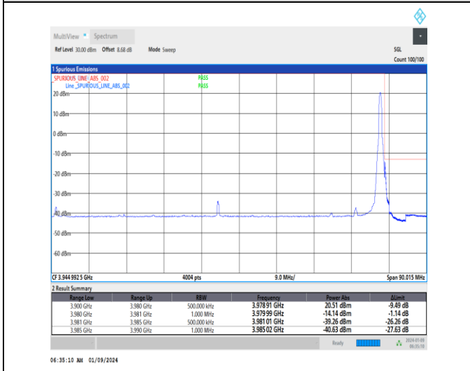
1-N77-3700-3980-30-80-H-5-CP-QPSK-Edge_1RB_Right-1@216-Ant4-1--PASS-see graph
