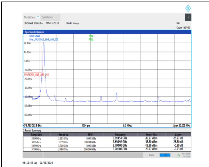
1-N77-3700-3980-30-80-L-1-DFT-PI2BPSK-Edge_1RB_Left-1@0-Ant4-1--PASS-see graph
