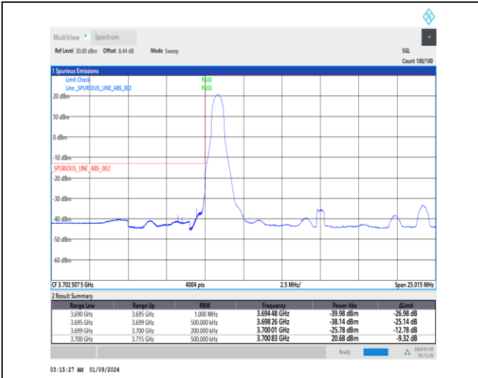
1-N77-3700-3980-30-15-L-1-DFT-PI2BPSK-Edge_1RB _Left-1@0-Ant4-1--PASS-see graph
