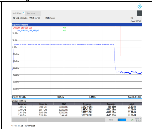
1-N77-3700-3980-30-50-H-3-DFT-PI2BPSK-Outer_Full-128@0-Ant4-1--PASS-see graph
