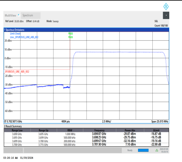
1-N77-3700-3980-30-15-L-6-CP-QPSK-Outer_Full -38@0-Ant4-1--PASS-see graph
