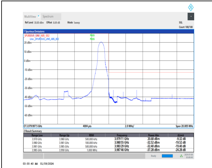
1-N77-3700-3980-30-10-H-2-DFT-PI2BPSK-Edge_1R_B_Right-1@23-Ant4-1--PASS-see graph
