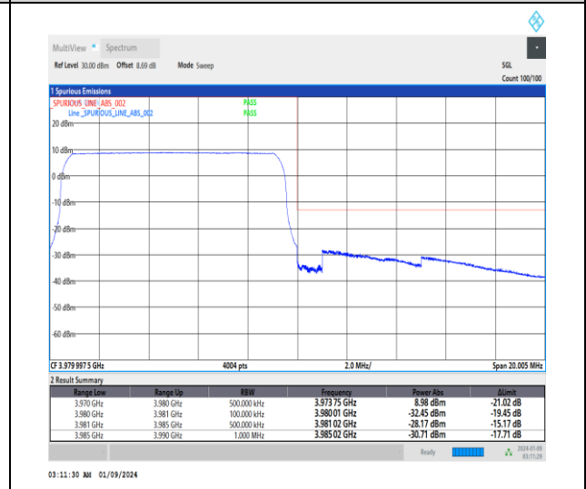
1-N77-3700-3980-30-10-H-6-CP-QPSK-Outer_Full-24@0-Ant4-1--PASS-see graph
