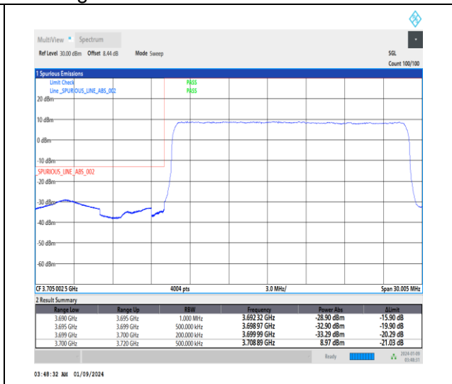
1-N77-3700-3980-30-20-L-3-DFT-PI2BPSK-Outer _Full-50@0-Ant4-1--PASS-see graph
