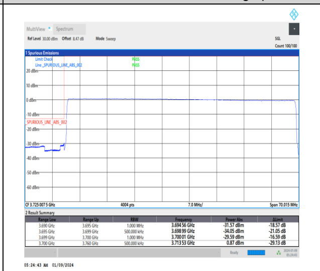
1-N77-3700-3980-30-60-L-6-CP-QPSK-Outer_Full -162@0-Ant4-1--PASS-see graph
