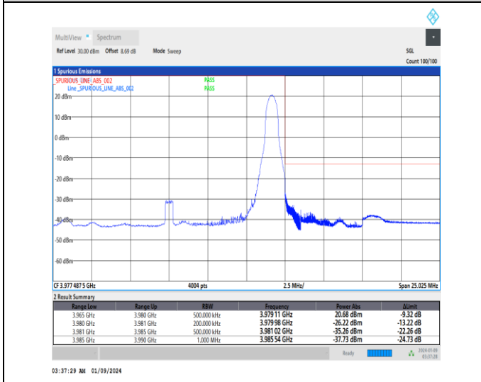
1-N77-3700-3980-30-15-H-5-CP-QPSK-Edge_1RB_Right-1@37-Ant4-1--PASS-see graph
