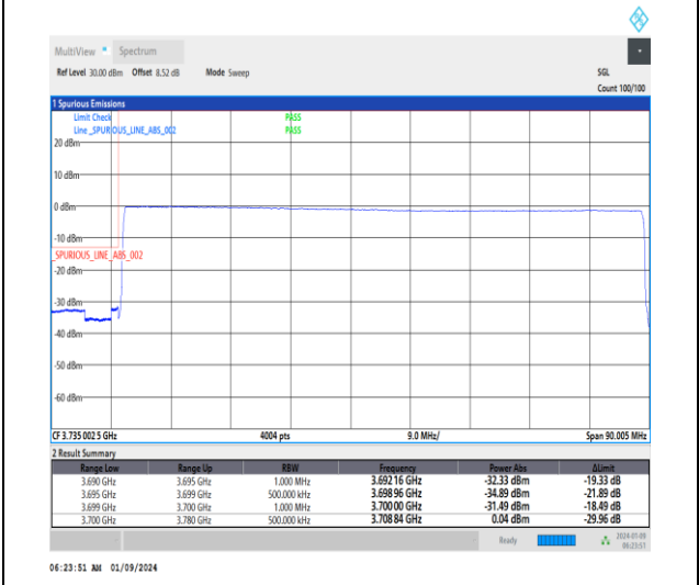
1-N77-3700-3980-30-80-L-6-CP-QPSK-Outer_Full -217@0-Ant4-1--PASS-see graph
