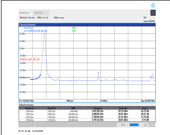
1-N77-3700-3980-30-50-L-4-CP-QPSK-Edge_1RB_Lef t-1@0-Ant4-1--PASS-see graph
