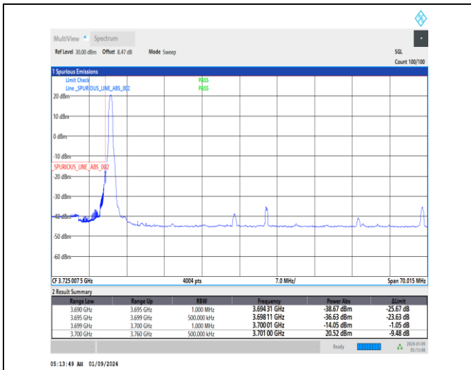
1-N77-3700-3980-30-60-L-1-DFT-PI2BPSK-Edge_1RB _Left-1@0-Ant4-1--PASS-see graph
