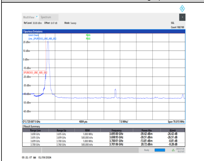
1-N77-3700-3980-30-60-L-4-CP-QPSK-Edge_1RB_Lef t-1@0-Ant4-1--PASS-see graph
