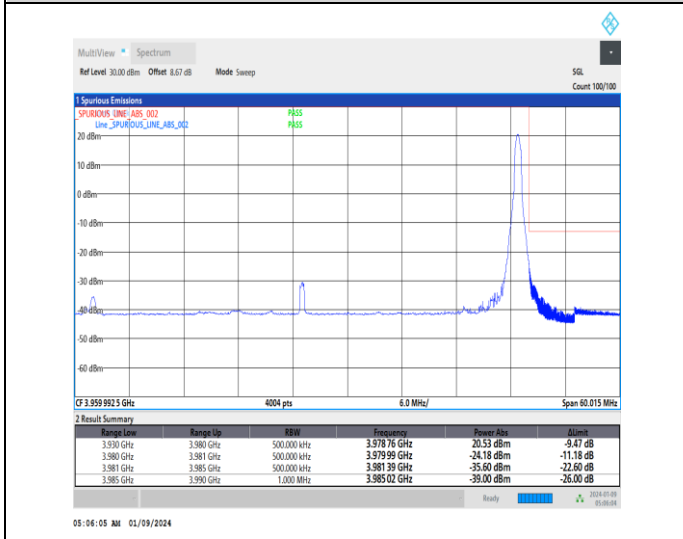
1-N77-3700-3980-30-50-H-5-CP-QPSK-Edge_1RB_Right-1@132-Ant4-1--PASS-see graph
