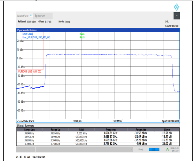
1-N77-3700-3980-30-50-L-3-DFT-PI2BPSK-Outer_Full-128@0-Ant4-1--PASS-see graph
