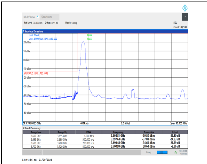
1-N77-3700-3980-30-20-L-1-DFT-PI2BPSK-Edge_1RB _Left-1@0-Ant4-1--PASS-see graph
