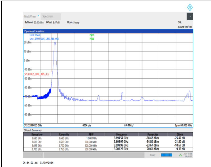
1-N77-3700-3980-30-50-L-1-DFT-PI2BPSK-Edge_1RB_Left-1@0-Ant4-1--PASS-see graph
