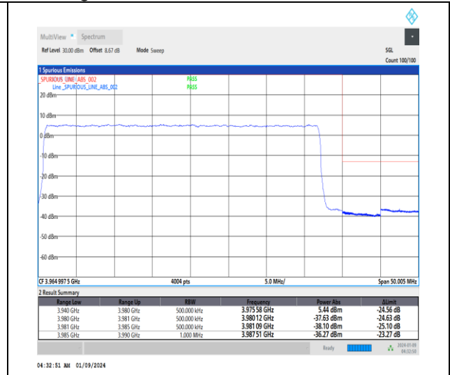
1-N77-3700-3980-30-40-H-3-DFT-PI2BPSK-Outer_Full-100@0-Ant4-1--PASS-see graph
