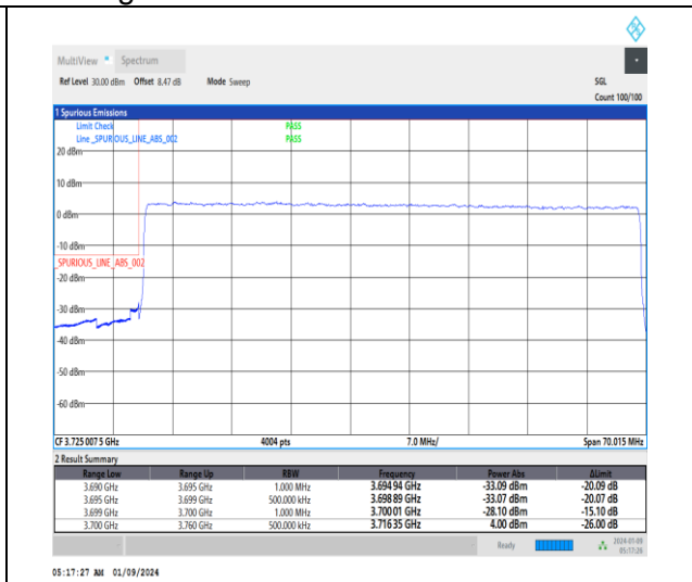
1-N77-3700-3980-30-60-L-3-DFT-PI2BPSK-Outer _Full-162@0-Ant4-1--PASS-see graph
