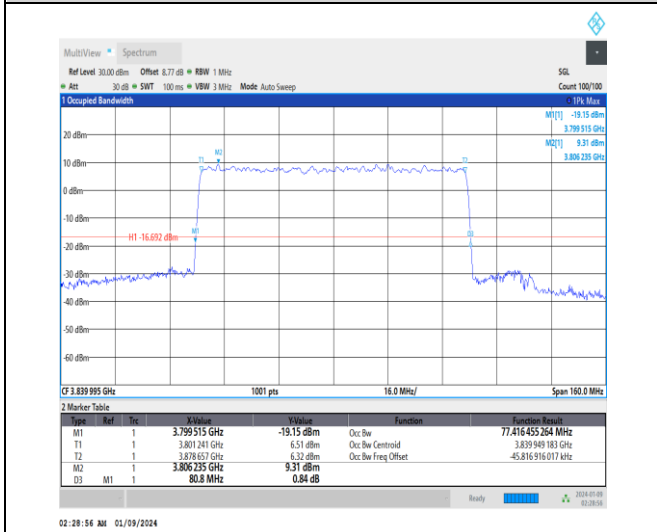
1-N77-3700-3980-30-80-M-9-CP-256QAM-Outer_Fu ll-217@0-Ant4-77.416-80.800-≤80-PASS
