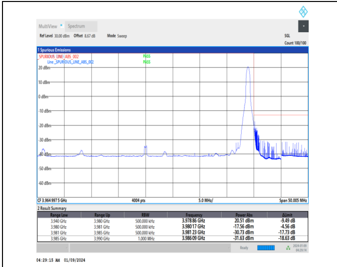
1-N77-3700-3980-30-40-H-2-DFT-PI2BPSK-Edge_1R_B_Right-1@105-Ant4-1--PASS-see graph
