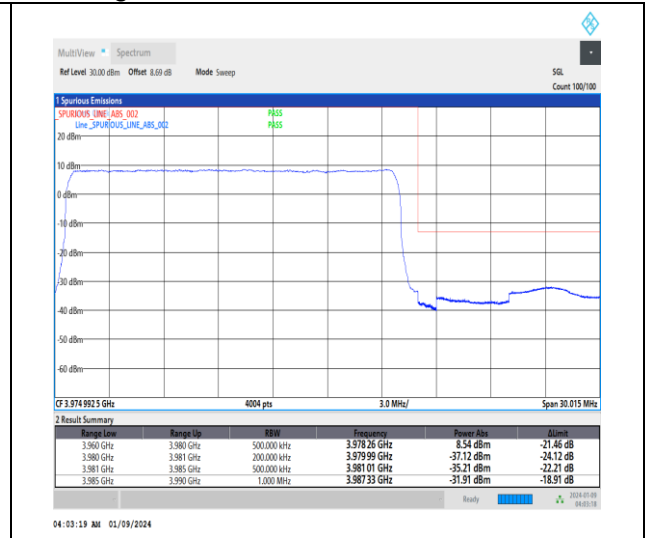
1-N77-3700-3980-30-20-H-3-DFT-PI2BPSK-Outer_Full-50@0-Ant4-1--PASS-see graph
