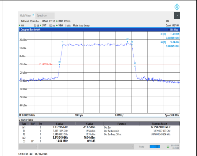
1-N77-3700-3980-30-15-M-3-DFT-16QAM-Outer_Full-36@0-Ant4-12.951-14.040-≤15-PASS
