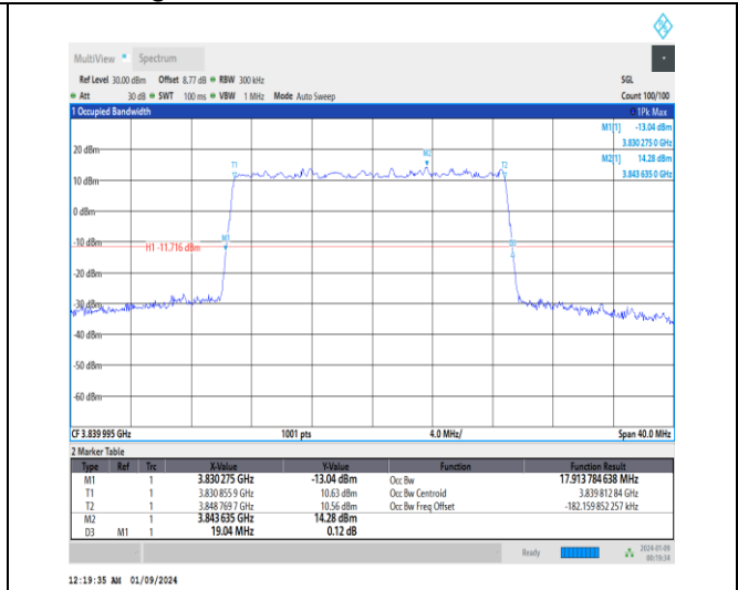
1-N77-3700-3980-30-20-M-4-DFT-64QAM-Outer_Ful I-50@0-Ant4-17.914-19.040-≤20-PASS
