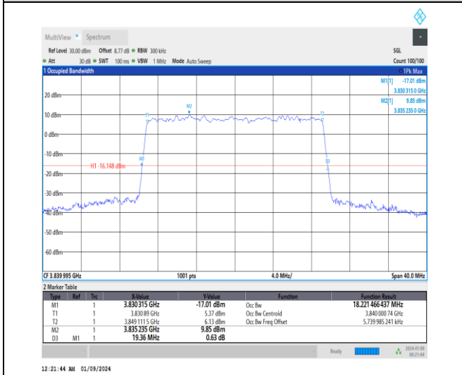
1-N77-3700-3980-30-20-M-9-CP-256QAM-Outer_Fu II-51@0-Ant4-18.221-19.360-<20-PASS
