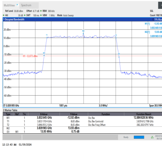
1-N77-3700-3980-30-15-M-5-DFT-256QAM-Outer_Full-36@0-Ant4-12.885-13.950-≤15-PASS
