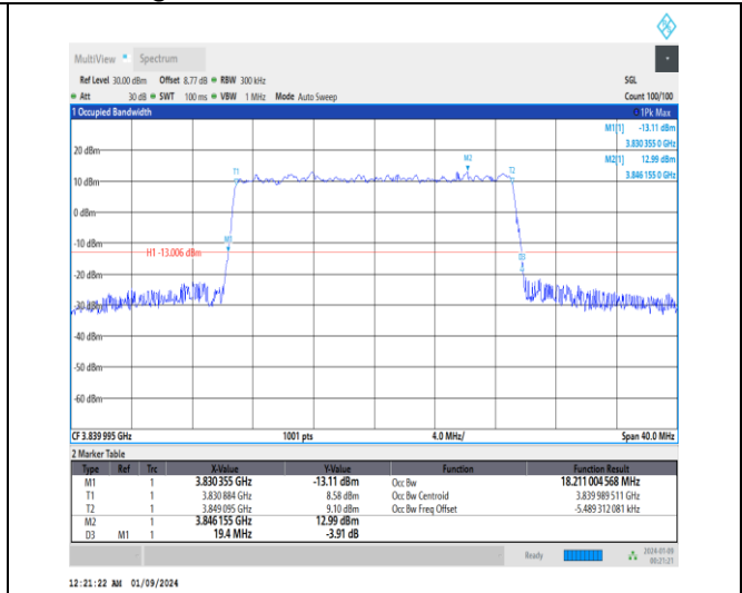
1-N77-3700-3980-30-20-M-8-CP-64QAM-Outer_Full -51@0-Ant4-18.211-19.400-<20-PASS
