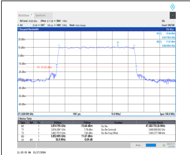
1-N77-3700-3980-30-50-M-9-CP-256QAM-Outer_Fu II-133@0-Ant4-47.584-50.400-≤50-PASS
