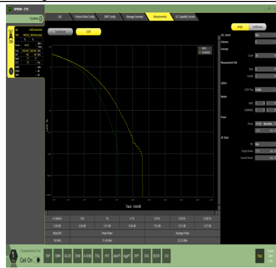
1-N77-3700-3980-30-100-H-15-CP-256QAM-Outer_ Full-270@0
