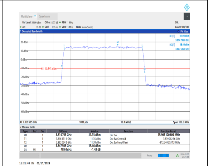
1-N77-3700-3980-30-50-M-4-DFT-64QAM-Outer_Full-128@0-Ant4-45.903-48.600-≤50-PASS
