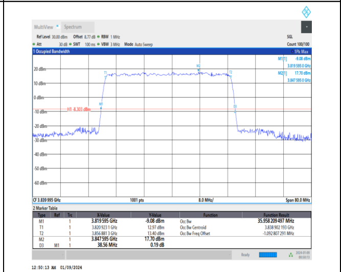
1-N77-3700-3980-30-40-M-1-DFT-QPSK-Outer_Full- 100@0-Ant4-35.958-38.560-<40-PASS
