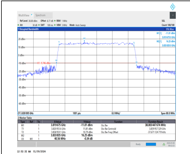
1-N77-3700-3980-30-40-M-6-CP-QPSK-Outer_Full-106@0-Ant4-38.003-40.560-≤40-PASS
