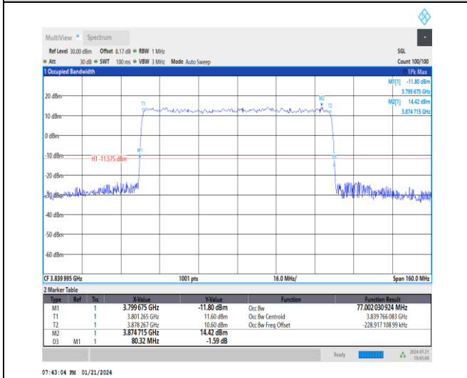
1-N77-3700-3980-30-80-M-1-DFT-PI2BPSK-Outer_Full-216@0-Ant4-77.002-80.320-≤80-PASS
