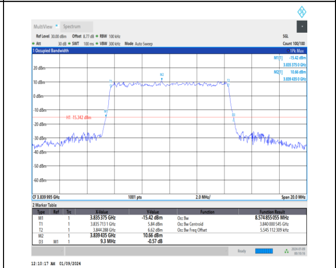
1-N77-3700-3980-30-10-M-8-CP-64QAM-Outer_Full-24@0-Ant4-8.575-9.300-≤10-PASS
