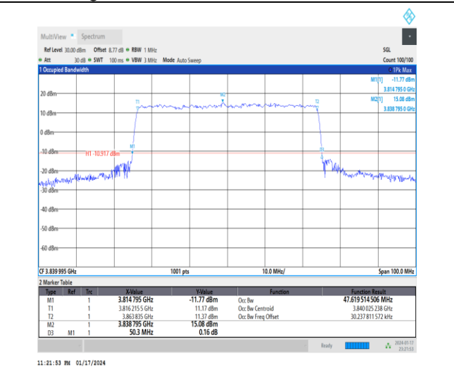
1-N77-3700-3980-30-50-M-6-CP-QPSK-Outer_Full-133@0-Ant4-47.62-50.300-≤50-PASS
