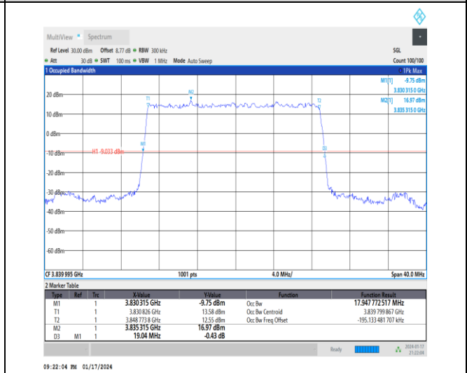
1-N77-3700-3980-30-20-M-2-DFT-PI2BPSK-Outer_F ull-50@0-Ant4-17.948-19.040-≤20-PASS
