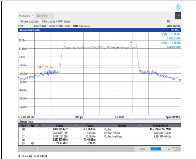
1-N77-3700-3980-30-20-M-7-CP-16QAM-Outer_Full -51@0-Ant4-18.238-19.360-<20-PASS
