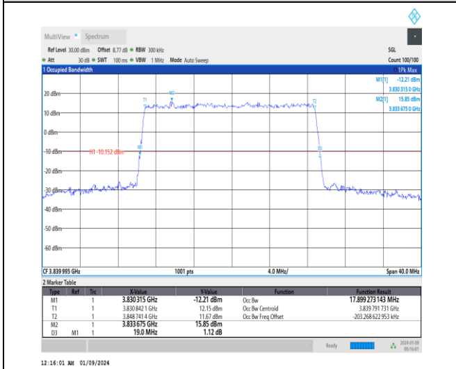
1-N77-3700-3980-30-20-M-1-DFT-QPSK-Outer_Full- 50@0-Ant4-17.899-19.000-≤20-PASS
