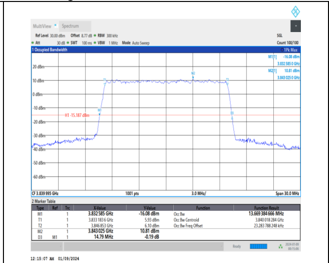
1-N77-3700-3980-30-15-M-9-CP-256QAM-Outer_Ful I-38@0-Ant4-13.669-14.790-≤15-PASS
