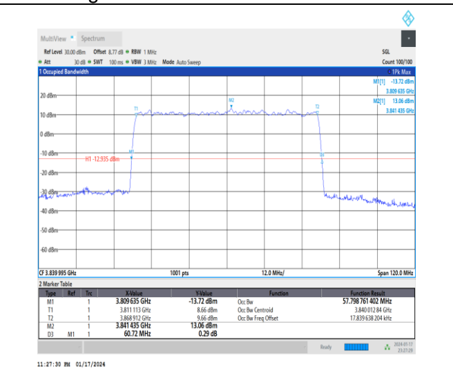
1-N77-3700-3980-30-60-M-5-DFT-256QAM-Outer_F uII-162@0-Ant4-57.799-60.720-≤60-PASS
