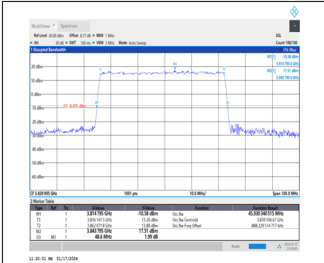
1-N77-3700-3980-30-50-M-1-DFT-QPSK-Outer_Full-128@0-Ant4-45.93-48.600-≤50-PASS
