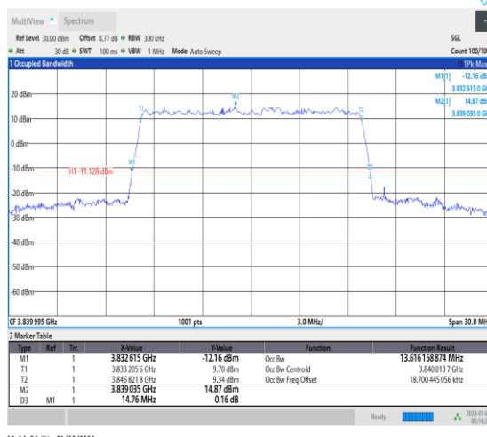
1-N77-3700-3980-30-15-M-7-CP-16QAM-Outer_Full-38@0-Ant4-13.616-14.760-≤15-PASS
