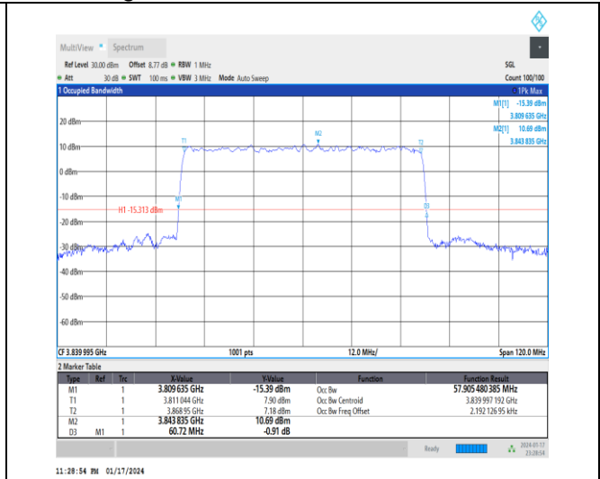
1-N77-3700-3980-30-60-M-9-CP-256QAM-Outer_Ful I-162@0-Ant4-57.905-60.720-≤60-PASS
