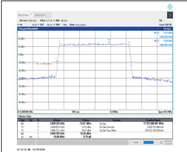
1-N77-3700-3980-30-20-M-3-DFT-16QAM-Outer_Fu II-50@0-Ant4-17.916-19.080-≤20-PASS
