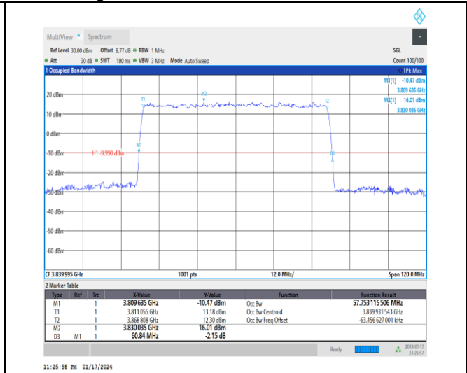
1-N77-3700-3980-30-60-M-1-DFT-QPSK-Outer_Full-162@0-Ant4-57.753-60.840-≤60-PASS
