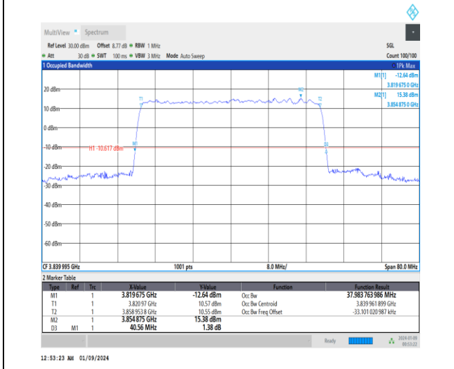
1-N77-3700-3980-30-40-M-8-CP-64QAM-Outer_Full-106@0-Ant4-37.984-40.560-≤40-PASS
