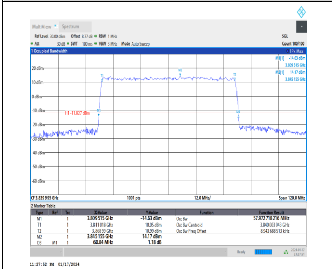
1-N77-3700-3980-30-60-M-6-CP-QPSK-Outer_Full-162@0-Ant4-57.973-60.840-≤60-PASS
