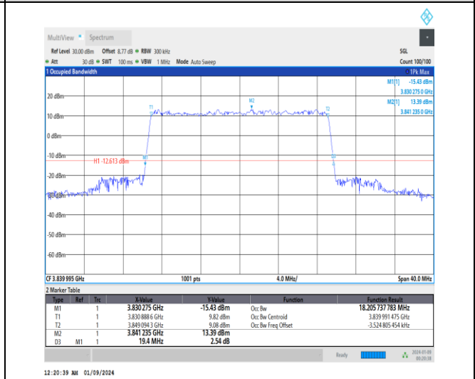
1-N77-3700-3980-30-20-M-6-CP-QPSK-Outer_Full-5@0-Ant4-18.206-19.400-≤20-PASS
