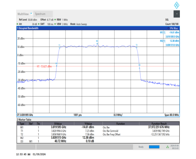
1-N77-3700-3980-30-40-M-9-CP-256QAM-Outer_Full-106@0-Ant4-37.972-40.720-≤40-PASS
