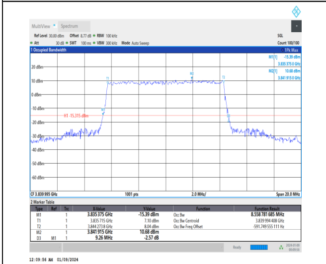
1-N77-3700-3980-30-10-M-7-CP-16QAM-Outer_Full-24@0-Ant4-8.559-9.260-≤10-PASS
