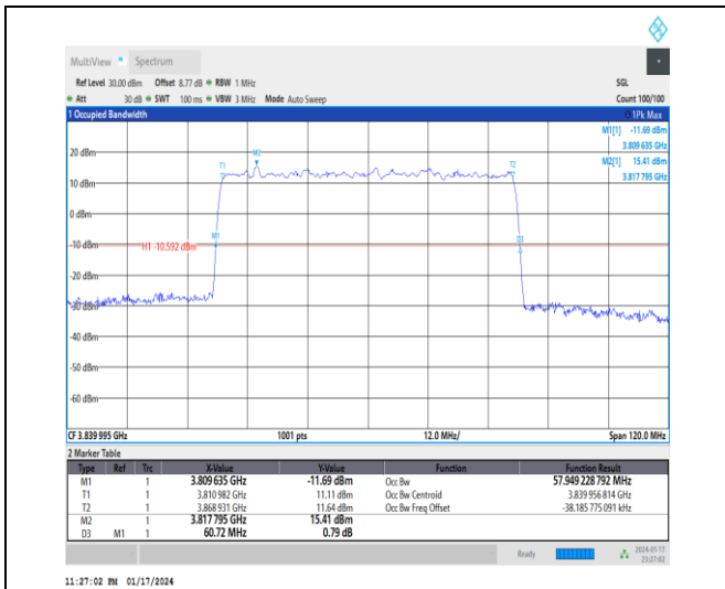
1-N77-3700-3980-30-60-M-4-DFT-64QAM-Outer_Fu II-162@0-Ant4-57.949-60.720-≤60-PASS
