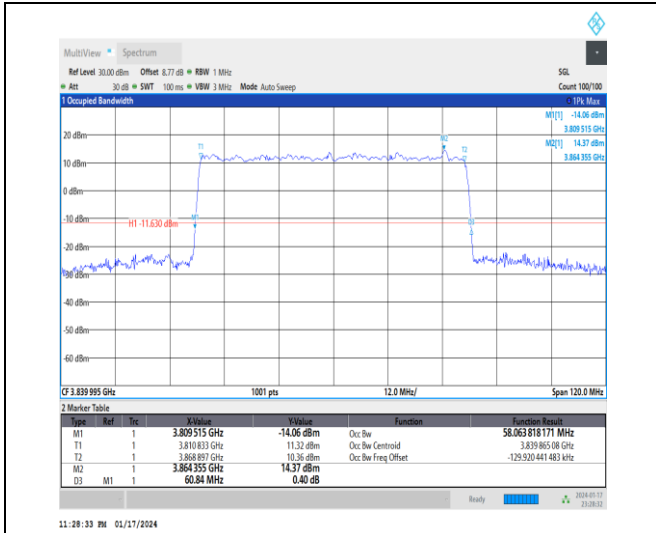
1-N77-3700-3980-30-60-M-8-CP-64QAM-Outer_Full -162@0-Ant4-58.064-60.840-≤60-PASS
