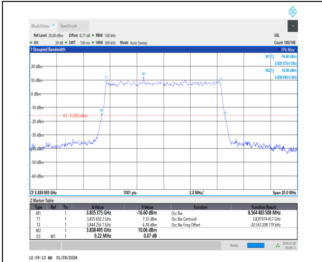
1-N77-3700-3980-30-10-M-5-DFT-256QAM-Outer_Full-24@0-Ant4-8.564-9.220-≤10-PASS
