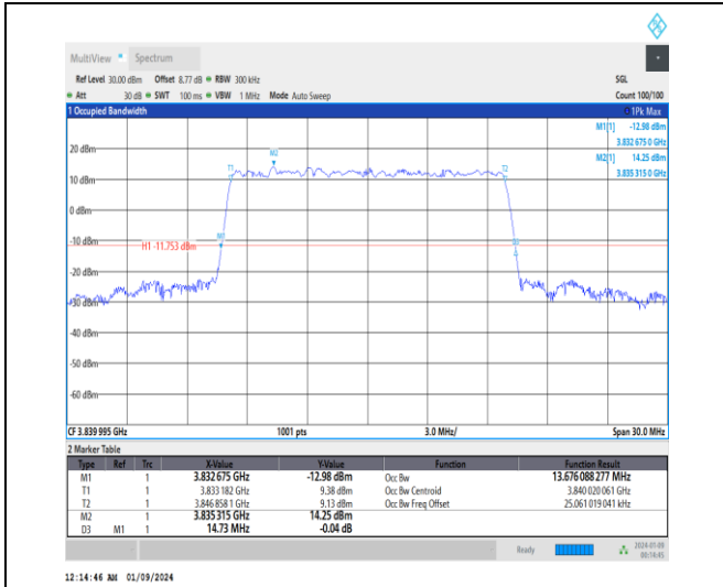
1-N77-3700-3980-30-15-M-8-CP-64QAM-Outer_Full -38@0-Ant4-13.676-14.730-≤15-PASS
