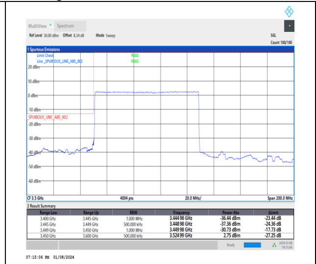
1-N77-3450-3550-30-80-L-3-DFT-PI2BPSK-Outer _Full-216@0-Ant4-1--PASS-see graph
