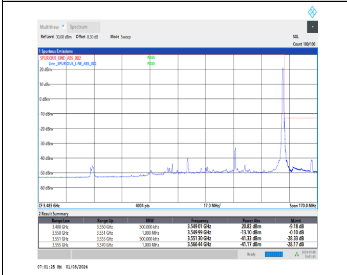
1-N77-3450-3550-30-60-H-5-CP-QPSK-Edge_1RB_Right-1@161-Ant4-1--PASS-see graph
