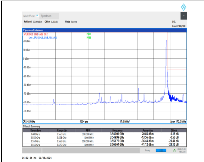
1-N77-3450-3550-30-60-H-2-DFT-PI2BPSK-Edge_1R_B_Right-1@161-Ant4-1--PASS-see graph
