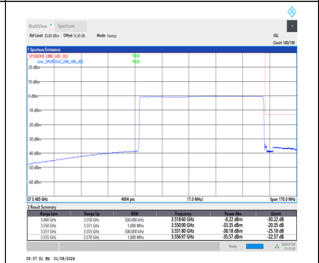
1-N77-3450-3550-30-80-H-6-CP-QPSK-Outer_Full-217@0-Ant4-1--PASS-see graph
