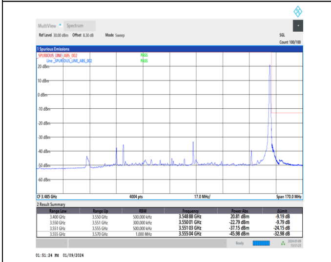
1-N77-3450-3550-30-100-H-5-CP-QPSK-Edge_1RB_Right-1@272-Ant4-1--PASS-see graph
