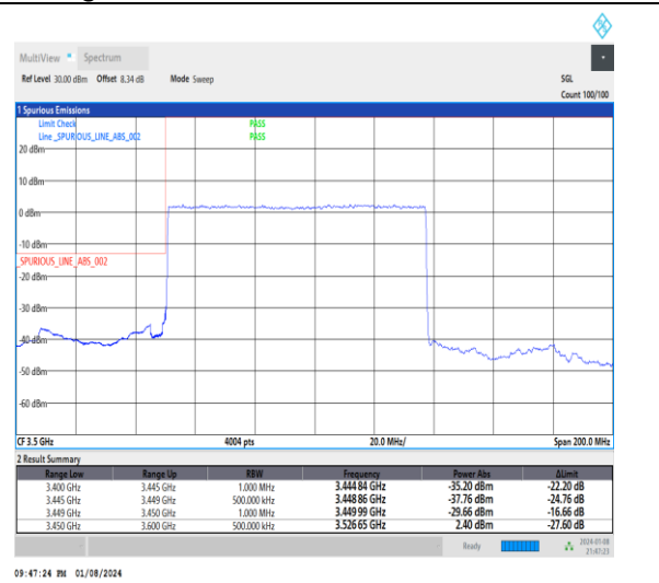
1-N77-3450-3550-30-90-L-3-DFT-PI2BPSK-Outer _Full-240@0-Ant4-1--PASS-see graph
