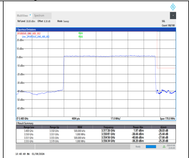
1-N77-3450-3550-30-100-H-3-DFT-PI2BPSK-Outer_Full-270@0-Ant4-1--PASS-see graph
