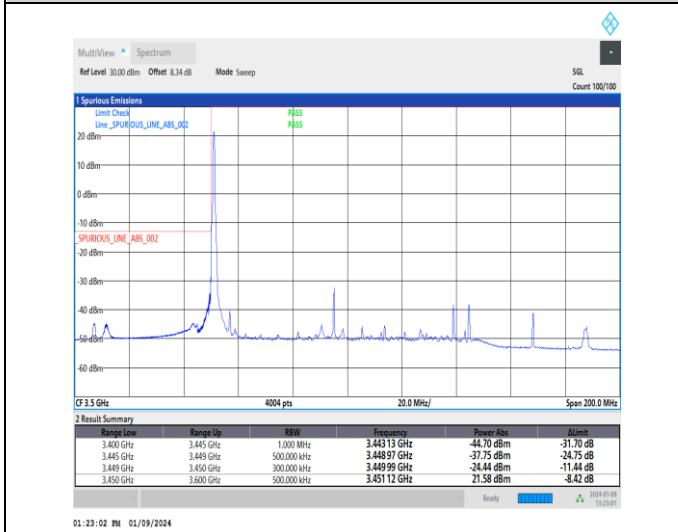
1-N77-3450-3550-30-90-L-4-CP-QPSK-Edge_1RB_Lef t-1@0-Ant4-1--PASS-see graph
