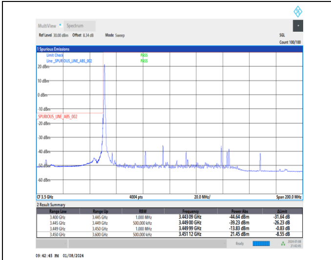
1-N77-3450-3550-30-90-L-1-DFT-PI2BPSK-Edge_1RB _Left-1@0-Ant4-1--PASS-see graph
