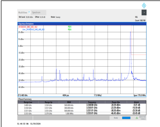
1-N77-3450-3550-30-100-H-2-DFT-PI2BPSK-Edge_1R_B_Right-1@272-Ant4-1--PASS-see graph
