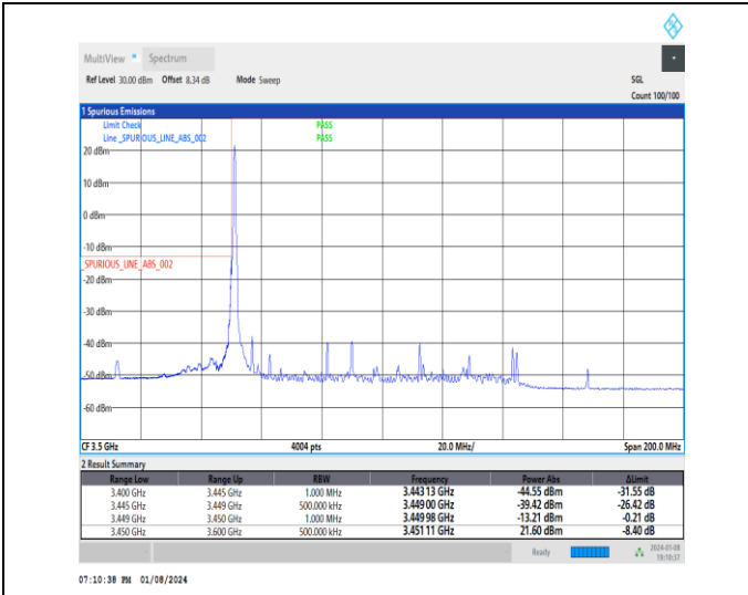
1-N77-3450-3550-30-80-L-1-DFT-PI2BPSK-Edge_1RB _Left-1@0-Ant4-1--PASS-see graph
