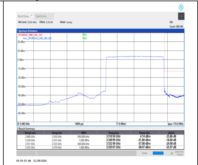
1-N77-3450-3550-30-60-H-3-DFT-PI2BPSK-Outer_Full-162@0-Ant4-1--PASS-see graph
