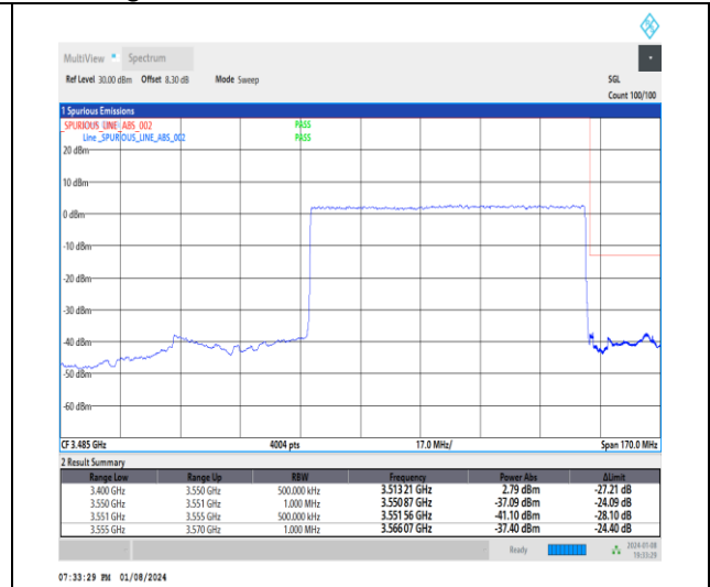
1-N77-3450-3550-30-80-H-3-DFT-PI2BPSK-Outer_Full-216@0-Ant4-1--PASS-see graph
