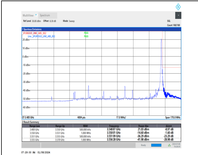
1-N77-3450-3550-30-80-H-2-DFT-PI2BPSK-Edge_1R_B_Right-1@216-Ant4-1--PASS-see graph
