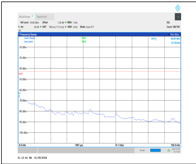
1-N77-3450-3550-30-100-H-1-DFT-PI2BPSK-Inner_1RB_Left-1@1-0.009-0.15-Ant4-0.01--66.60--43-PA SS
