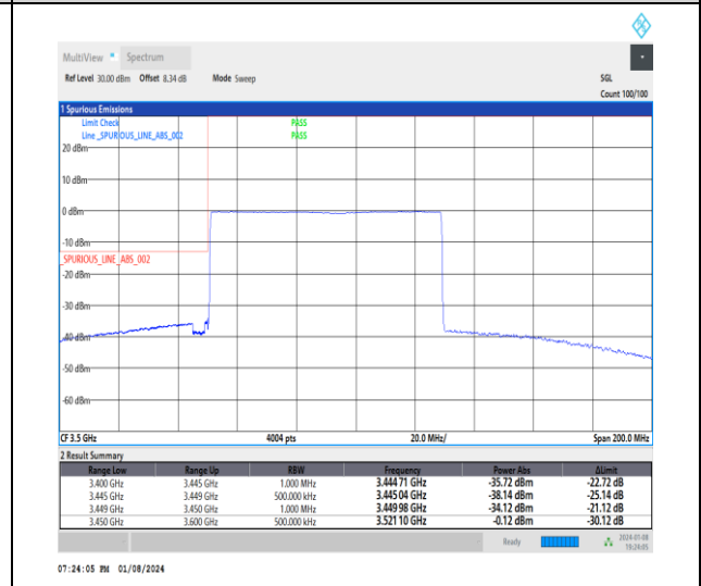
1-N77-3450-3550-30-80-L-6-CP-QPSK-Outer_Full -217@0-Ant4-1--PASS-see graph
