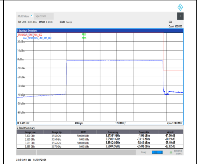
1-N77-3450-3550-30-100-H-6-CP-QPSK-Outer_Full-273@0-Ant4-1--PASS-see graph
