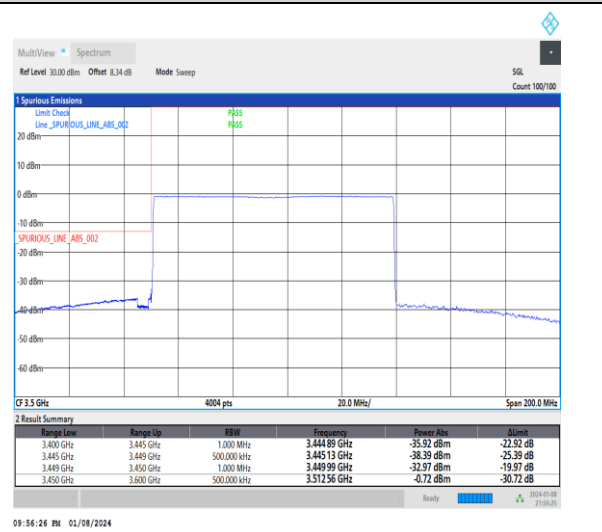
1-N77-3450-3550-30-90-L-6-CP-QPSK-Outer_Full -245@0-Ant4-1--PASS-see graph
