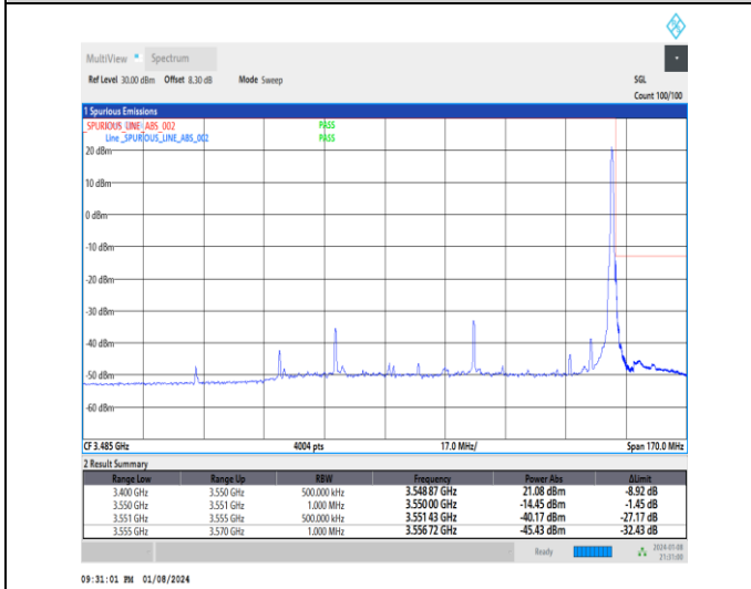
1-N77-3450-3550-30-80-H-5-CP-QPSK-Edge_1RB_Right-1@216-Ant4-1--PASS-see graph
