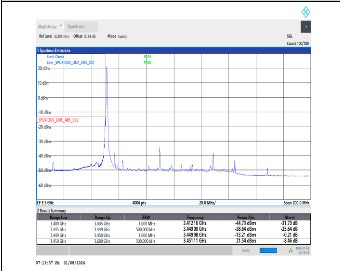
1-N77-3450-3550-30-80-L-4-CP-QPSK-Edge_1RB_Lef t-1@0-Ant4-1--PASS-see graph
