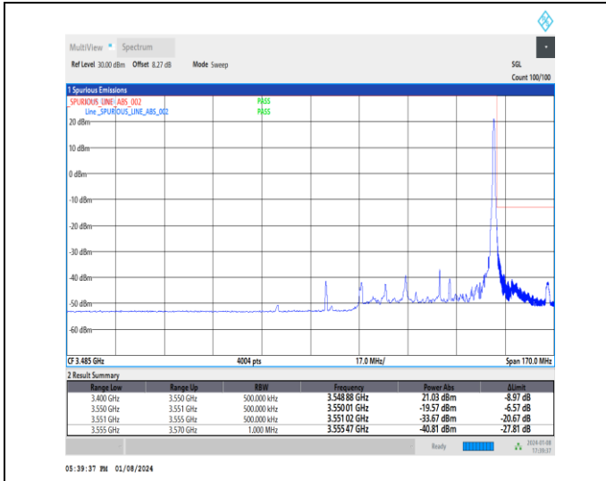
1-N77-3450-3550-30-40-H-2-DFT-PI2BPSK-Edge_1R_B_Right-1@105-Ant4-1--PASS-see graph
