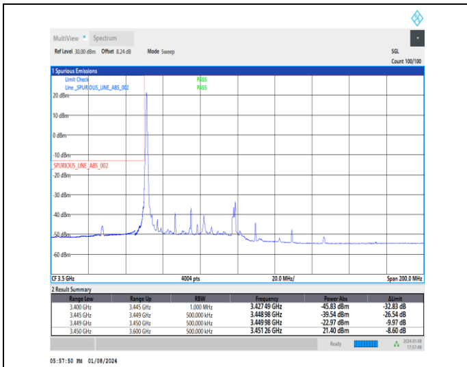
1-N77-3450-3550-30-50-L-1-DFT-PI2BPSK-Edge_1RB _Left-1@0-Ant4-1--PASS-see graph
