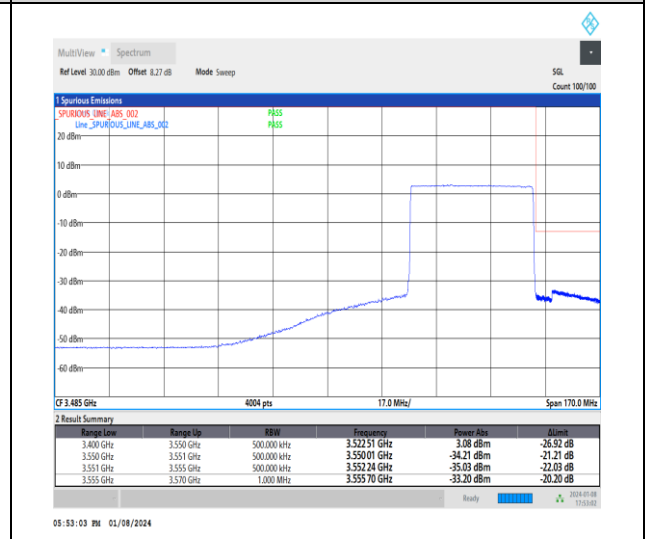
1-N77-3450-3550-30-40-H-6-CP-QPSK-Outer_Full-106@0-Ant4-1--PASS-see graph
