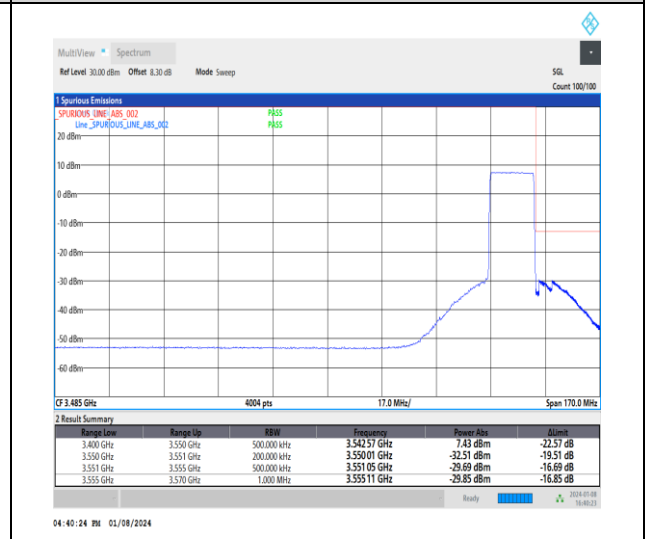
1-N77-3450-3550-30-15-H-6-CP-QPSK-Outer_Full-38@0-Ant4-1--PASS-see graph
