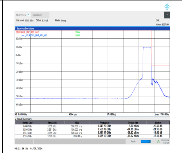
1-N77-3450-3550-30-10-H-6-CP-QPSK-Outer_Full-24@0-Ant4-1--PASS-see graph
