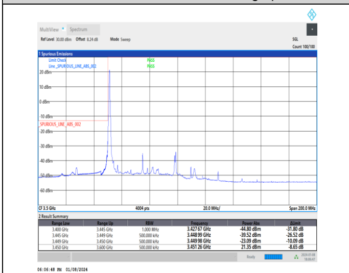
1-N77-3450-3550-30-50-L-4-CP-QPSK-Edge_1RB_Lef t-1@0-Ant4-1--PASS-see graph
