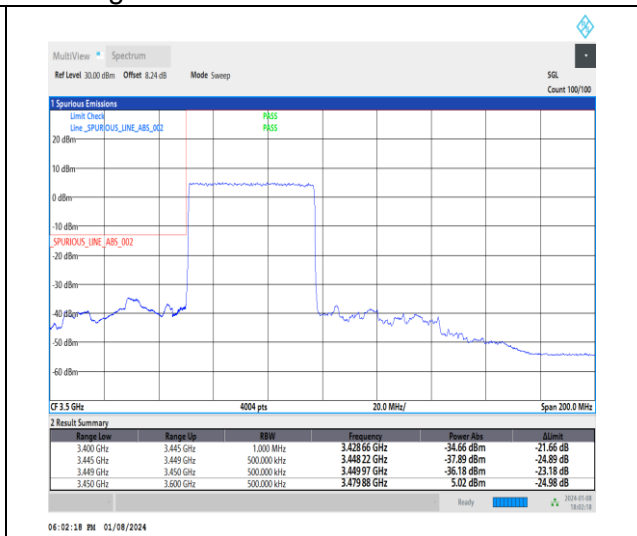
1-N77-3450-3550-30-50-L-3-DFT-PI2BPSK-Outer _Full-128@0-Ant4-1--PASS-see graph
