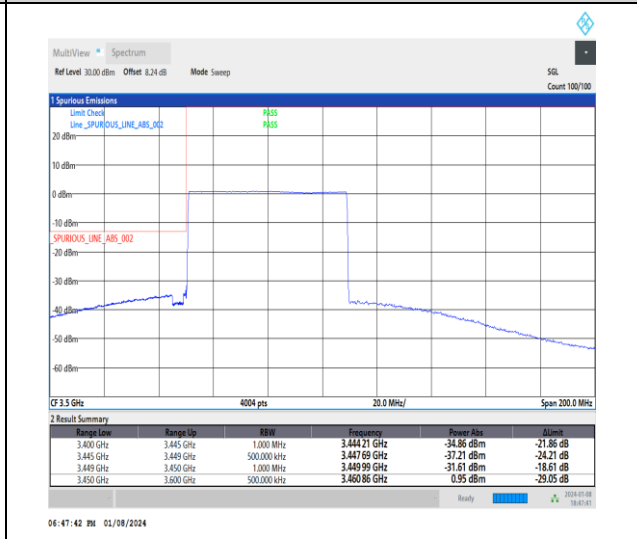
1-N77-3450-3550-30-60-L-6-CP-QPSK-Outer_Full -162@0-Ant4-1--PASS-see graph
