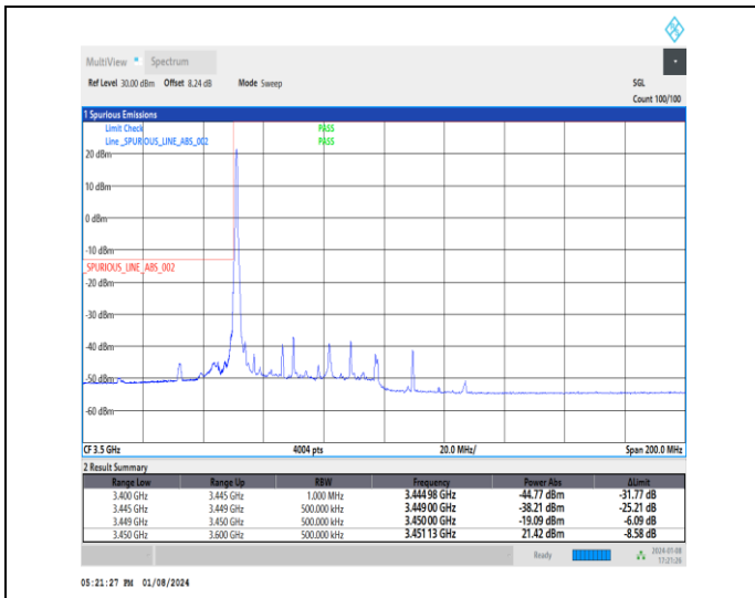
1-N77-3450-3550-30-40-L-1-DFT-PI2BPSK-Edge_1RB _Left-1@0-Ant4-1--PASS-see graph
