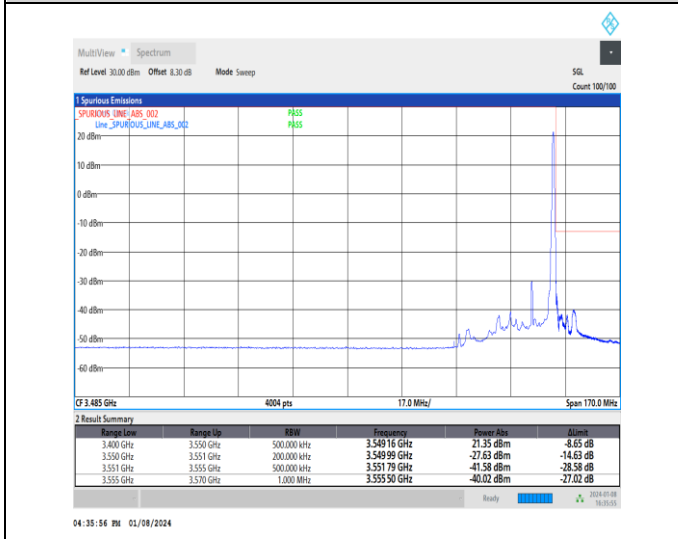
1-N77-3450-3550-30-15-H-5-CP-QPSK-Edge_1RB_Right-1@37-Ant4-1--PASS-see graph
