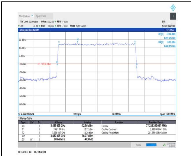
1-N77-3450-3550-30-80-M-2-DFT-PI2BPSK-Outer_F ull-216@0-Ant4-77.226-80.640-≤80-PASS
