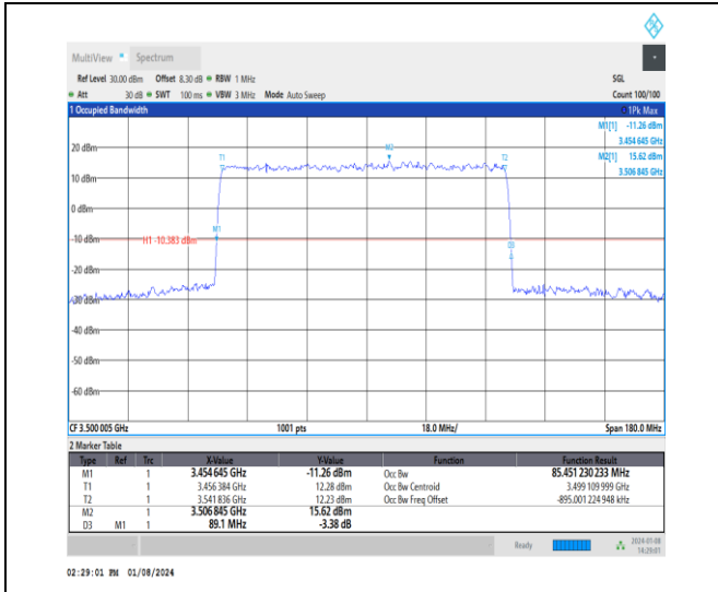
1-N77-3450-3550-30-90-M-1-DFT-QPSK-Outer_Full-240@0-Ant4-85.451-89.100-≤90-PASS
