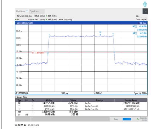
1-N77-3450-3550-30-80-M-4-DFT-64QAM-Outer_Ful l-216@0-Ant4-77.168-80.480-≤80-PASS
