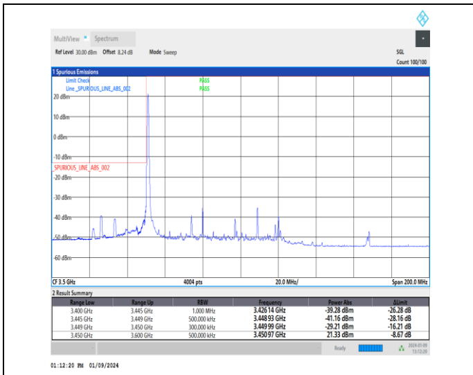
1-N77-3450-3550-30-60-L-1-DFT-PI2BPSK-Edge_1RB _Left-1@0-Ant4-1--PASS-see graph
