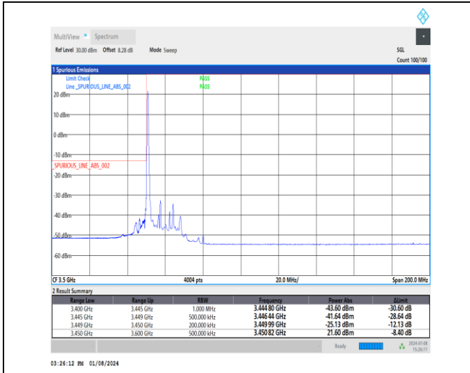
1-N77-3450-3550-30-15-L-1-DFT-PI2BPSK-Edge_1RB _Left-1@0-Ant4-1--PASS-see graph
