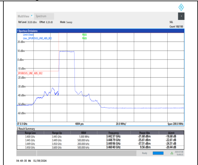
1-N77-3450-3550-30-20-L-3-DFT-PI2BPSK-Outer _Full-50@0-Ant4-1--PASS-see graph
