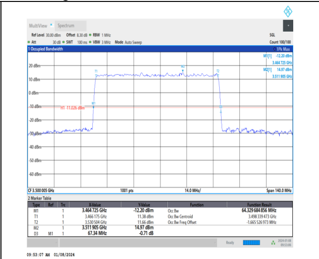
1-N77-3450-3550-30-70-M-4-DFT-64QAM-Outer_Fu II-180@0-Ant4-64.33-67.340-≤70-PASS
