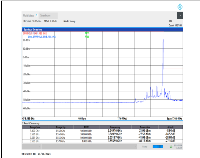
1-N77-3450-3550-30-15-H-2-DFT-PI2BPSK-Edge_1R_B_Right-1@37-Ant4-1--PASS-see graph
