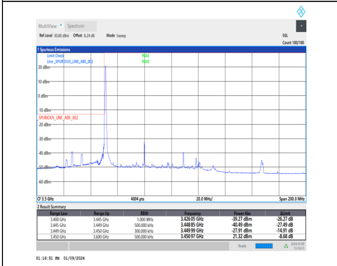
1-N77-3450-3550-30-60-L-4-CP-QPSK-Edge_1RB_Lef t-1@0-Ant4-1--PASS-see graph
