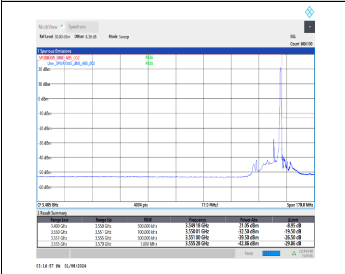
1-N77-3450-3550-30-10-H-5-CP-QPSK-Edge_1RB_Right-1@23-Ant4-1--PASS-see graph
