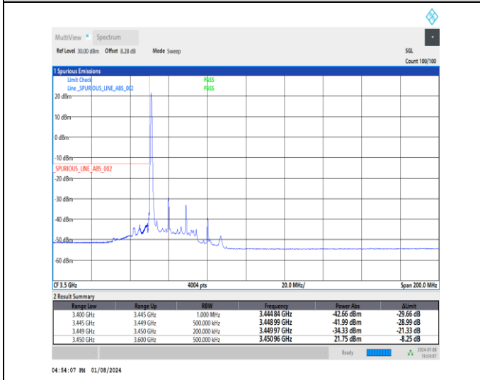
1-N77-3450-3550-30-20-L-4-CP-QPSK-Edge_1RB_Lef t-1@0-Ant4-1--PASS-see graph
