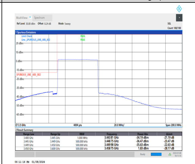
1-N77-3450-3550-30-50-L-6-CP-QPSK-Outer_Full -133@0-Ant4-1--PASS-see graph
