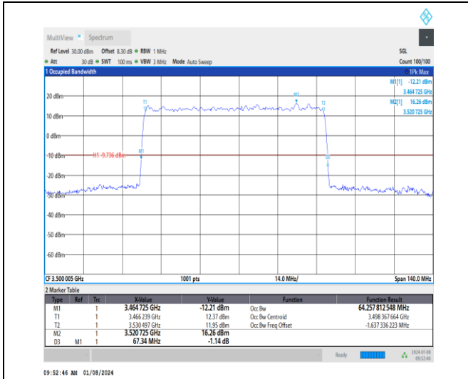
1-N77-3450-3550-30-70-M-3-DFT-16QAM-Outer_Ful I-180@0-Ant4-64.258-67.340-≤70-PASS
