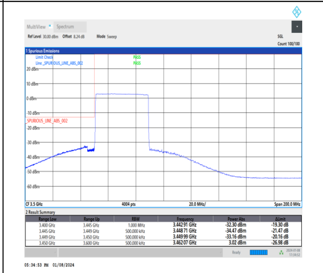
1-N77-3450-3550-30-40-L-6-CP-QPSK-Outer_Full -106@0-Ant4-1--PASS-see graph
