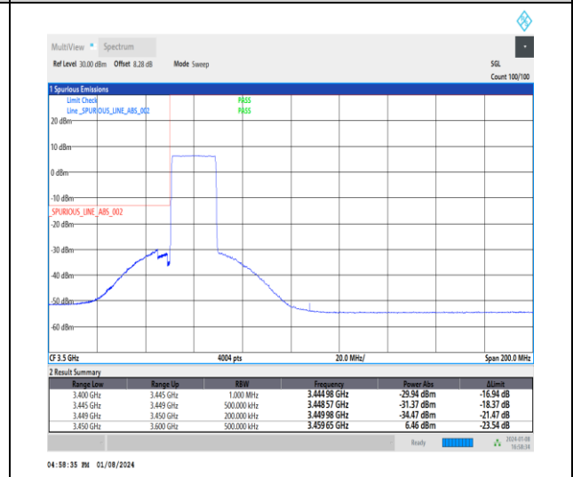
1-N77-3450-3550-30-20-L-6-CP-QPSK-Outer_Full -51@0-Ant4-1--PASS-see graph
