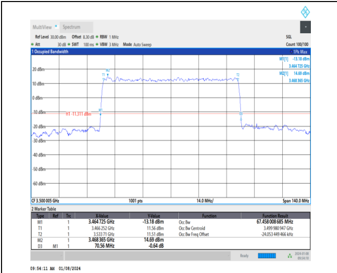
1-N77-3450-3550-30-70-M-7-CP-16QAM-Outer_Full-189@0-Ant4-67.458-70.560-≤70-PASS
