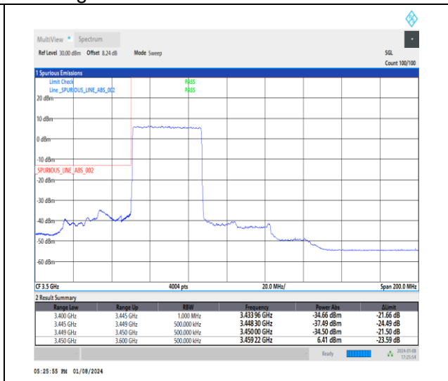
1-N77-3450-3550-30-40-L-3-DFT-PI2BPSK-Outer _Full-100@0-Ant4-1--PASS-see graph
