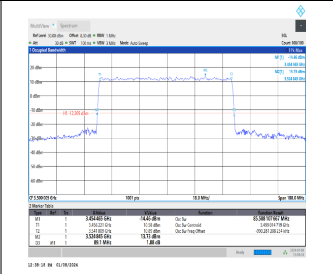
1-N77-3450-3550-30-90-M-4-DFT-64QAM-Outer_Fu ll-240@0-Ant4-85.588-89.100-≤90-PASS
