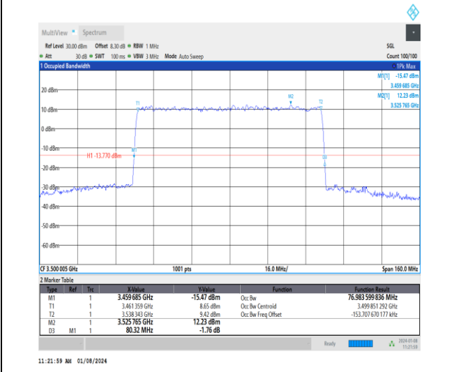
1-N77-3450-3550-30-80-M-5-DFT-256QAM-Outer_F ull-216@0-Ant4-76.984-80.320-≤80-PASS
