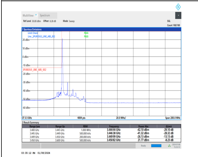
1-N77-3450-3550-30-15-L-4-CP-QPSK-Edge_1RB_Lef t-1@0-Ant4-1--PASS-see graph
