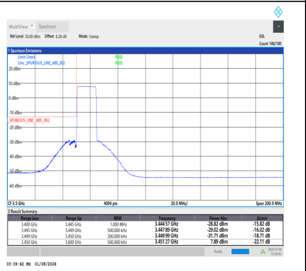
1-N77-3450-3550-30-15-L-6-CP-QPSK-Outer_Full -38@0-Ant4-1--PASS-see graph
