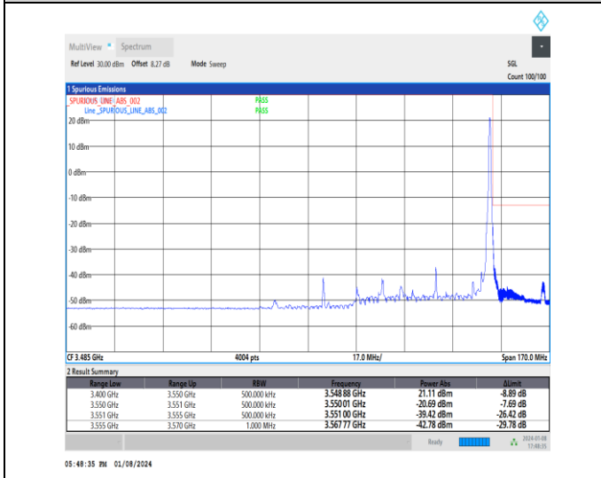
1-N77-3450-3550-30-40-H-5-CP-QPSK-Edge_1RB_Right-1@105-Ant4-1--PASS-see graph
