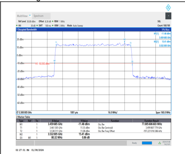
1-N77-3450-3550-30-80-M-3-DFT-16QAM-Outer_Fu ll-216@0-Ant4-77.006-80.320-≤80-PASS
