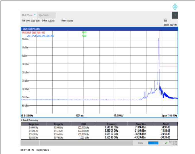
1-N77-3450-3550-30-10-H-2-DFT-PI2BPSK-Edge_1R_B_Right-1@23-Ant4-1--PASS-see graph
