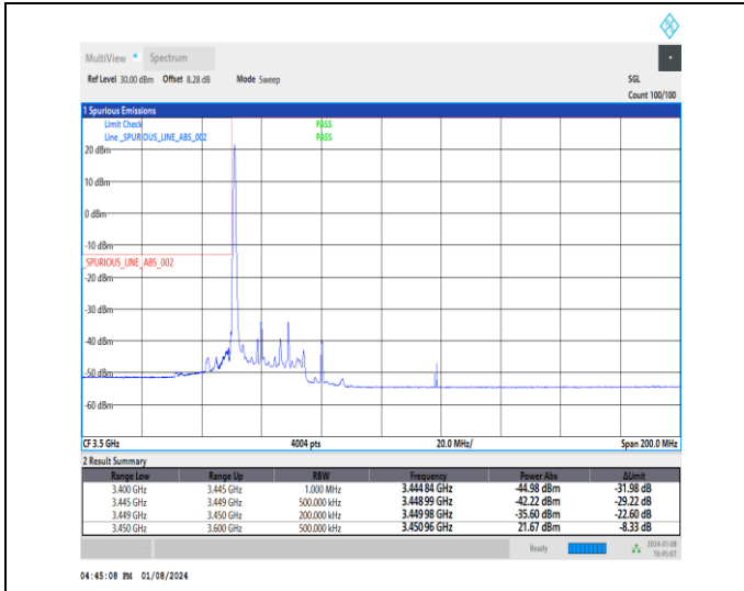
1-N77-3450-3550-30-20-L-1-DFT-PI2BPSK-Edge_1RB _Left-1@0-Ant4-1--PASS-see graph
