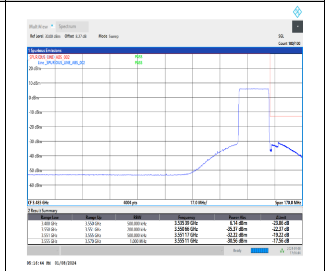
1-N77-3450-3550-30-20-H-6-CP-QPSK-Outer_Full-51@0-Ant4-1--PASS-see graph
