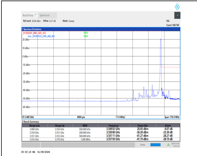
1-N77-3450-3550-30-20-H-2-DFT-PI2BPSK-Edge_1R_B_Right-1@50-Ant4-1--PASS-see graph
