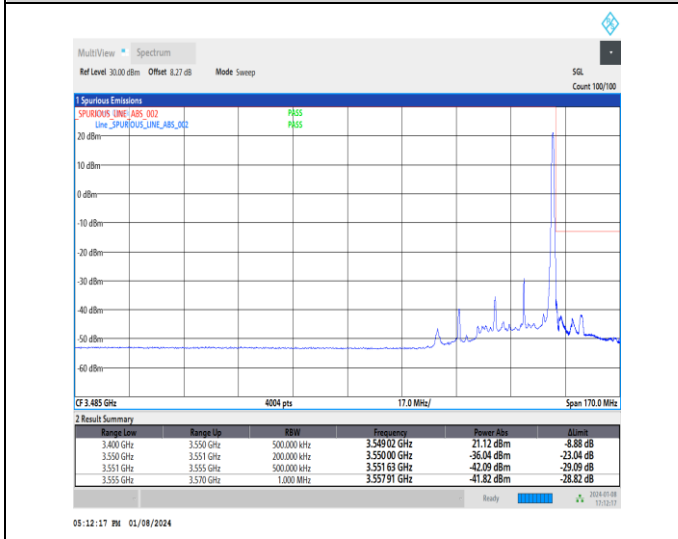
1-N77-3450-3550-30-20-H-5-CP-QPSK-Edge_1RB_Right-1@50-Ant4-1--PASS-see graph
