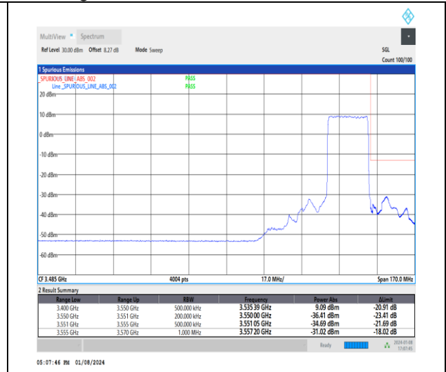
1-N77-3450-3550-30-20-H-3-DFT-PI2BPSK-Outer_Full-50@0-Ant4-1--PASS-see graph
