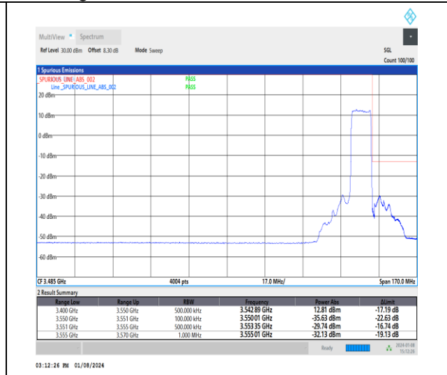
1-N77-3450-3550-30-10-H-3-DFT-PI2BPSK-Outer_Full-24@0-Ant4-1--PASS-see graph
