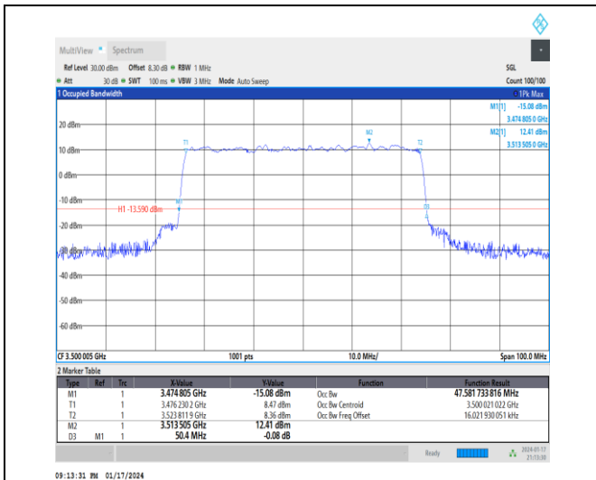
1-N77-3450-3550-30-50-M-9-CP-256QAM-Outer_Full-I-133@0-Ant4-47.582-50.400-≤50-PASS
