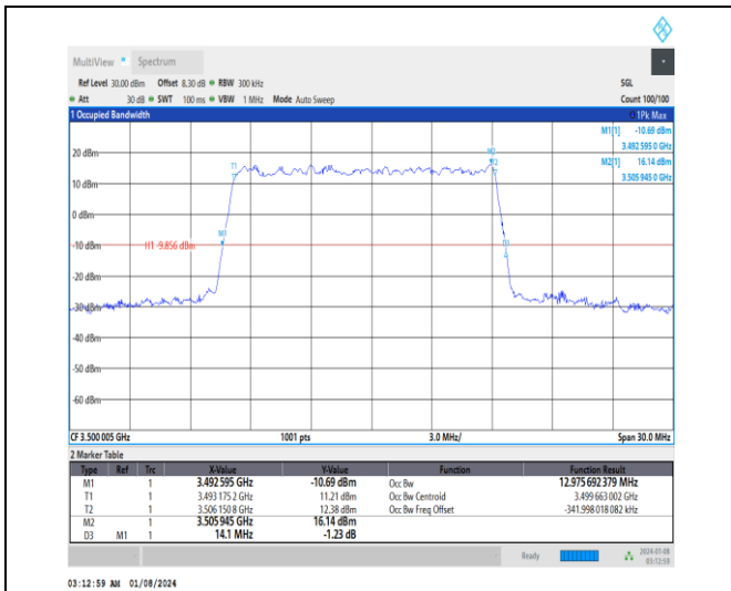
1-N77-3450-3550-30-15-M-4-DFT-64QAM-Outer_Full-I-36@0-Ant4-12.976-14.100-≤15-PASS
