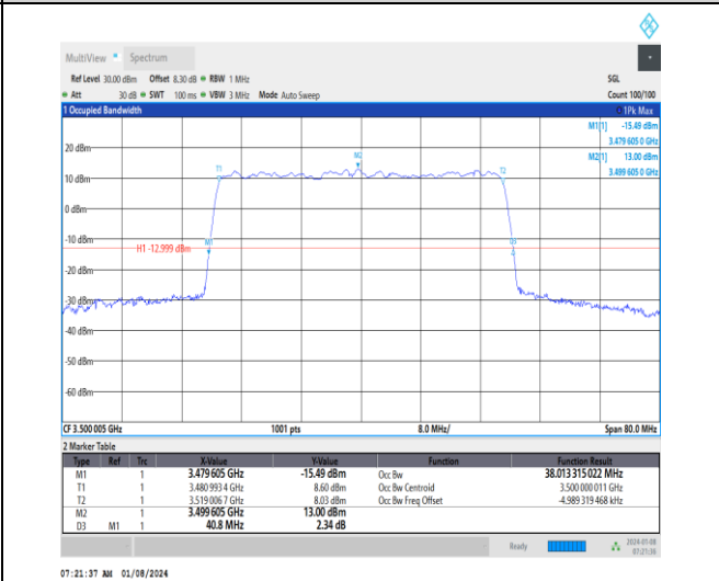
1-N77-3450-3550-30-40-M-9-CP-256QAM-Outer_Full-1 106@0-Ant4-38.013-40.800-≤40-PASS
