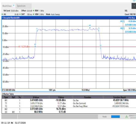
1-N77-3450-3550-30-50-M-3-DFT-16QAM-Outer_Full-128@0-Ant4-45.829-48.600-≤50-PASS
