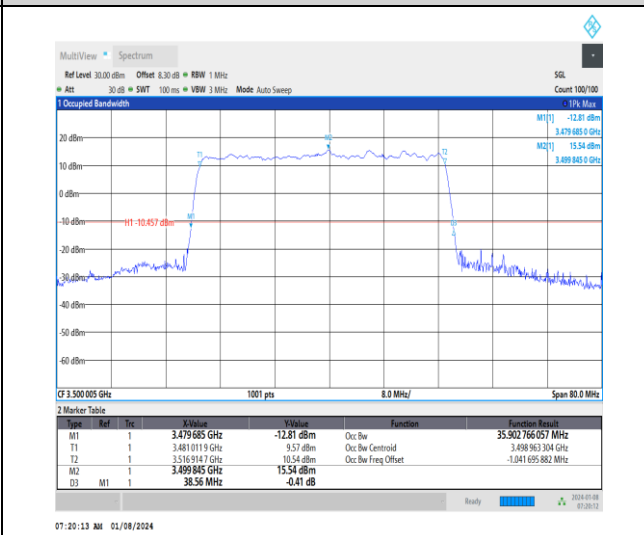
1-N77-3450-3550-30-40-M-5-DFT-256QAM-Outer_F ull-100@0-Ant4-35.903-38.560-≤40-PASS
