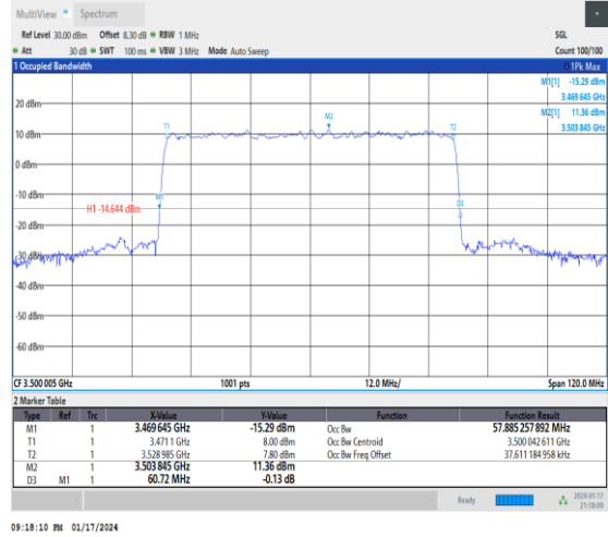
1-N77-3450-3550-30-60-M-9-CP-256QAM-Outer_Fu-II-162@0-Ant4-57.885-60.720-≤60-PASS
