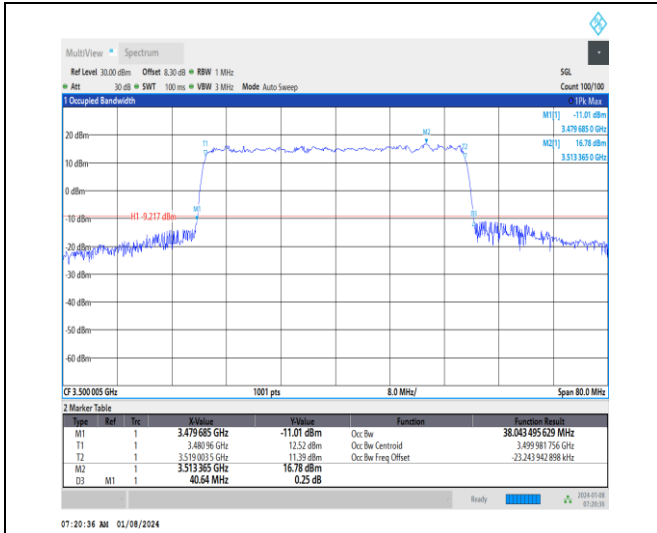
1-N77-3450-3550-30-40-M-6-CP-QPSK-Outer_Full-1 06@0-Ant4-38.043-40.640-≤40-PASS
