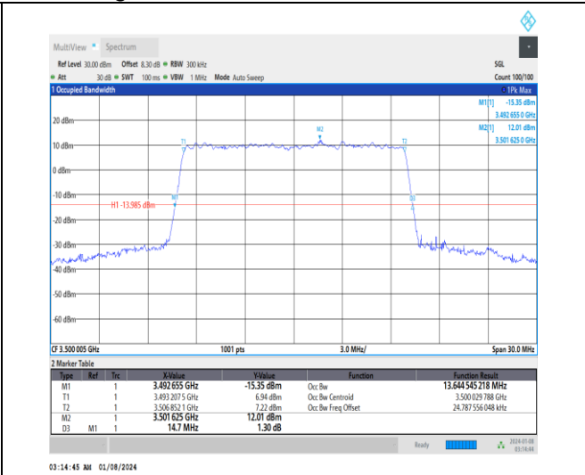
1-N77-3450-3550-30-15-M-9-CP-256QAM-Outer_Fu ll-38@0-Ant4-13.645-14.700-≤15-PASS
