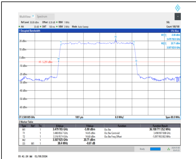
1-N77-3450-3550-30-40-M-2-DFT-PI2BPSK-Outer_F ull-100@0-Ant4-36.101-38.400-≤40-PASS
