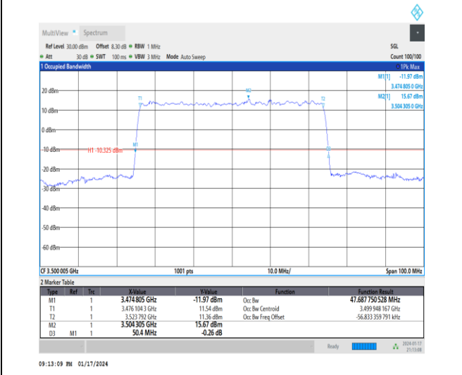
1-N77-3450-3550-30-50-M-8-CP-64QAM-Outer_Full-133@0-Ant4-47.688-50.400-≤50-PASS
