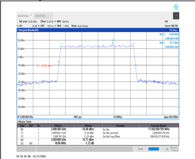
1-N77-3450-3550-30-20-M-4-DFT-64QAM-Outer_Fu II-50@0-Ant4-17.933-18.960-≤20-PASS
