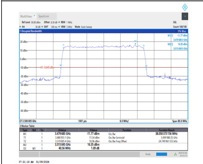
1-N77-3450-3550-30-40-M-8-CP-64QAM-Outer_Full-1 106@0-Ant4-38.05-40.560-≤40-PASS
