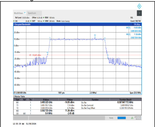
1-N77-3450-3550-30-10-M-6-CP-QPSK-Outer_Full-24@0-Ant4-8.588-9.400-≤10-PASS
