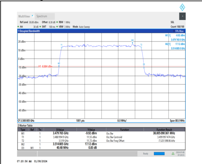
1-N77-3450-3550-30-40-M-7-CP-16QAM-Outer_Full -106@0-Ant4-38.005-40.480-≤40-PASS
