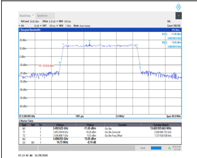
1-N77-3450-3550-30-15-M-6-CP-QPSK-Outer_Full-I-38@0-Ant4-13.604-14.730-≤15-PASS
