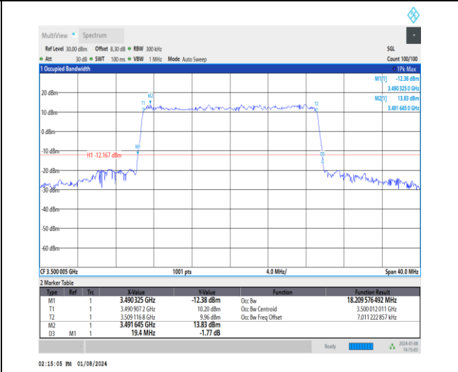
1-N77-3450-3550-30-20-M-6-CP-QPSK-Outer_Full-51@0-Ant4-18.21-19.400-≤20-PASS
