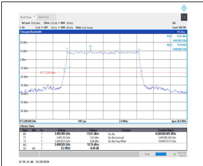
1-N77-3450-3550-30-10-M-5-DFT-256QAM-Outer_Full-24@0-Ant4-8.565-9.200-≤10-PASS
