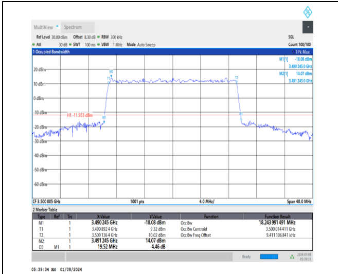
1-N77-3450-3550-30-20-M-7-CP-16QAM-Outer_Full-51@0-Ant4-18.244-19.520-≤20-PASS
