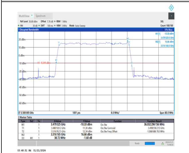
1-N77-3450-3550-30-40-M-4-DFT-64QAM-Outer_Ful l-100@0-Ant4-36.032-38.720-≤40-PASS
