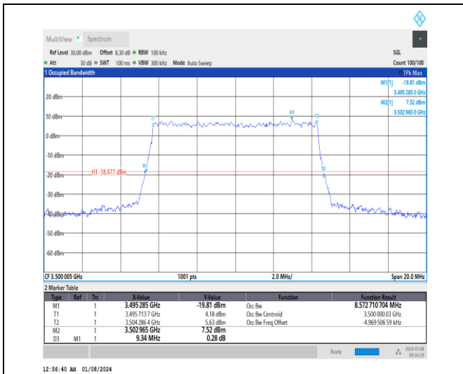
1-N77-3450-3550-30-10-M-9-CP-256QAM-Outer_Ful I-24@0-Ant4-8.573-9.340-≤10-PASS
