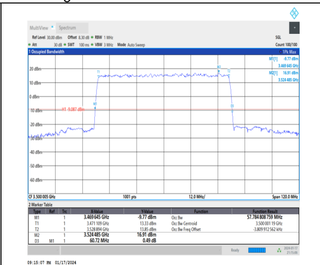
1-N77-3450-3550-30-60-M-1-DFT-QPSK-Outer_Full-162@0-Ant4-57.785-60.720-≤60-PASS
