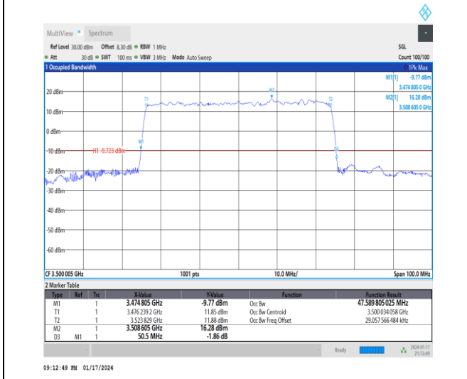
1-N77-3450-3550-30-50-M-7-CP-16QAM-Outer_Full-133@0-Ant4-47.59-50.500-≤50-PASS
