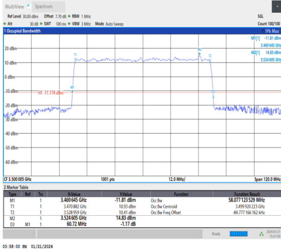
1-N77-3450-3550-30-60-M-8-CP-64QAM-Outer_Full-162@0-Ant4-58.077-60.720-≤60-PASS
