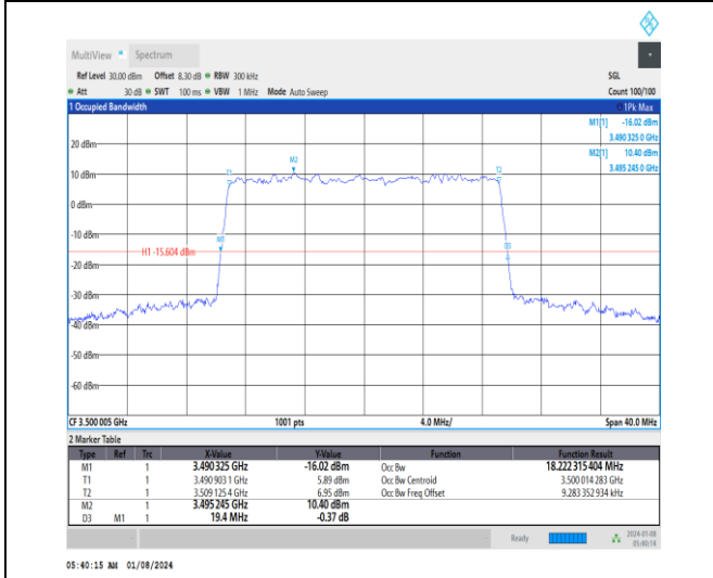
1-N77-3450-3550-30-20-M-9-CP-256QAM-Outer_Ful-I-51@0-Ant4-18.222-19.400-≤20-PASS
