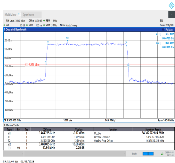
1-N77-3450-3550-30-70-M-2-DFT-PI2BPSK-Outer_Full-180@0-Ant4-64.382-67.340-≤70-PASS
