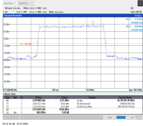
1-N77-3450-3550-30-50-M-2-DFT-PI2BPSK-Outer_Full-128@0-Ant4-45.782-48.600-≤50-PASS
