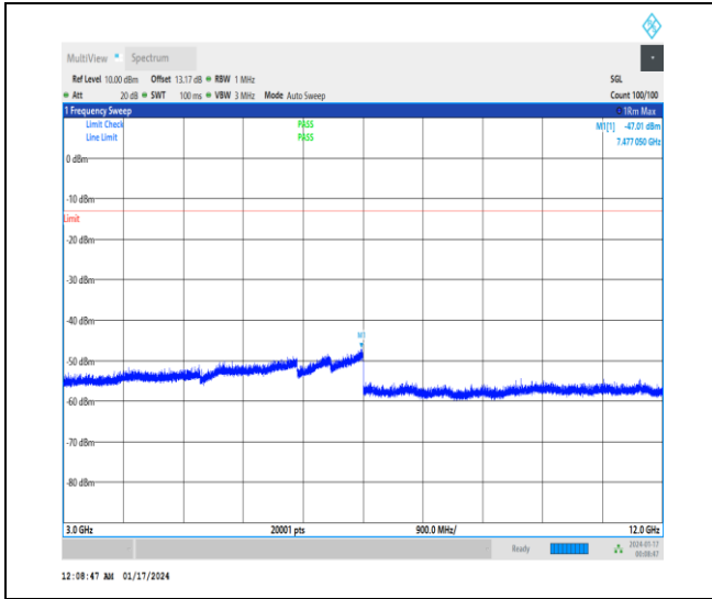
1-N71-15-20-L-1-DFT-PI2BPSK-Inner_1RB_Left-1 @ 1-3000-12000-Ant0-7477.05--47.01--13-PASS
