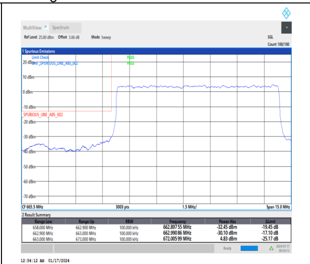
1-N71-15-10-L-3-DFT-PI2BPSK-Outer_Full-50@0-Ant0-1--PASS-see graph
