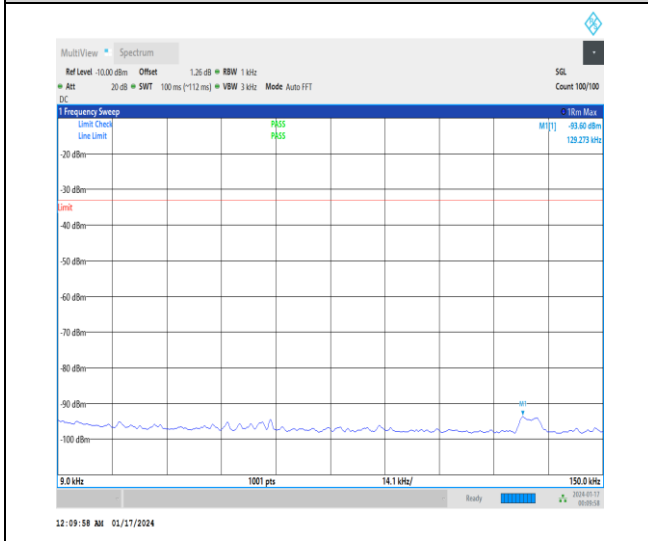
1-N71-15-20-M-1-DFT-PI2BPSK-Inner_1RB_Left-1 @ 1-0.009-0.15-Ant0-0.13--93.60--33-PASS
