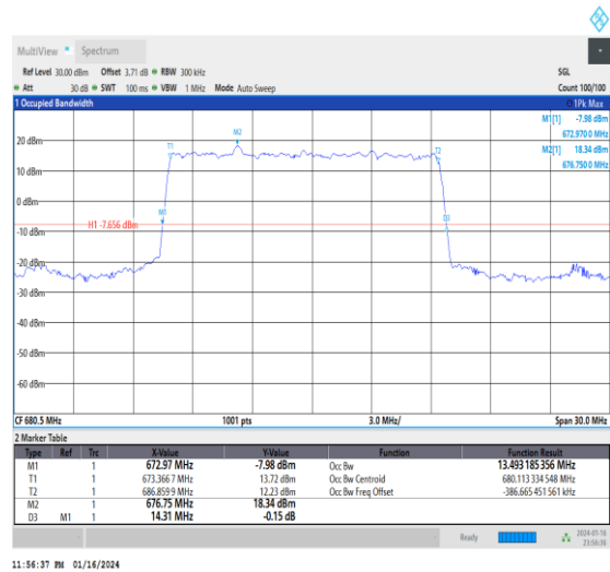
1-N71-15-15-M-2-DFT-PI2BPSK-Outer_Full-75@0-Ant0 -13.493-14.310-≤15-PASS
