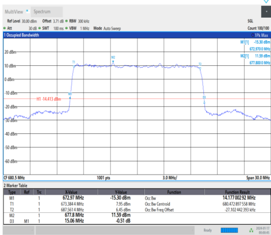
1-N71-15-15-M-9-CP-256QAM-Outer_Full-79@0-Ant0 0-14.177-15.060-≤15-PASS
