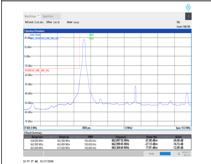
1-N71-15-10-L-4-CP-QPSK-Edge_1RB_Left-1@0-Ant0-1--PASS-see graph
