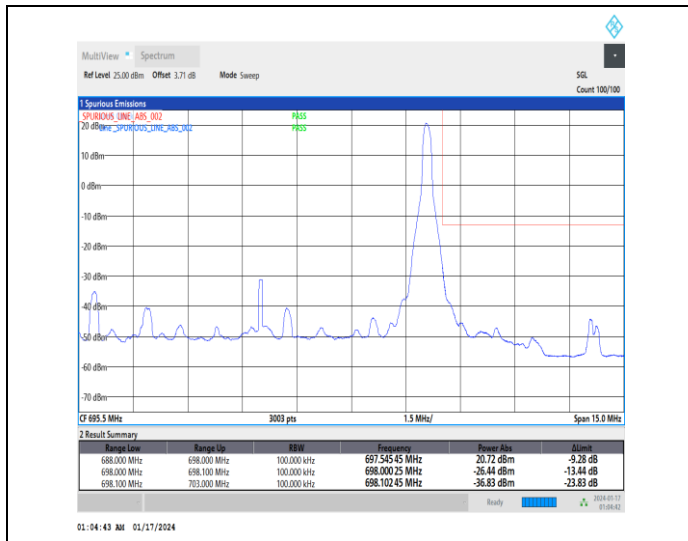
1-N71-15-10-H-2-DFT-PI2BPSK-Edge_1RB_Right-1@51-Ant0-1--PASS-see graph
