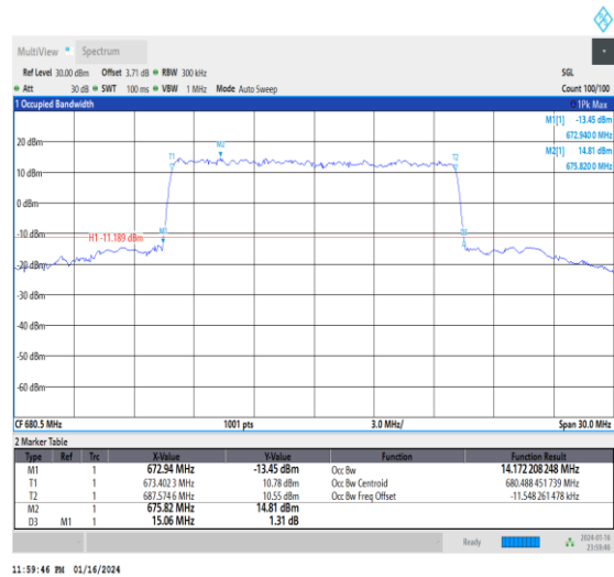
1-N71-15-15-M-6-CP-QPSK-Outer_Full-79@0-Ant0 14.172-15.060-≤15-PASS
