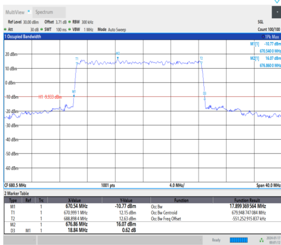
1-N71-15-20-M-1-DFT-QPSK-Outer_Full-100@0-Ant0 0-17.899-18.840-≤20-PASS
