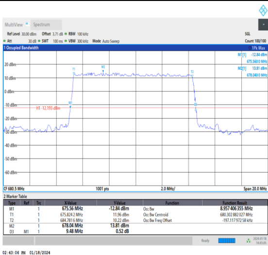
1-N71-15-10-M-2-DFT-PI2BPSK-Outer_Full-50@0-Ant0 -8.957-9.480-≤10-PASS
