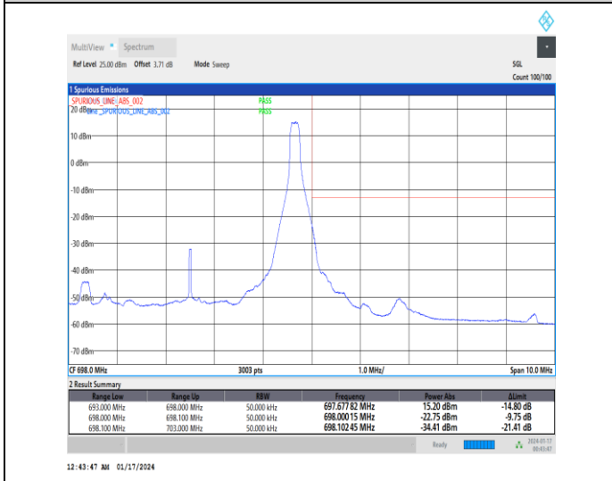
1-N71-15-5-H-5-CP-QPSK-Edge_1RB_Right-1@24-Ant0-1--PASS-see graph
