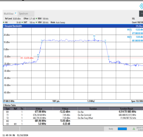
1-N71-15-5-M-6-CP-QPSK-Outer_Full-25@0-Ant0-4 .515-5.000-≤5-PASS
