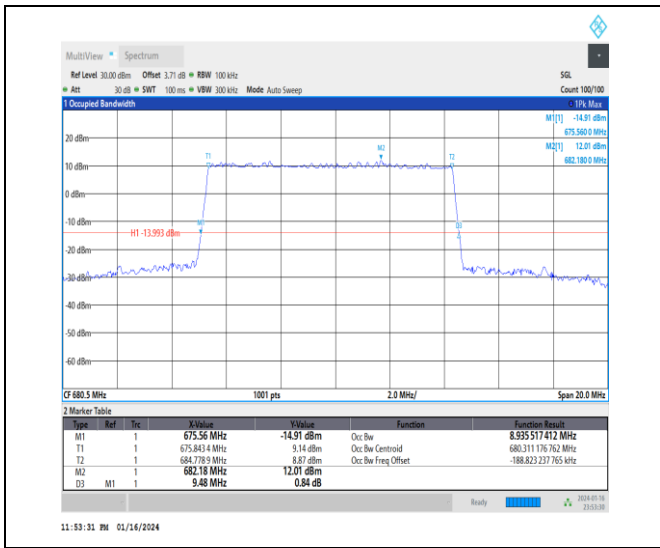
1-N71-15-10-M-4-DFT-64QAM-Outer_Full-50@0-Ant 0-8.936-9.480-≤10-PASS
