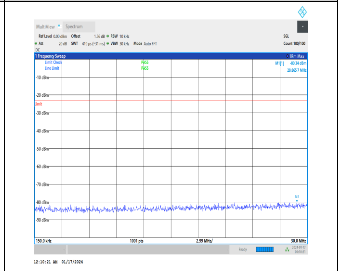
1-N71-15-20-M-1-DFT-PI2BPSK-Inner_1RB_Left-1 @ 1-0.15-30-Ant0-28.87--80.34--23-PASS
