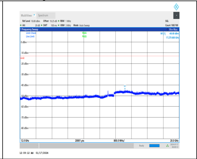
1-N71-15-20-L-1-DFT-PI2BPSK-Inner_1RB_Left-1 @ 1-12000-20000-Ant0-17275.60--44.49--13-PASS
