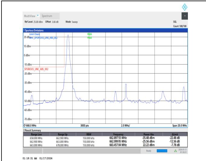
1-N71-15-15-L-1-DFT-PI2BPSK-Edge_1RB_Left-1@0-Ant0-1--PASS-see graph
