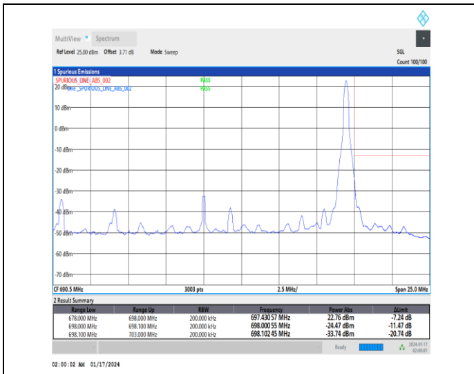
1-N71-15-20-H-2-DFT-PI2BPSK-Edge_1RB_Right-1 @ 105-Ant0-1--PASS-see graph
