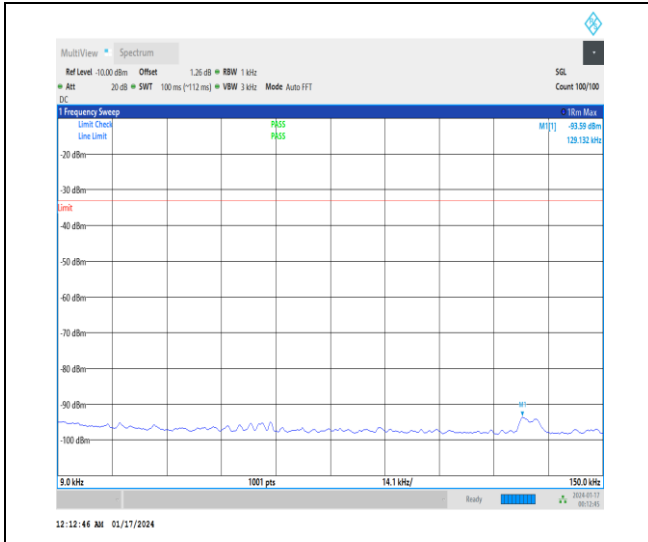
1-N71-15-20-H-1-DFT-PI2BPSK-Inner_1RB_Left-1 @ 1-0.009-0.15-Ant0-0.13--93.59--33-PASS
