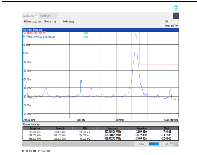
1-N71-15-15-H-2-DFT-PI2BPSK-Edge_1RB_Right-1@78-Ant0-1--PASS-see graph
