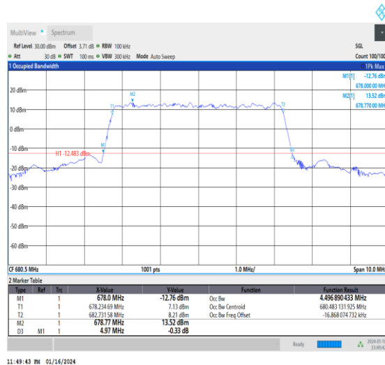
1-N71-15-5-M-8-CP-64QAM-Outer_Full-25@0-Ant0-4 4.497-4.970-≤5-PASS
