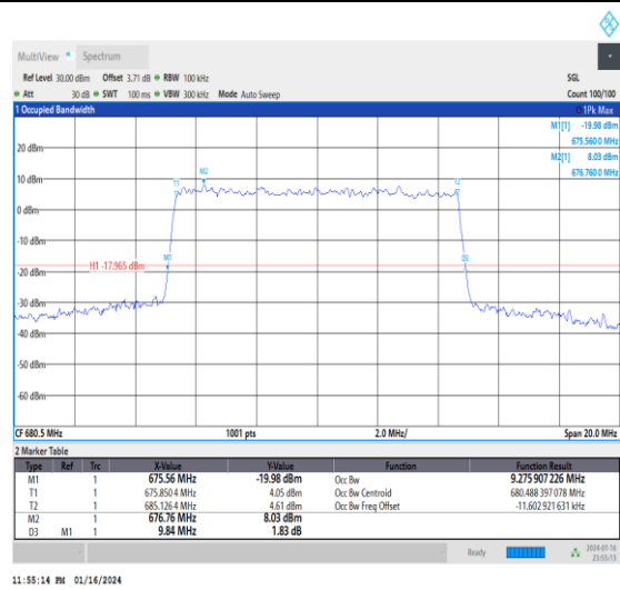
1-N71-15-10-M-9-CP-256QAM-Outer_Full-52@0-Ant0 -9.276-9.840-≤10-PASS
