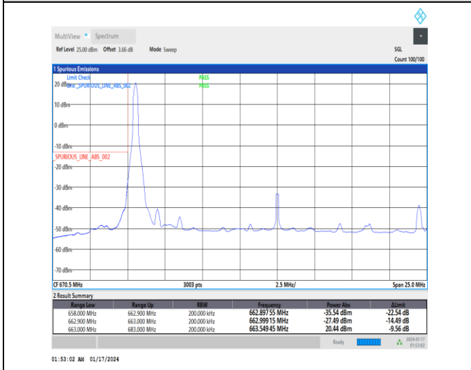
1-N71-15-20-L-4-CP-QPSK-Edge_1RB_Left-1@0-Ant0-1--PASS-see graph
