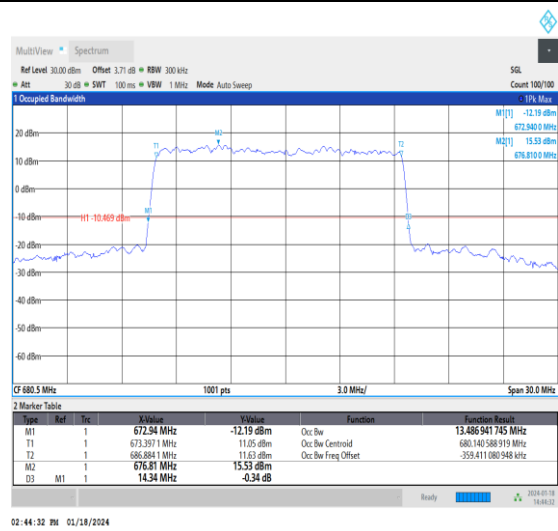
1-N71-15-15-M-4-DFT-64QAM-Outer_Full-75@0-Ant 0-13.487-14.340-≤15-PASS
