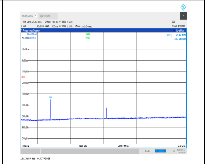
1-N71-15-20-H-1-DFT-PI2BPSK-Inner_1RB_Left-1 @ 1-1000-3000-Ant0-1357.50--36.59--13-PASS
