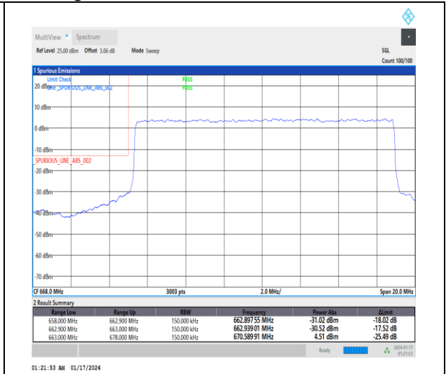
1-N71-15-15-L-3-DFT-PI2BPSK-Outer_Full-75@0-Ant0-1--PASS-see graph
