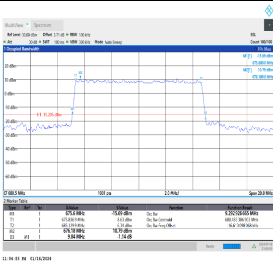
1-N71-15-10-M-8-CP-64QAM-Outer_Full-52@0-Ant0 -9.293-9.840-≤10-PASS
