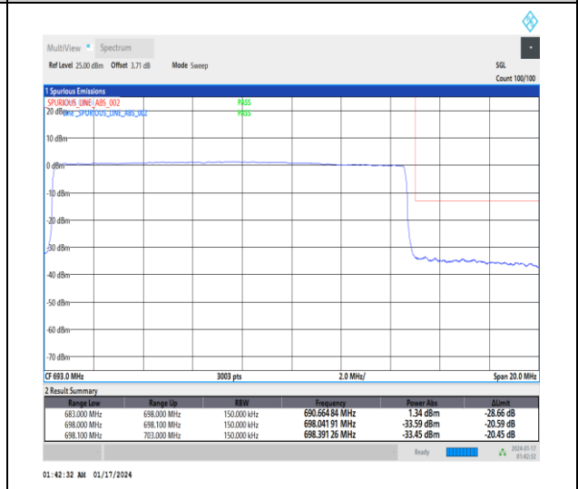
1-N71-15-15-H-6-CP-QPSK-Outer_Full-79@0-Ant0-1--PASS-see graph
