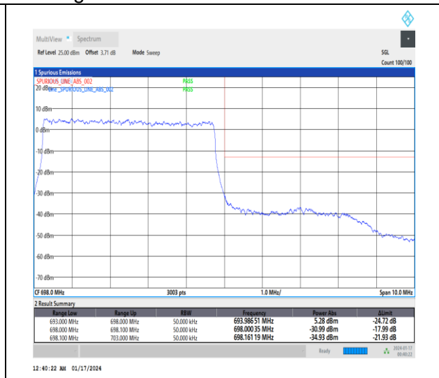
1-N71-15-5-H-3-DFT-PI2BPSK-Outer_Full-25@0-Ant0-1--PASS-see graph
