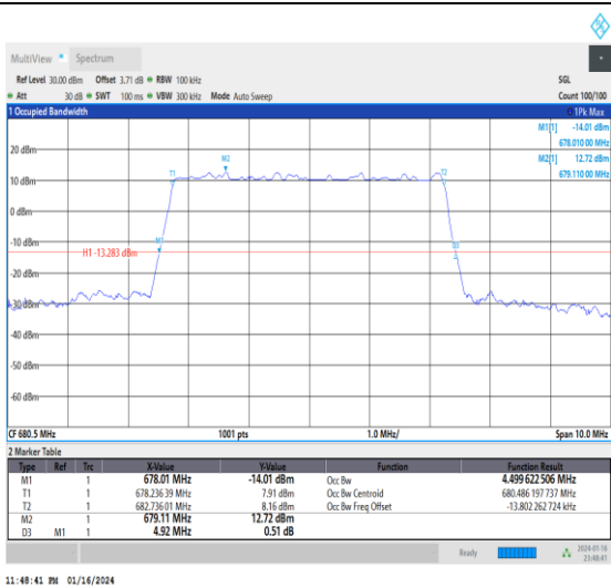
1-N71-15-5-M-5-DFT-256QAM-Outer_Full-25@0-Ant 0-4.5-4.920-≤5-PASS
