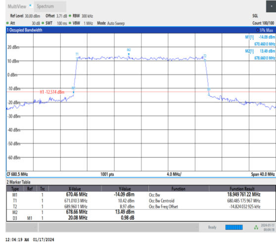
1-N71-15-20-M-7-CP-16QAM-Outer_Full-106@0-Ant0 t0-18.95-20.080-≤20-PASS
