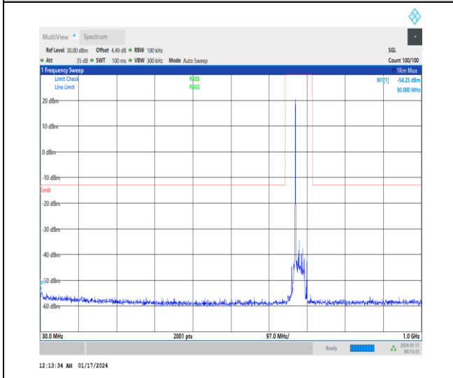
1-N71-15-20-H-1-DFT-PI2BPSK-Inner_1RB_Left-1 @ 1-30-1000-Ant0-30.00--54.25--13-PASS
