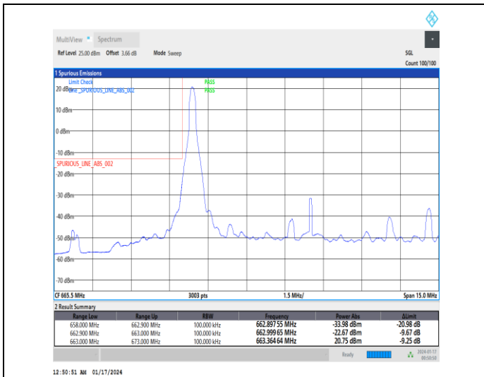
1-N71-15-10-L-1-DFT-PI2BPSK-Edge_1RB_Left-1@0-Ant0-1--PASS-see graph
