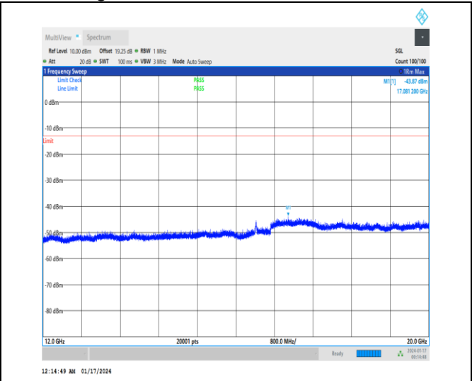
1-N71-15-20-H-1-DFT-PI2BPSK-Inner_1RB_Left-1 @ 1-12000-20000-Ant0-17081.20--43.87--13-PASS
