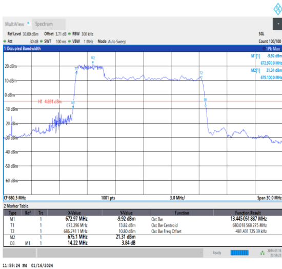
1-N71-15-15-M-5-DFT-256QAM-Outer_Full-75@0-A nt0-13.445-14.220-≤15-PASS
