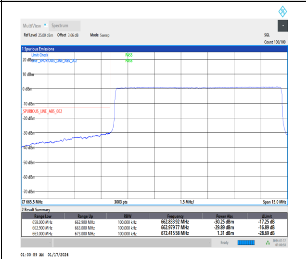
1-N71-15-10-L-6-CP-QPSK-Outer_Full-52@0-Ant0-1--PASS-see graph
