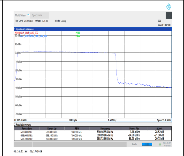
1-N71-15-10-H-6-CP-QPSK-Outer_Full-52@0-Ant0-1--PASS-see graph
