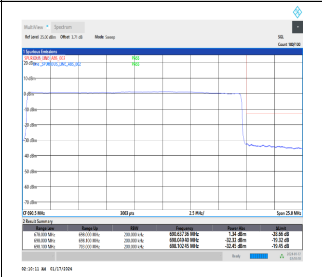
1-N71-15-20-H-6-CP-QPSK-Outer_Full-106@0-Ant0-1--PASS-see graph
