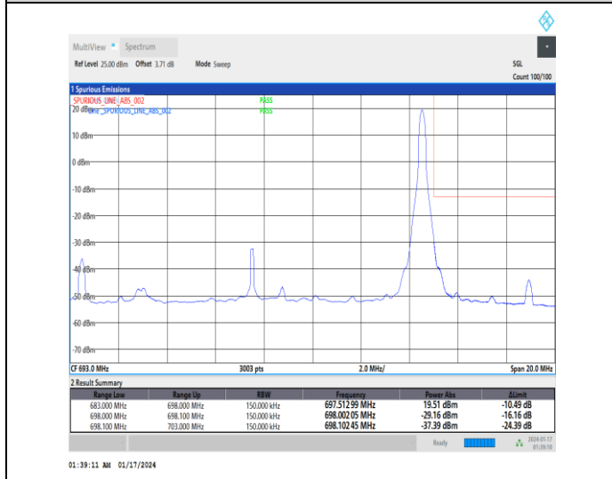
1-N71-15-15-H-5-CP-QPSK-Edge_1RB_Right-1@78-Ant0-1--PASS-see graph
