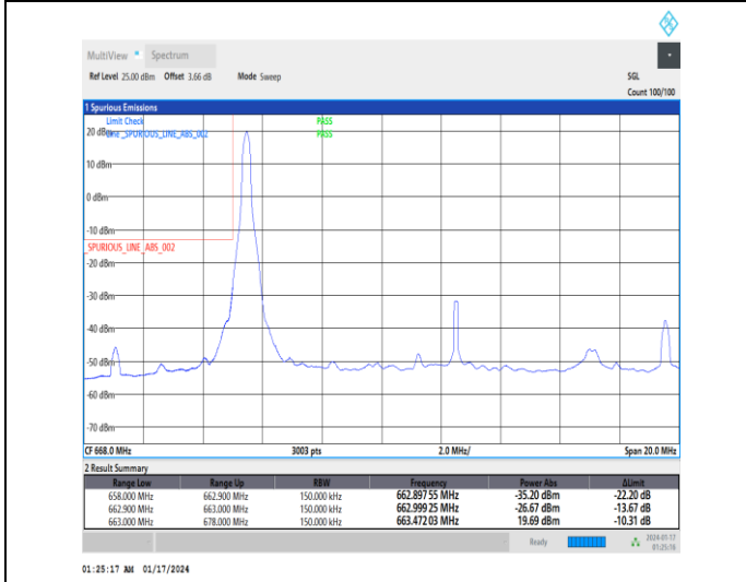
1-N71-15-15-L-4-CP-QPSK-Edge_1RB_Left-1@0-Ant0-1--PASS-see graph
