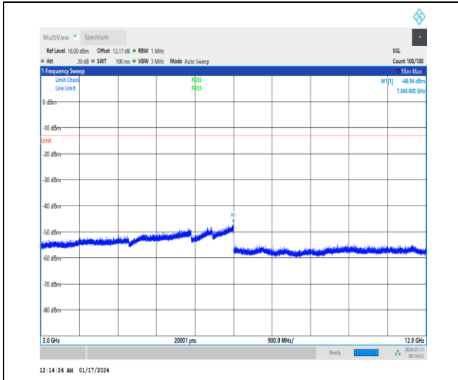
1-N71-15-20-H-1-DFT-PI2BPSK-Inner_1RB_Left-1 @ 1-3000-12000-Ant0-7494.60--46.94--13-PASS
