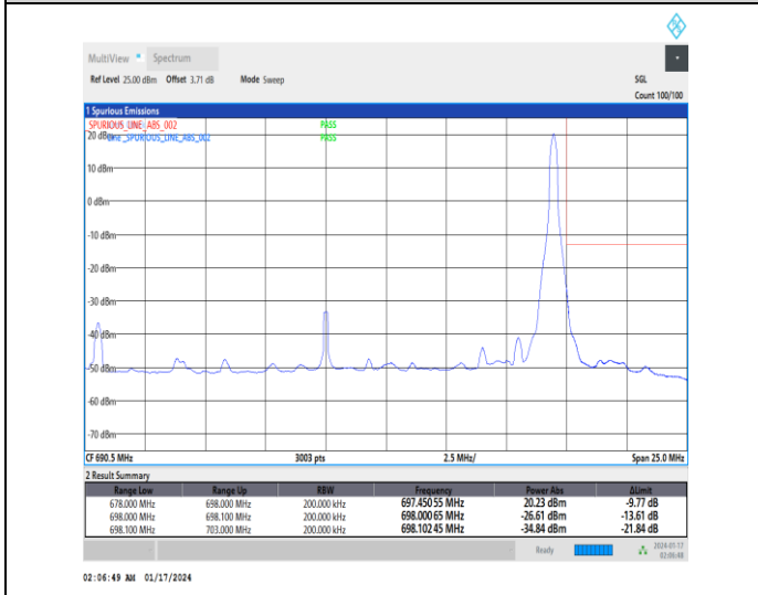
1-N71-15-20-H-5-CP-QPSK-Edge_1RB_Right-1 @ 105-Ant0-1--PASS-see graph
