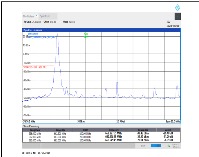
1-N71-15-20-L-1-DFT-PI2BPSK-Edge_1RB_Left-1@0-Ant0-1--PASS-see graph
