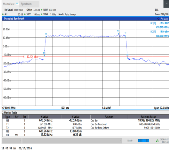
1-N71-15-20-M-6-CP-QPSK-Outer_Full-106@0-Ant0 -18.982-19.920-≤20-PASS
