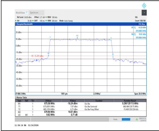
1-N71-15-10-M-6-CP-QPSK-Outer_Full-52@0-Ant0- 9.29-9.820-≤10-PASS
