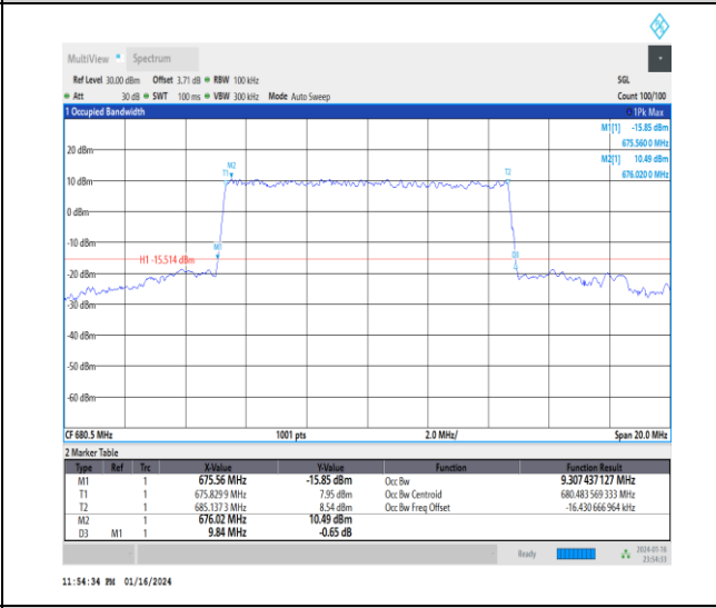
1-N71-15-10-M-7-CP-16QAM-Outer_Full-52@0-Ant 0-9.307-9.840-≤10-PASS
