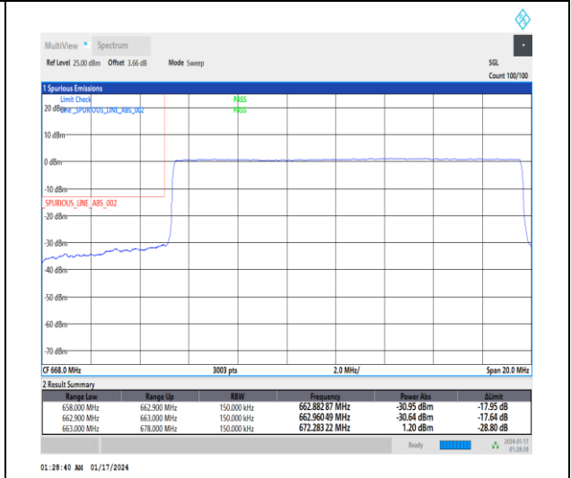
1-N71-15-15-L-6-CP-QPSK-Outer_Full-79@0-Ant0-1--PASS-see graph
