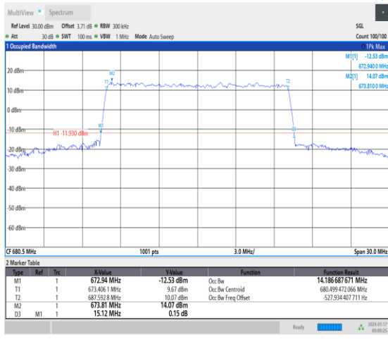
1-N71-15-15-M-8-CP-64QAM-Outer_Full-79@0-Ant0 0-14.187-15.120-≤15-PASS
