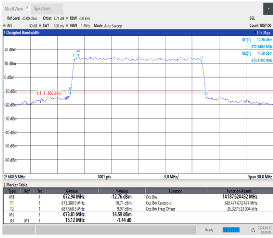
1-N71-15-15-M-7-CP-16QAM-Outer_Full-79@0-Ant0 -14.188-15.120-≤15-PASS
