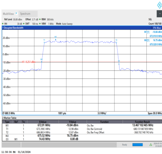
1-N71-15-15-M-1-DFT-QPSK-Outer_Full-75@0-Ant0 -13.467-14.430-≤15-PASS
