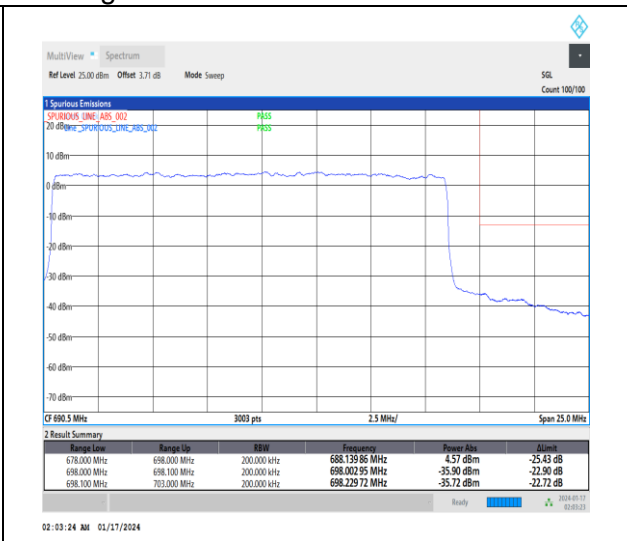
1-N71-15-20-H-3-DFT-PI2BPSK-Outer_Full-100@ 0-Ant0-1--PASS-see graph
