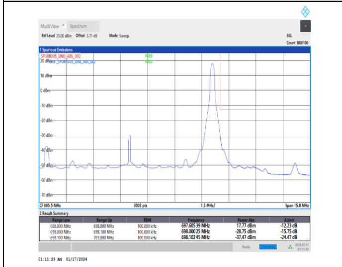
1-N71-15-10-H-5-CP-QPSK-Edge_1RB_Right-1@51-Ant0-1--PASS-see graph
