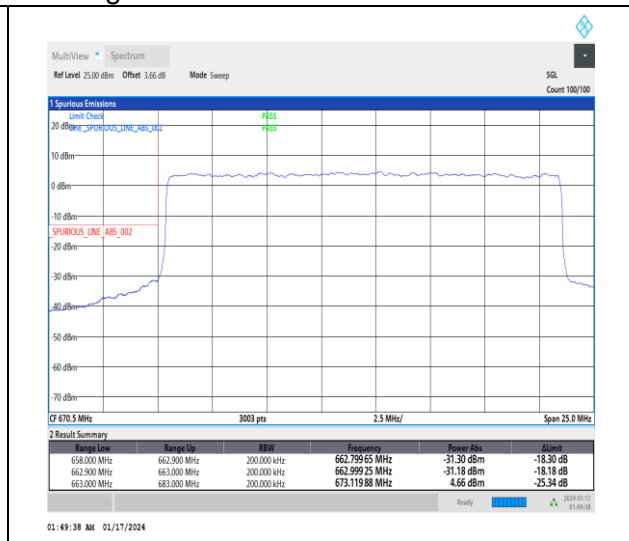
1-N71-15-20-L-3-DFT-PI2BPSK-Outer_Full-100@0-Ant0-1--PASS-see graph
