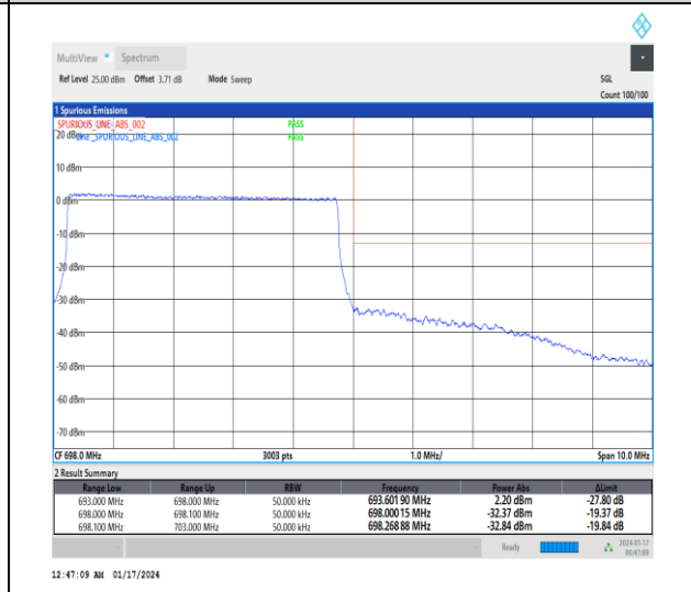
1-N71-15-5-H-6-CP-QPSK-Outer_Full-25@0-Ant0-1--PASS-see graph
