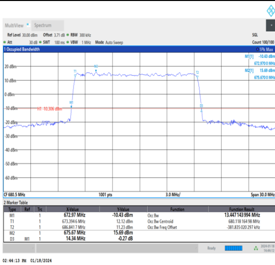
1-N71-15-15-M-3-DFT-16QAM-Outer_Full-75@0-Ant 0-13.447-14.340-≤15-PASS
