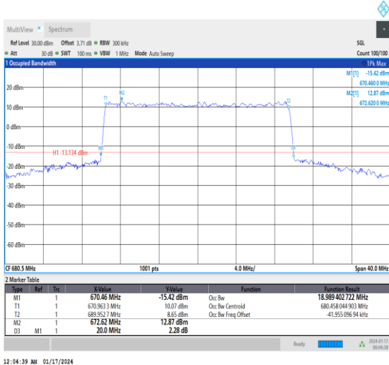
1-N71-15-20-M-8-CP-64QAM-Outer_Full-106@0-Ant0 0-18.989-20.000-≤20-PASS
