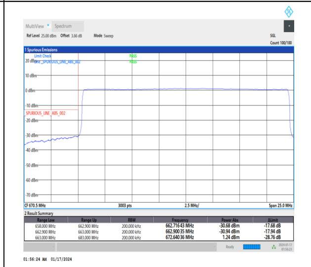
1-N71-15-20-L-6-CP-QPSK-Outer_Full-106@0-Ant0-1--PASS-see graph
