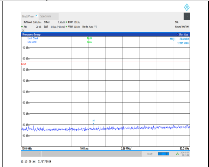
1-N71-15-20-H-1-DFT-PI2BPSK-Inner_1RB_Left-1 @ 1-0.15-30-Ant0-12.99--79.82--23-PASS
