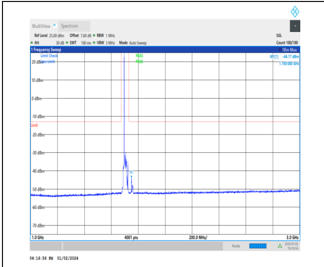
1-N70-15-15-M-1-DFT-PI2BPSK-Inner_1RB_Left-1 @ 1-1000-3000-Ant3-1750.00--44.17--13-PASS
