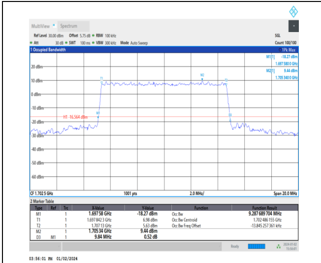
1-N70-15-10-M-8-CP-64QAM-Outer_Full-52@0-Ant 3-9.288-9.840-≤10-PASS
