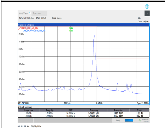
1-N70-15-15-H-5-CP-QPSK-Edge_1RB_Right-1@78-Ant3-1-seegraph-PASS-see graph
