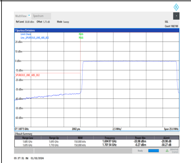
1-N70-15-15-L-6-CP-QPSK-Outer_Full-79@0-Ant3-1-seegraph-PASS-see graph
