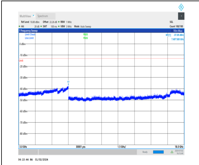
1-N70-15-15-L-1-DFT-PI2BPSK-Inner_1RB_Left-1 @ 1-3000-18000-Ant3-7497.50--37.09--13-PASS
