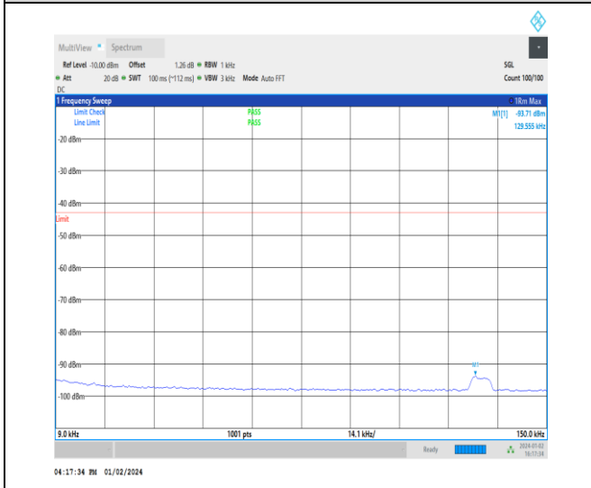
1-N70-15-15-H-1-DFT-PI2BPSK-Inner_1RB_Left-1 @ 1-0.009-0.15-Ant3-0.13--93.71--43-PASS
