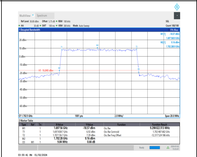
1-N70-15-10-M-7-CP-16QAM-Outer_Full-52@0-Ant3 -9.298-9.840-≤10-PASS
