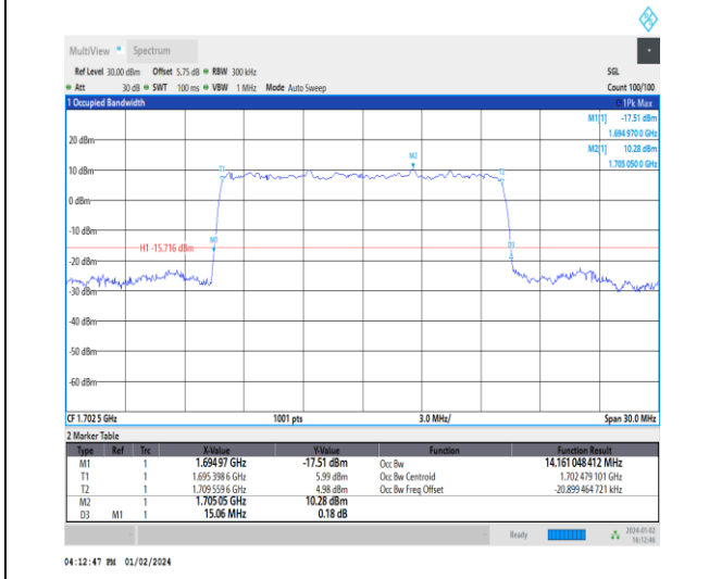
1-N70-15-15-M-9-CP-256QAM-Outer_Full-79@0-An t3-14.161-15.060≤15-PASS
