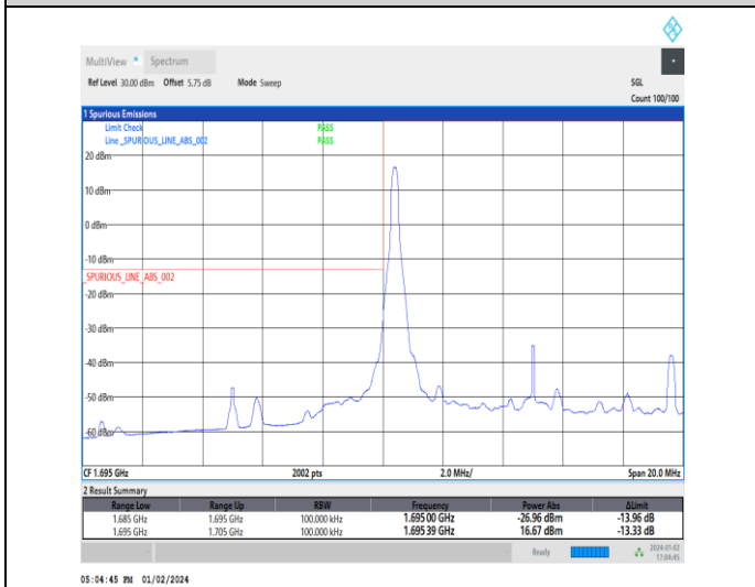
1-N70-15-10-L-4-CP-QPSK-Edge_1RB_Left-1@0-Ant3-1-seegraph-PASS-see graph
