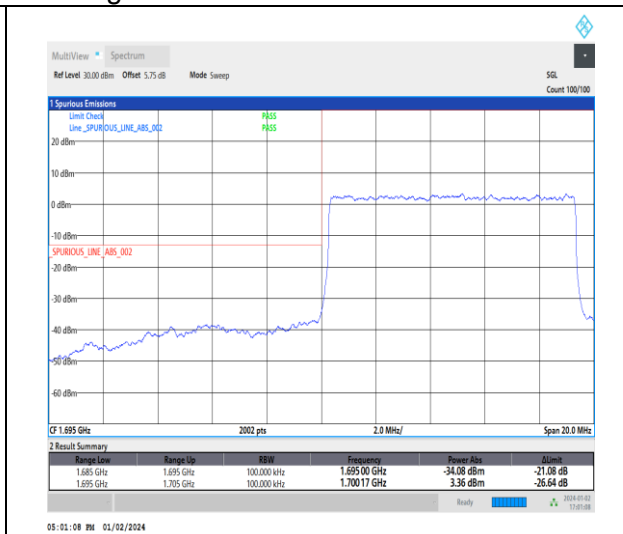
1-N70-15-10-L-3-DFT-PI2BPSK-Outer_Full-50@0-Ant3-1-seegraph-PASS-see graph
