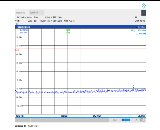
1-N70-15-15-H-1-DFT-PI2BPSK-Inner_1RB_Left-1 @ 1-0.15-30-Ant3-27.10--80.01--33-PASS
