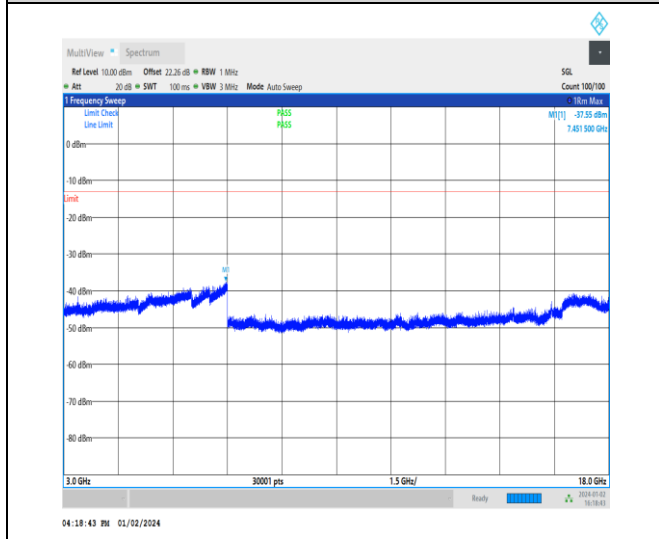
1-N70-15-15-H-1-DFT-PI2BPSK-Inner_1RB_Left-1 @ 1-3000-18000-Ant3-7451.50--37.55--13-PASS
