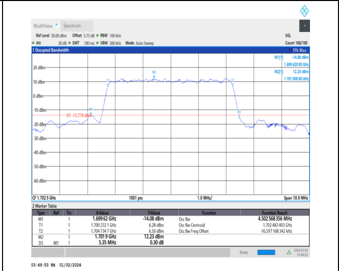
1-N70-15-5-M-8-CP-64QAM-Outer_Full-25@0-Ant3- 4.503-5.350-≤5-PASS
