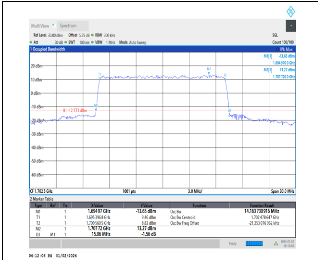
1-N70-15-15-M-7-CP-16QAM-Outer_Full-79@0-Ant 3-14.164-15.060≤15-PASS
