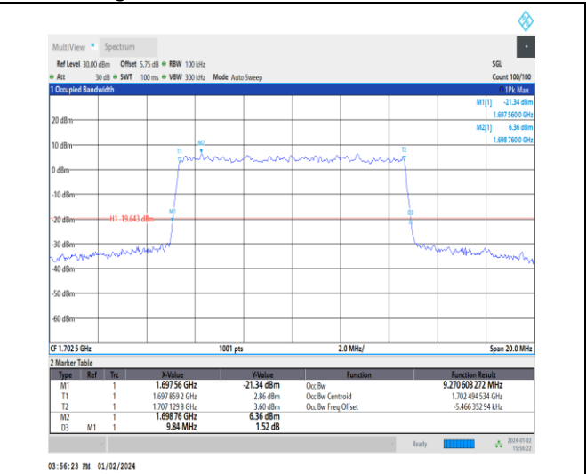
1-N70-15-10-M-9-CP-256QAM-Outer_Full-52@0-Ant 3-9.271-9.840-≤10-PASS
