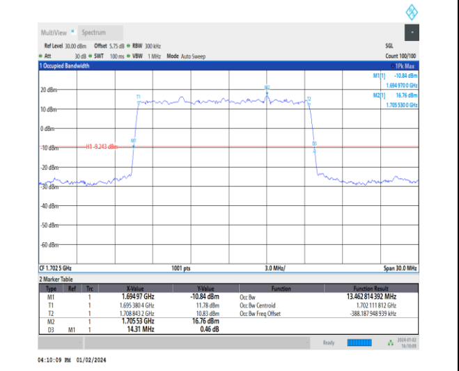
1-N70-15-15-M-2-DFT-PI2BPSK-Outer_Full-75@0-Ant3 -13.463-14.310-≤15-PASS
