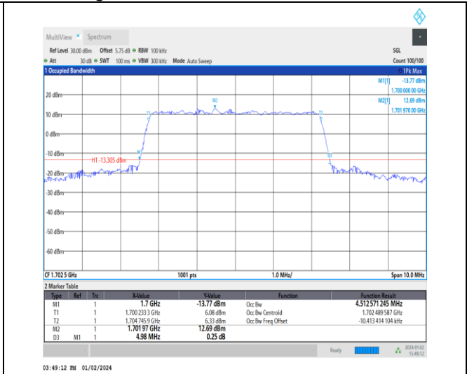
1-N70-15-5-M-6-CP-QPSK-Outer_Full-25@0-Ant3-4. 513-4.980-≤5-PASS
