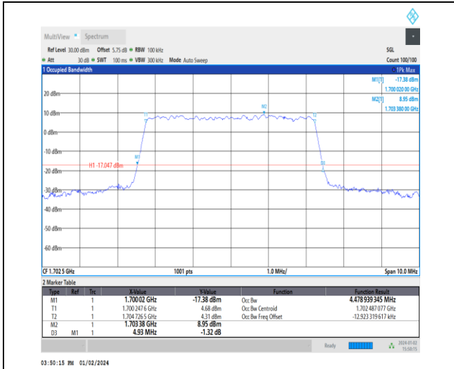
1-N70-15-5-M-9-CP-256QAM-Outer_Full-25@0-Ant 3-4.479-4.930-≤5-PASS
