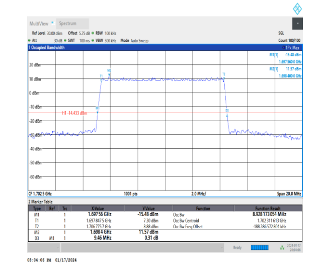
1-N70-15-10-M-3-DFT-16QAM-Outer_Full-50@0-Ant 3-8.928-9.460-≤10-PASS
