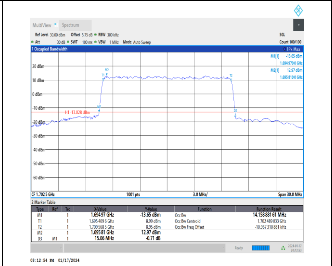
1-N70-15-15-M-6-CP-QPSK-Outer_Full-79@0-Ant3 14.159-15.060-≤15-PASS
