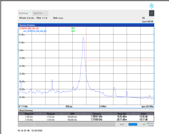
1-N70-15-10-H-5-CP-QPSK-Edge_1RB_Right-1@51-Ant3-1-seegraph-PASS-see graph
