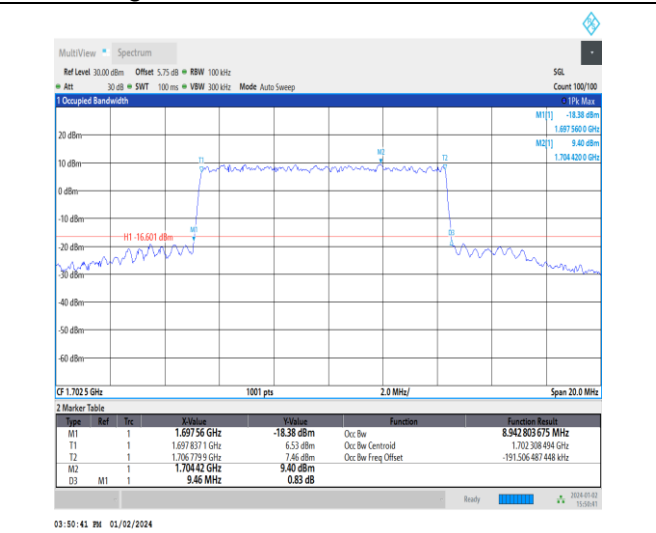
1-N70-15-10-M-1-DFT-QPSK-Outer_Full-50@0-Ant3 -8.943-9.460-≤10-PASS
