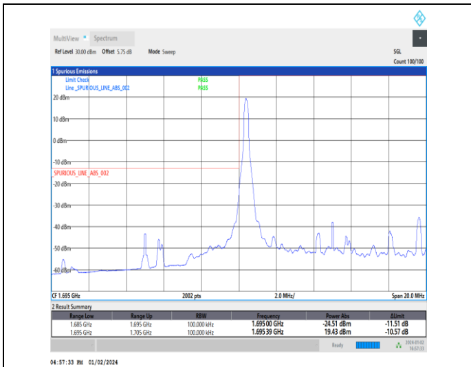
1-N70-15-10-L-1-DFT-PI2BPSK-Edge_1RB_Left-1@0-Ant3-1-seegraph-PASS-see graph
