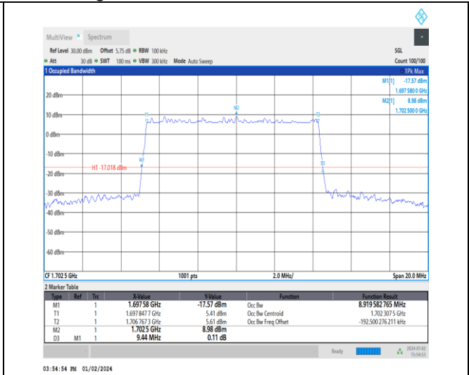
1-N70-15-10-M-5-DFT-256QAM-Outer_Full-50@0-A nt3-8.92-9.440-≤10-PASS
