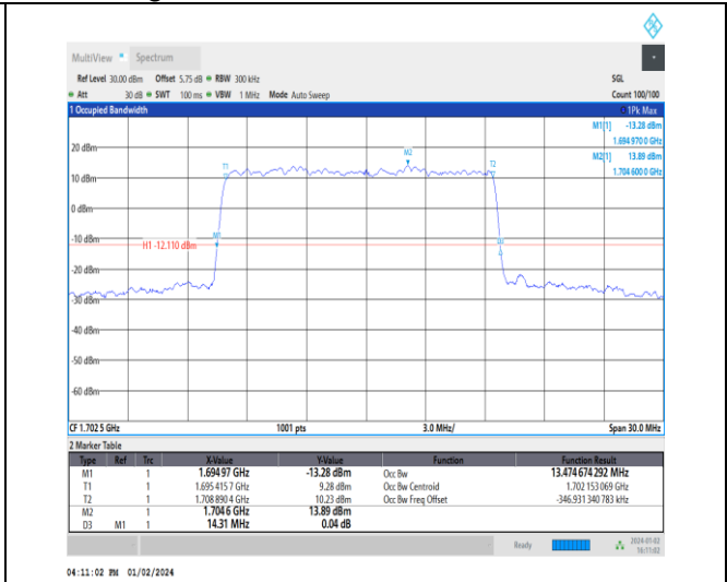
1-N70-15-15-M-4-DFT-64QAM-Outer_Full-75@0-Ant 3-13.475-14.310-≤15-PASS
