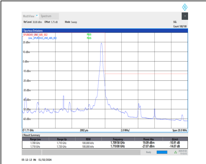
1-N70-15-10-H-2-DFT-PI2BPSK-Edge_1RB_Right-1@51-Ant3-1-seegraph-PASS-see graph
