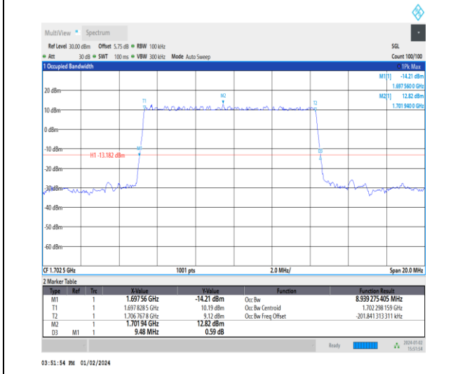
1-N70-15-10-M-2-DFT-PI2BPSK-Outer_Full-50@0-A nt3-8.939-9.480-≤10-PASS
