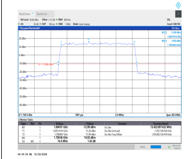
1-N70-15-15-M-1-DFT-QPSK-Outer_Full-75@0-Ant3 -13.452-14.400-≤15-PASS
