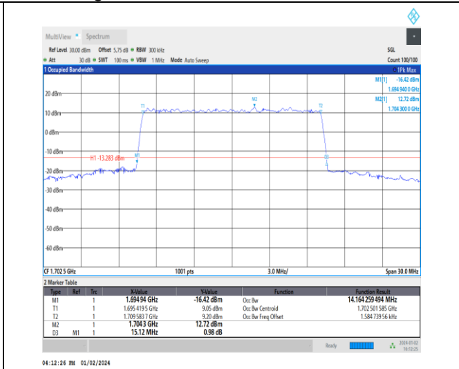
1-N70-15-15-M-8-CP-64QAM-Outer_Full-79@0-Ant3 -14.164-15.120≤15-PASS
