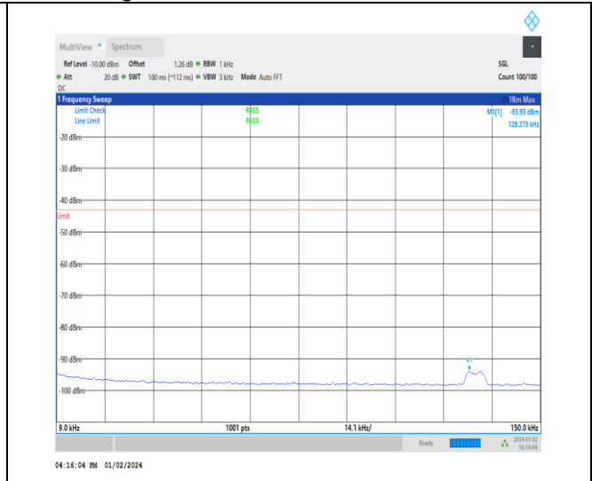
1-N70-15-15-M-1-DFT-PI2BPSK-Inner_1RB_Left-1 @ 1-0.009-0.15-Ant3-0.13--93.93--43-PASS
