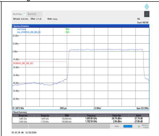
1-N70-15-15-L-3-DFT-PI2BPSK-Outer_Full-75@0-Ant3-1-seegraph-PASS-see graph
