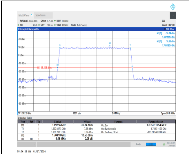
1-N70-15-10-M-4-DFT-64QAM-Outer_Full-50@0-Ant 3-8.935-9.480-≤10-PASS
