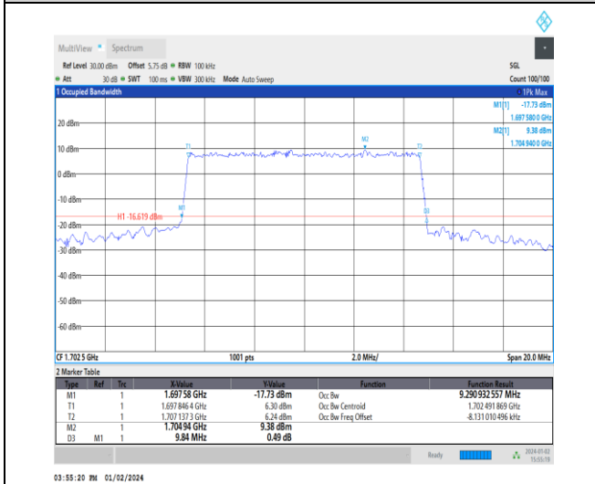
1-N70-15-10-M-6-CP-QPSK-Outer_Full-52@0-Ant3 9.291-9.840-≤10-PASS
