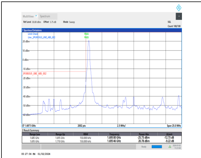
1-N70-15-15-L-1-DFT-PI2BPSK-Edge_1RB_Left-1@0-Ant3-1-seegraph-PASS-see graph
