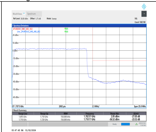
1-N70-15-15-H-3-DFT-PI2BPSK-Outer_Full-75@0-Ant3-1-seegraph-PASS-see graph
