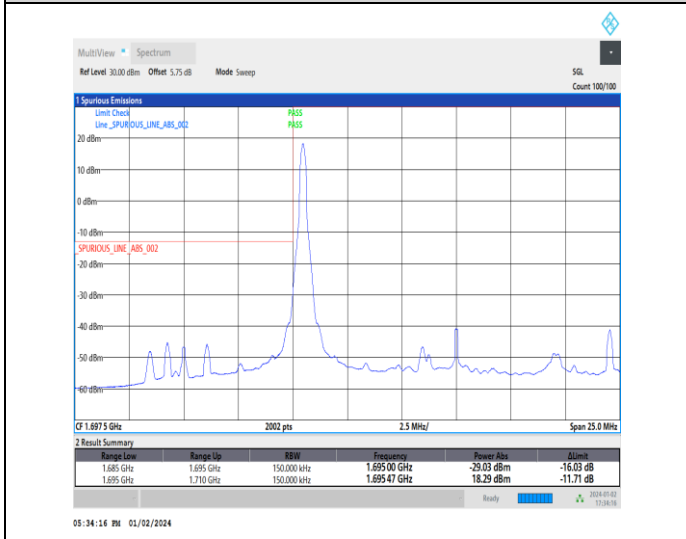
1-N70-15-15-L-4-CP-QPSK-Edge_1RB_Left-1@0-Ant3-1-seegraph-PASS-see graph
