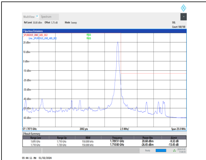
1-N70-15-15-H-2-DFT-PI2BPSK-Edge_1RB_Right-1@78-Ant3-1-seegraph-PASS-see graph
