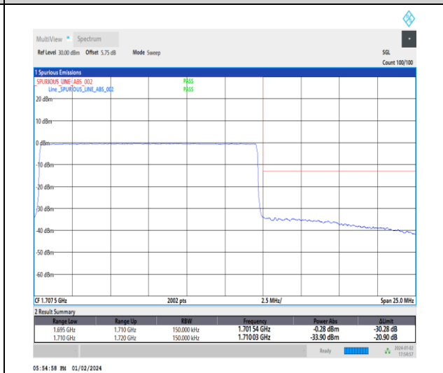
1-N70-15-15-H-6-CP-QPSK-Outer_Full-79@0-Ant3-1-seegraph-PASS-see graph
