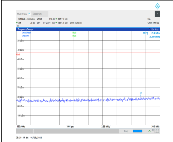
1-N70-15-15-M-1-DFT-PI2BPSK-Inner_1RB_Left-1 @ 1-0.15-30-Ant3-26.00--79.41--33-PASS
