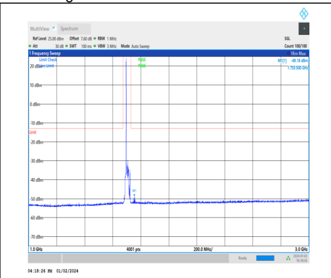
1-N70-15-15-H-1-DFT-PI2BPSK-Inner_1RB_Left-1 @ 1-1000-3000-Ant3-1753.50--49.18--13-PASS
