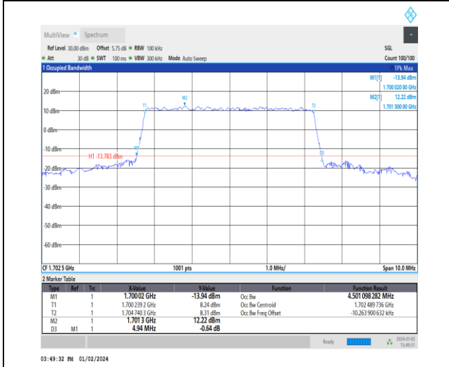
1-N70-15-5-M-7-CP-16QAM-Outer_Full-25@0-Ant3- 4.501-4.940-≤5-PASS
