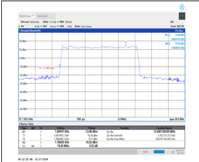
1-N70-15-15-M-3-DFT-16QAM-Outer_Full-75@0-Ant 3-13.438-14.340-≤15-PASS
