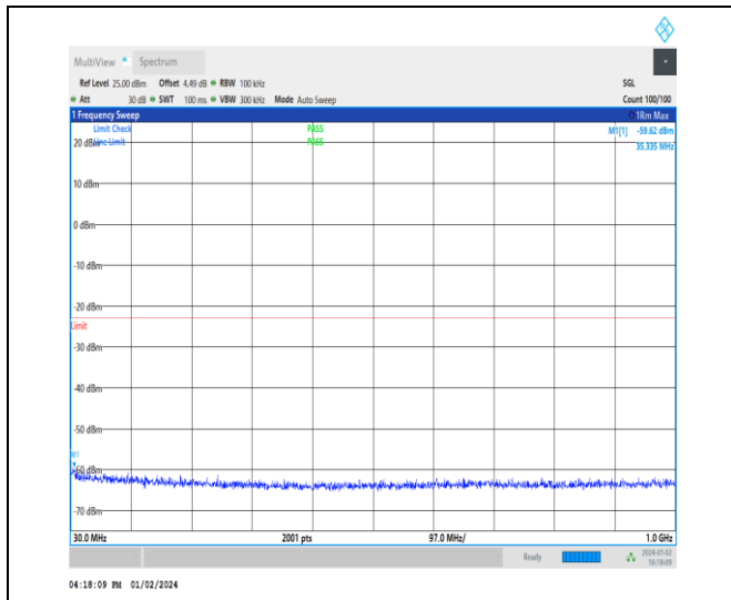
1-N70-15-15-H-1-DFT-PI2BPSK-Inner_1RB_Left-1 @ 1-30-1000-Ant3-35.34--59.62--23-PASS
