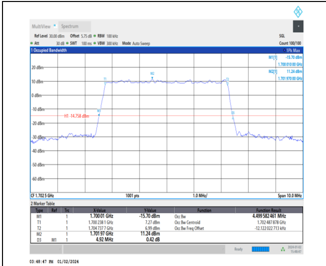
1-N70-15-5-M-5-DFT-256QAM-Outer_Full-25@0-Ant 3-4.5-4.920-≤5-PASS
