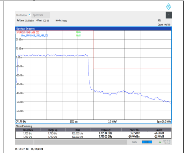
1-N70-15-10-H-3-DFT-PI2BPSK-Outer_Full-50@0-Ant3-1-seegraph-PASS-see graph
