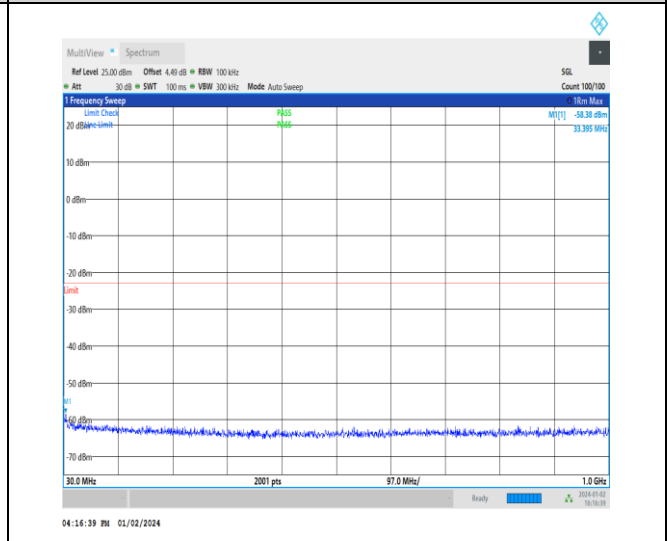
1-N70-15-15-M-1-DFT-PI2BPSK-Inner_1RB_Left-1 @ 1-30-1000-Ant3-33.40--58.38--23-PASS
