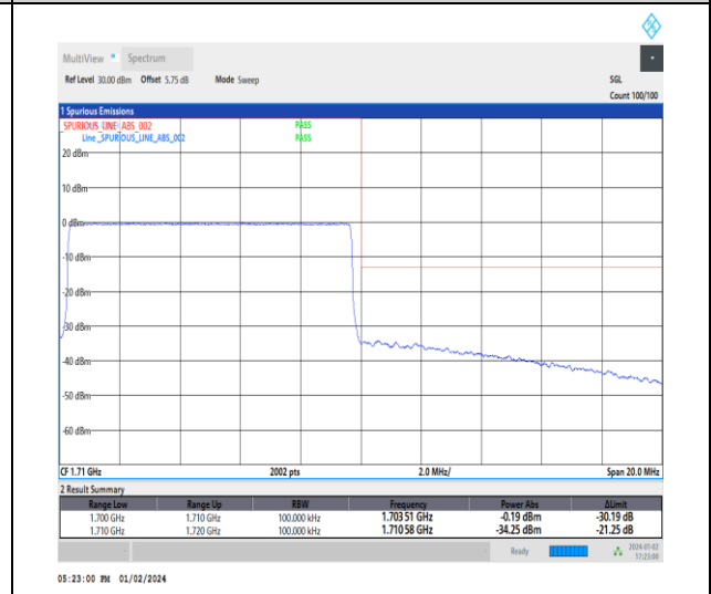
1-N70-15-10-H-6-CP-QPSK-Outer_Full-52@0-Ant3-1-seegraph-PASS-see graph
