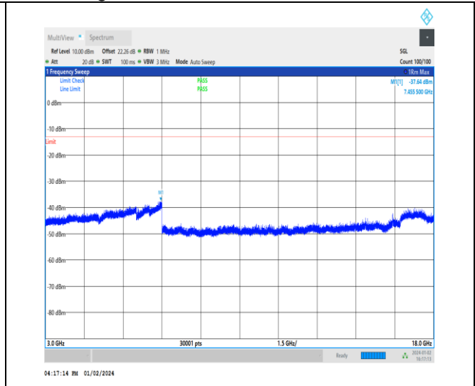
1-N70-15-15-M-1-DFT-PI2BPSK-Inner_1RB_Left-1 @ 1-3000-18000-Ant3-7455.50--37.64--13-PASS
