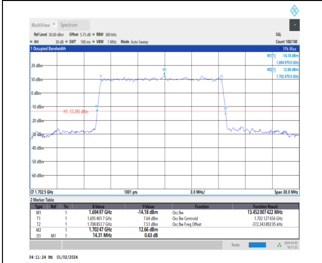
1-N70-15-15-M-5-DFT-256QAM-Outer_Full-75@0-A nt3-13.452-14.310-≤15-PASS
