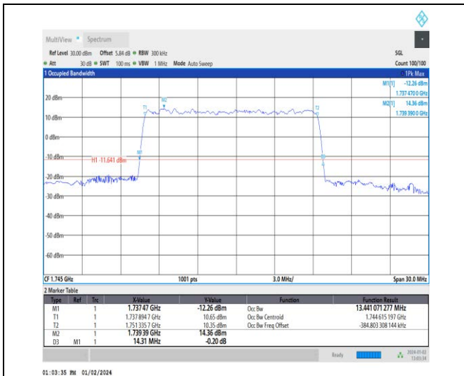
1-N66-15-15-M-3-DFT-16QAM-Outer_Full-75@0-Ant 3-13.441-14.310-≤15-PASS
