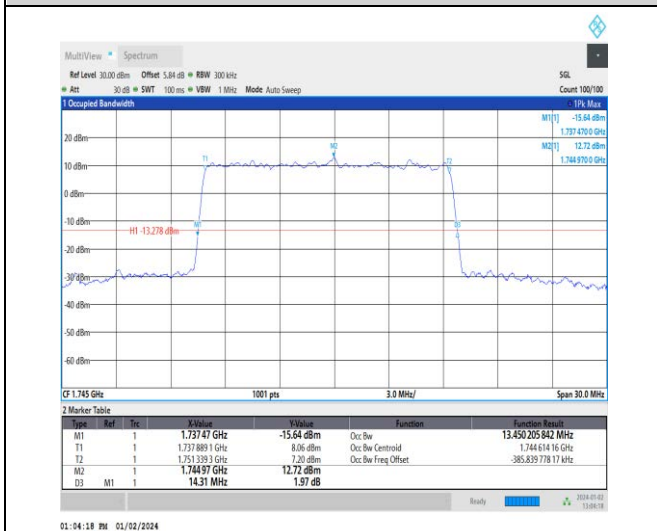
1-N66-15-15-M-5-DFT-256QAM-Outer_Full-75@0-A nt3-13.45-14.310-≤15-PASS
