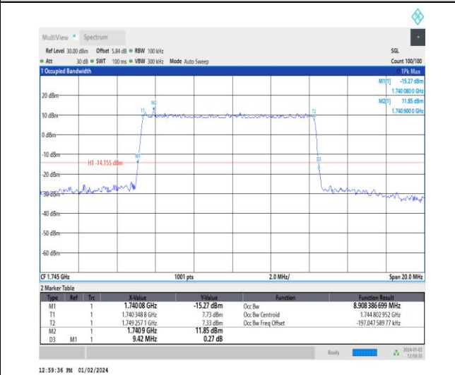
1-N66-15-10-M-3-DFT-16QAM-Outer_Full-50@0-Ant3 3-8.908-9.420-≤10-PASS
