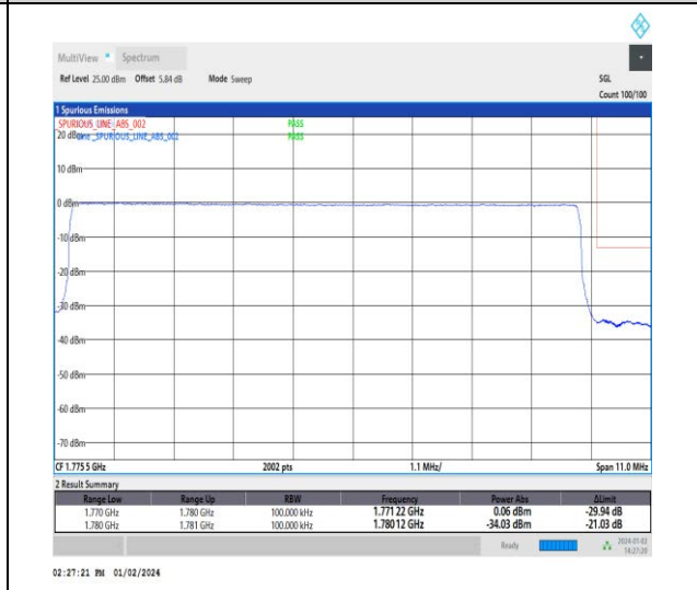
1-N66-15-10-H-6-CP-QPSK-Outer_Full-52@0-Ant3-1-seegraph-PASS-see graph
