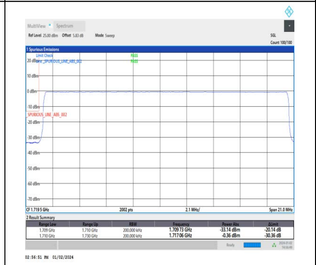
1-N66-15-20-L-6-CP-QPSK-Outer_Full-106@0-Ant3-1-seegraph-PASS-see graph
