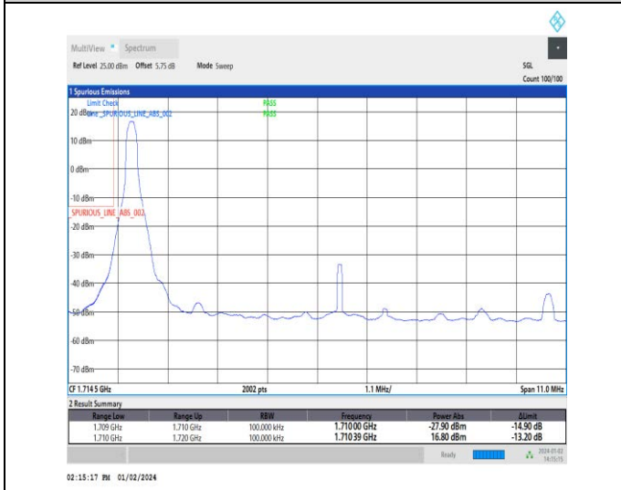
1-N66-15-10-L-4-CP-QPSK-Edge_1RB_Left-1@0-Ant3-1-seegraph-PASS-see graph
