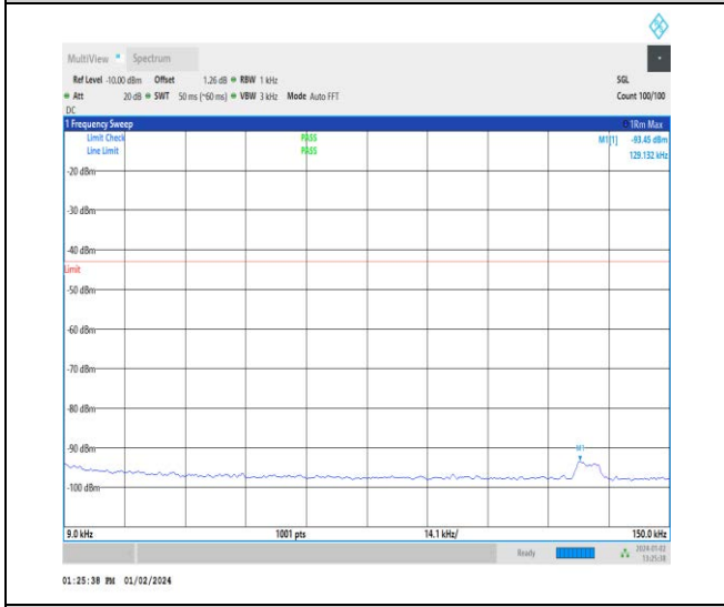
1-N66-15-40-M-1-DFT-PI2BPSK-Inner_1RB_Left-1 @ 1-0.009-0.15-Ant3-0.13--93.45--43-PASS
