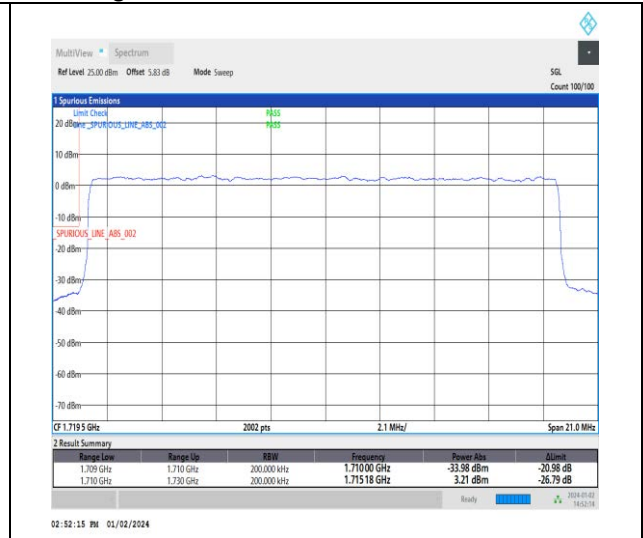
1-N66-15-20-L-3-DFT-PI2BPSK-Outer_Full-100@0-Ant3-1-seegraph-PASS-see graph
