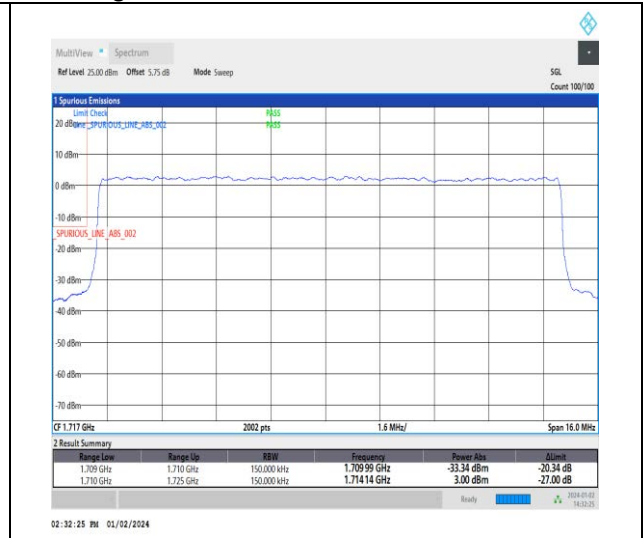
1-N66-15-15-L-3-DFT-PI2BPSK-Outer_Full-75@0-Ant3-1-seegraph-PASS-see graph
