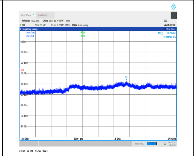
1-N41-30-100-M-1-DFT-PI2BPSK-Inner_1RB_Left-1 @ 1-12000-27000-Ant3-22198.50--36.79--25-PASS
