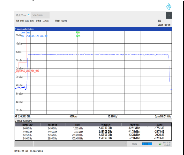
1-N41-30-100-L-3-DFT-PI2BPSK-Outer_Full-270@0-Ant3-1--PASS-see graph
