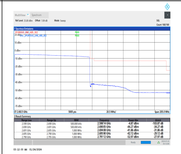
1-N41-30-100-H-6-CP-QPSK-Outer_Full-273@0-Ant3-1--PASS-see graph
