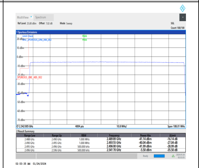
1-N41-30-100-L-6-CP-QPSK-Outer_Full-273@0-Ant3-1--PASS-see graph
