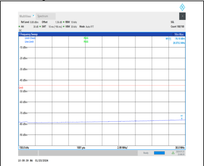
1-N41-30-100-H-1-DFT-PI2BPSK-Inner_1RB_Left-1 @ 1-0.15-30-Ant3-29.37--76.10--45-PASS
