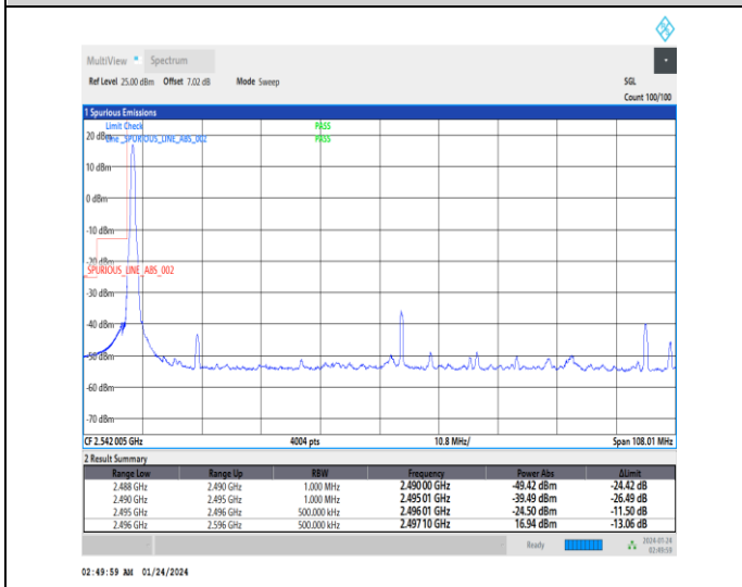
1-N41-30-100-L-4-CP-QPSK-Edge_1RB_Left-1@0-Ant3-1--PASS-see graph
