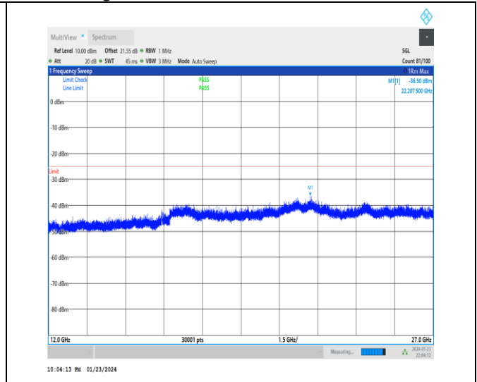
1-N41-30-100-L-1-DFT-PI2BPSK-Inner_1RB_Left-1 @ 1-12000-27000-Ant3-22207.50--36.50--25-PASS
