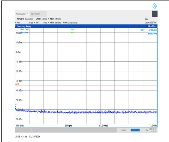
1-N41-30-100-M-1-DFT-PI2BPSK-Inner_1RB_Left-1 @ 1-30-1000-Ant3-33.88--57.93--35-PASS
