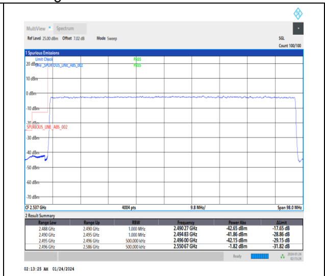
1-N41-30-90-L-3-DFT-PI2BPSK-Outer_Full-240@0-Ant3-1--PASS-see graph
