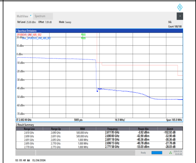
1-N41-30-80-H-6-CP-QPSK-Outer_Full-217@0-Ant3-1--PASS-see graph
