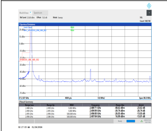
1-N41-30-90-L-4-CP-QPSK-Edge_1RB_Left-1@0-Ant3-1--PASS-see graph
