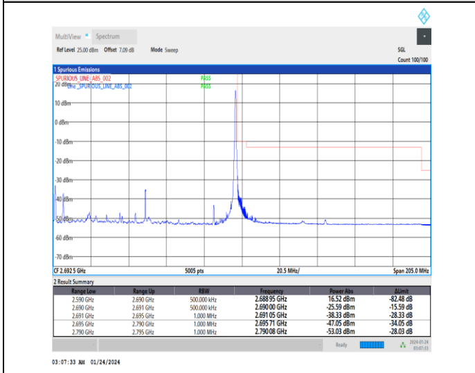
1-N41-30-100-H-5-CP-QPSK-Edge_1RB_Right-1 @272 -Ant3-1--PASS-see graph
