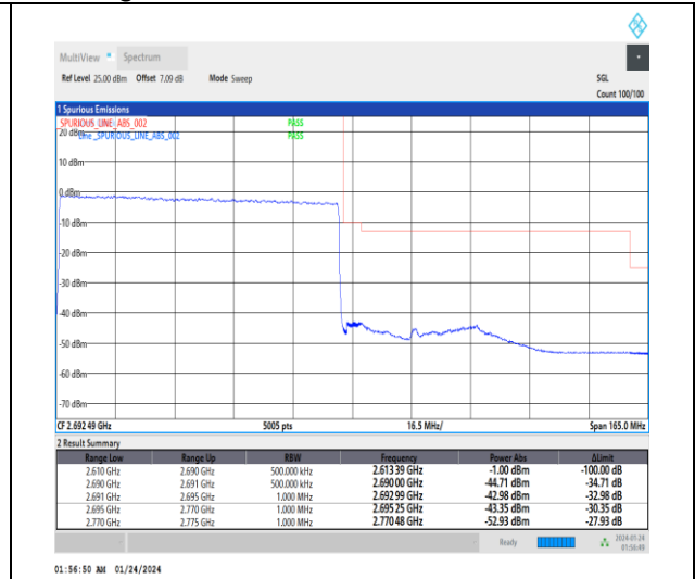
1-N41-30-80-H-3-DFT-PI2BPSK-Outer_Full-216@0-Ant3-1--PASS-see graph
