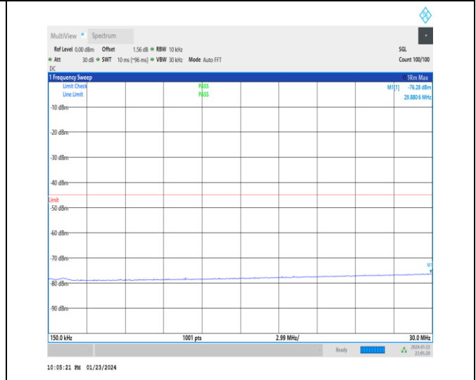
1-N41-30-100-M-1-DFT-PI2BPSK-Inner_1RB_Left-1 @ 1-0.15-30-Ant3-29.88--76.28--45-PASS
