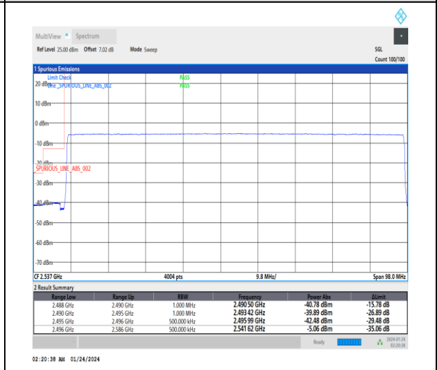
1-N41-30-90-L-6-CP-QPSK-Outer_Full-245@0-Ant3-1--PASS-see graph
