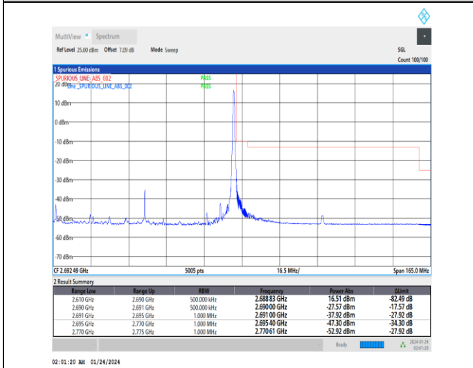
1-N41-30-80-H-5-CP-QPSK-Edge_1RB_Right-1@216-Ant3-1--PASS-see graph
