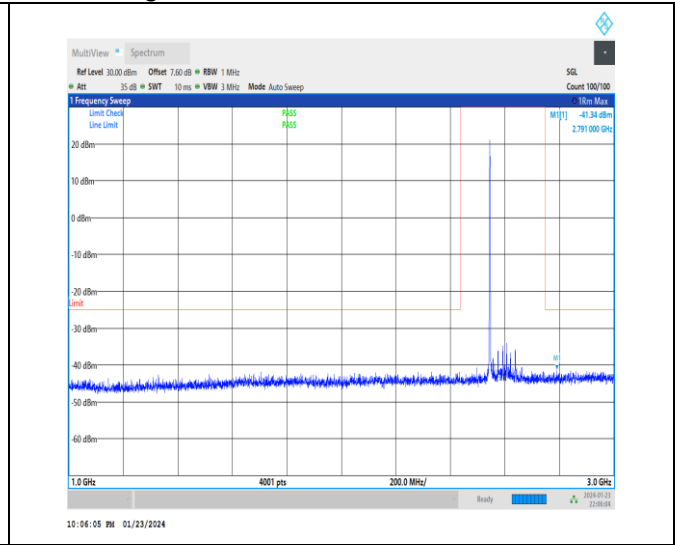
1-N41-30-100-M-1-DFT-PI2BPSK-Inner_1RB_Left-1 @ 1-1000-3000-Ant3-2791.00--41.34--25-PASS
