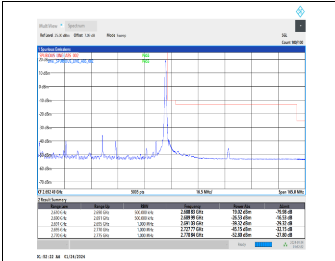
1-N41-30-80-H-2-DFT-PI2BPSK-Edge_1RB_Right-1@216-Ant3-1--PASS-see graph
