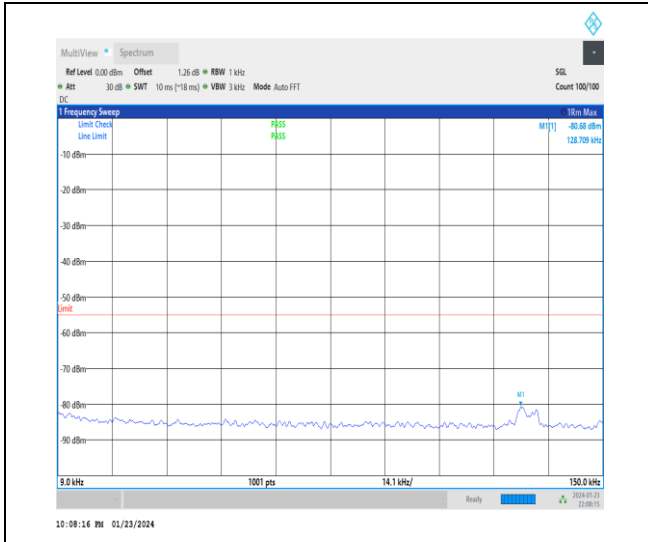
1-N41-30-100-H-1-DFT-PI2BPSK-Inner_1RB_Left-1 @ 1-0.009-0.15-Ant3-0.13--80.68--55-PASS
