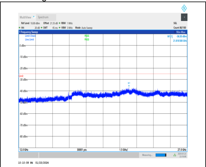
1-N41-30-100-H-1-DFT-PI2BPSK-Inner_1RB_Left-1 @ 1-12000-27000-Ant3-21818.50--36.50--25-PASS
