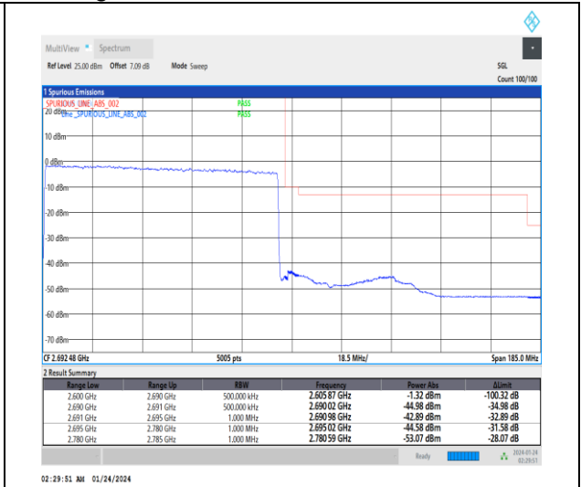
1-N41-30-90-H-3-DFT-PI2BPSK-Outer_Full-240@0-Ant3-1--PASS-see graph
