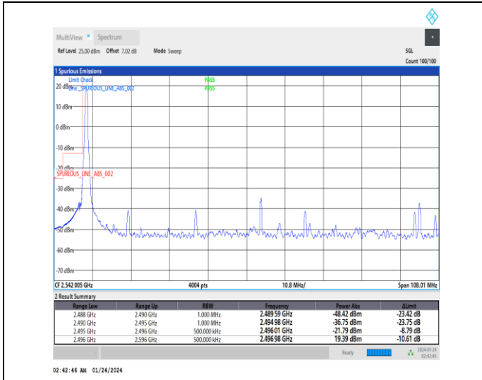
1-N41-30-100-L-1-DFT-PI2BPSK-Edge_1RB_Left-1@0-Ant3-1--PASS-see graph
