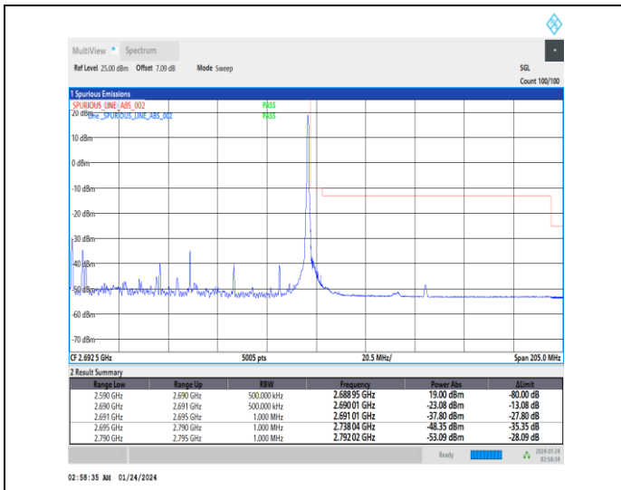
1-N41-30-100-H-2-DFT-PI2BPSK-Edge_1RB_Right-1 @272-Ant3-1--PASS-see graph
