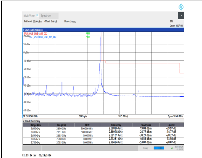
1-N41-30-90-H-2-DFT-PI2BPSK-Edge_1RB_Right-1@244-Ant3-1--PASS-see graph
