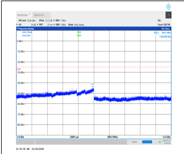
1-N41-30-100-L-1-DFT-PI2BPSK-Inner_1RB_Left-1 @ 1-3000-12000-Ant3-7432.50--44.61--25-PASS
