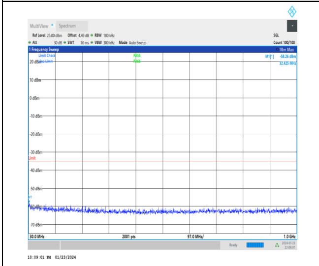
1-N41-30-100-H-1-DFT-PI2BPSK-Inner_1RB_Left-1 @ 1-30-1000-Ant3-32.43--58.26--35-PASS
