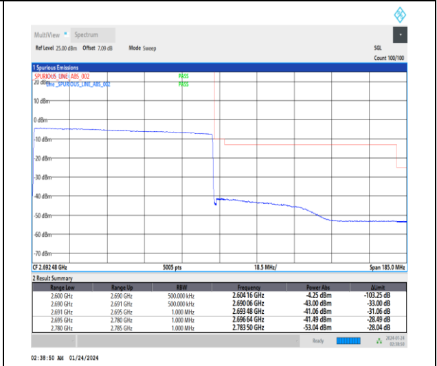
1-N41-30-90-H-6-CP-QPSK-Outer_Full-245@0-Ant3-1--PASS-see graph
