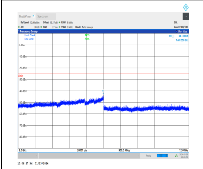
1-N41-30-100-M-1-DFT-PI2BPSK-Inner_1RB_Left-1 @ 1-3000-12000-Ant3-7481.55--43.18--25-PASS
