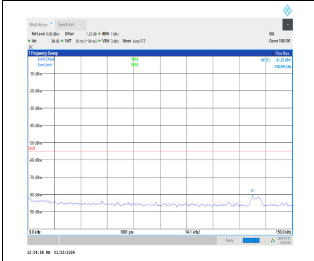
1-N41-30-100-M-1-DFT-PI2BPSK-Inner_1RB_Left-1 @ 1-0.009-0.15-Ant3-0.13--81.22--55-PASS
