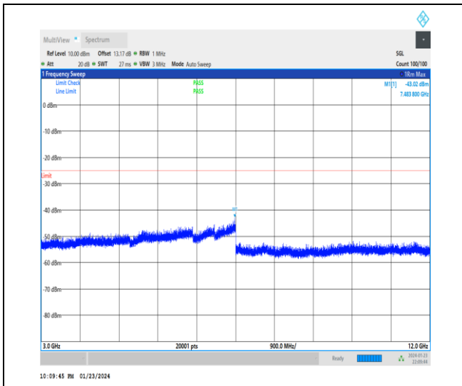
1-N41-30-100-H-1-DFT-PI2BPSK-Inner_1RB_Left-1 @ 1-3000-12000-Ant3-7483.80--43.02--25-PASS
