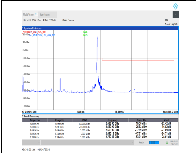
1-N41-30-90-H-5-CP-QPSK-Edge_1RB_Right-1@244-Ant3-1--PASS-see graph
