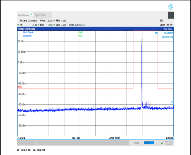
1-N41-30-100-H-1-DFT-PI2BPSK-Inner_1RB_Left-1 @ 1-1000-3000-Ant3-2997.50--40.92--25-PASS
