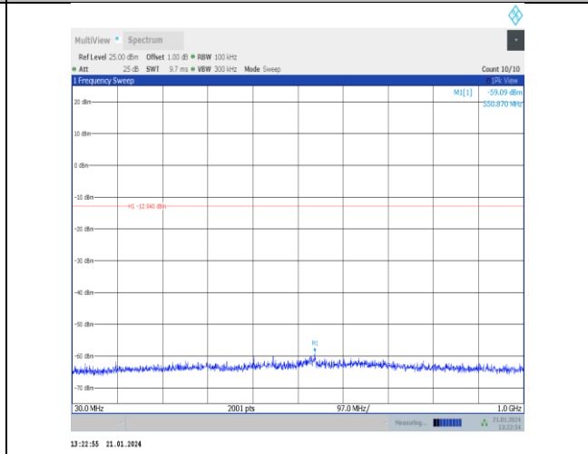
11n20SISO-Ant5-2457-30~1000-PASS
