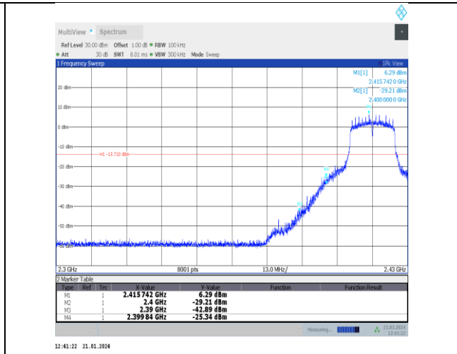
11g-Ant5-2417-PASS
