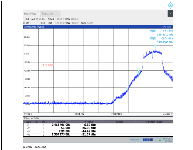
11g-Ant5-2412-PASS
