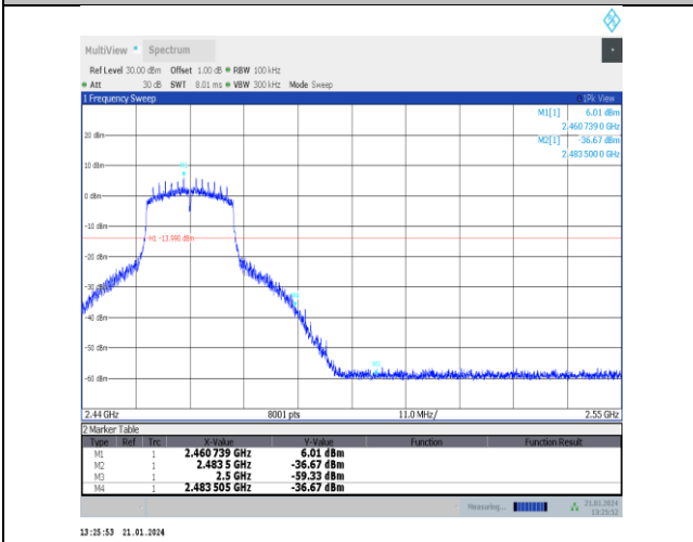
11n20SISO-Ant5-2462-PASS
