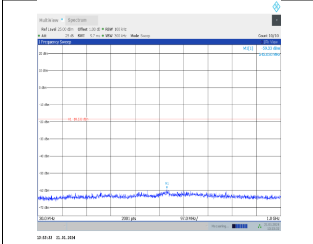
11n40SISO-Ant5-2427-30~1000-PASS
