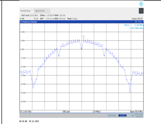
11b-Ant5-2437-0~Reference-PASS
