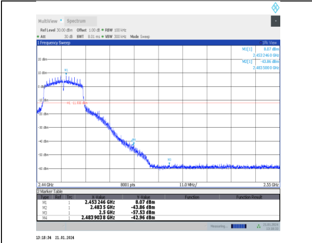
11n20SISO-Ant5-2452-PASS
