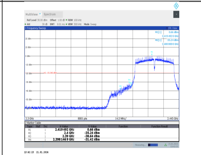
11n40SISO-Ant5-2422-PASS
