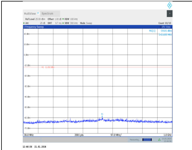
11g-Ant5-2422-30~1000-PASS
