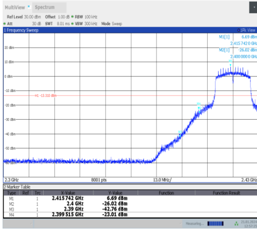
11n20SISO-Ant5-2417-PASS
