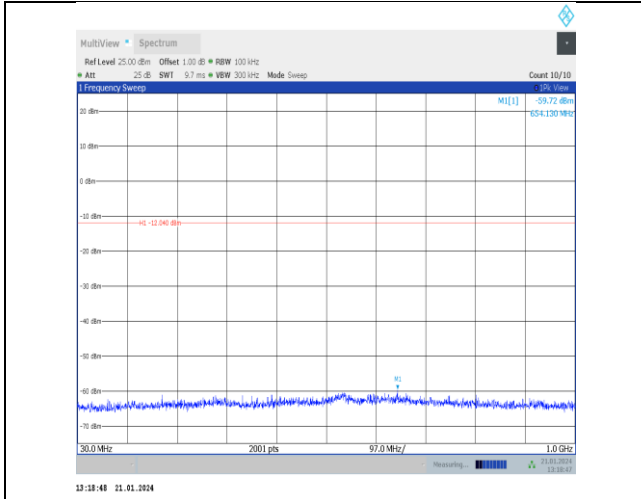
11n20SISO-Ant5-2452-30~1000-PASS
