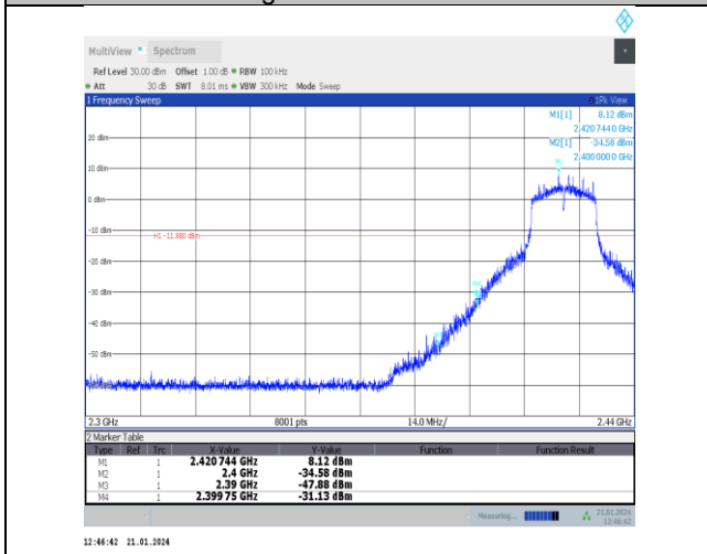
11g-Ant5-2422-PASS
