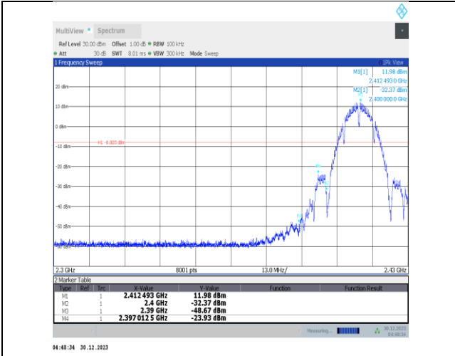
11b-Ant5-2412-PASS
