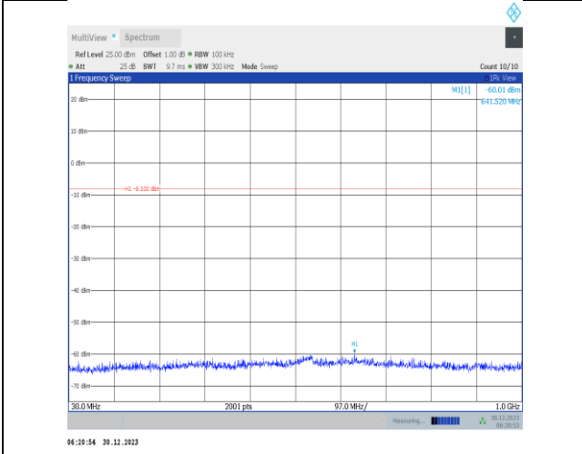
11b-Ant5-2437-30~1000-PASS
