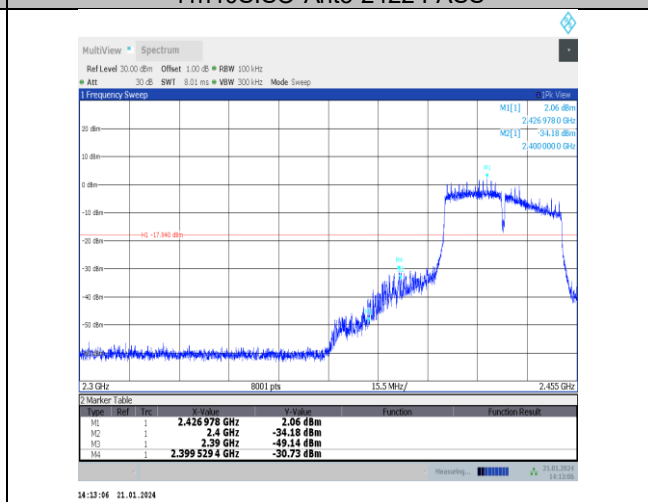
11n40SISO-Ant5-2422-PASS
