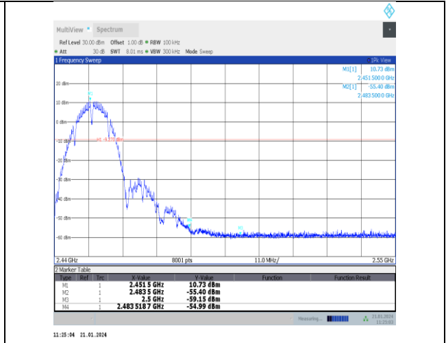
11b-Ant5-2452-PASS
