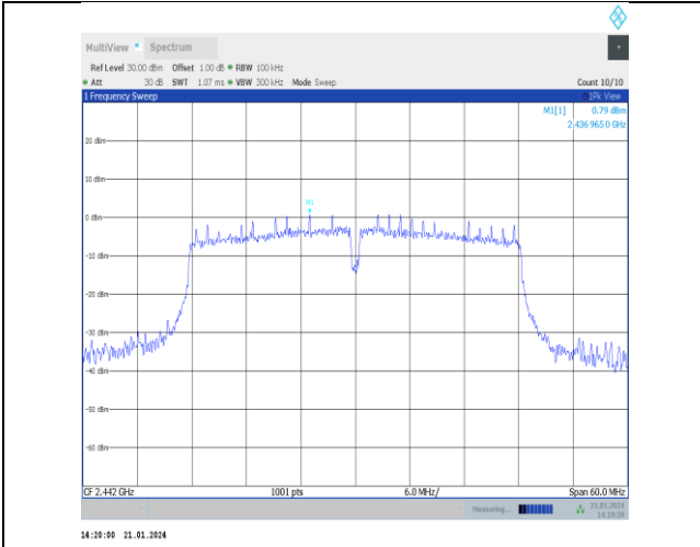
11n40ISO-Ant5-2442-0~Reference-PASS
