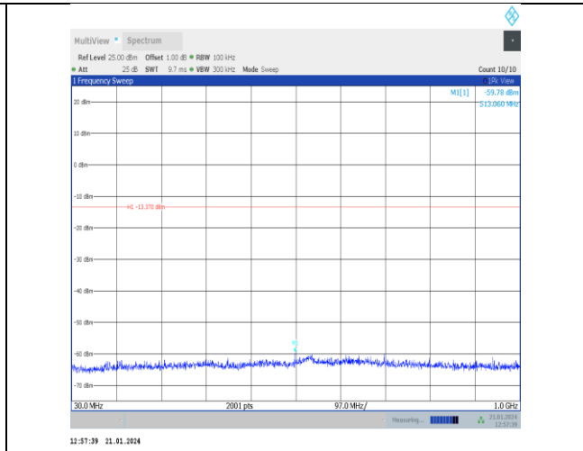
11n20SISO-Ant5-2417-30~1000-PASS
