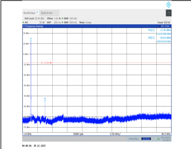
11b-Ant5-2412-1000~26500-PASS
