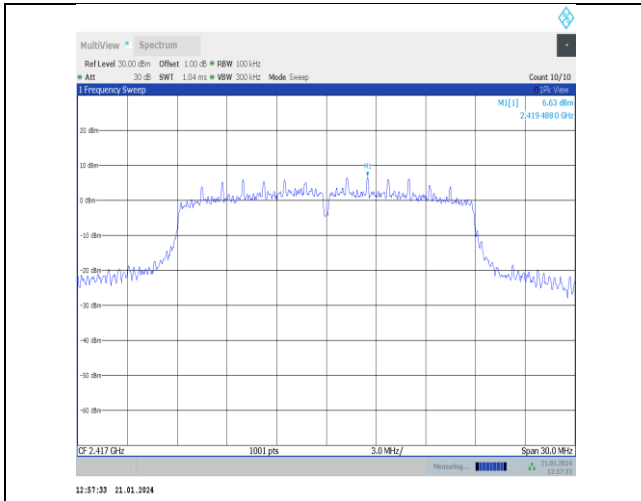
11n20SISO-Ant5-2417-0~Reference-PASS
