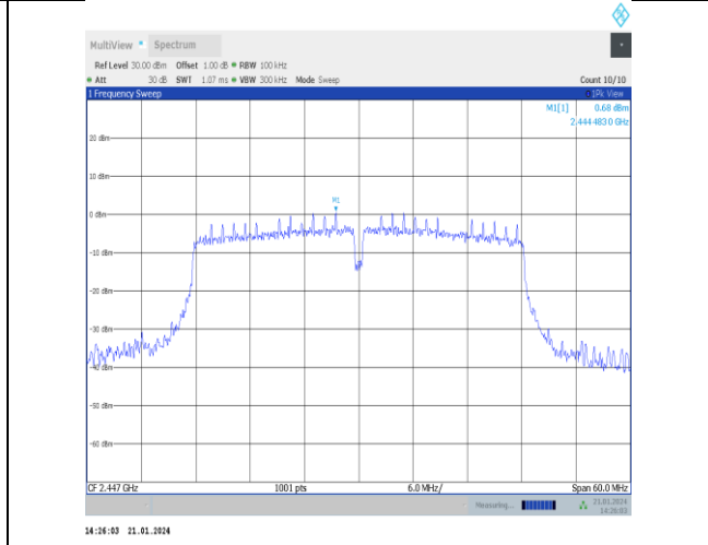
11n40ISO-Ant5-2447-0~Reference-PASS
