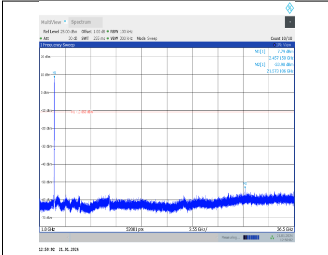
11g-Ant5-2452-1000~26500-PASS
