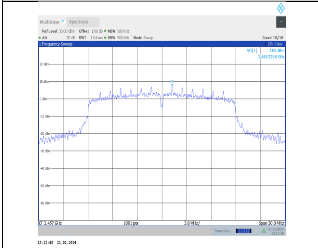
11n20SISO-Ant5-2457-0~Reference-PASS
