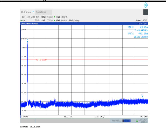
11g-Ant5-2412-0~Reference-PASS
