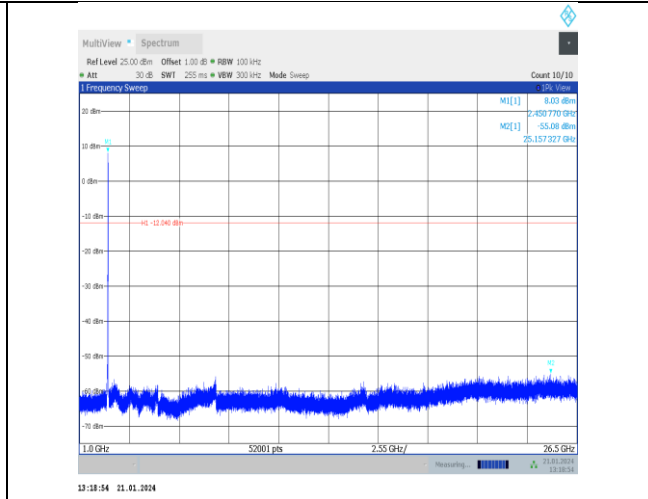
11n20SISO-Ant5-2452-1000~26500-PASS
