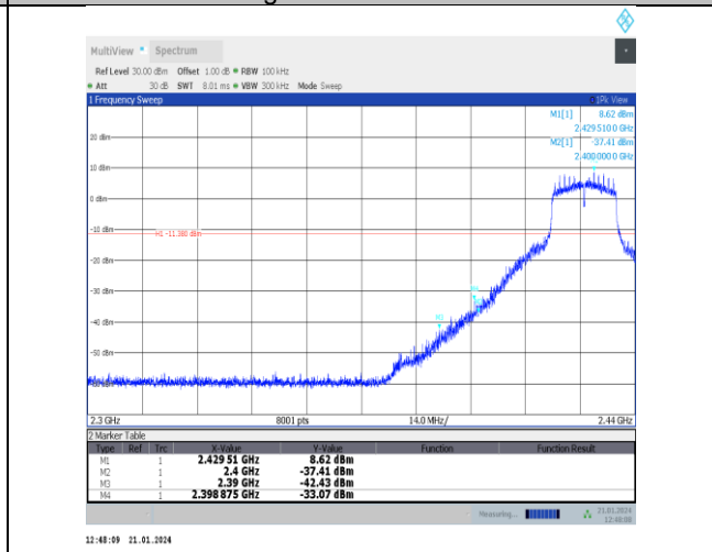
11g-Ant5-2427-PASS
