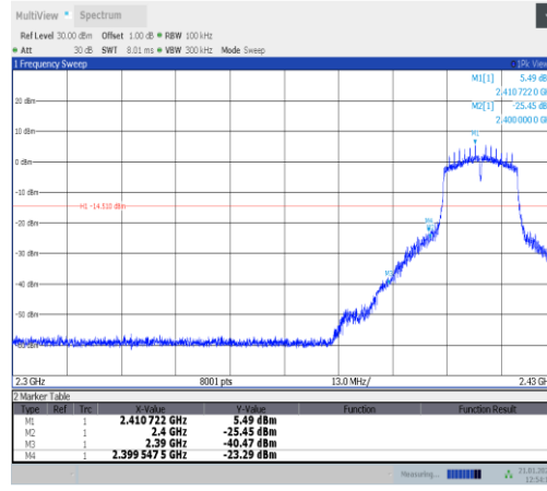
11n20SISO-Ant5-2412-PASS
