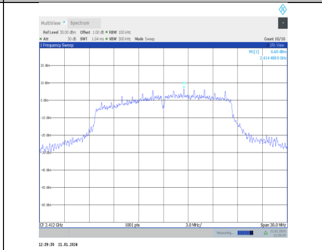
11g-Ant5-2412-0~Reference-PASS
