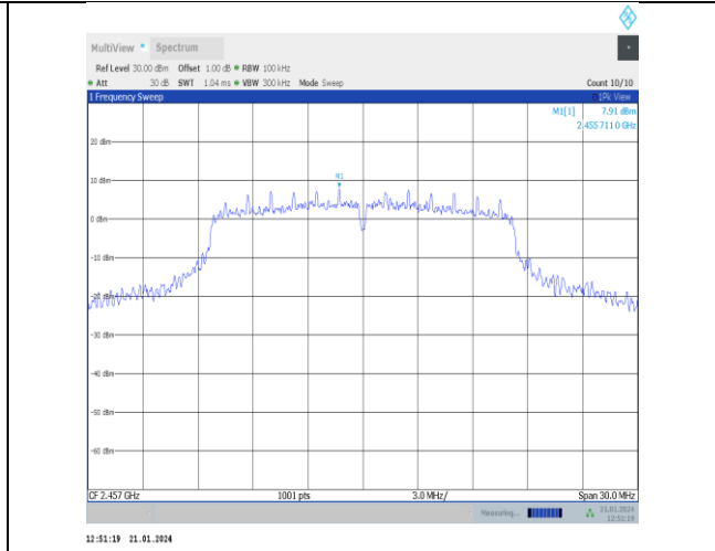
11g-Ant5-2457-0~Reference-PASS
