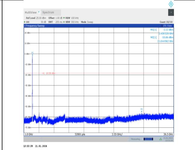
11n40SISO-Ant5-2427-1000~26500-PASS
