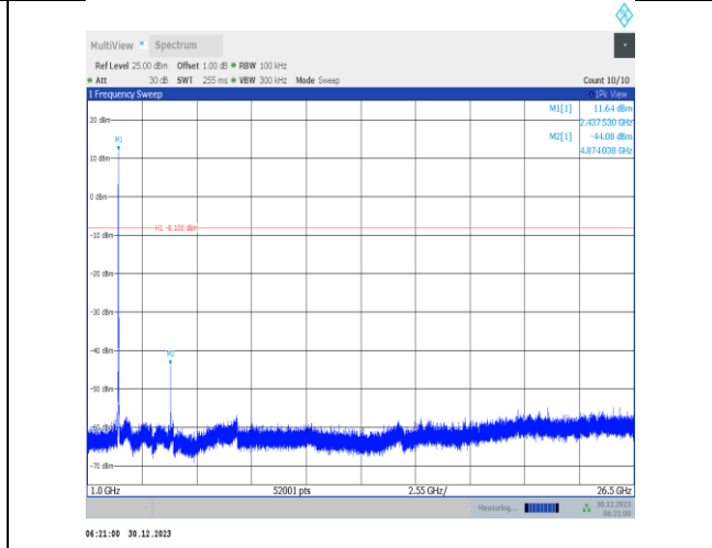
11b-Ant5-2437-1000~26500-PASS
