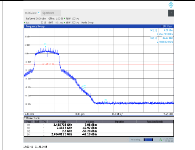
11n20SISO-Ant5-2457-PASS
