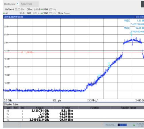
11n20SISO-Ant5-2422-PASS
