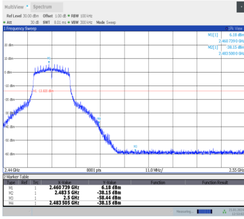
11g-Ant5-2462-PASS
