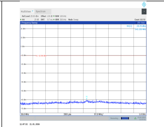
11b-Ant5-2462-30~1000-PASS
