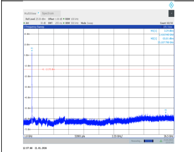
11n20SISO-Ant5-2417-1000~26500-PASS
