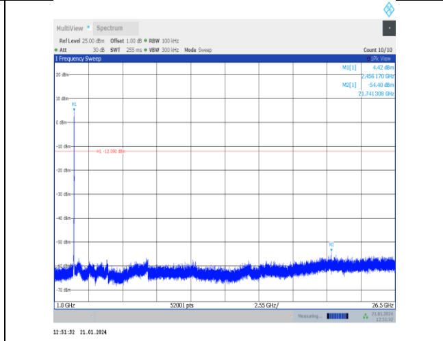
11g-Ant5-2457-1000~26500-PASS
