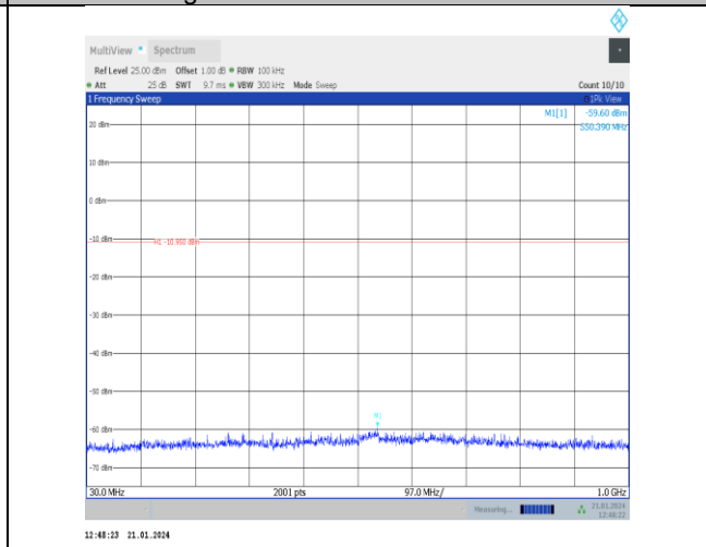
11g-Ant5-2427-30~1000-PASS
