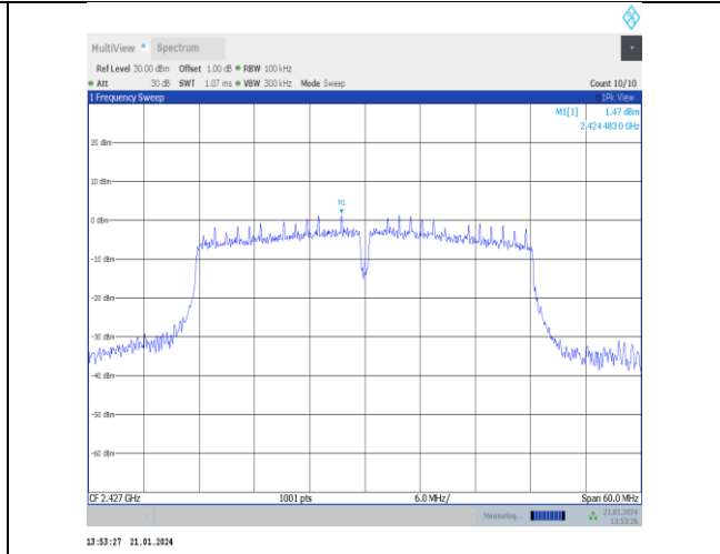
11n40SISO-Ant5-2427-0~Reference-PASS
