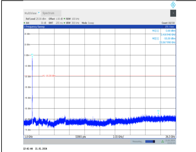
11n40SISO-Ant5-2422-1000~26500-PASS
