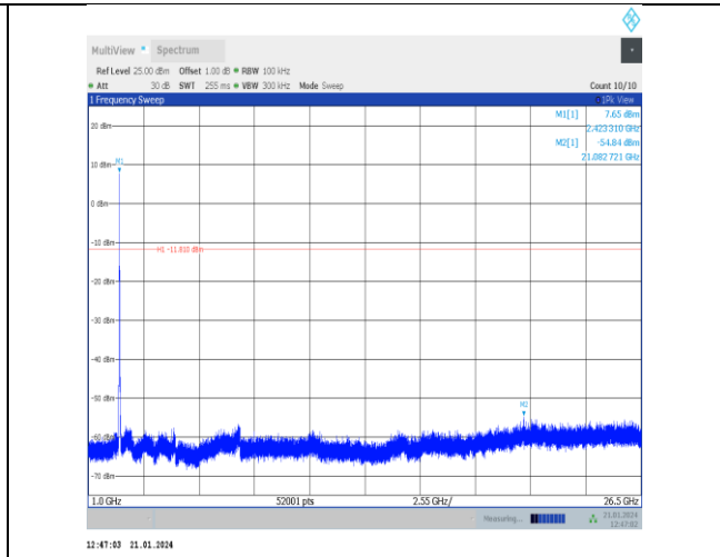
11g-Ant5-2422-1000~26500-PASS
