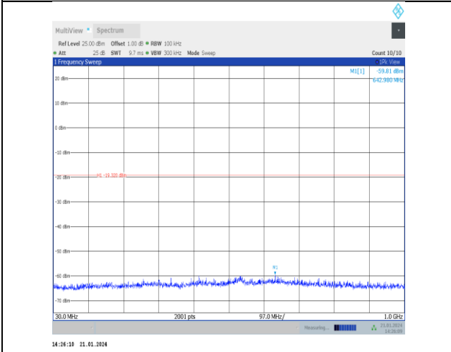
11n40ISO-Ant5-2447-0~Reference-PASS
