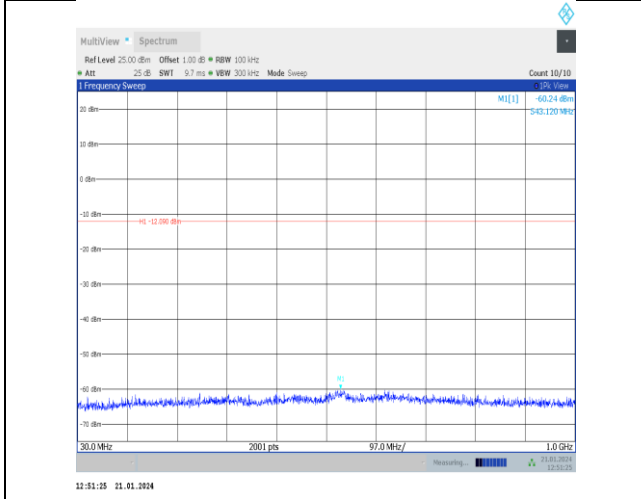
11g-Ant5-2457-30~1000-PASS
