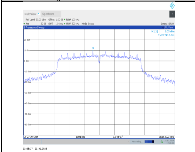
11g-Ant5-2427-0~Reference-PASS
