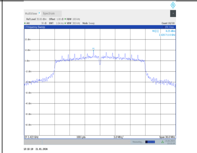
11n20SISO-Ant5-2422-0~Reference-PASS
